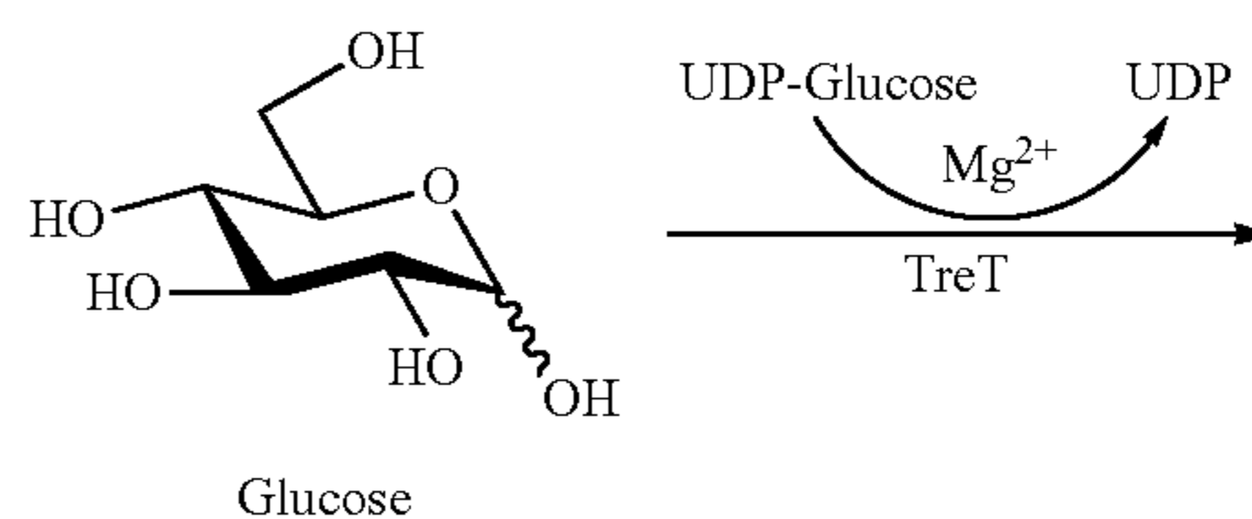
Scheme 1. Synthesis of trehalose from glucose (glc) and UDP-glucose (UDP-glc) by TreT from Thermoproteus tenax .
