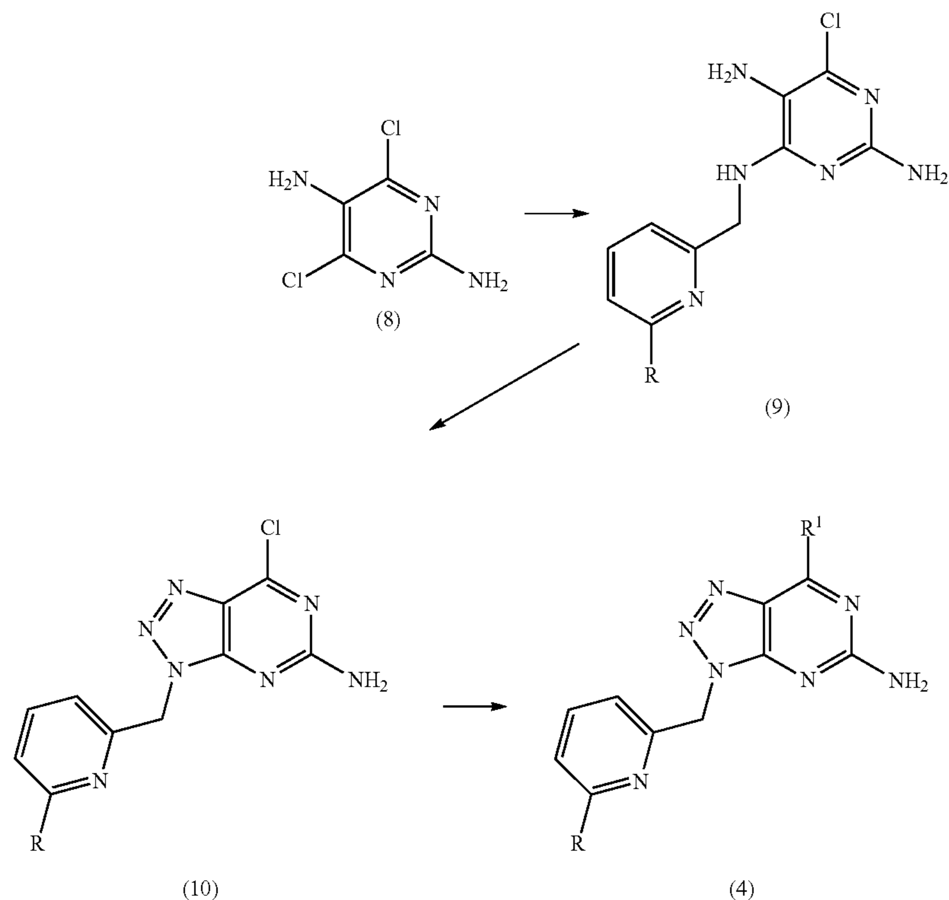
Reaction Scheme 2
