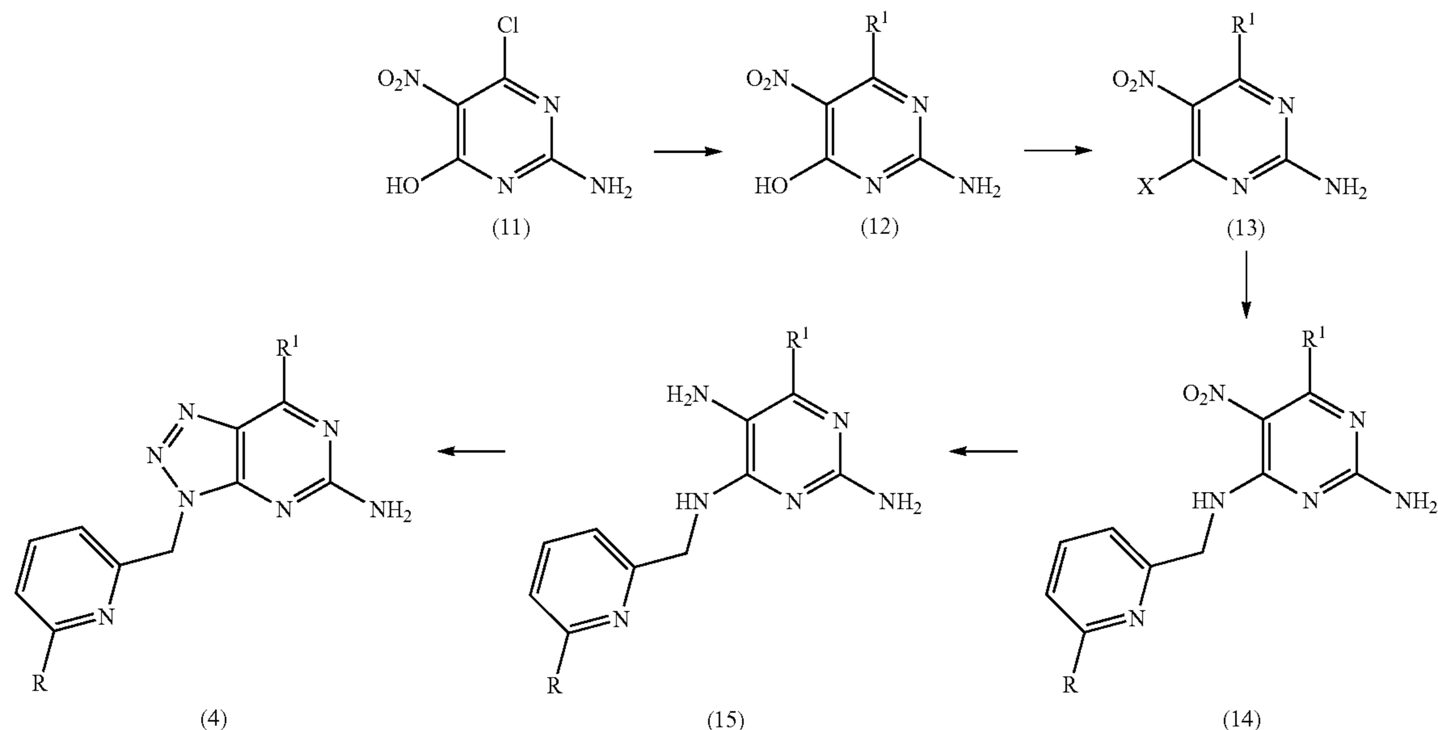
Reaction Scheme 3
