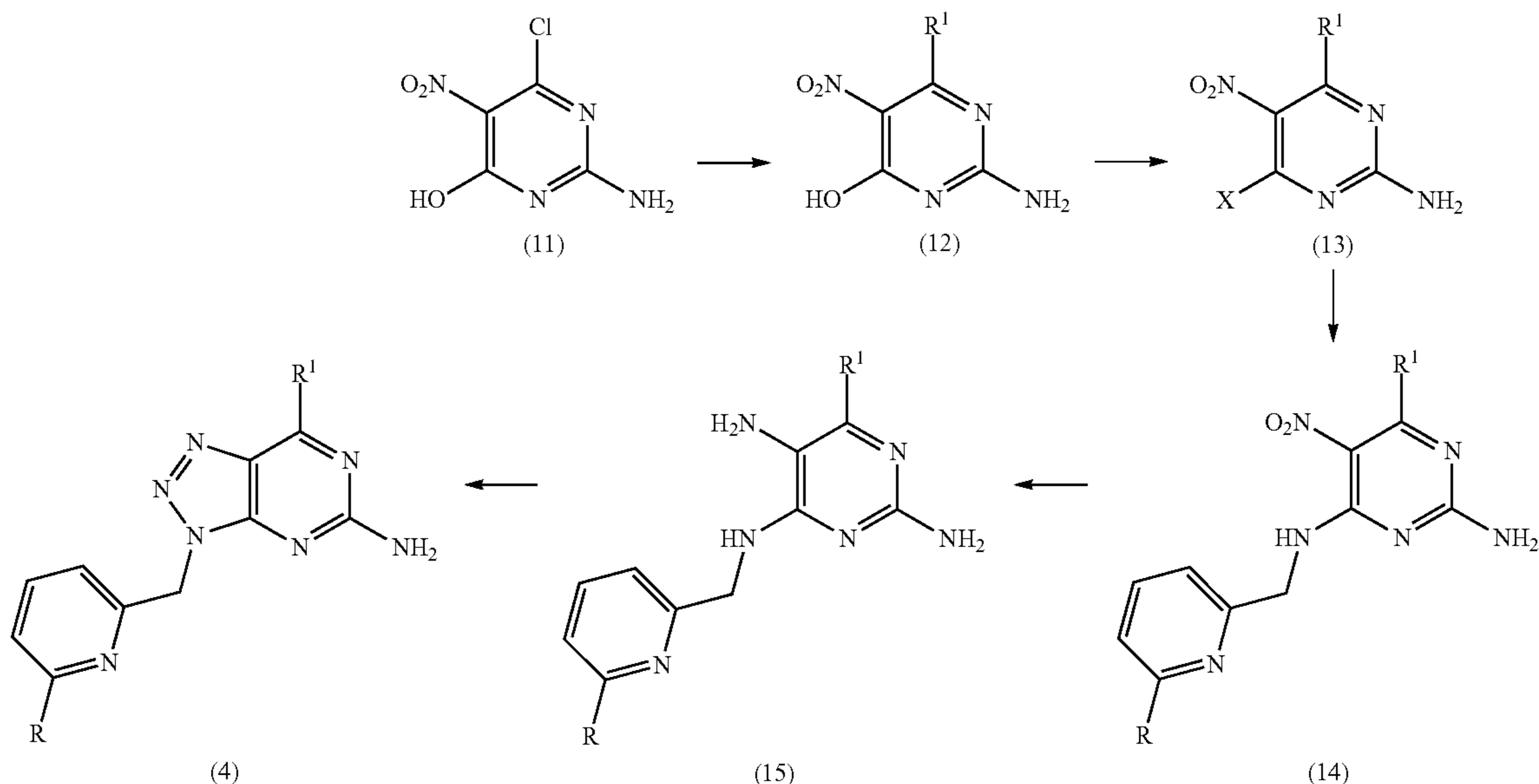
Reaction Scheme 3
