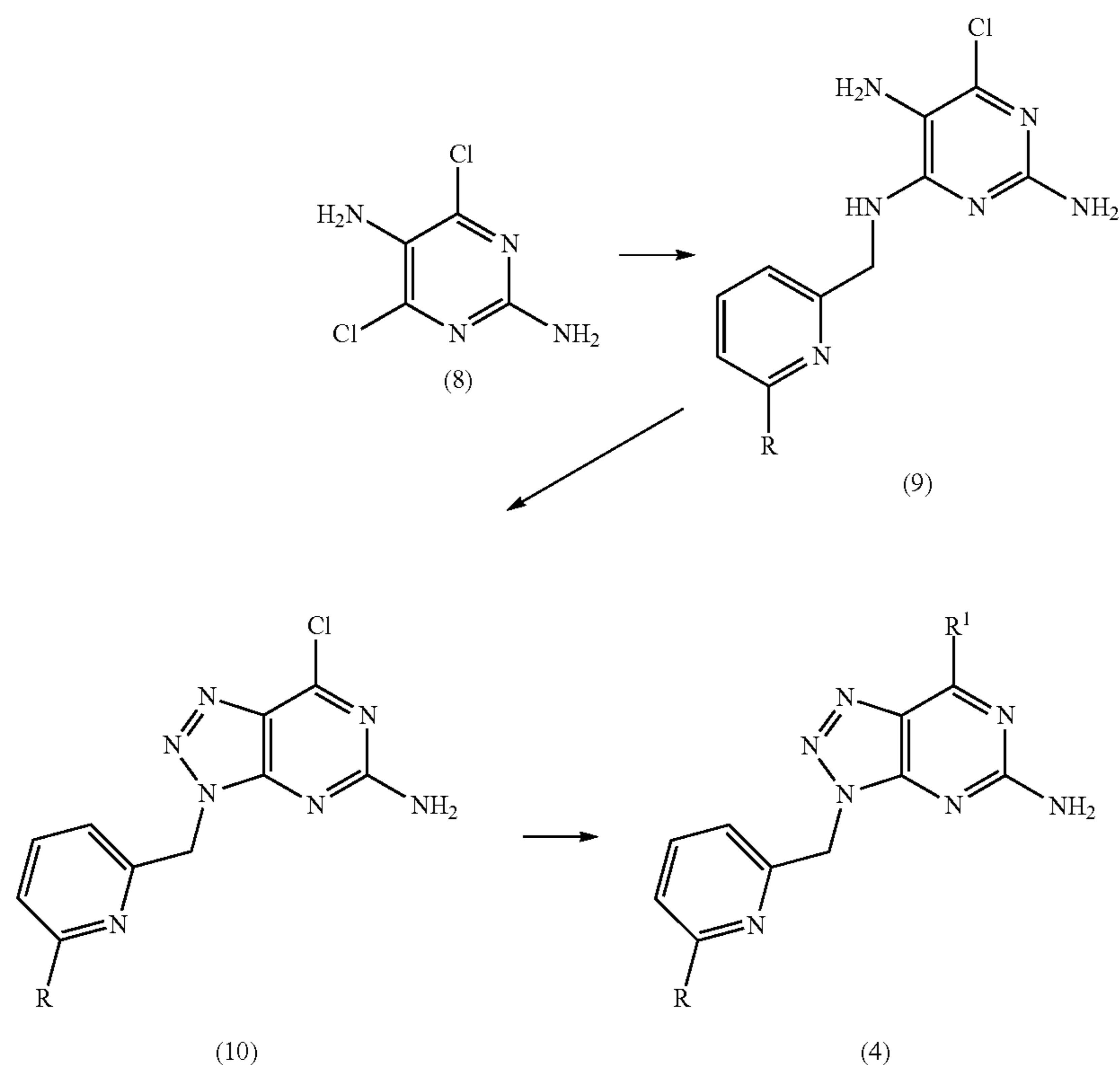
Reaction Scheme 2
