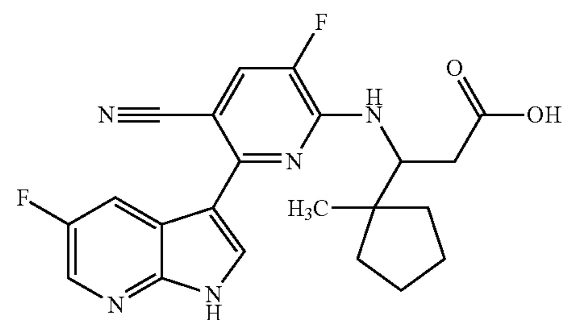
Compound 13
