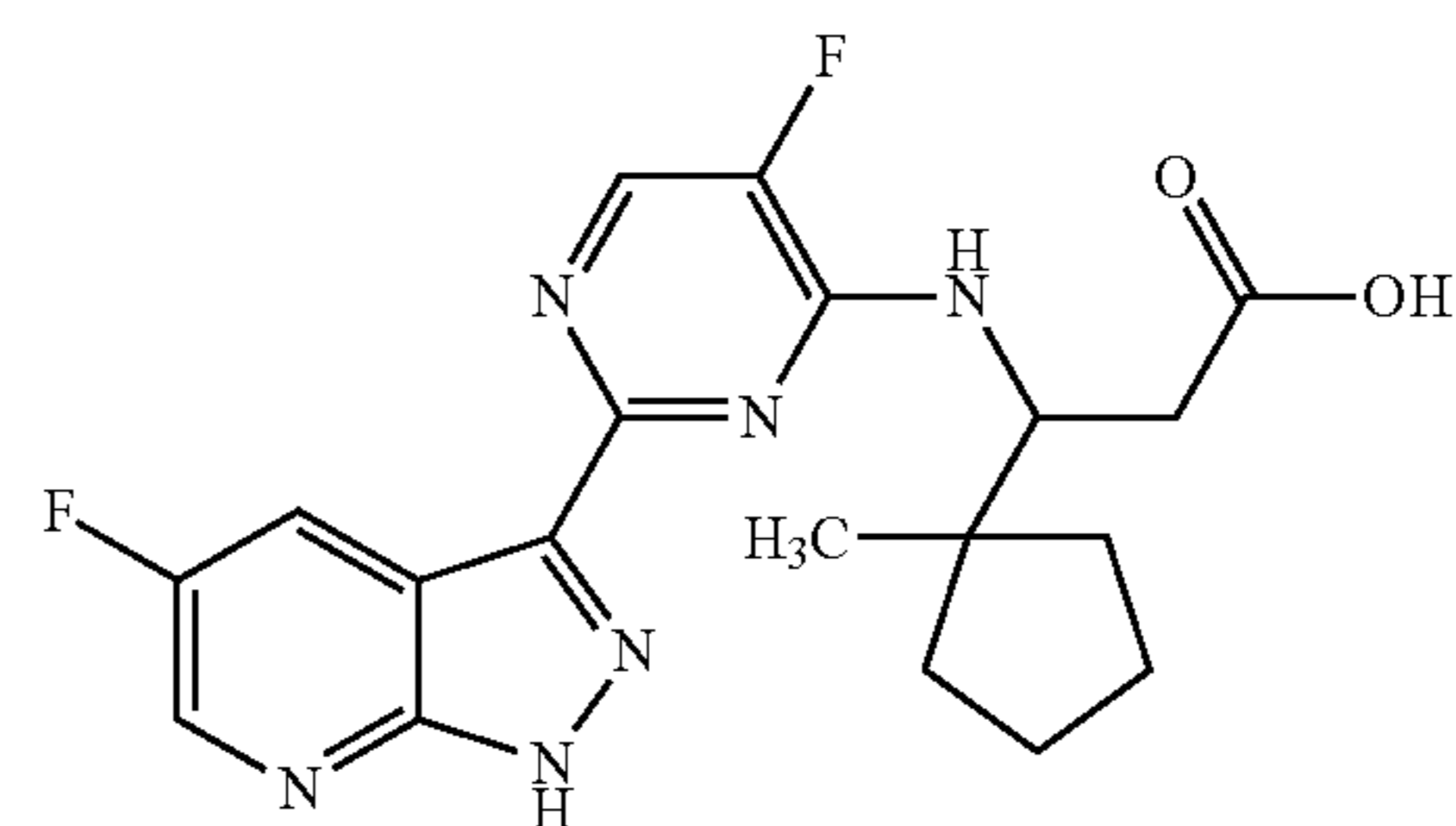
Compound 12
