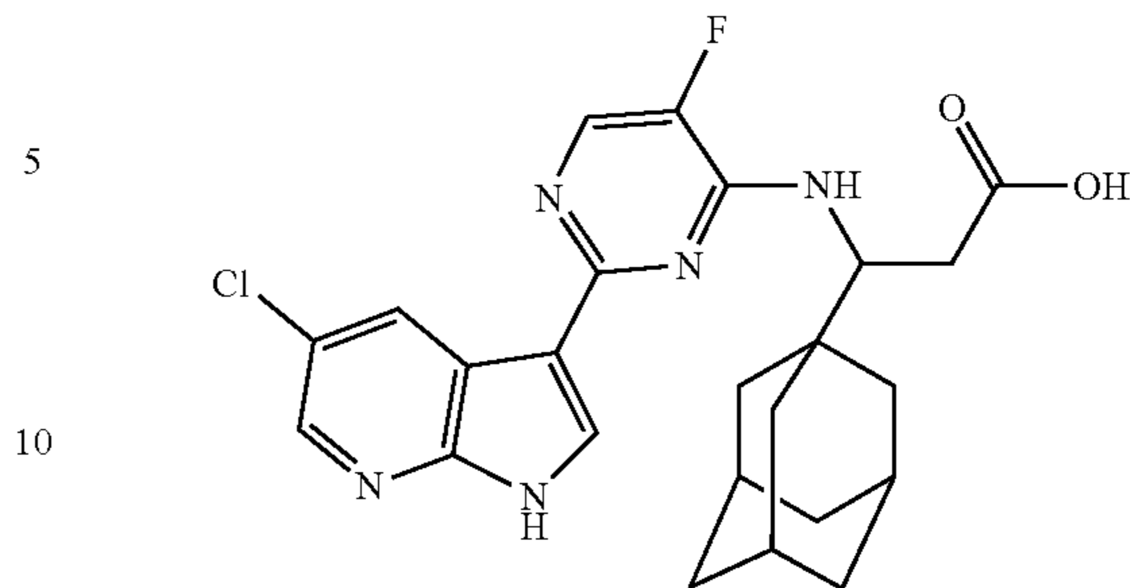
(+/-)-3-(1-Adamantyl)-3-[[2-(5-chloro-1H-pyrrolo[2,3-b]pyridin-3-yl)-5-fluoro-pyrimidin-4-yl]amino]propanoic acid (94)
