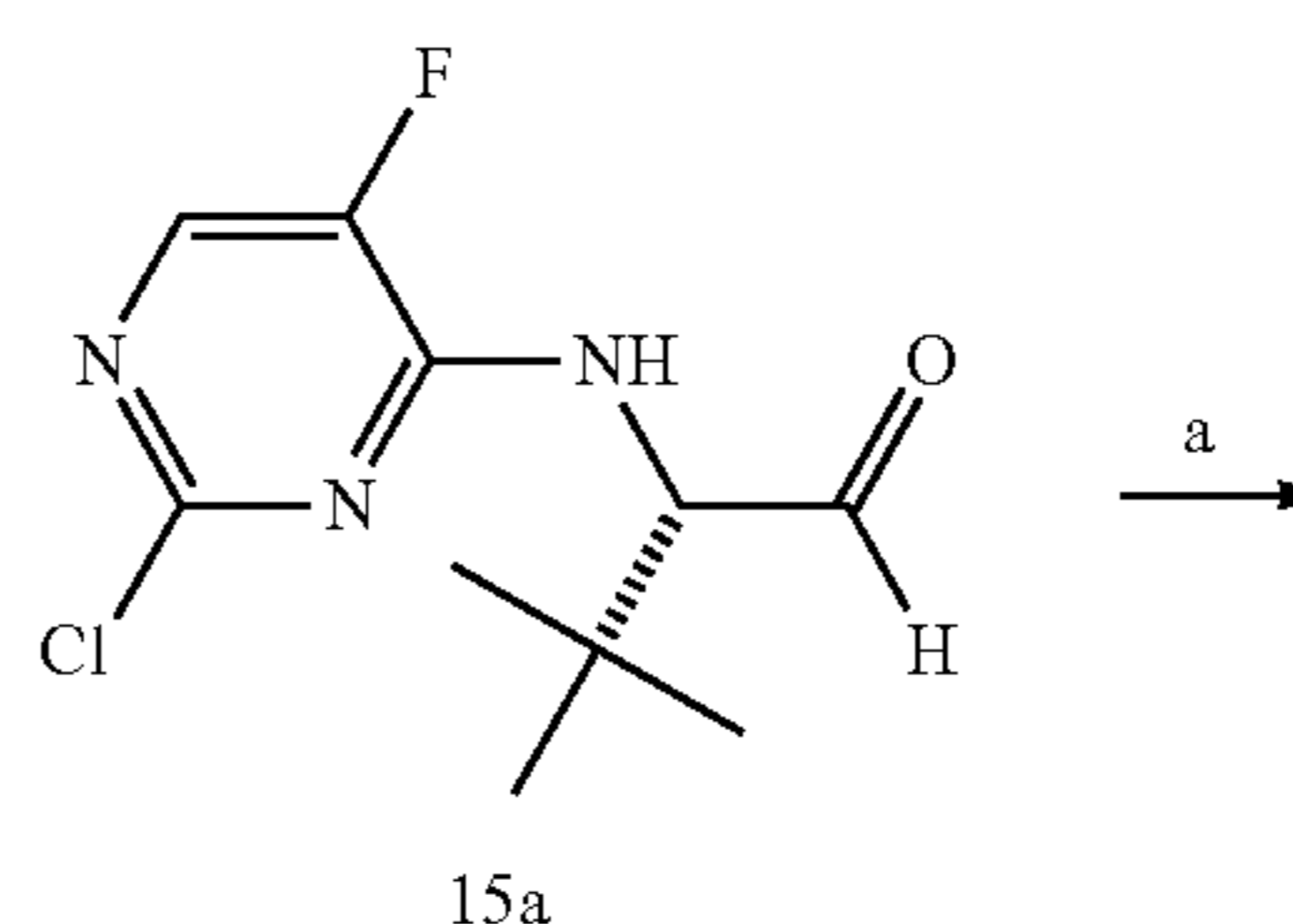
Synthetic Scheme 7
