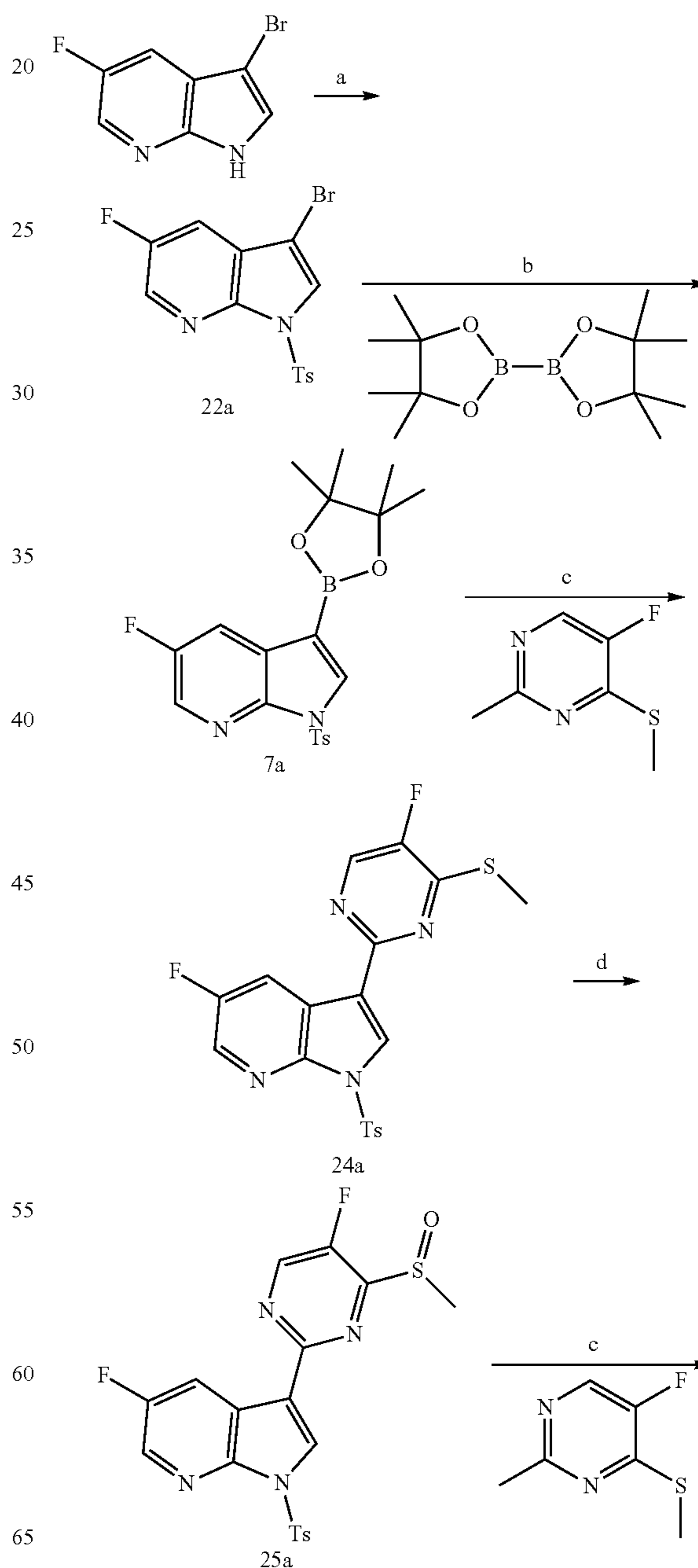
Synthetic Scheme 4
