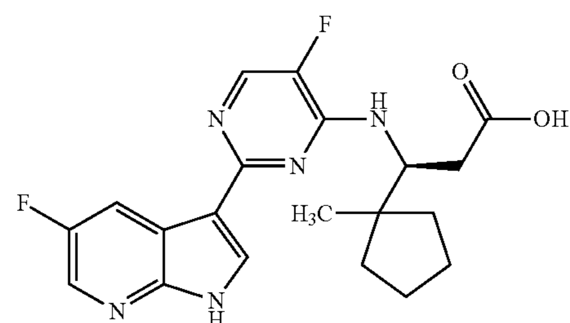
Compound 15
