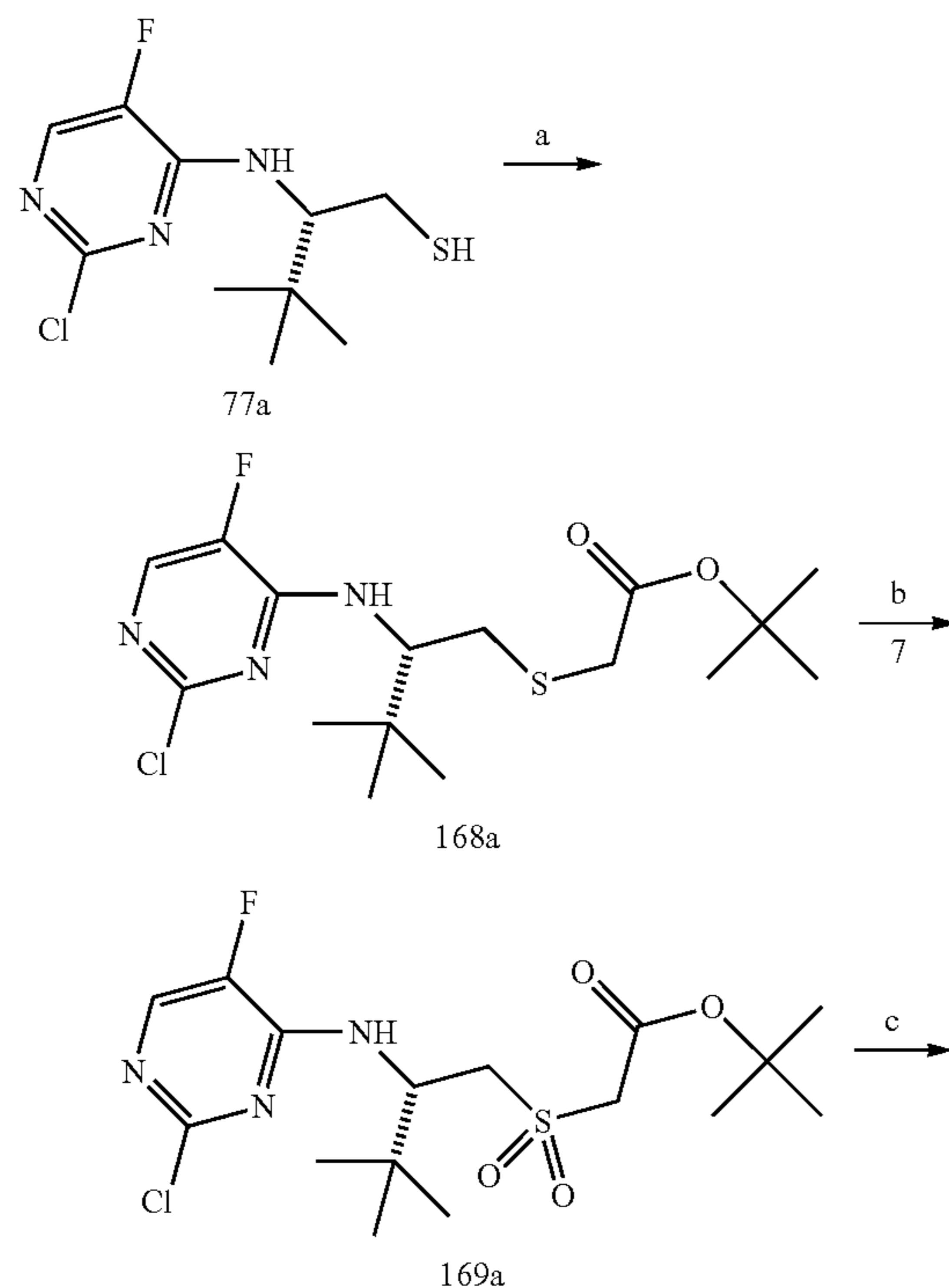
Synthetic Scheme 26
