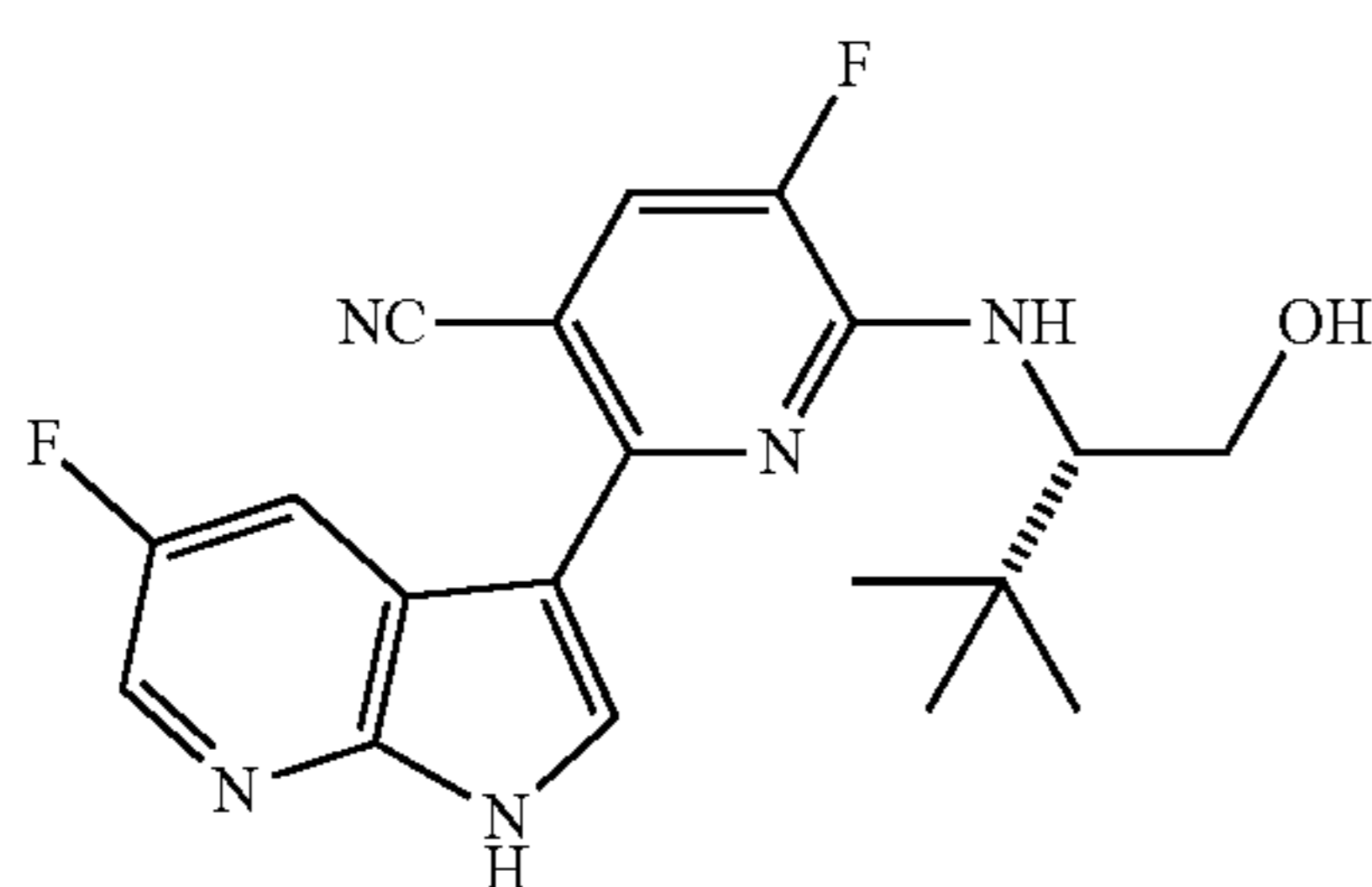
(S)-5-fluoro-2-(5-fluoro-1H-pyrrolo[2,3-b]pyridin-3-yl)-6-((1-hydroxy-3,3-dimethylbutan-2-yl)amino)nicotinonitrile (24)
