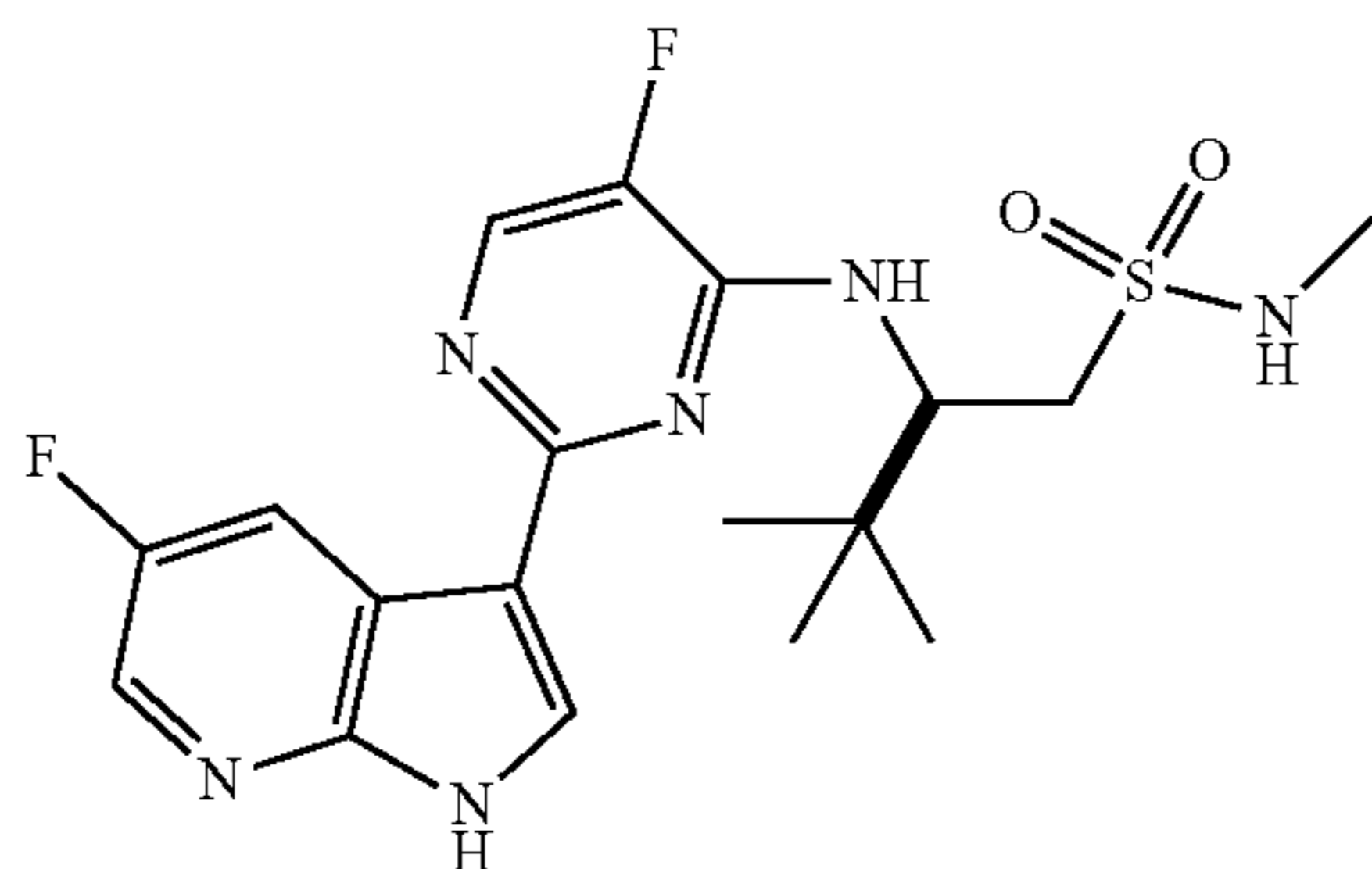
(R)-2-((5-fluoro-2-(5-fluoro-1H-pyrrolo[2,3-b]pyridin-3-yl)pyrimidin-4-yl)amino)-N,3,3-trimethylbutane-1-sulfonamide (38)
