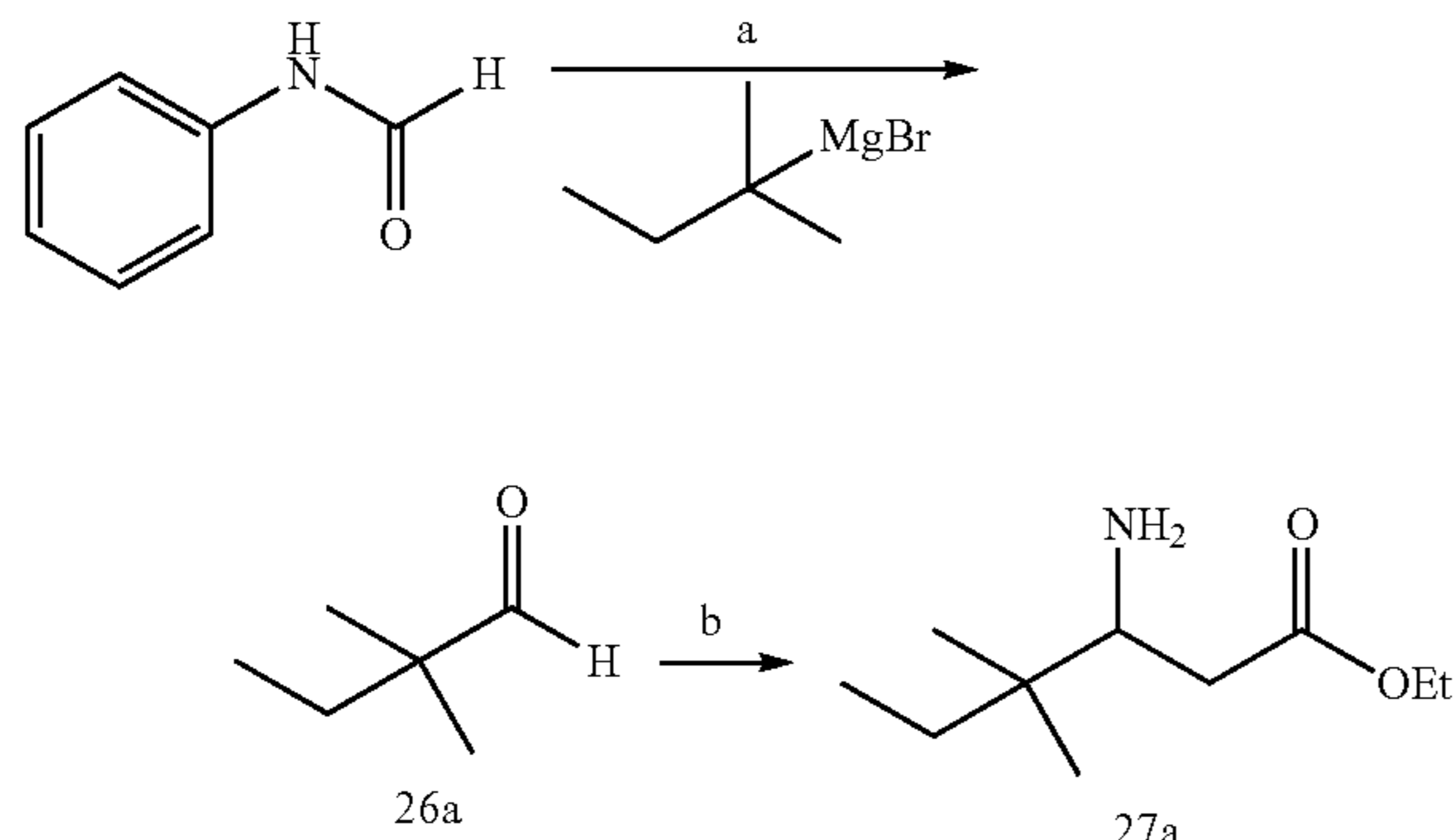
Synthetic Scheme 5
