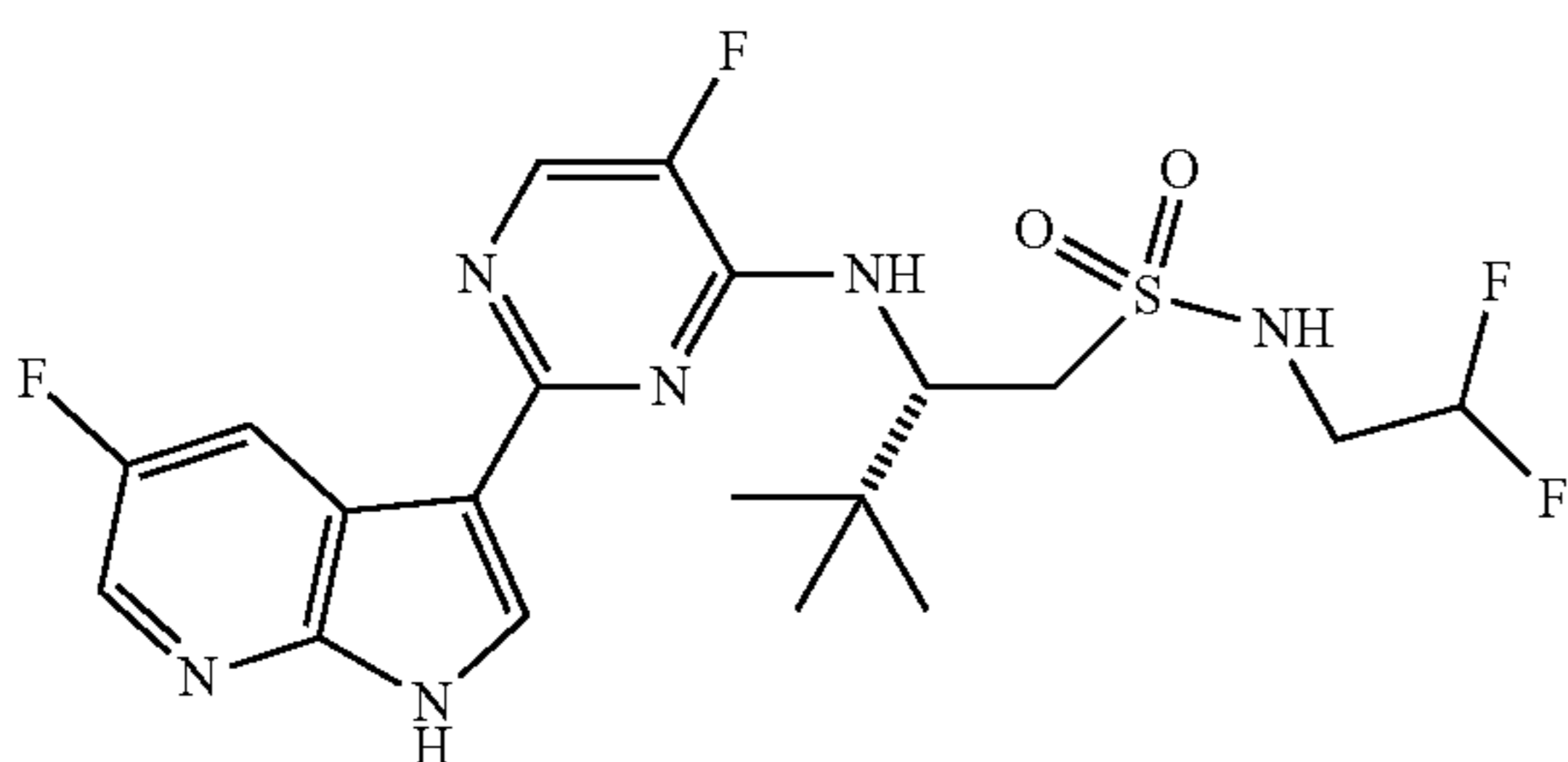
(S)-N-(2,2-difluoroethyl)-2-(5-fluoro-2-(5-fluoro-1H-pyrrolo[2,3-b]pyridin-3-yl)pyrimidin-4-ylamino)-3,3-dimethylbutane-1-sulfonamide (57)
