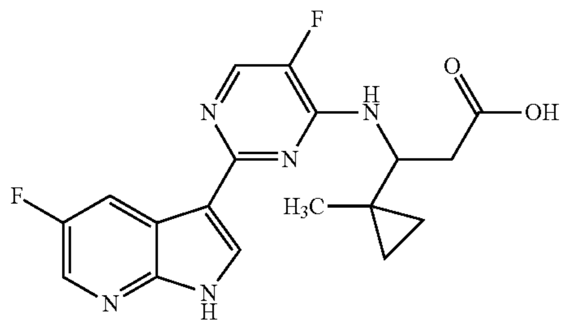
Compound 93
