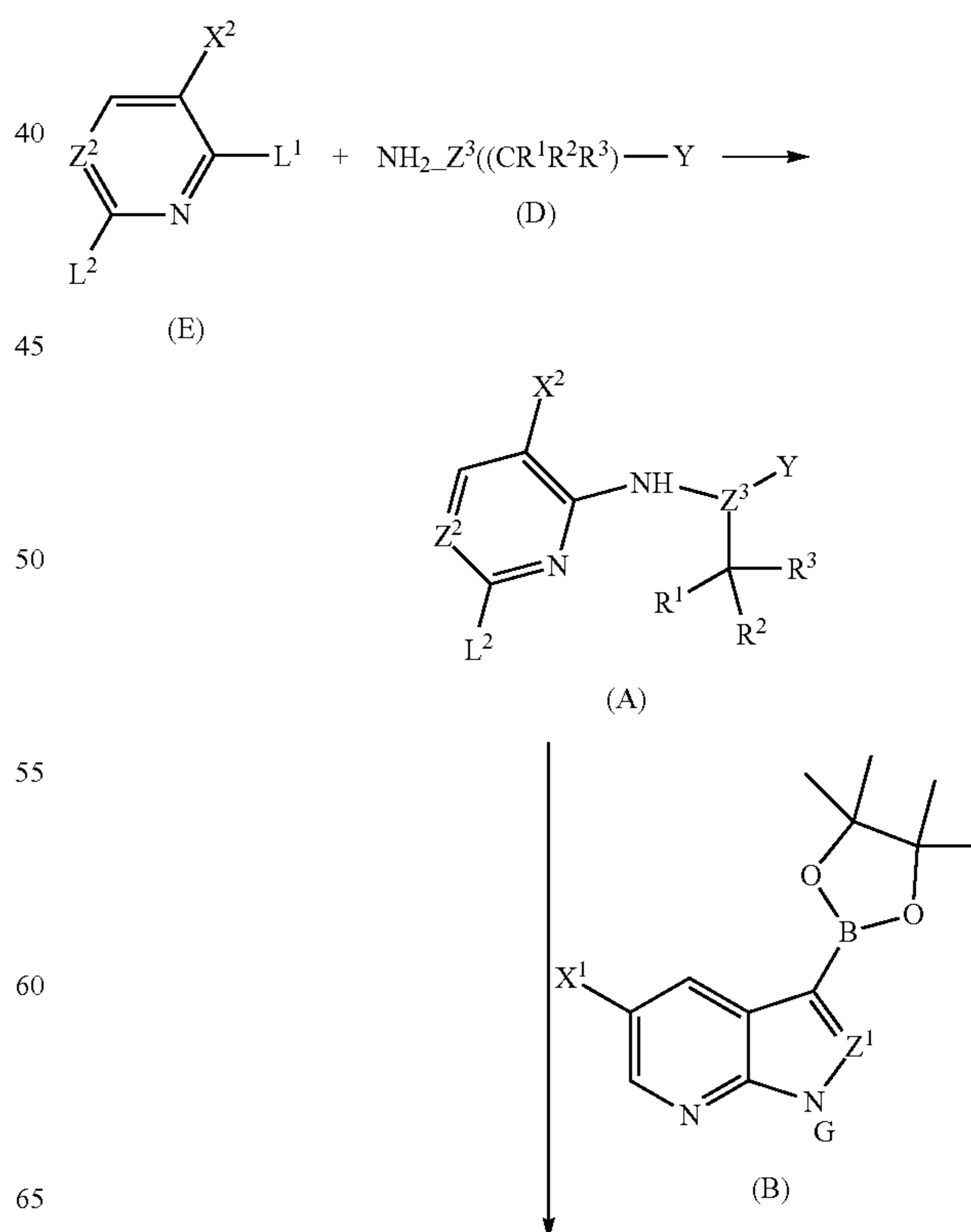
General Scheme 1
