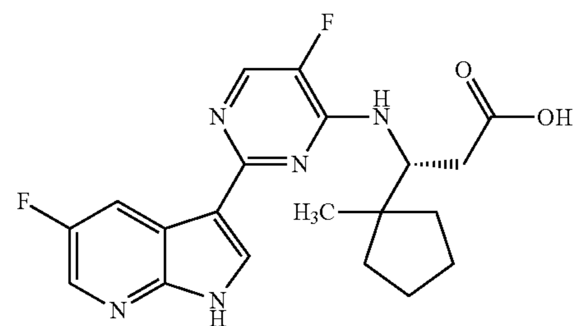
Compound 14
