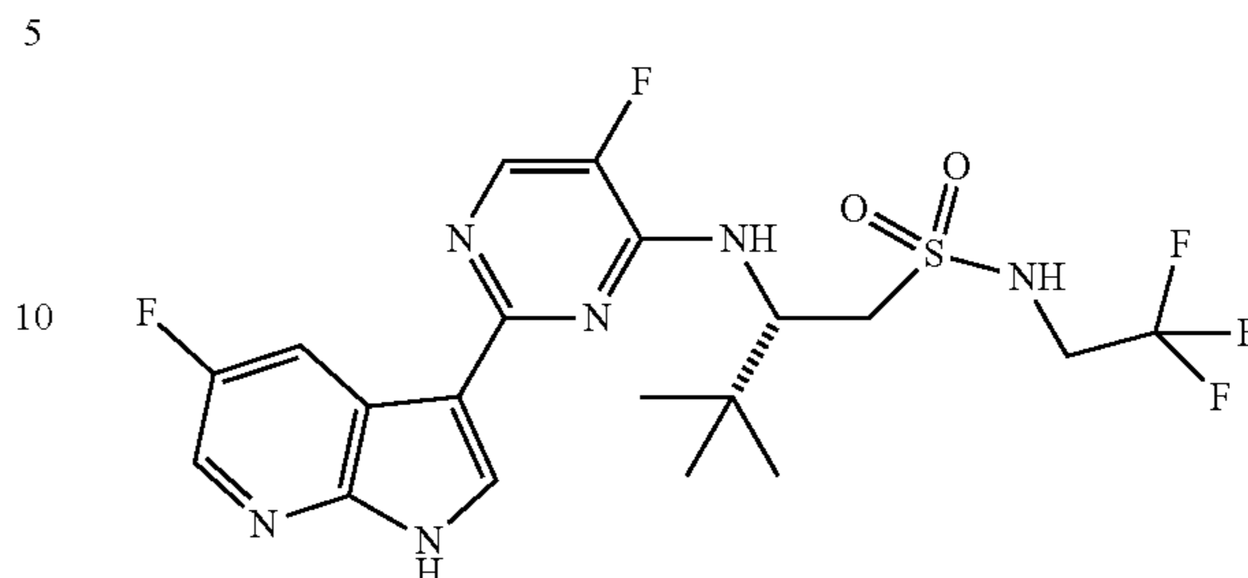
(S)-2-(5-fluoro-2-(5-fluoro-1H-pyrrolo[2,3-b]pyridin-3-yl)pyrimidin-4-ylamino)-3,3-dimethyl-N-(2,2,2-trifluoroethyl)butane-1-sulfonamide (58)
