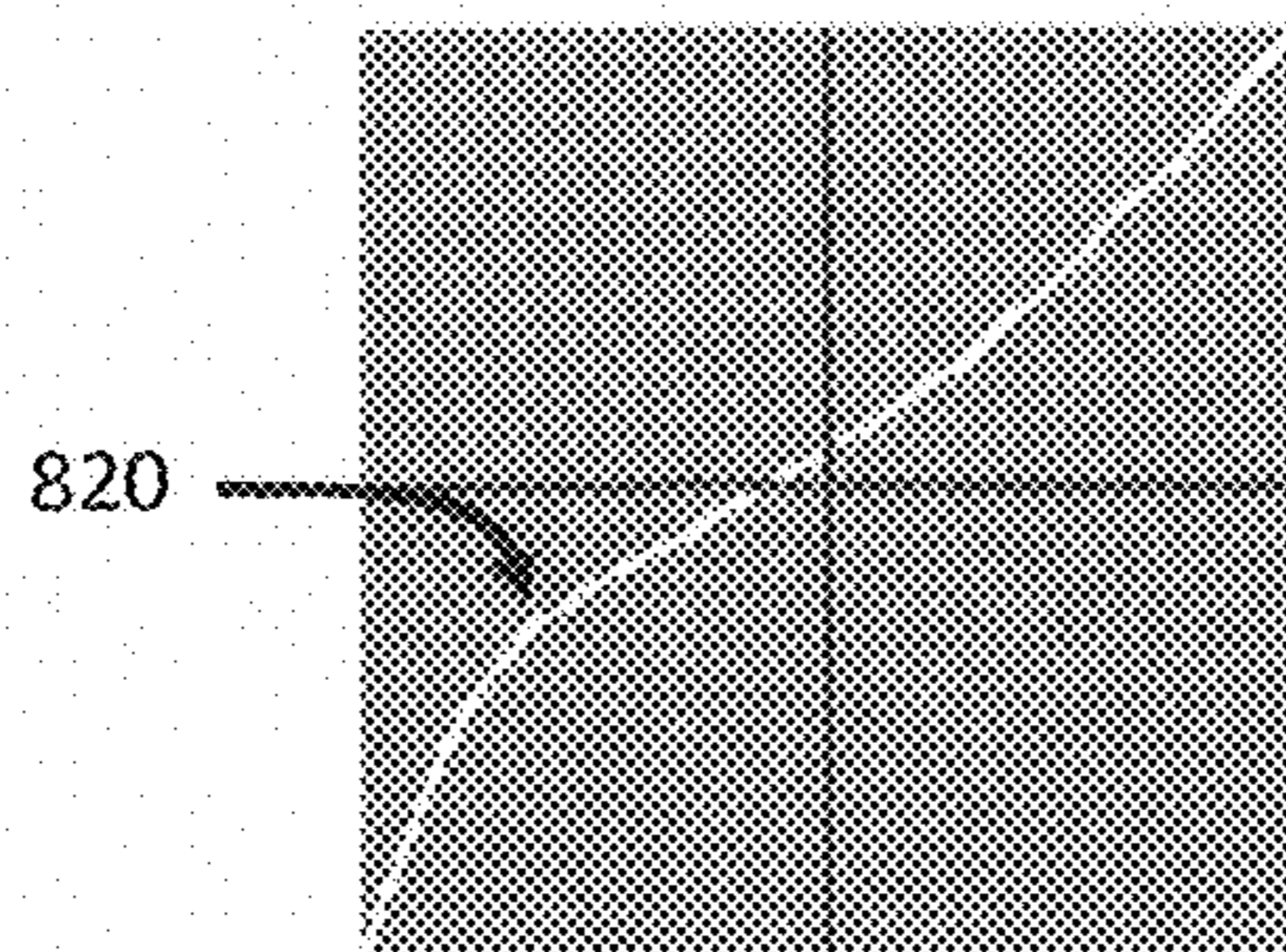
Figure 8r RF PLUT 4 lookup table plot
