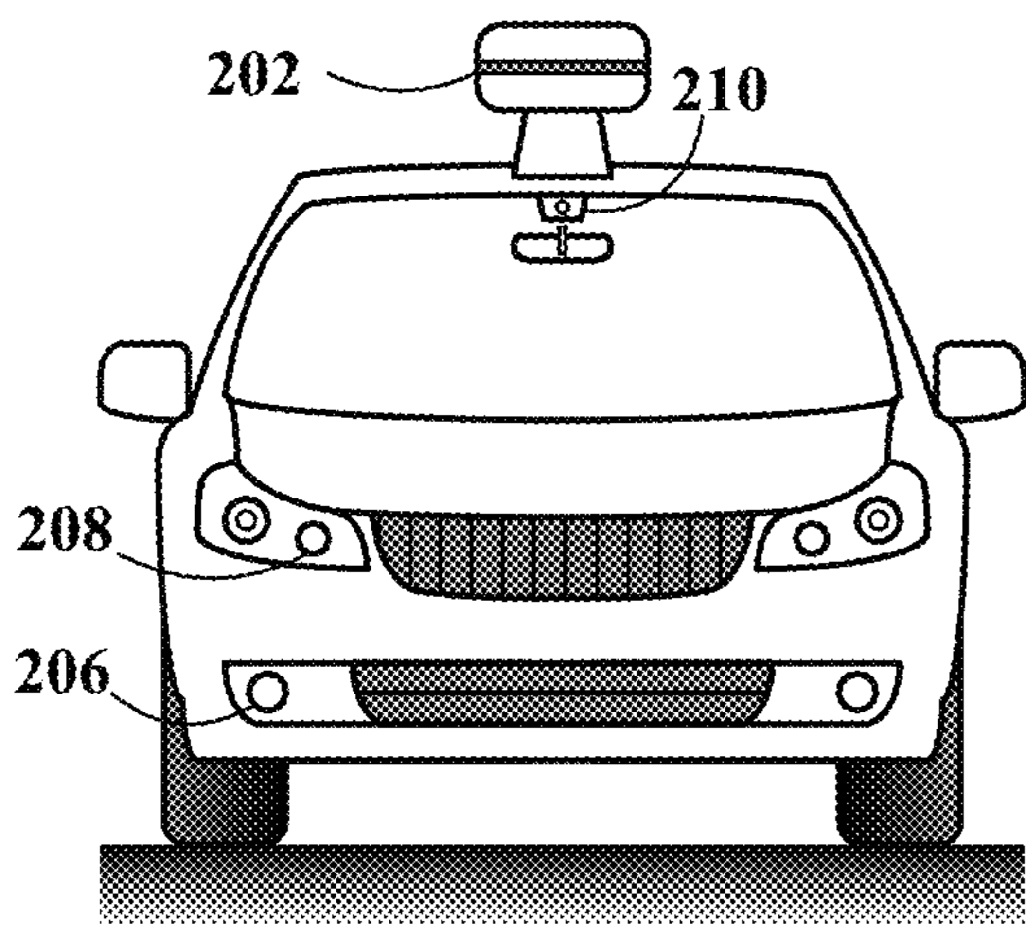
Front View
