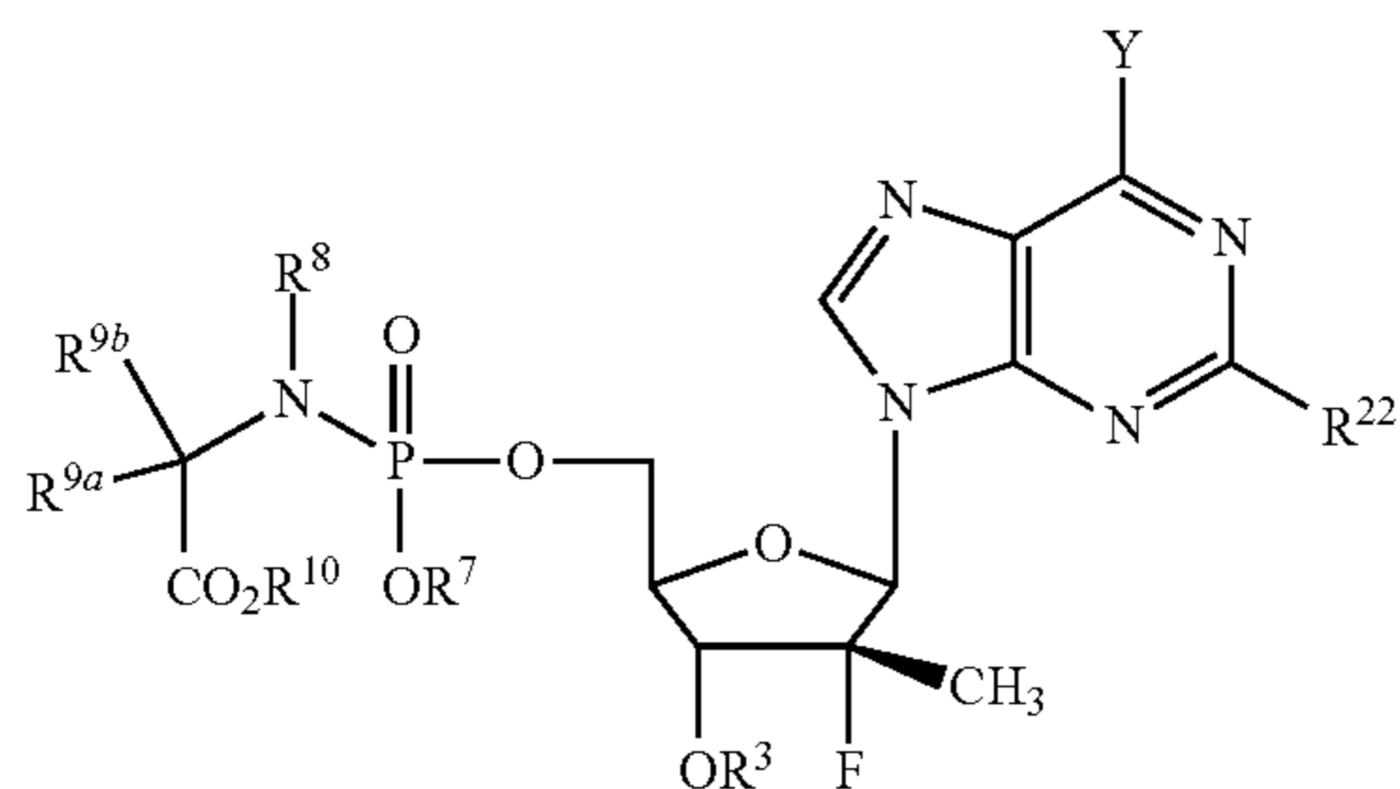
Formula IV
