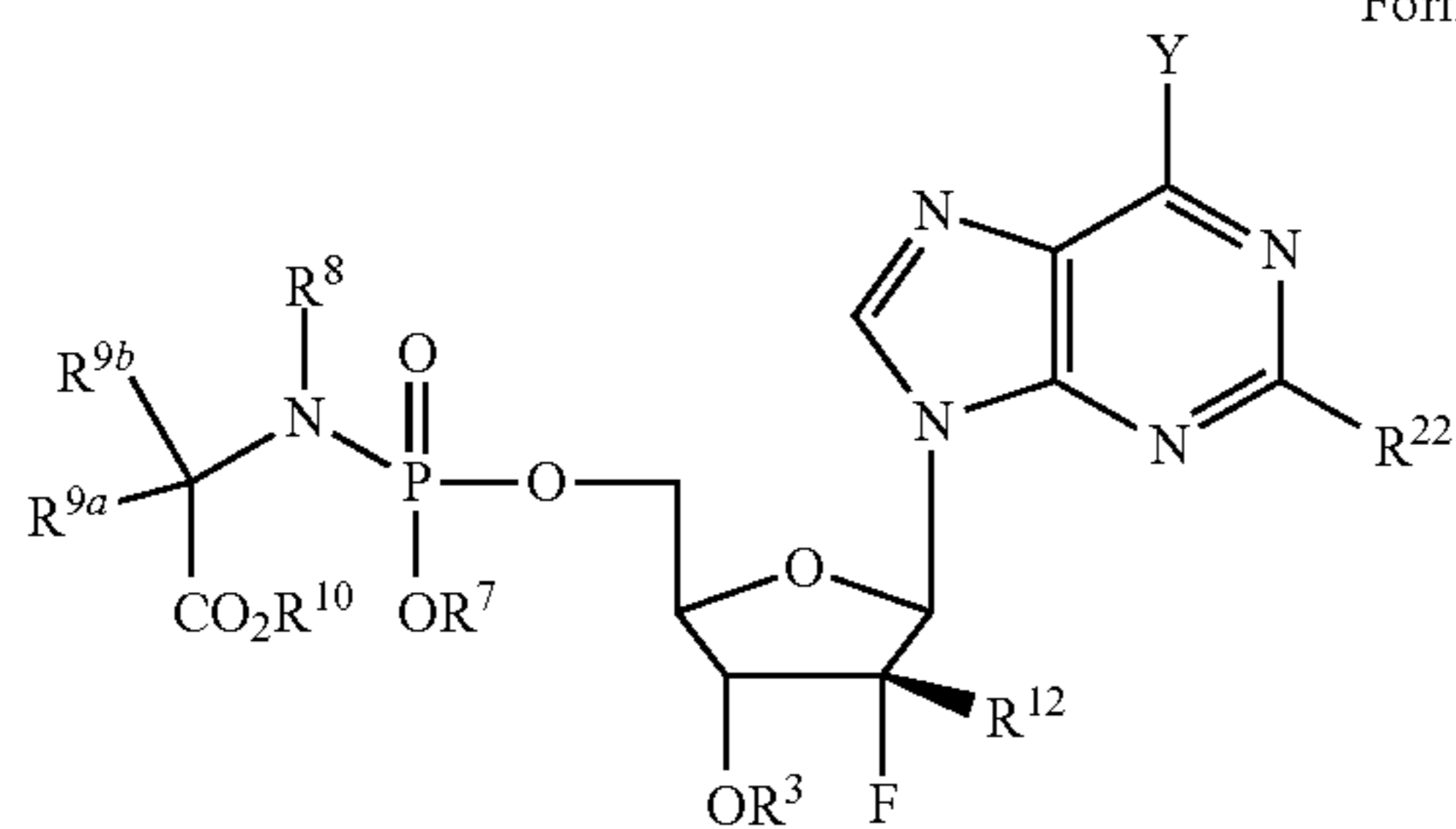
Formula III
