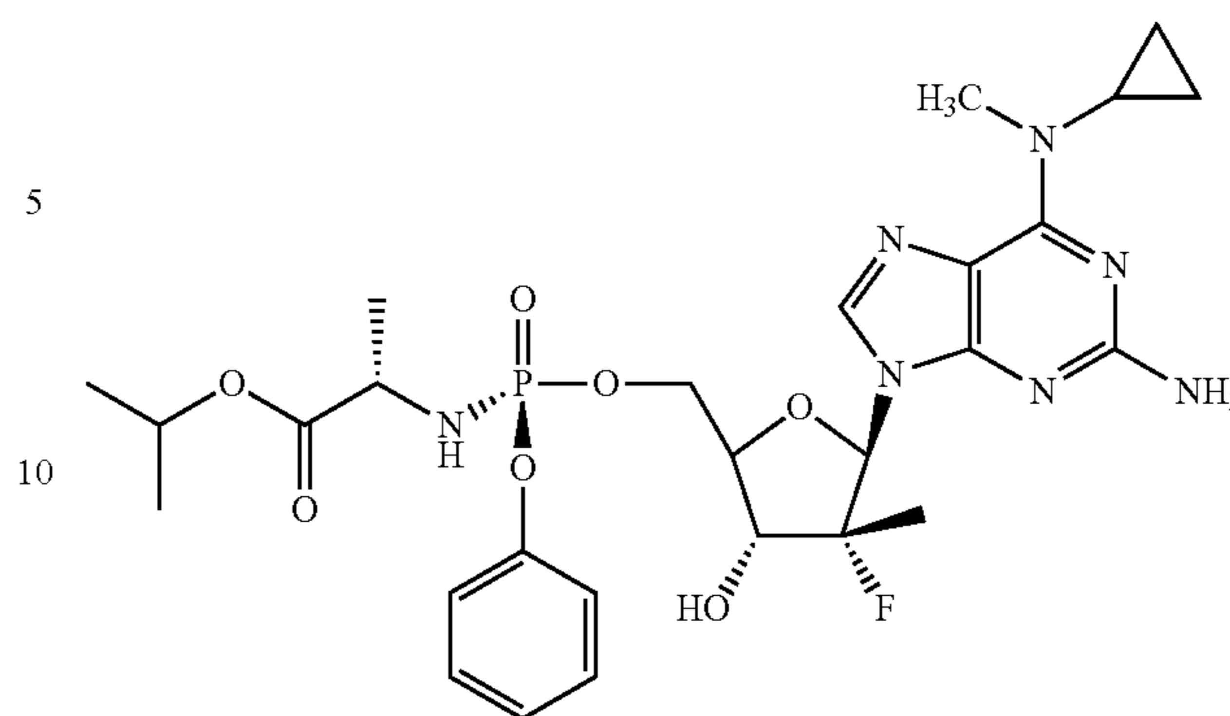
Compound 5-2 (Table 7)
