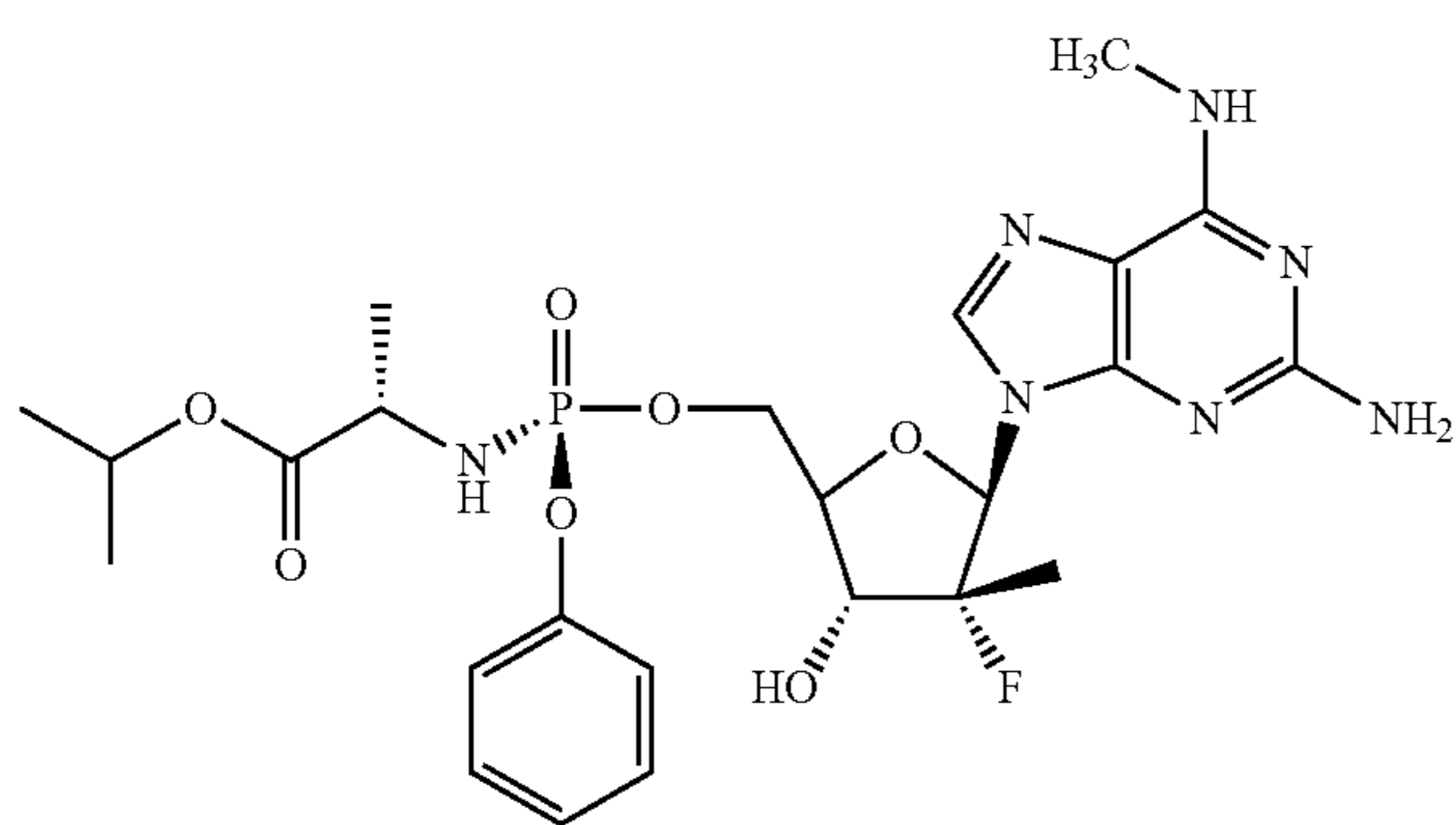
Compound 5-2 (Table 7)
