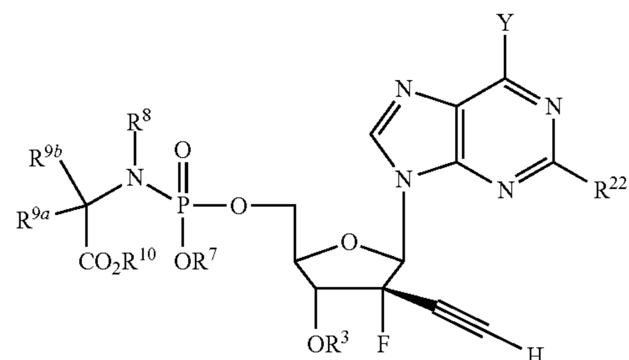
Formula V
