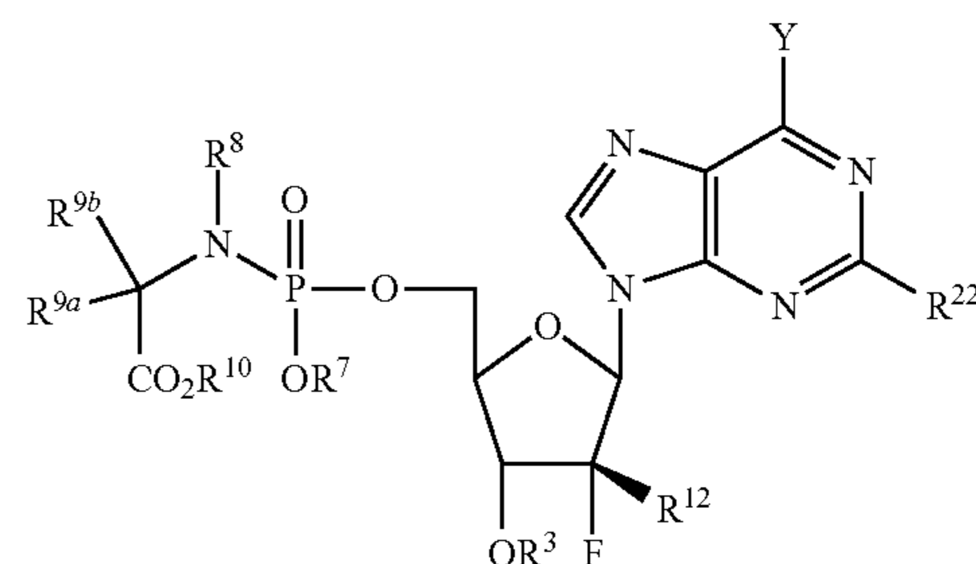
Formula III
