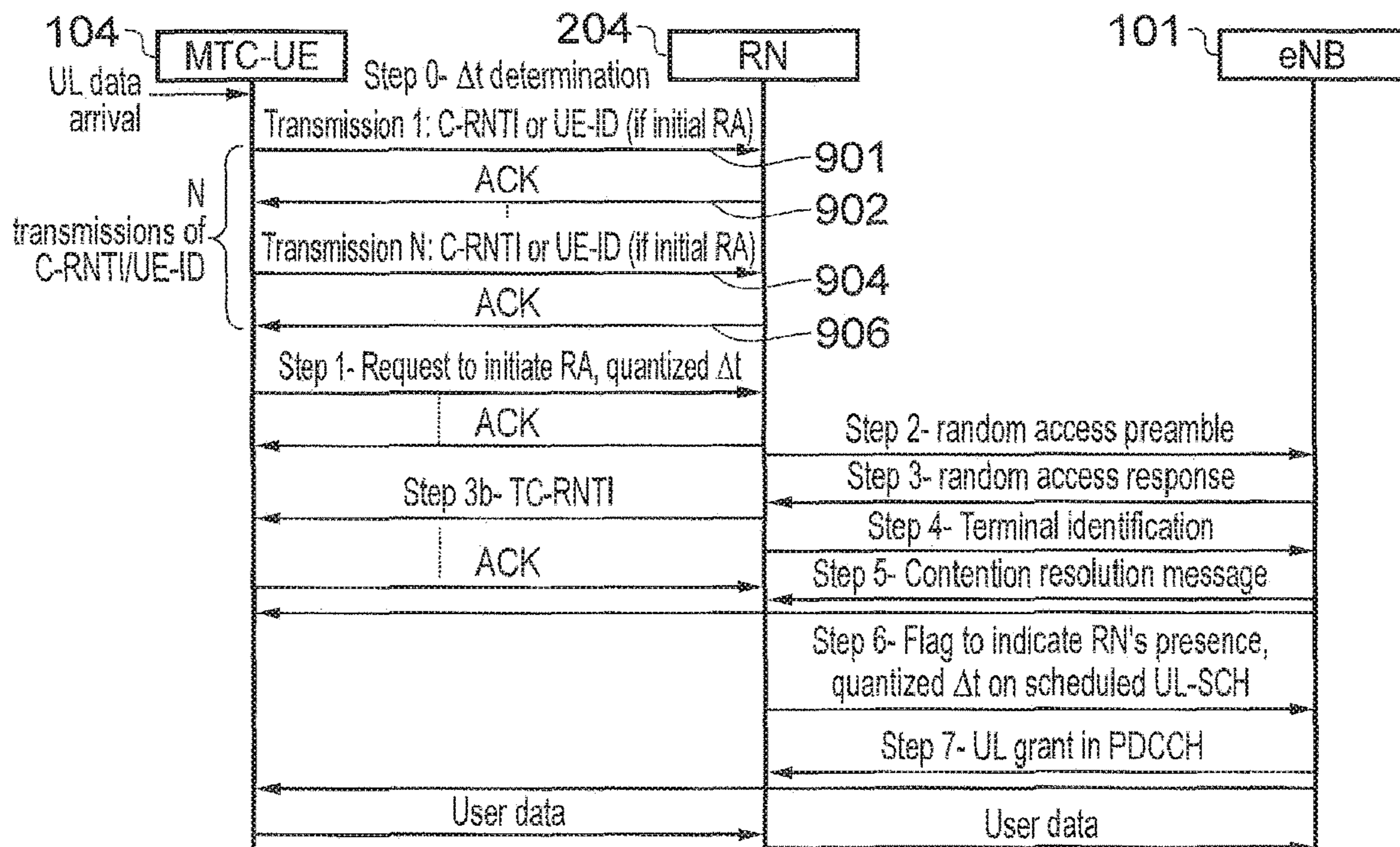
FIG. 12 Random Access procedure through RN (Solution 4)
