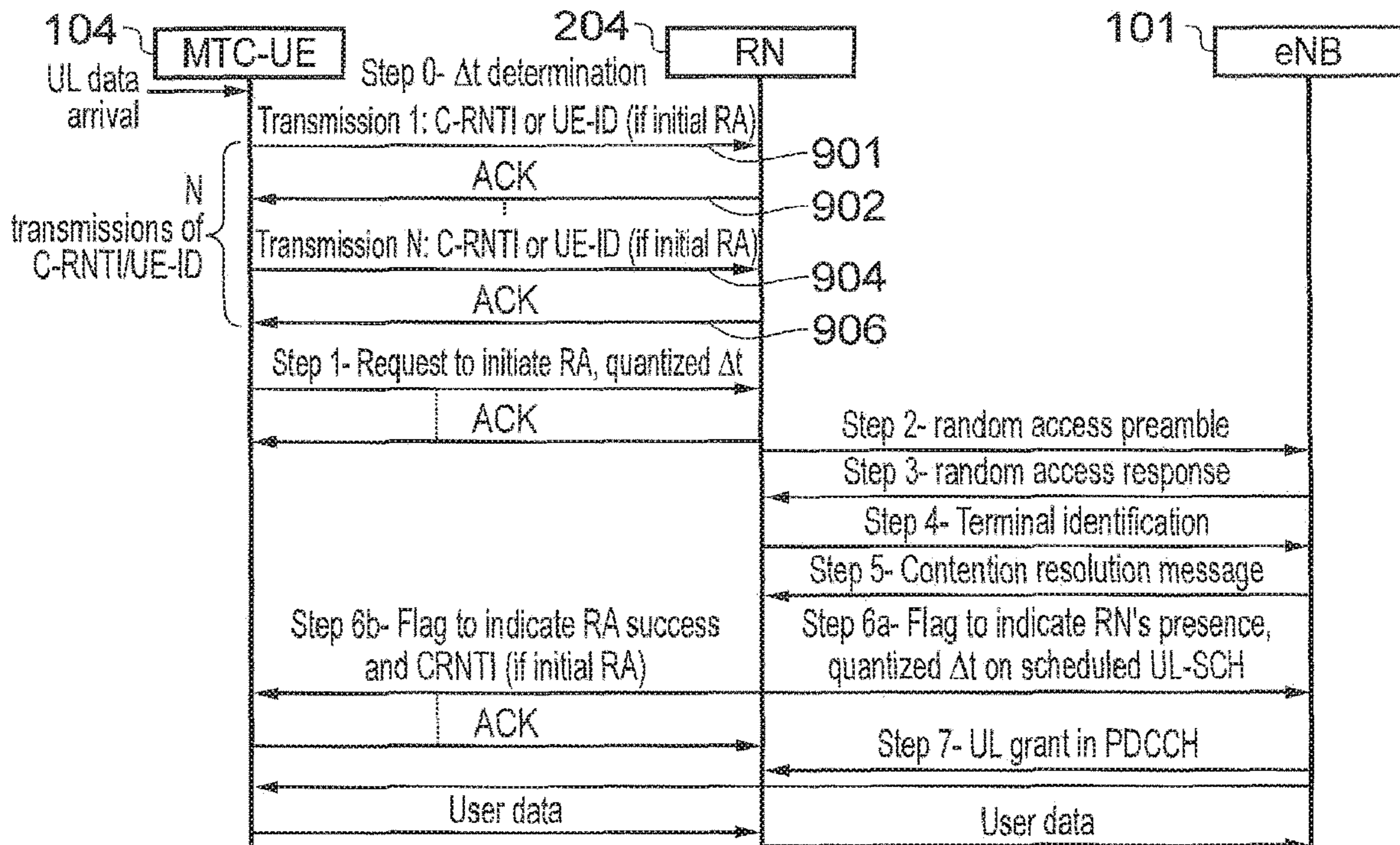
FIG. 11 Random Access procedure through RN (Solution 3)
