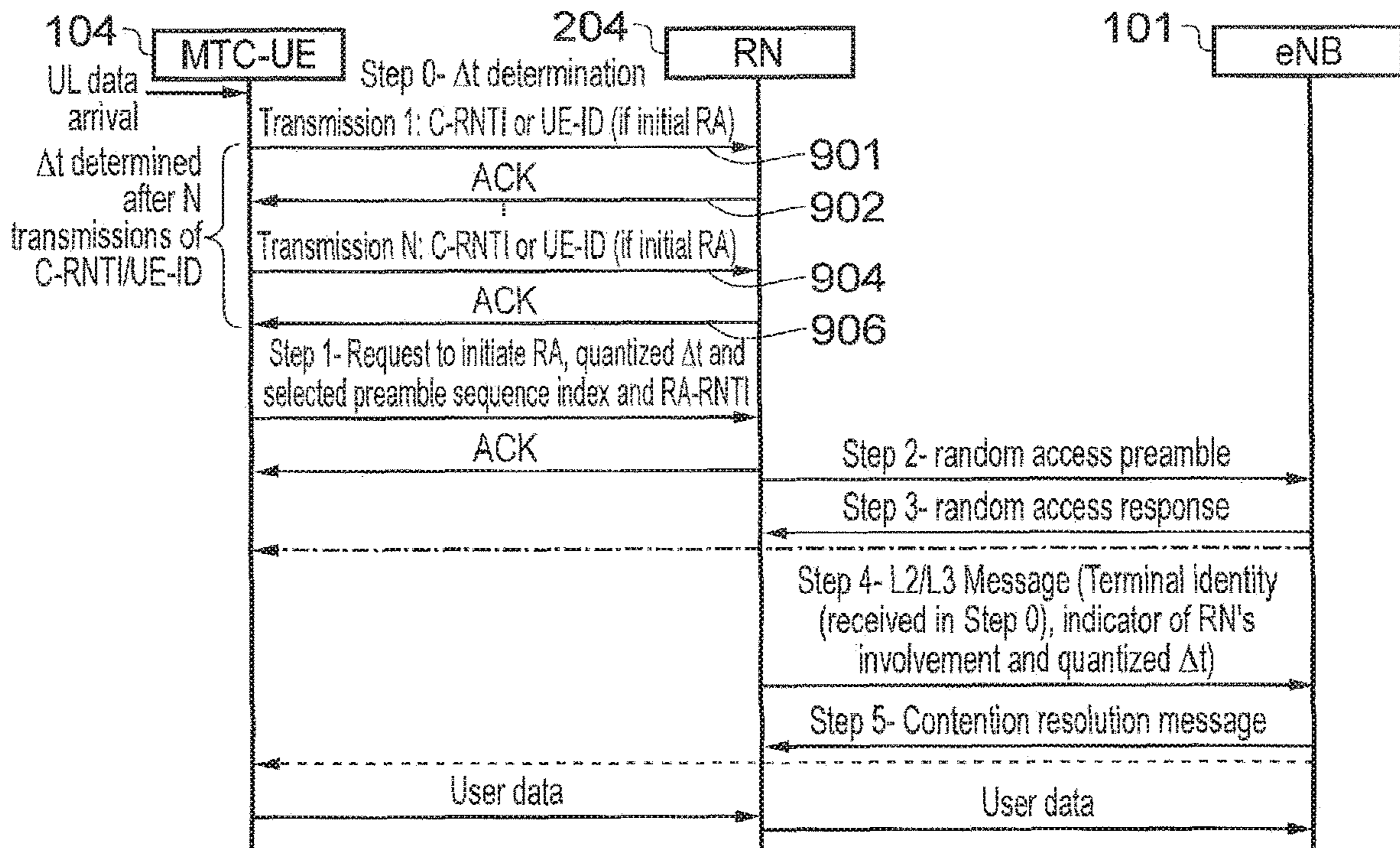
FIG. 9 Random Access procedure through RN (Solution 1)
