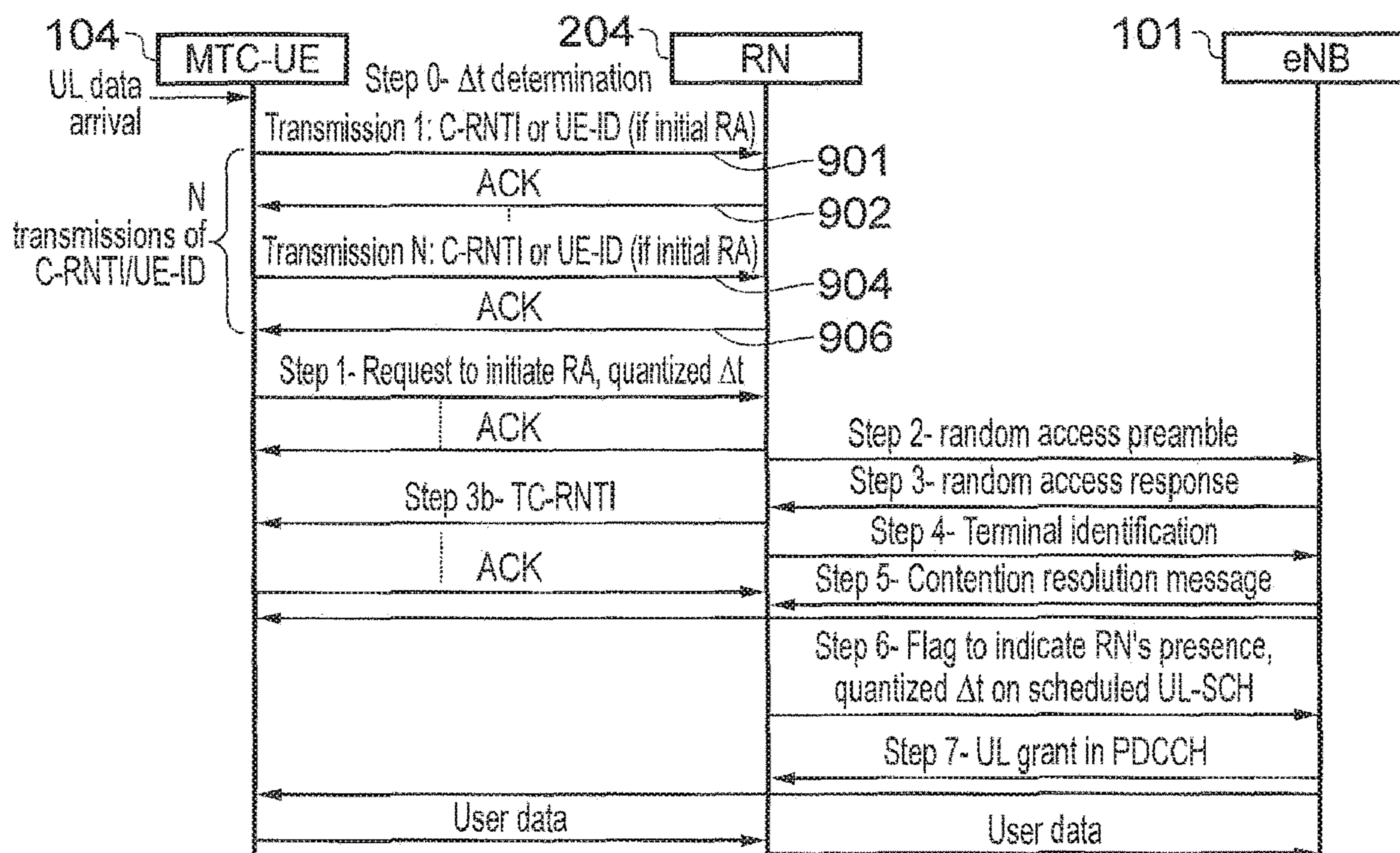
FIG. 12 Random Access procedure through RN (Solution 4)
