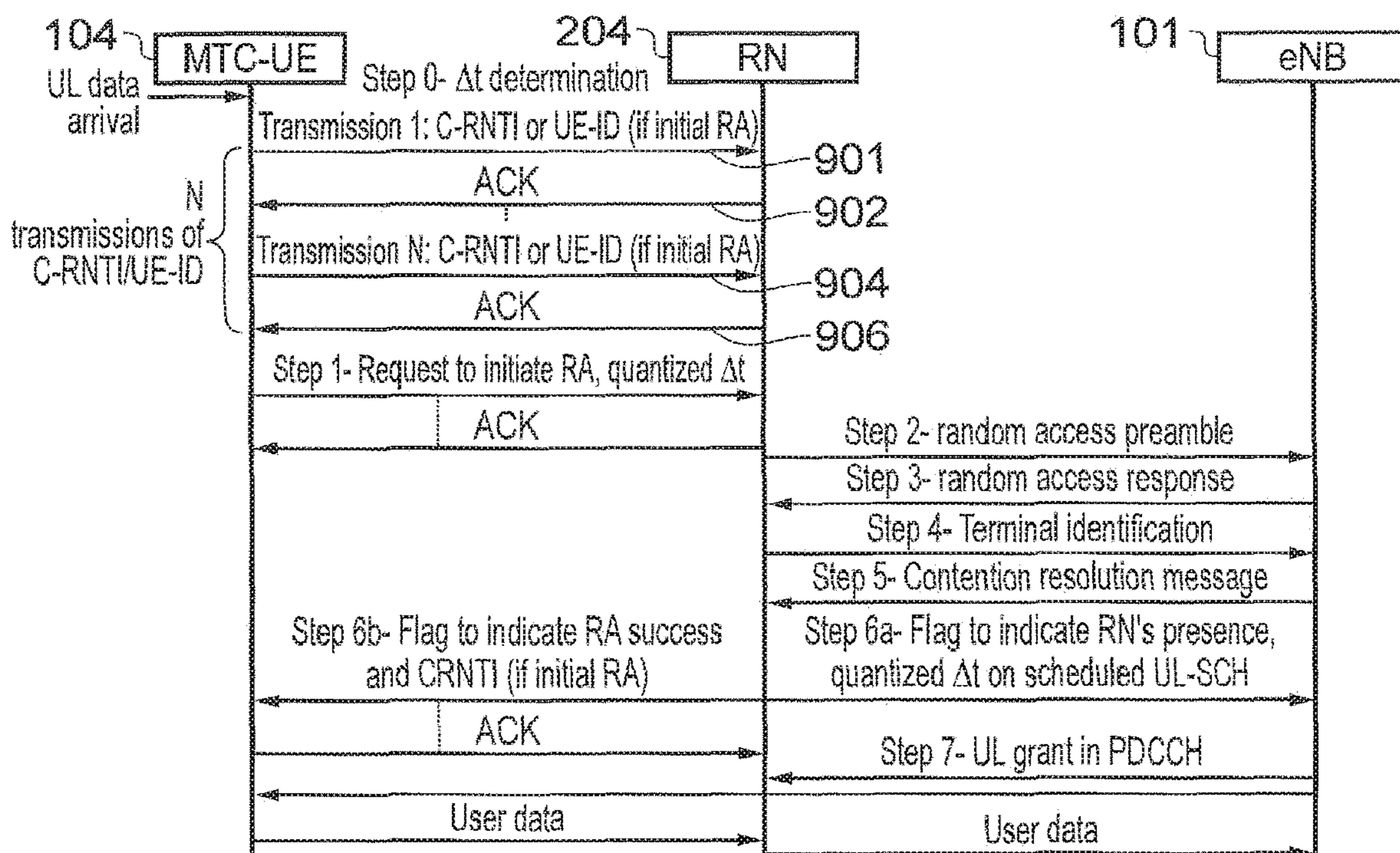
FIG. 11 Random Access procedure through RN (Solution 3)
