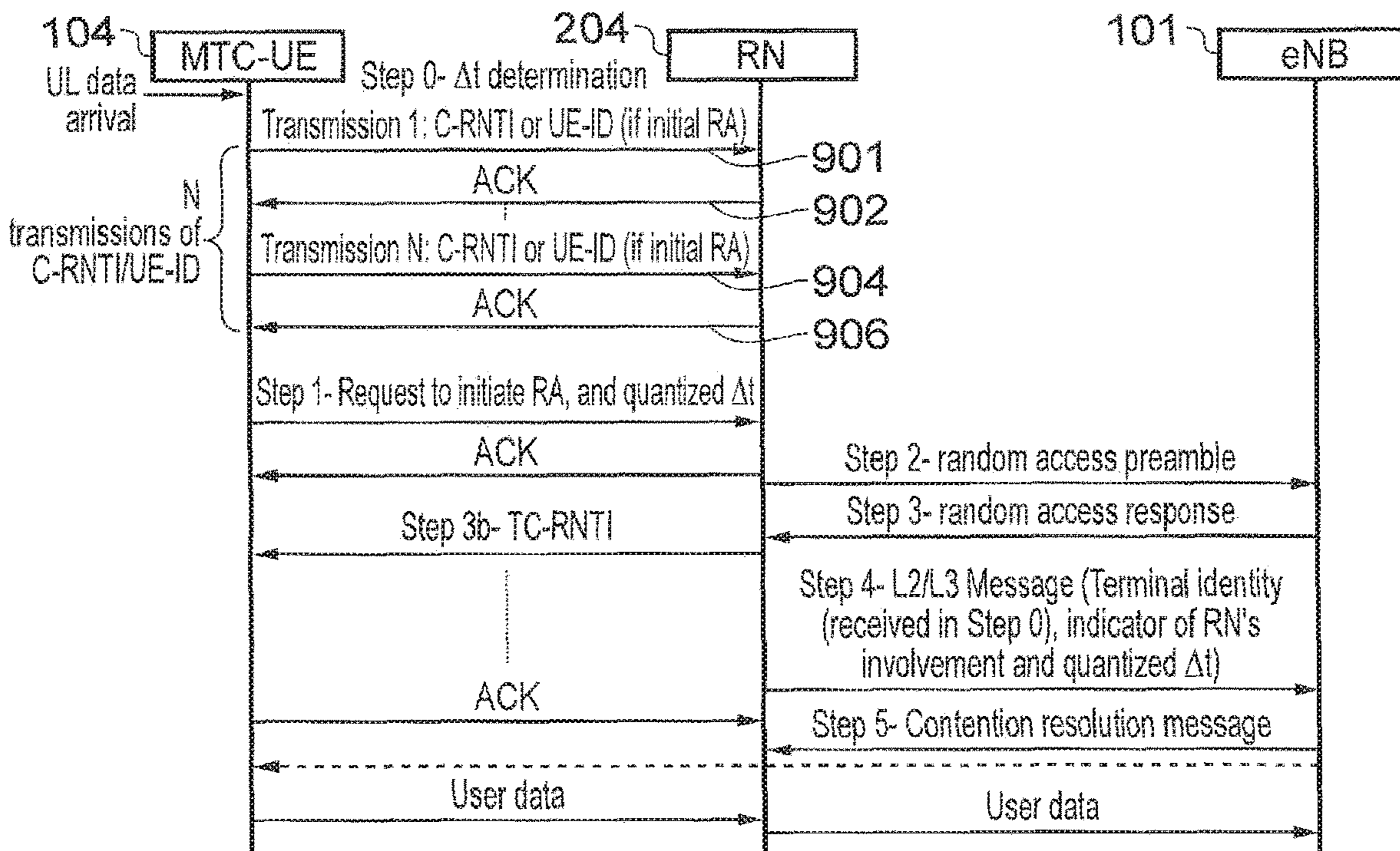
FIG. 10 Random Access procedure through RN (Solution 2)
