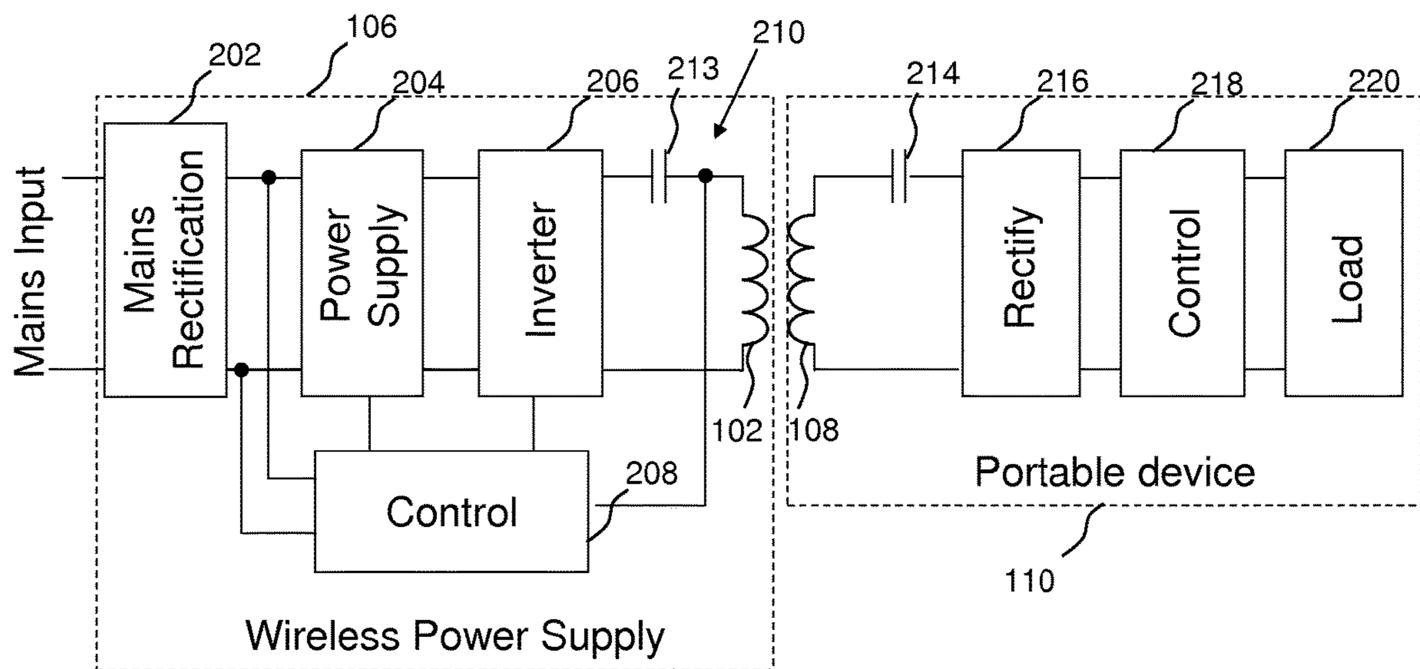
Fig. 2 PRIOR ART
