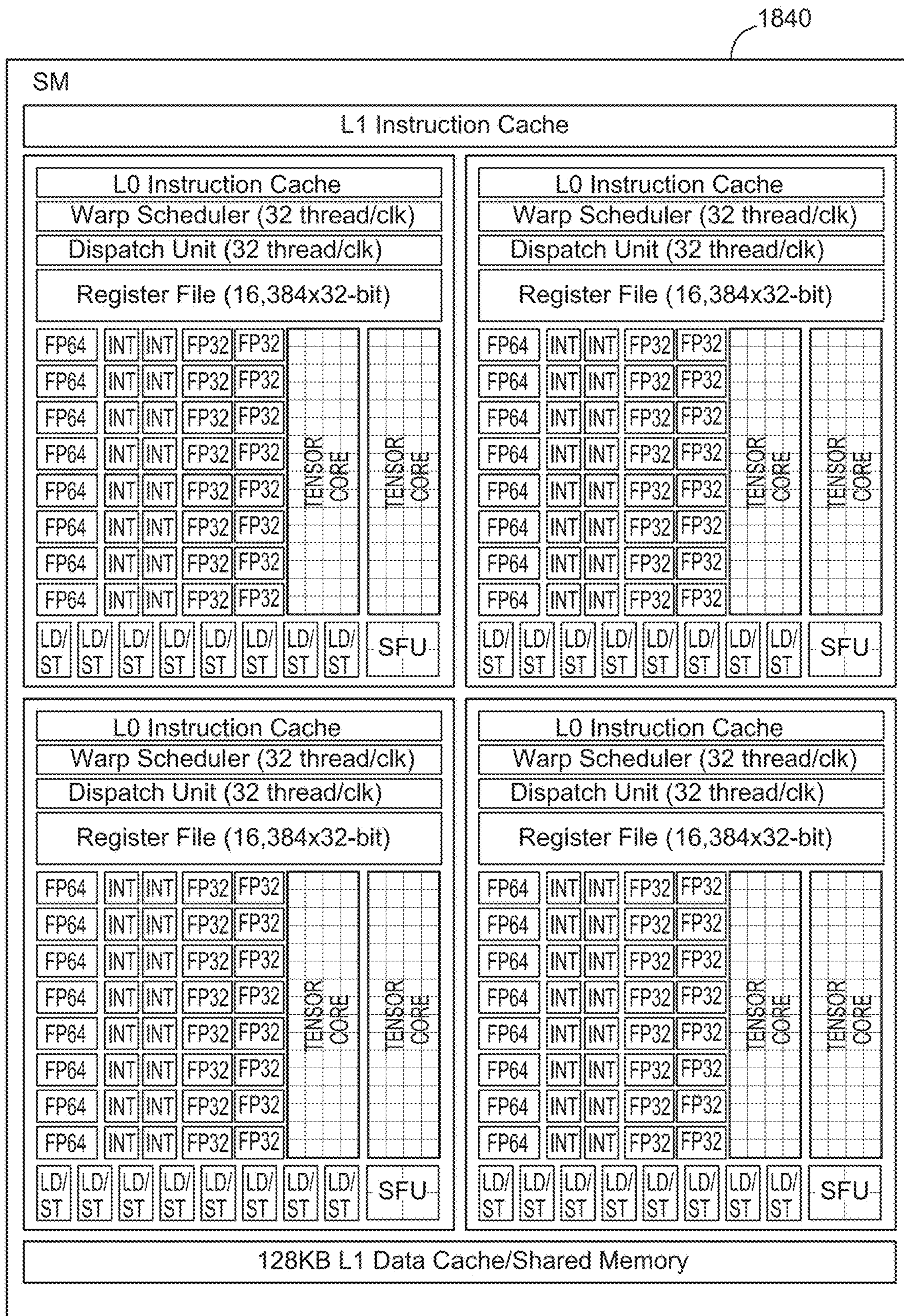
FIG. 21 Example Streaming Multiprocessor
