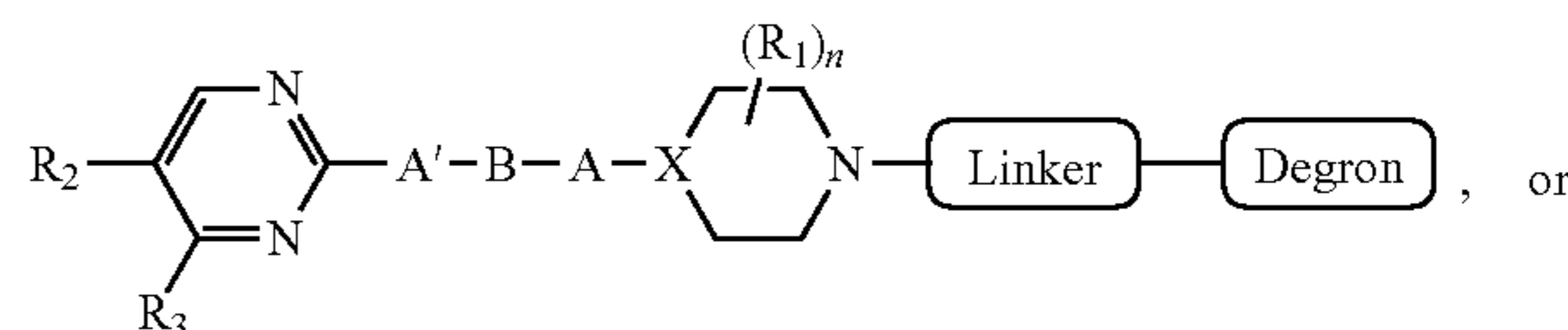
Targeting Ligand
