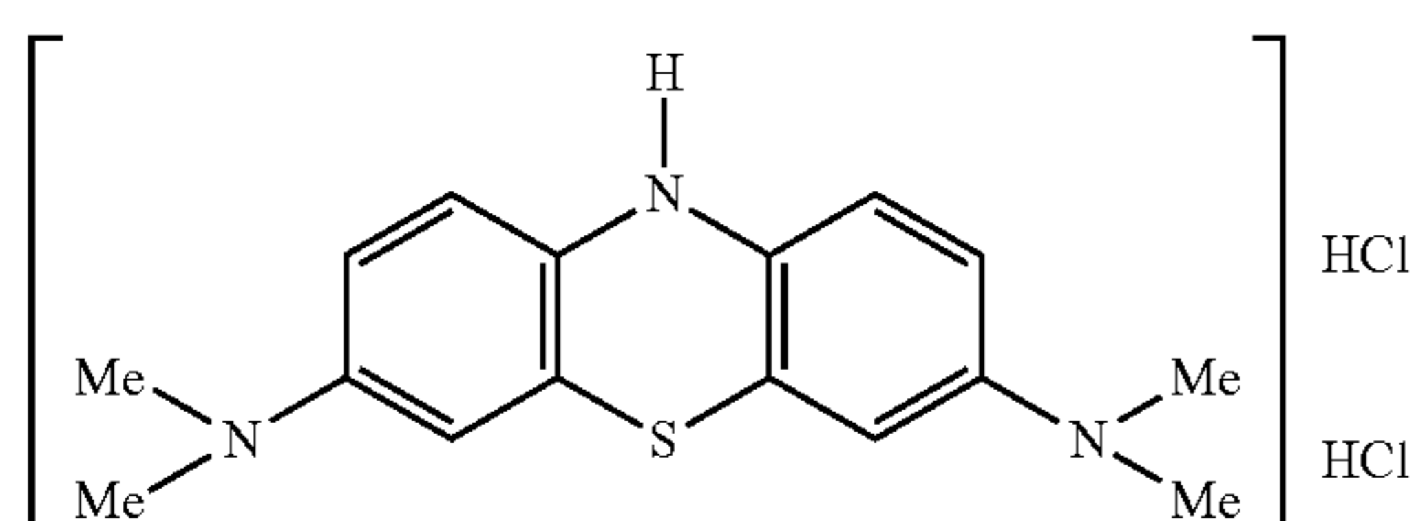
N,N,N',N'-tetramethyl-10H-phenothiazine 3,7-diaminium di(chloride), (LMT•2HCl)
