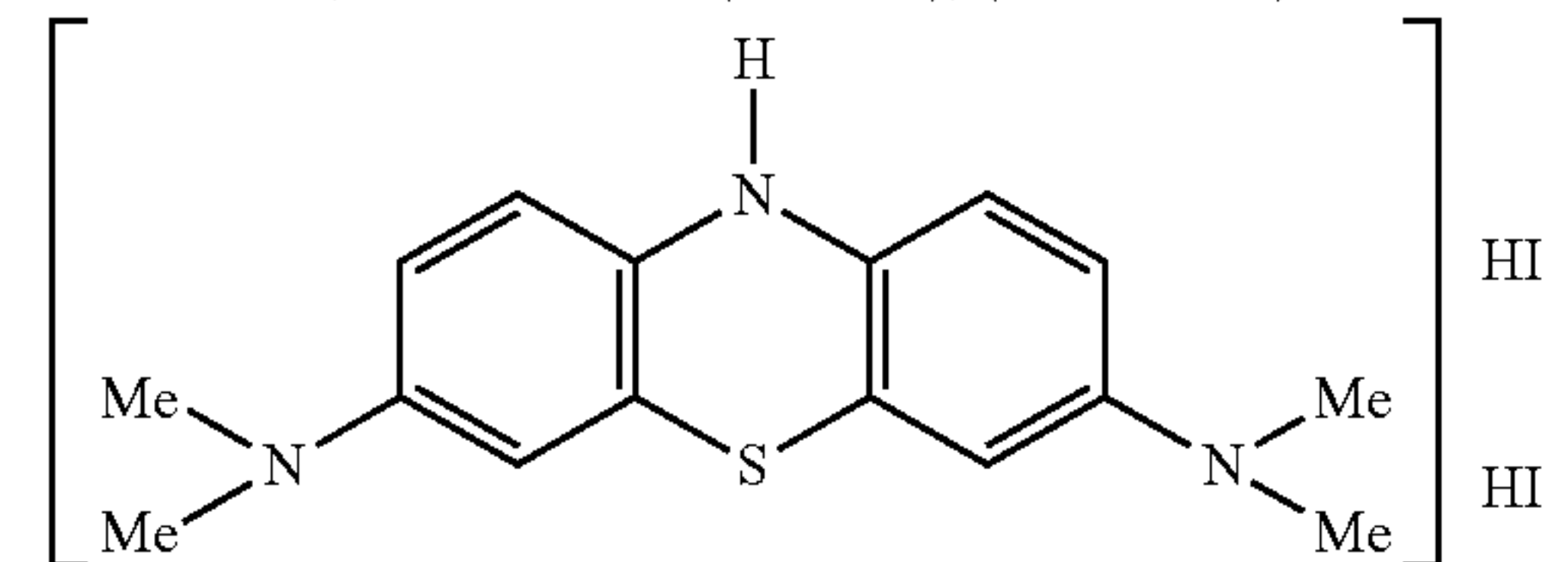
N,N,N',N'-tetramethyl-10H-phenothiazine 3,7-diaminium di(iodide), (LMT•2HI)
