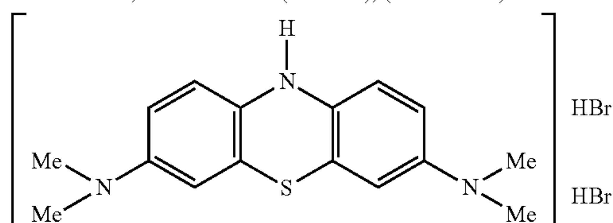
N,N,N',N'-tetramethyl-10H-phenothiazine 3,7-diaminium di(bromide), (LMT•2HBr)
