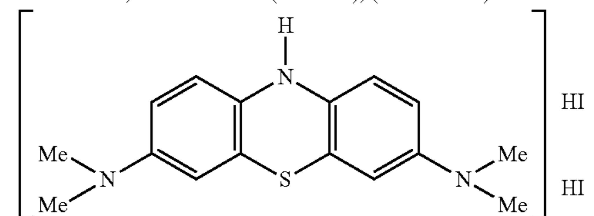
N,N,N',N'-tetramethyl-10H-phenothiazine 3,7-diaminium di(iodide), (LMT•2HI)
