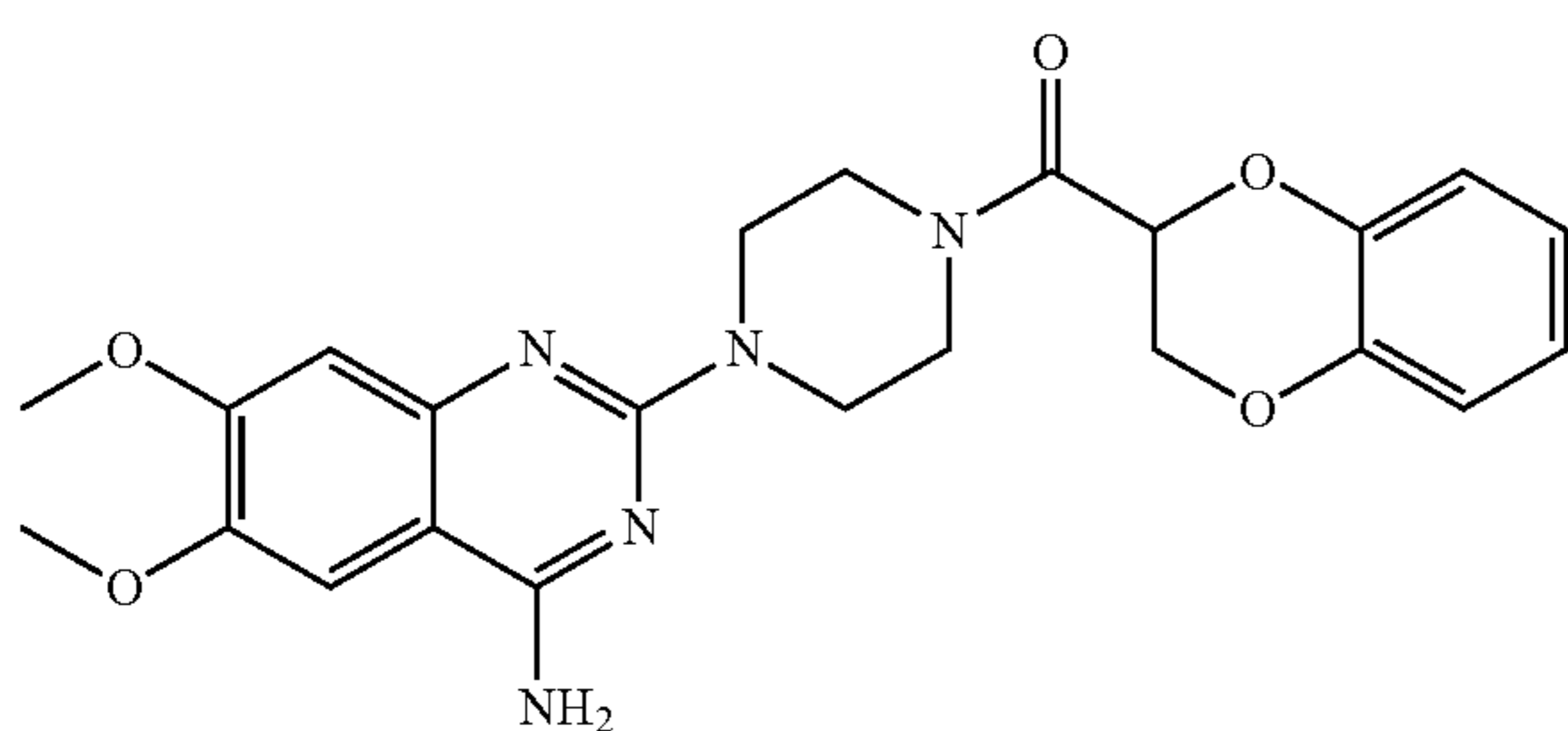
(4-(4-amino-6,7-dimethoxyquinazolin-2-yl)piperazin-1-yl)(2,3-dihydrobenzo[b][1,4]dioxin-2-yl)methanone
