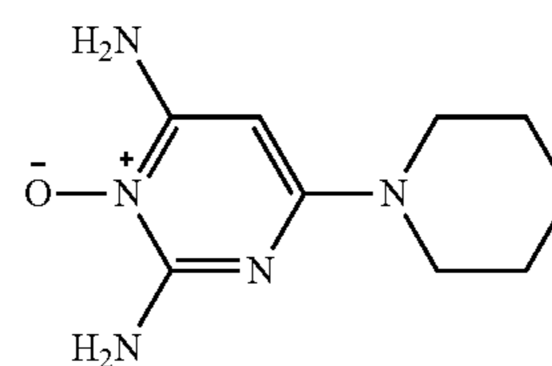
2,6-diamino-4-(piperidin-1-yl)pyrimidine 1-oxide
