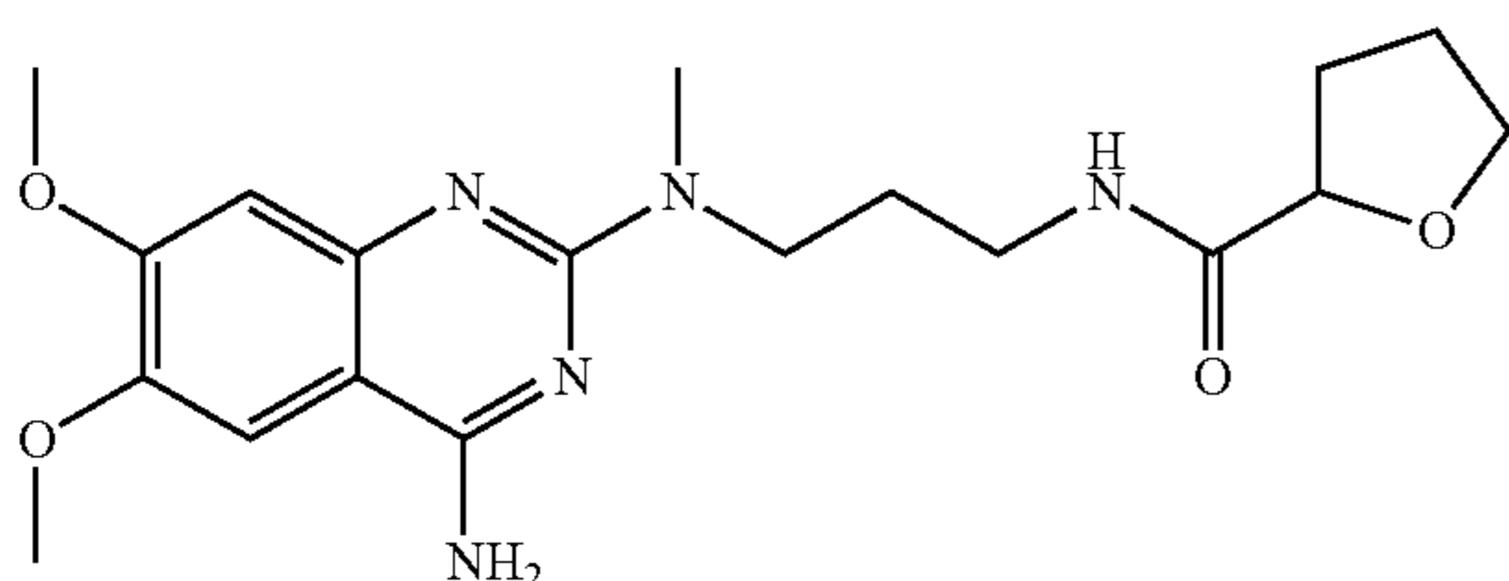
N-(3((4-amino-6,7-dimethoxyquinazolin-2-yl)(methyl)amino)propyl)tetrahydrofuran-2-carboxamide
