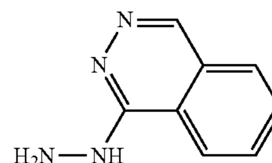
1-hydrazinylphthalazine
