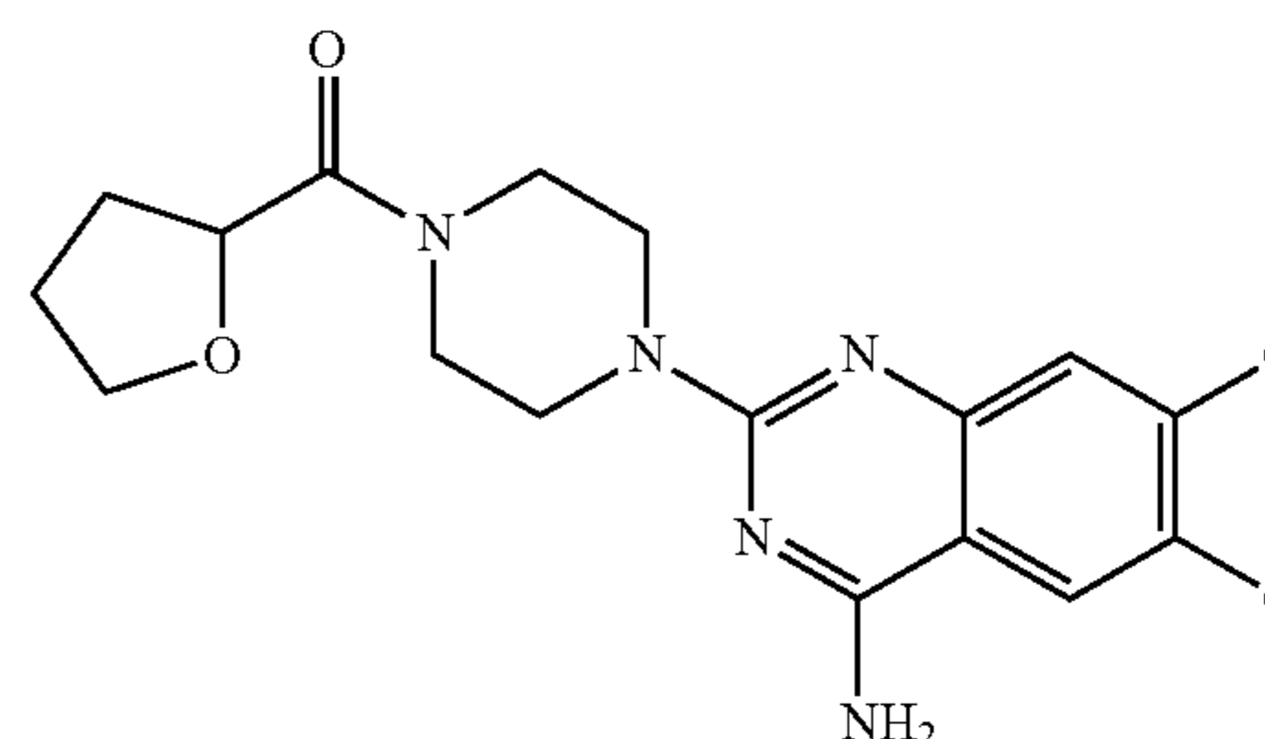
(4-(4-amino-6,7-dimethoxyquinazolin-2-yl)piperazin-1-yl)(tetrahydrofuran-2-yl)methanone
