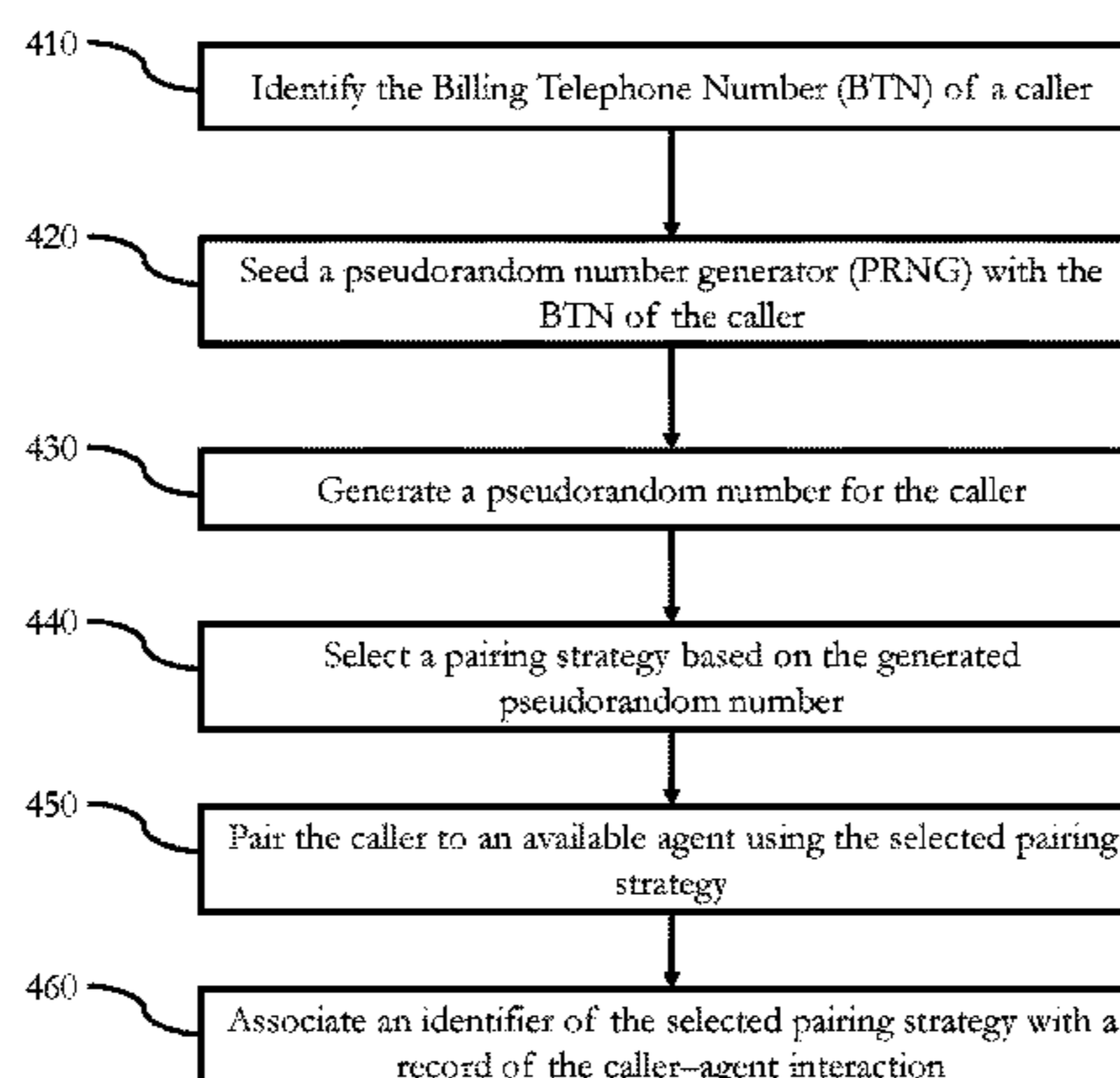
Benchmarking Method 400
