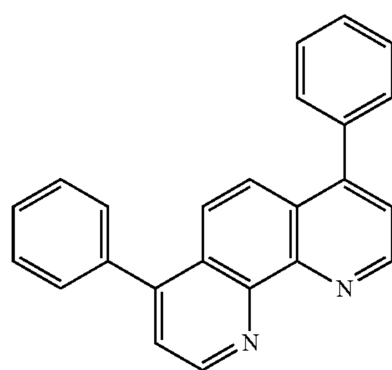
BPhen
