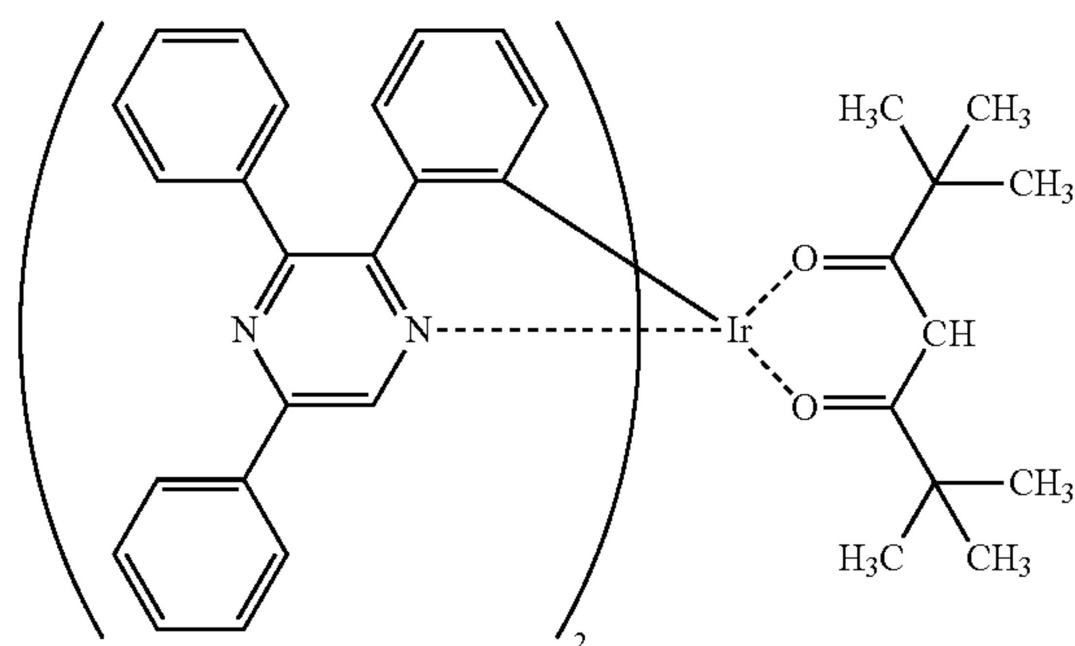
Ir(tppr) 2 (dpm)
