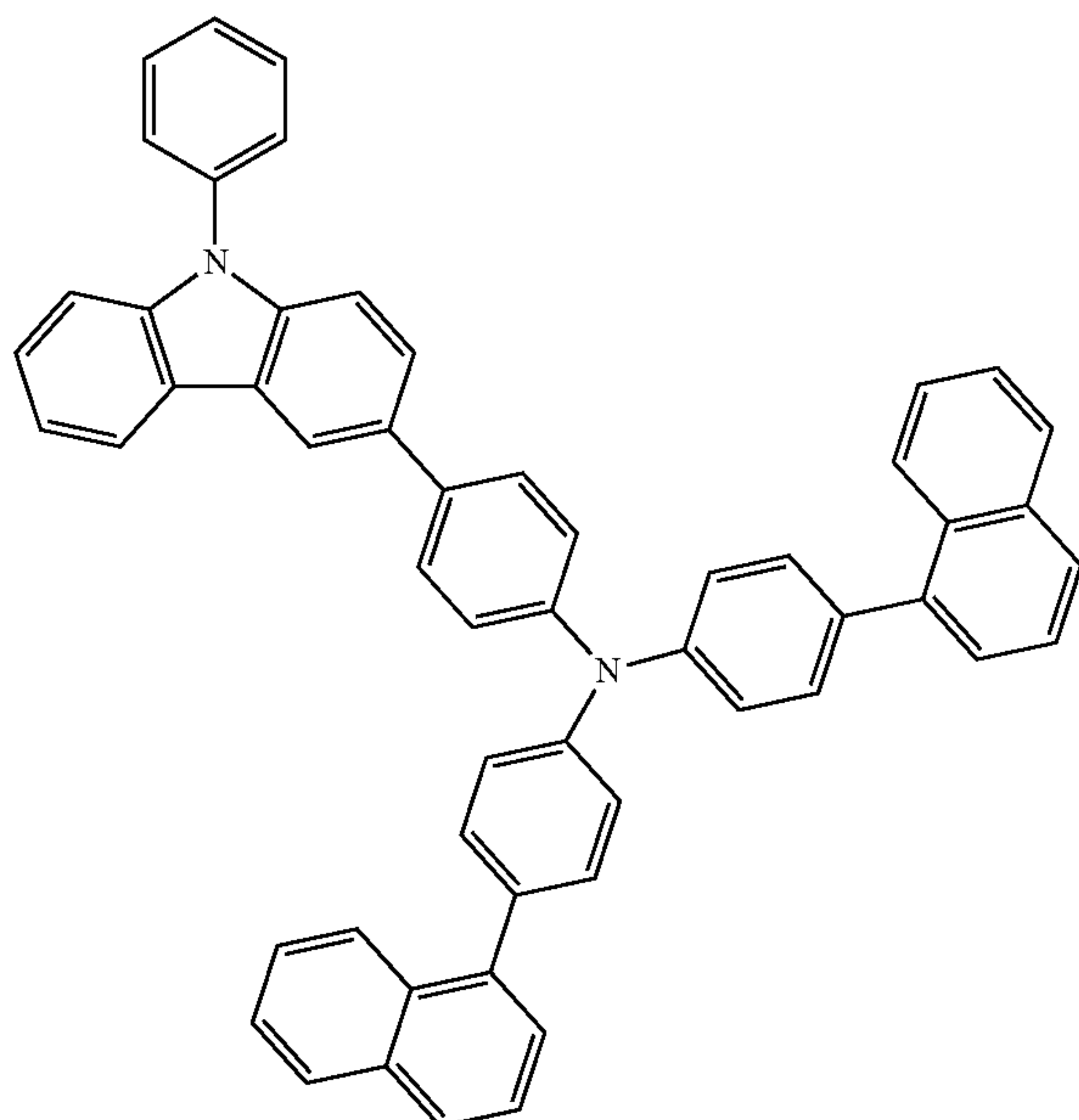
PCBNBB
