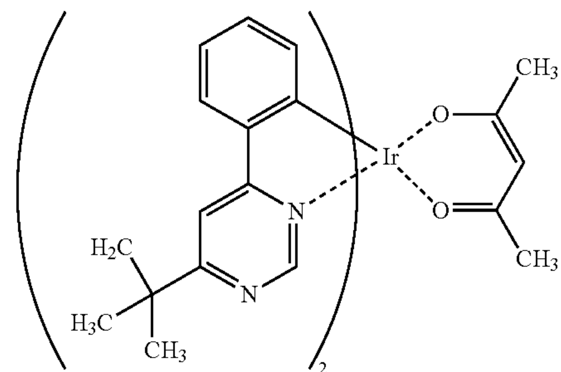
\text{Ir}(\text{tBuppm})_2(\text{acac})
