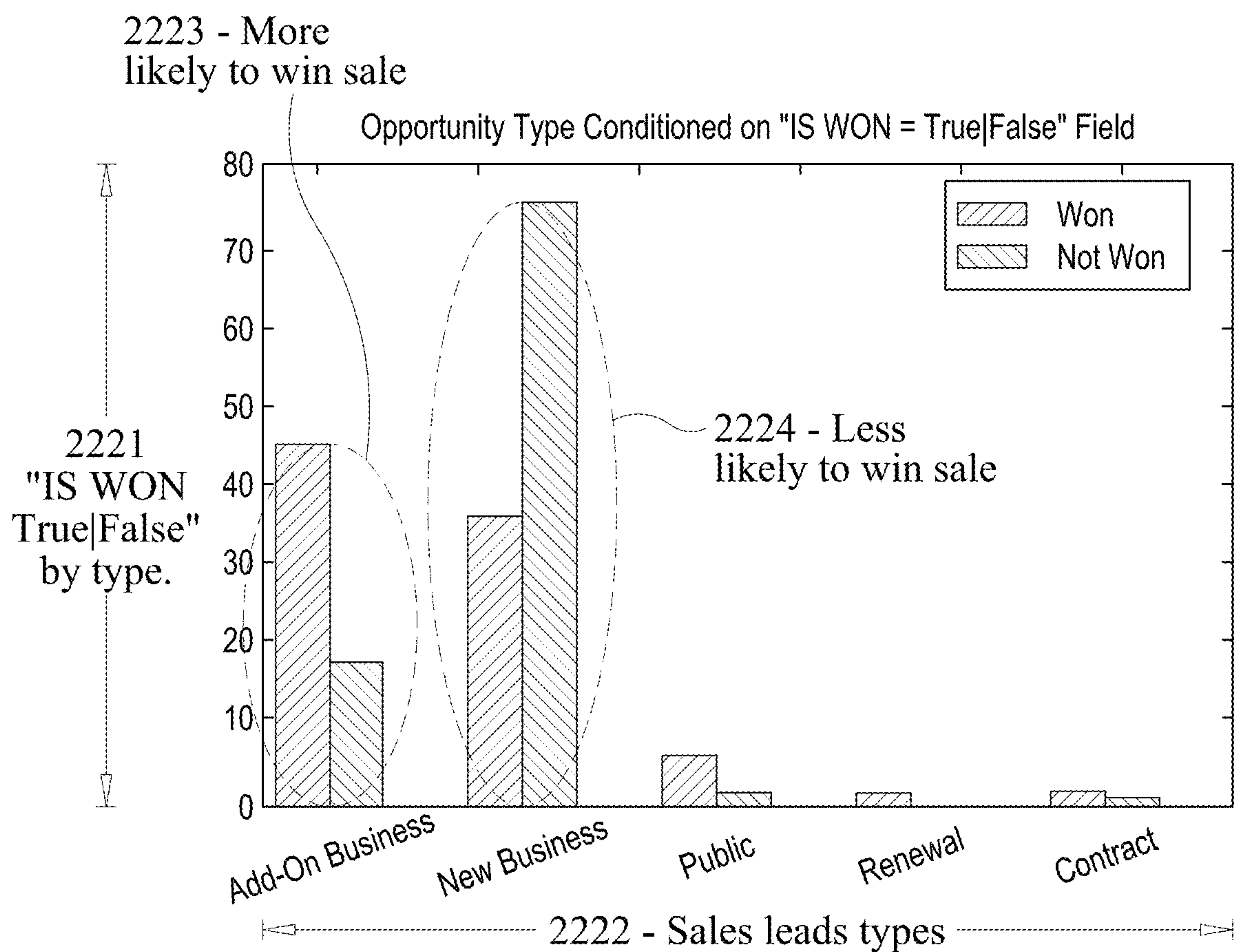
FIG. 22B Predictive Relationships for Opportunity Scoring
