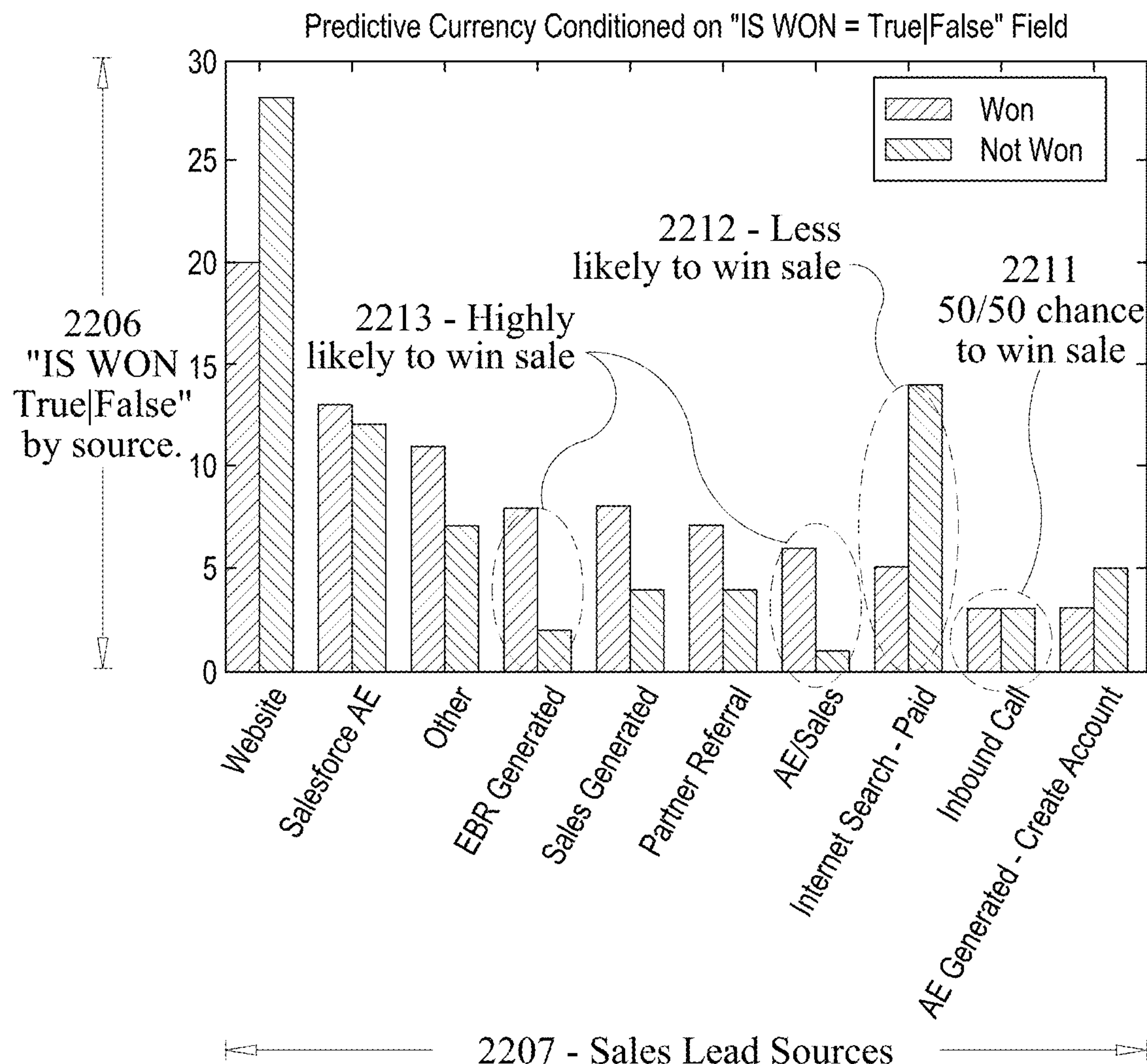
FIG. 22A Predictive Relationships for Opportunity Scoring
