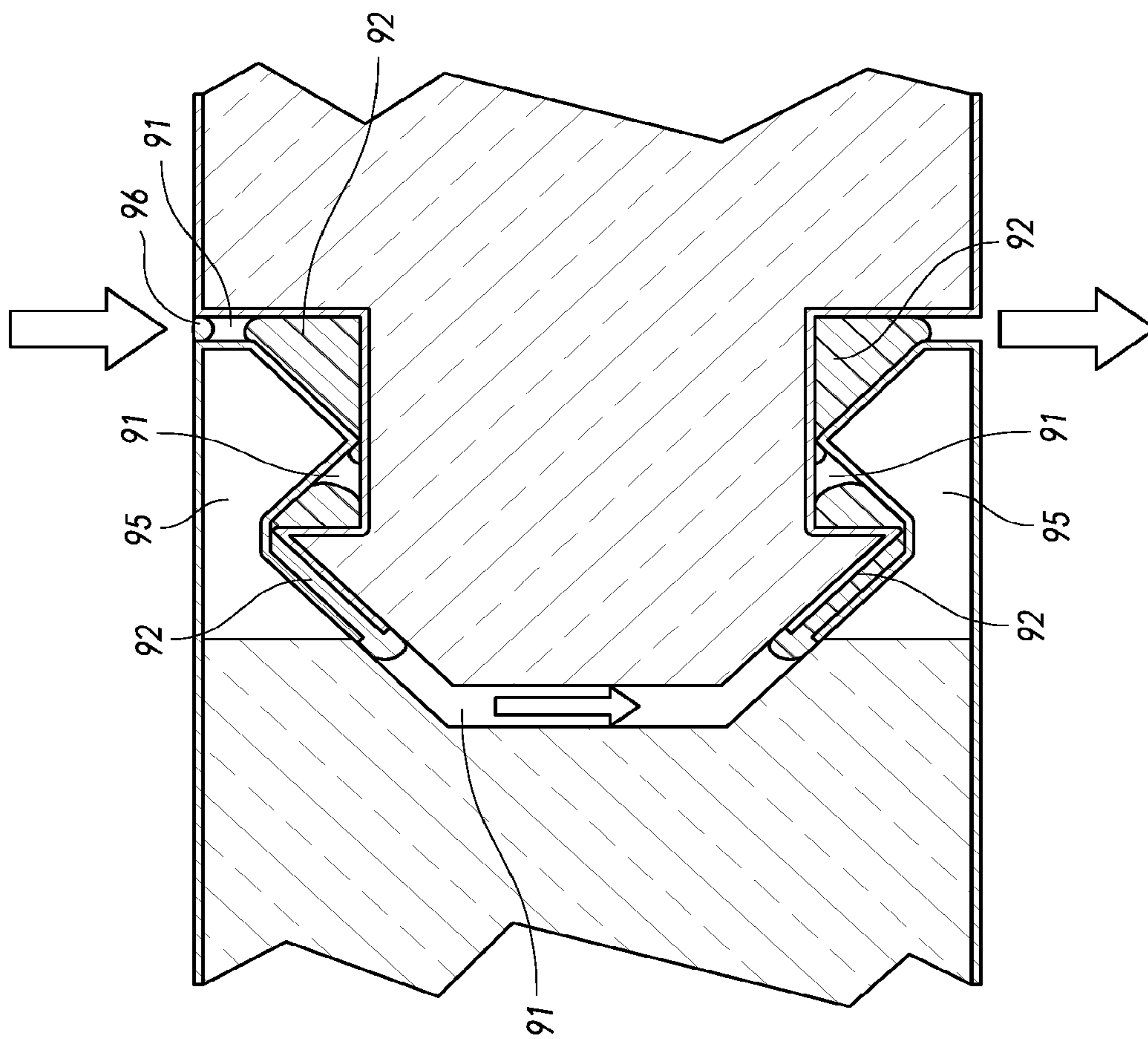
FIG. 9 (PRIOR ART)
