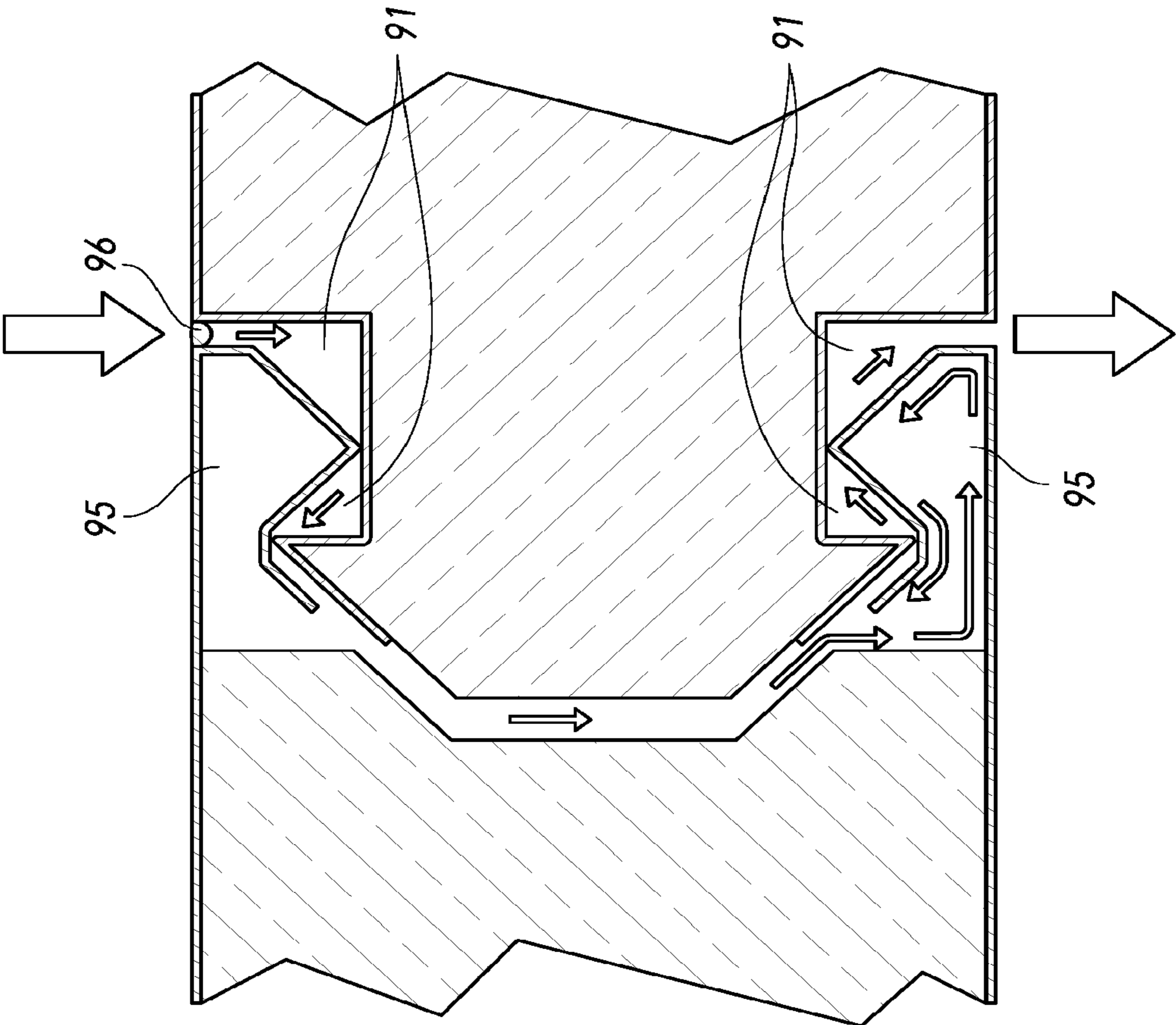
FIG. 10 (PRIOR ART)
