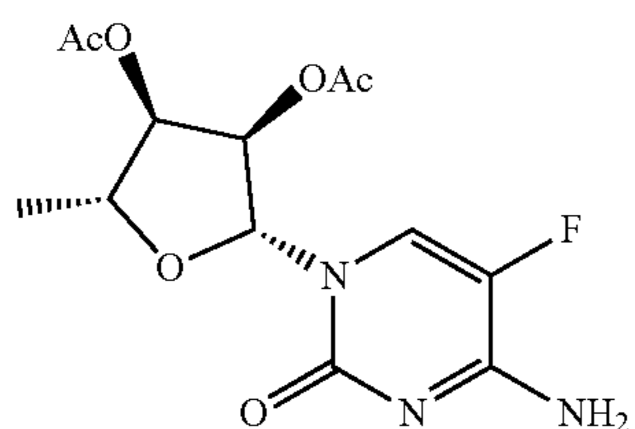
(2R,3R,4R,5R)-2-(4-amino-5-fluoro-2-oxypyrimidin-1(2H)-yl)-5-methyltetrahydrofuran-3,4-diyl diacetate
