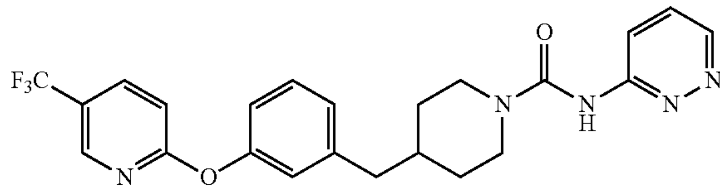
Phenyl pyridazin-3-ylcarbamate
