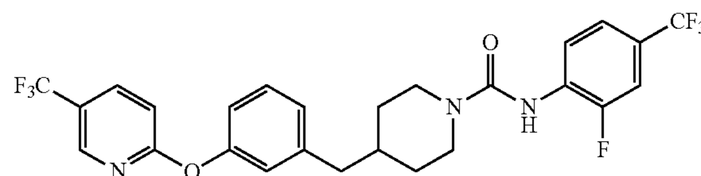
Phenyl (2-fluoro-4-(trifluoromethyl)phenyl)carbamate
