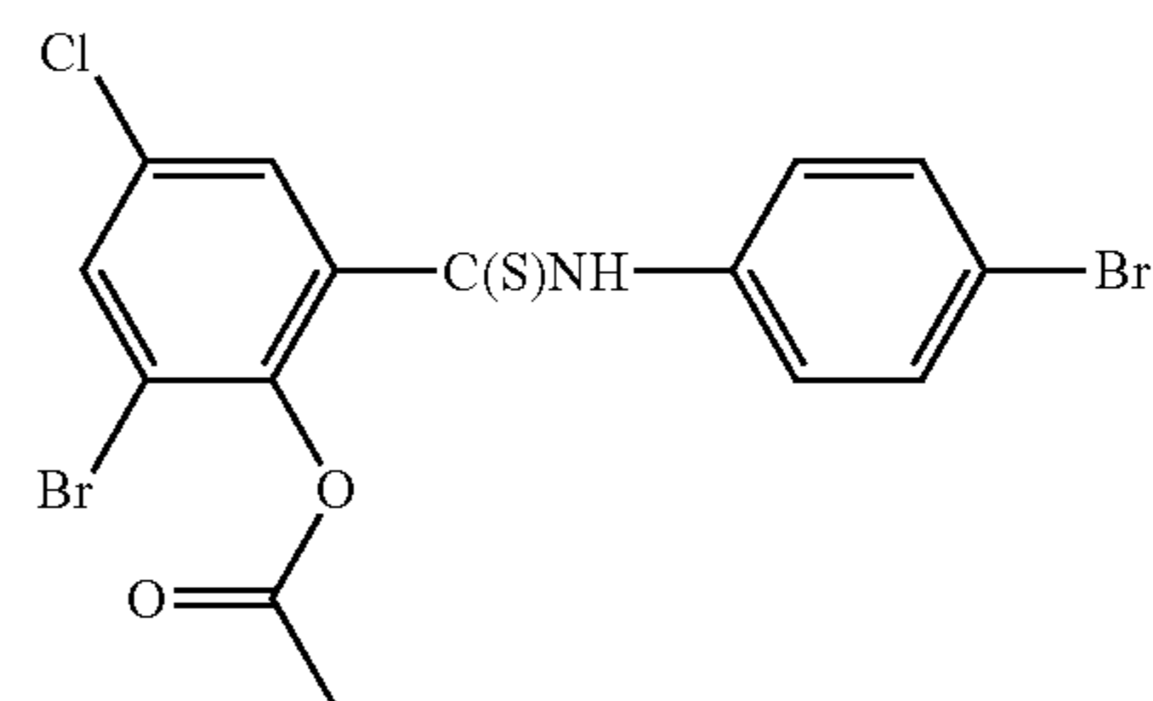
brotianide
