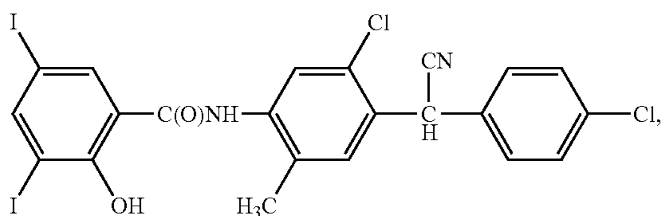
closantel
