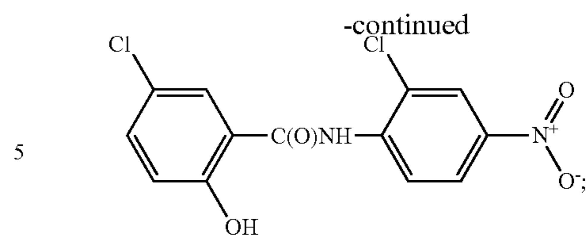
Niclosamine
