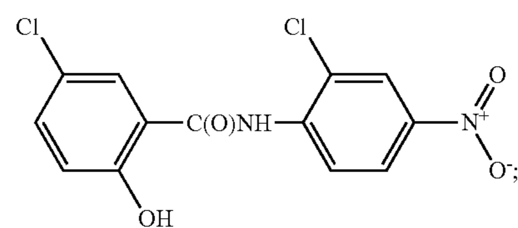
niclosamide
