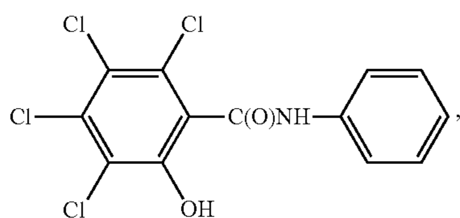
tetrachlorosalicylanilide
