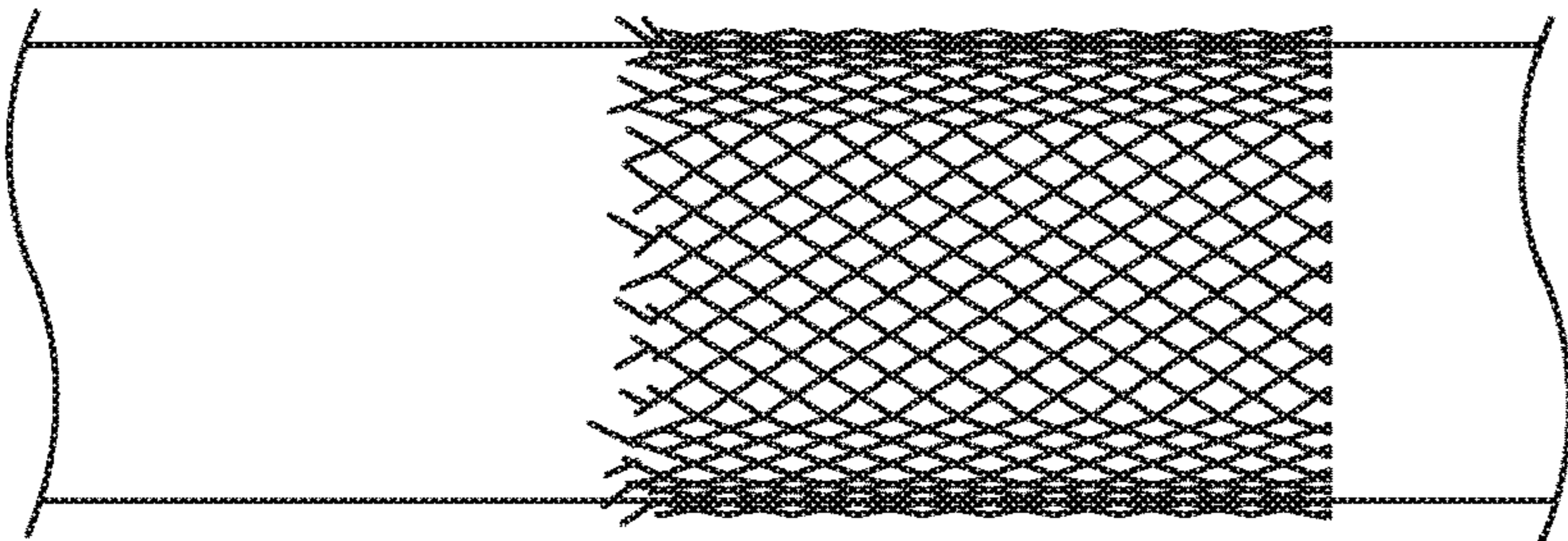
NITI braid with exposed fingers
