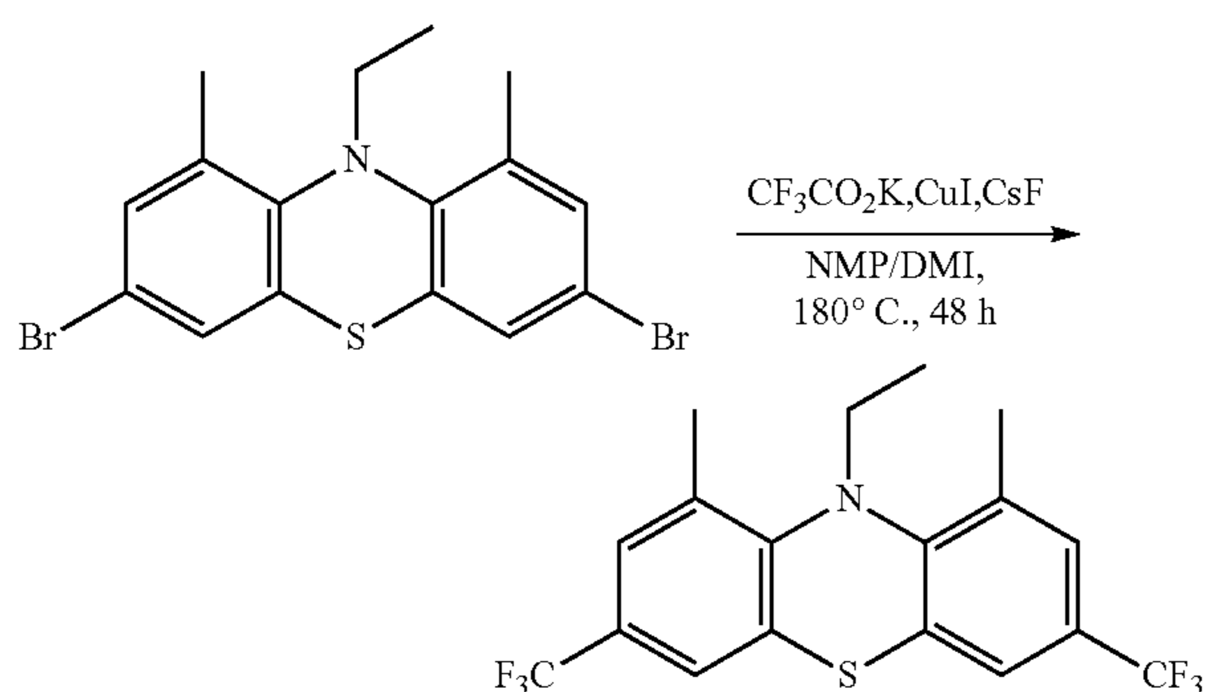
N-ethyl-1,9-dimethyl-3,7-bis(trifluoromethyl)phenothiazine (1,9-DMe-3,7 BCF3EPT)
