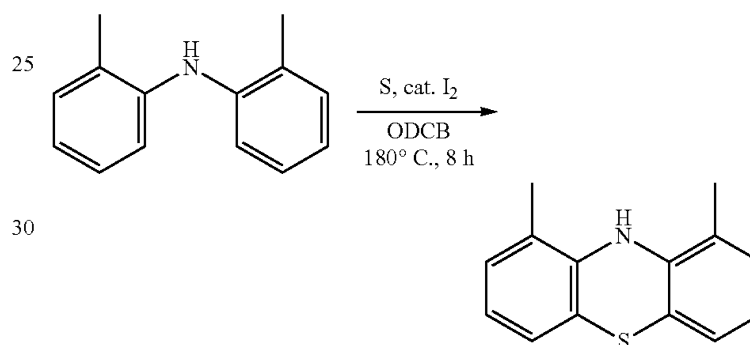
1,9-Dimethylphenothiazine (1,9-DMePT)
