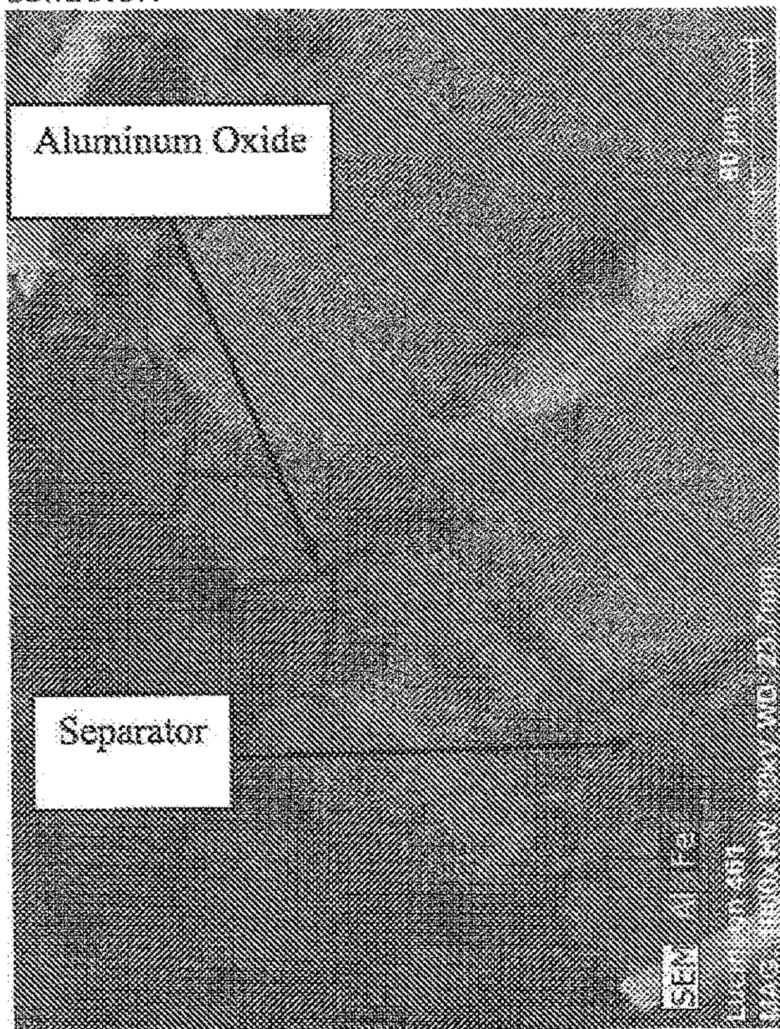
Figure 3B: SEM of cross section of nail penetrated cell: zoom on aluminum current collector.
