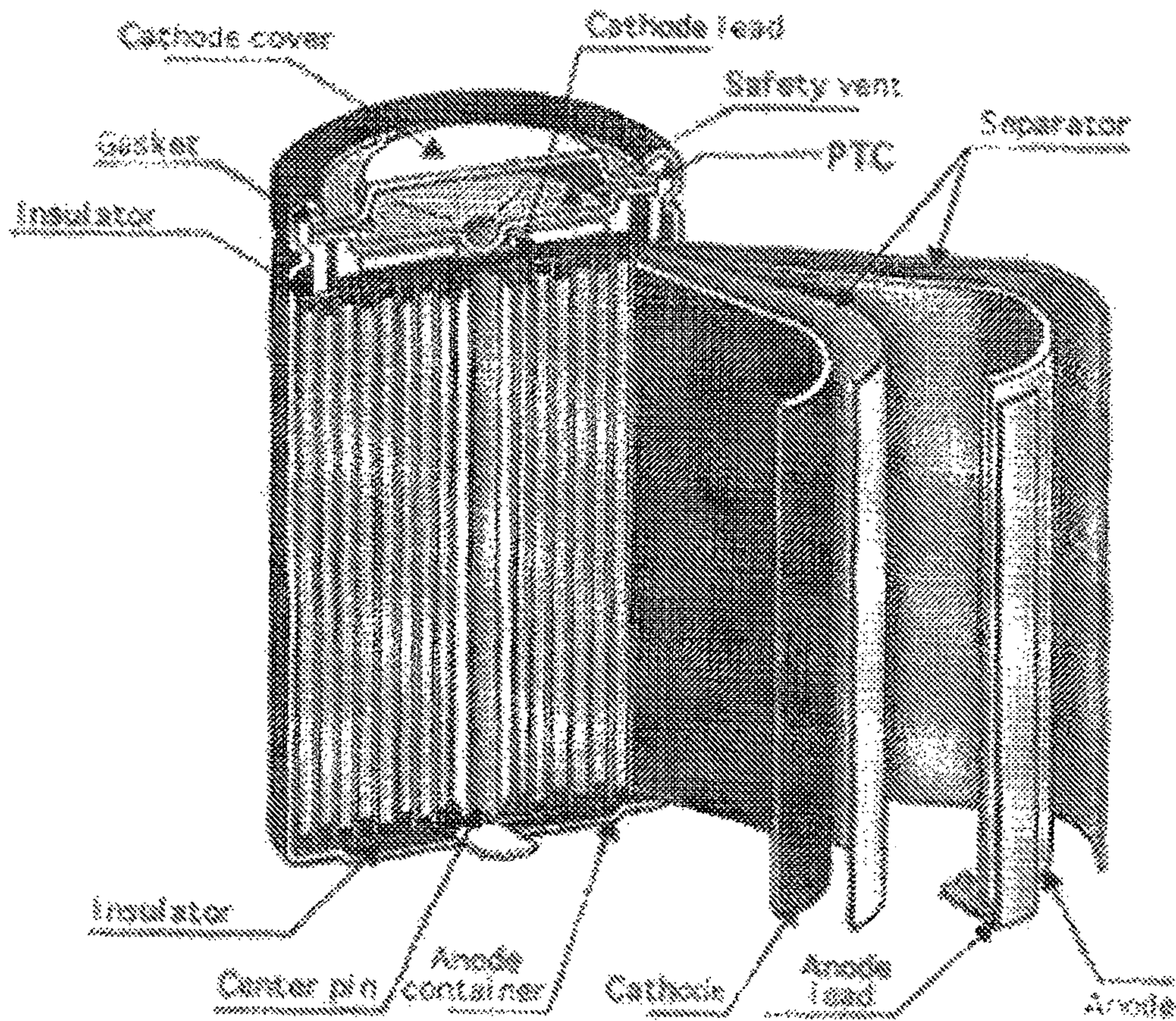
Figure 1—Wound cell
