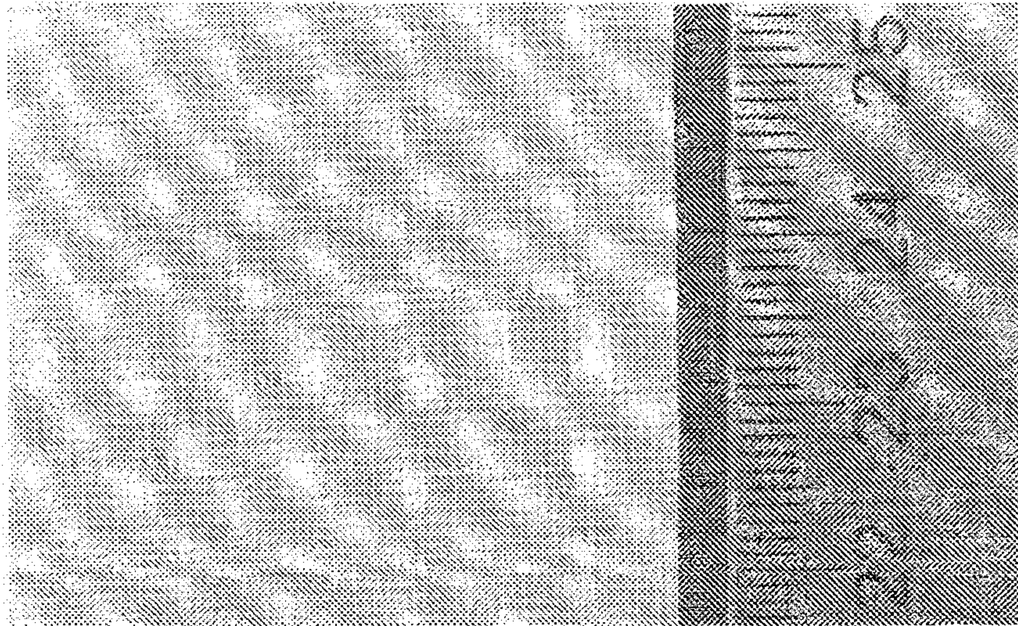
Example 6 after touching with hot solder iron
