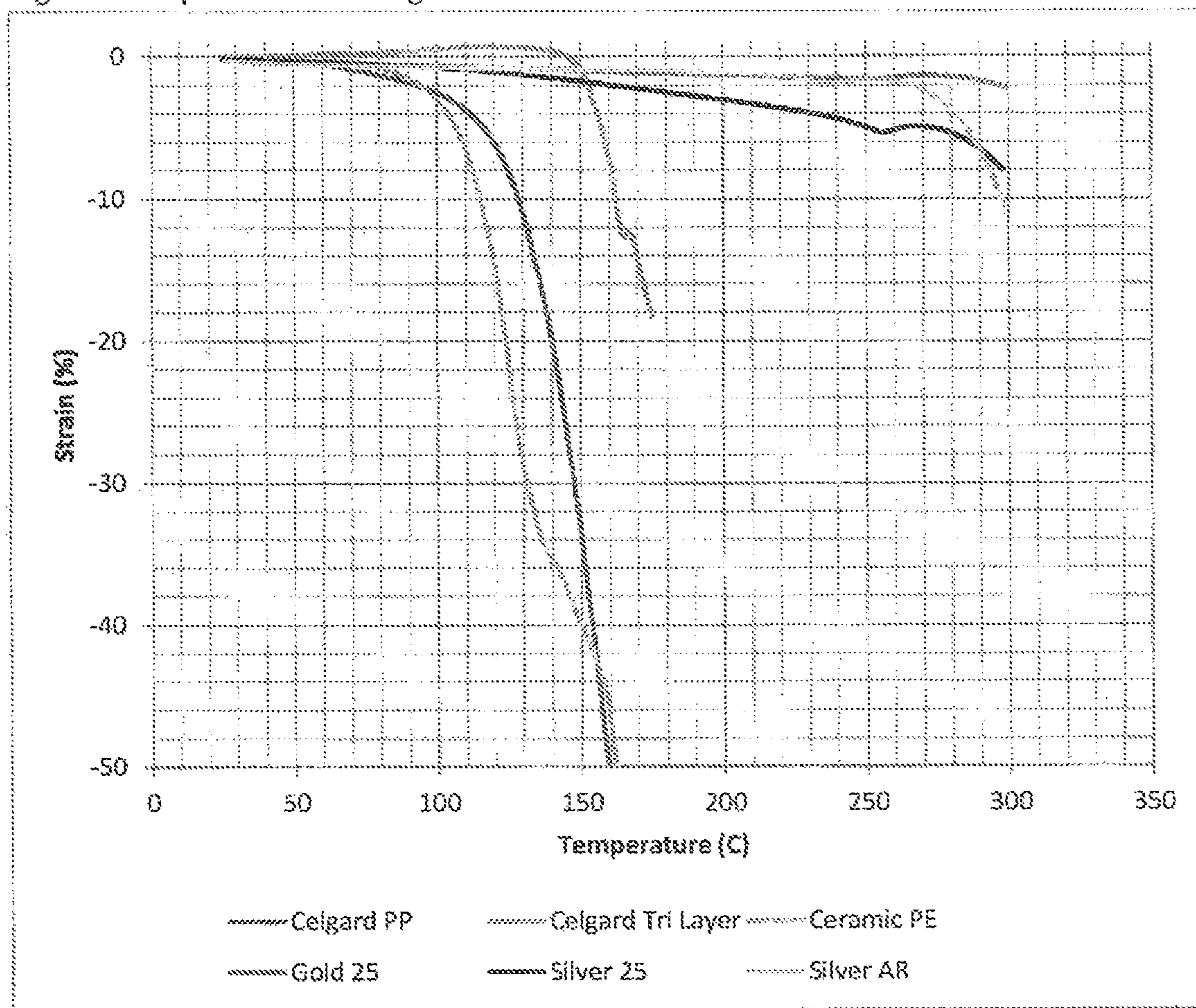
Figure 2: Separator Shrinkage
