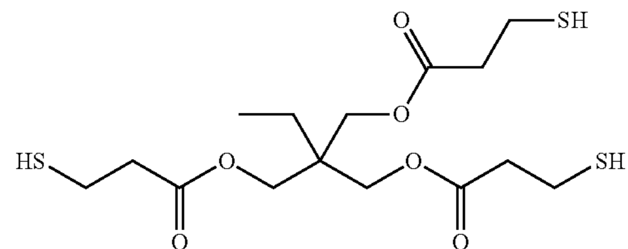
Chemical Formula 1-3
