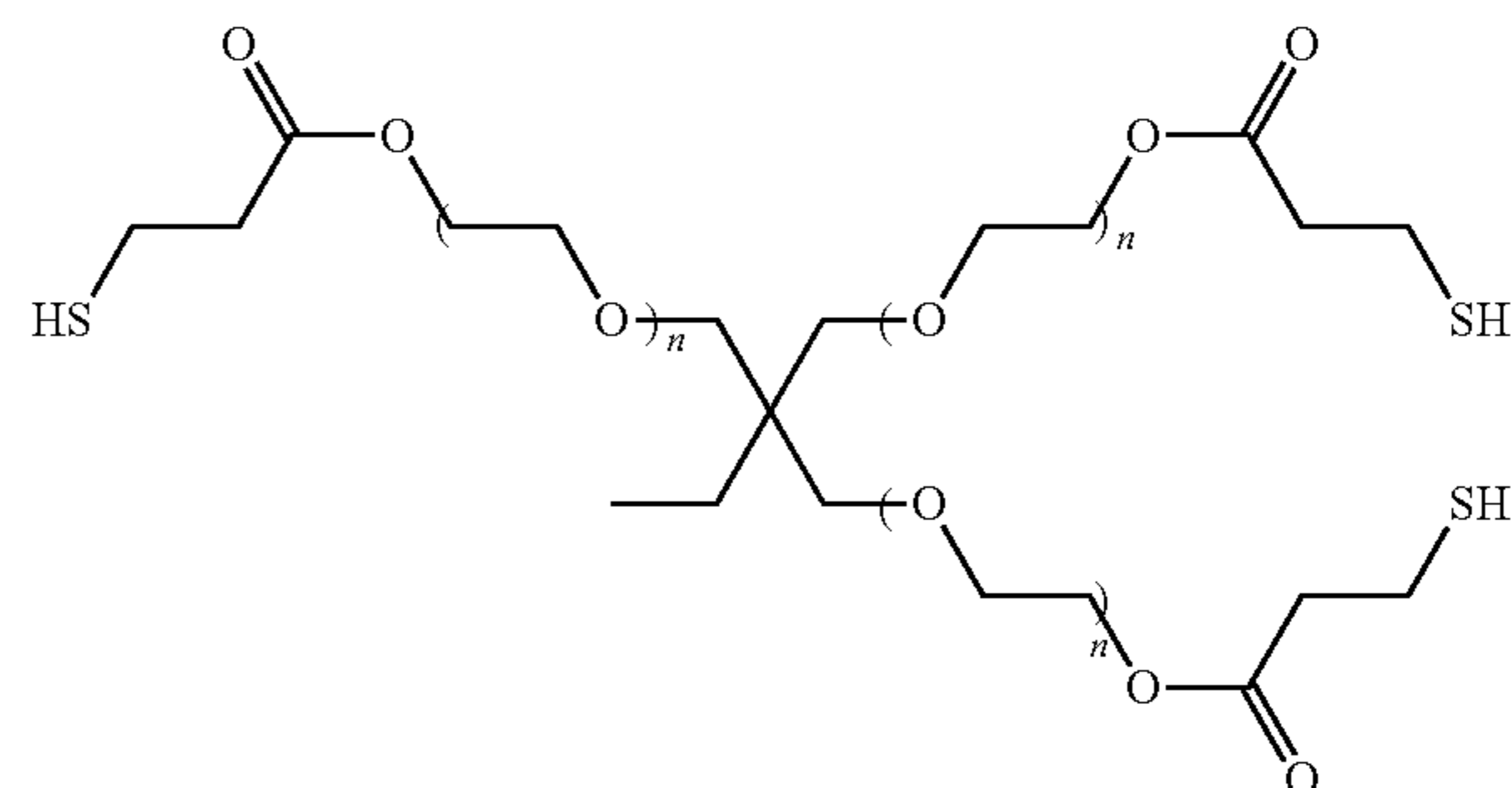
Chemical Formula 1-6
