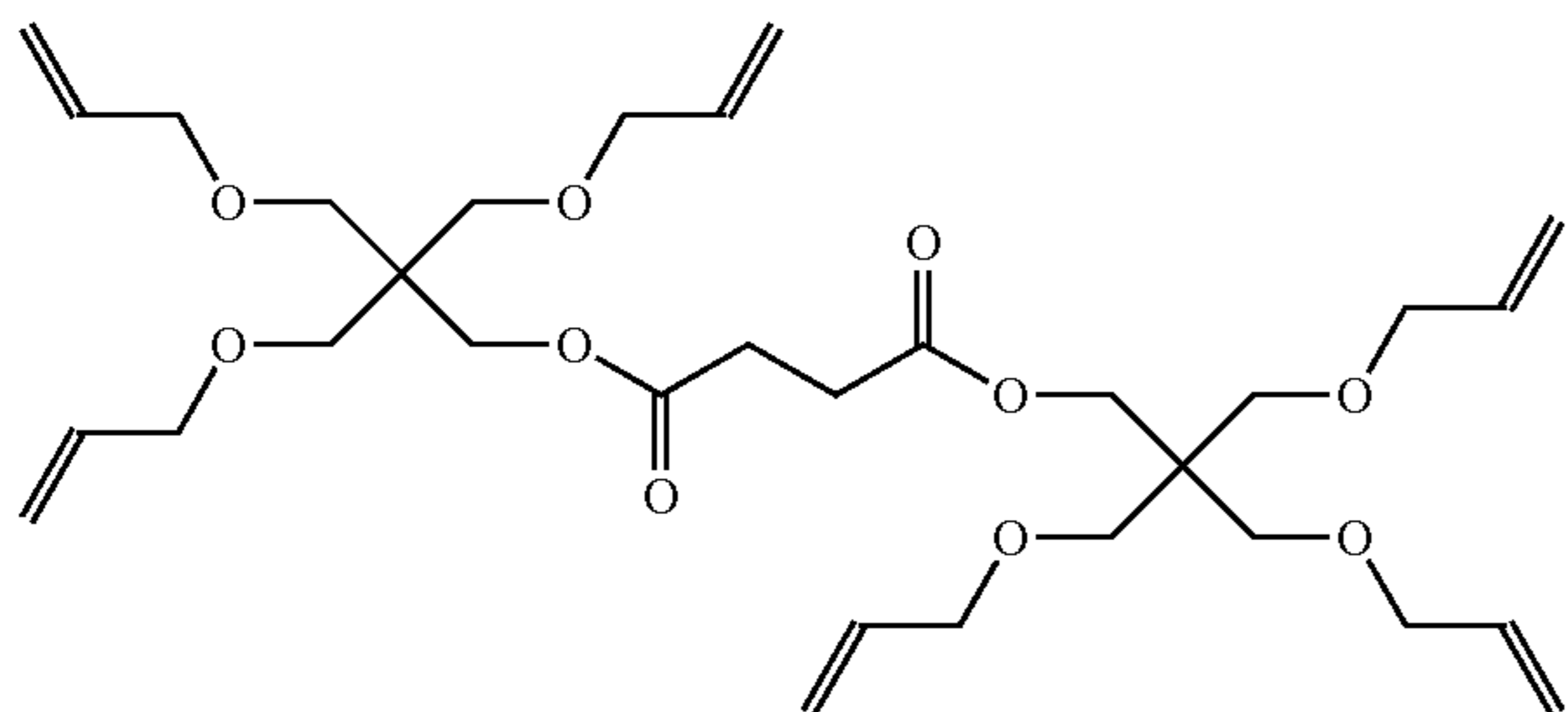
Chemical Formula 2-15
