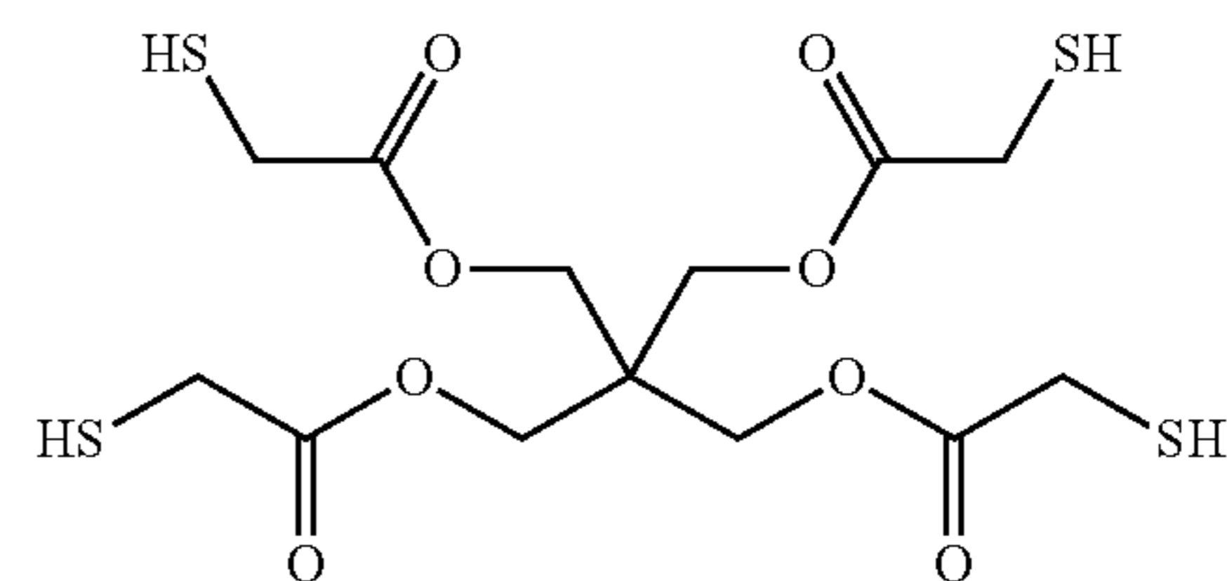
Chemical Formula 1-4
