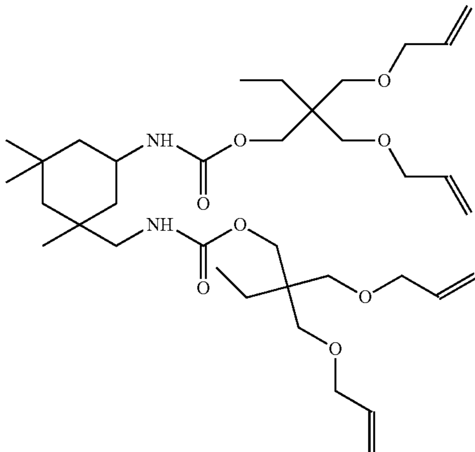
Chemical Formula 2-14
