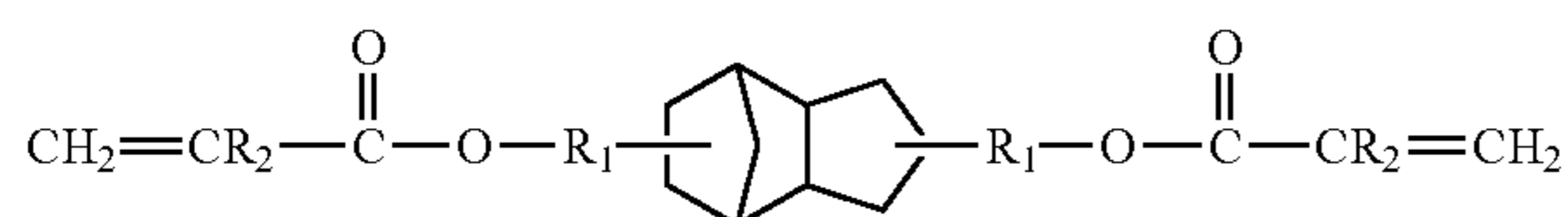
Chemical Formula 2-7
