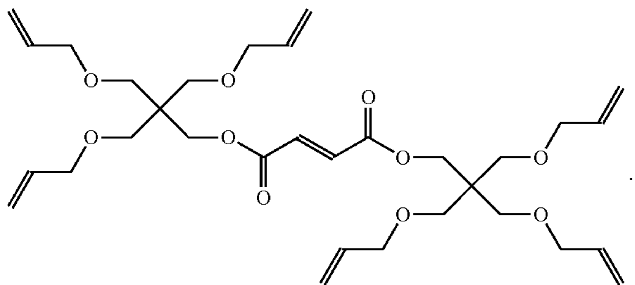
Chemical Formula 2-15
