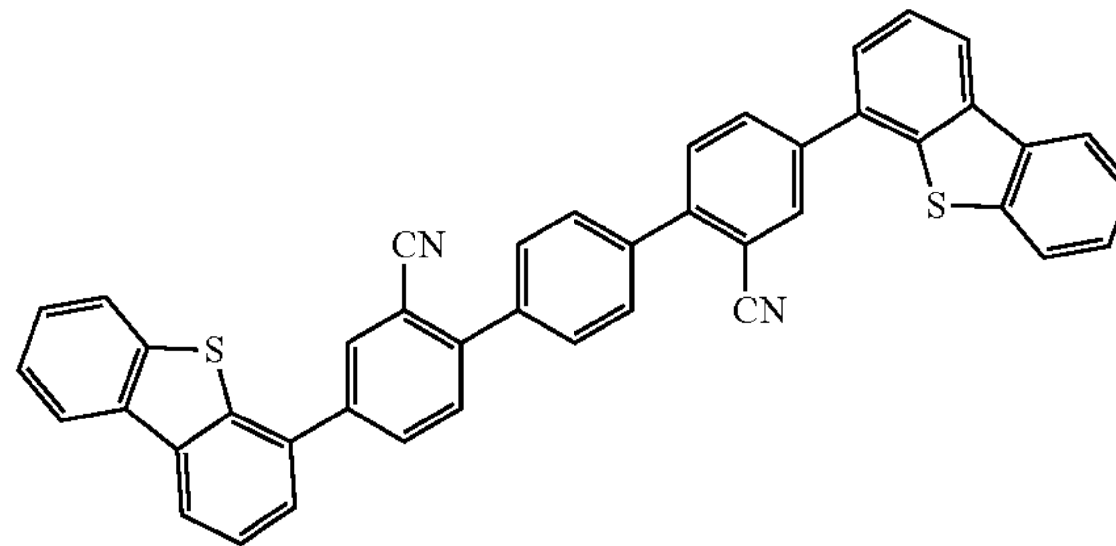
Compound 1B-17
