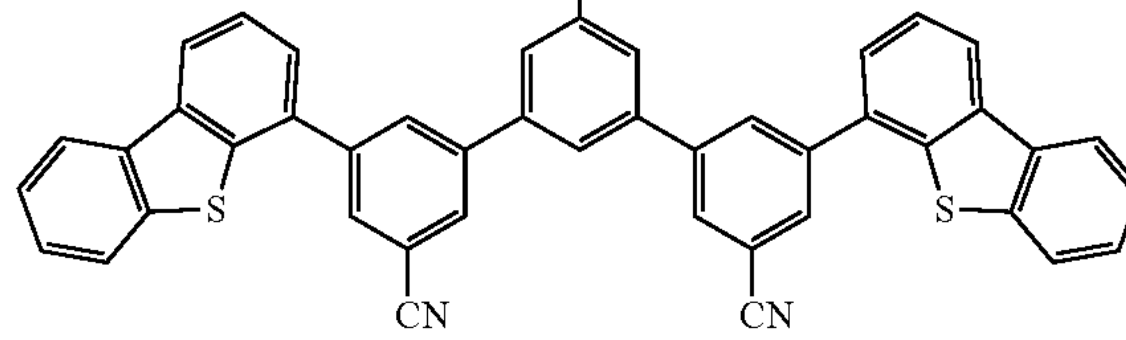
Compound 1B-14
