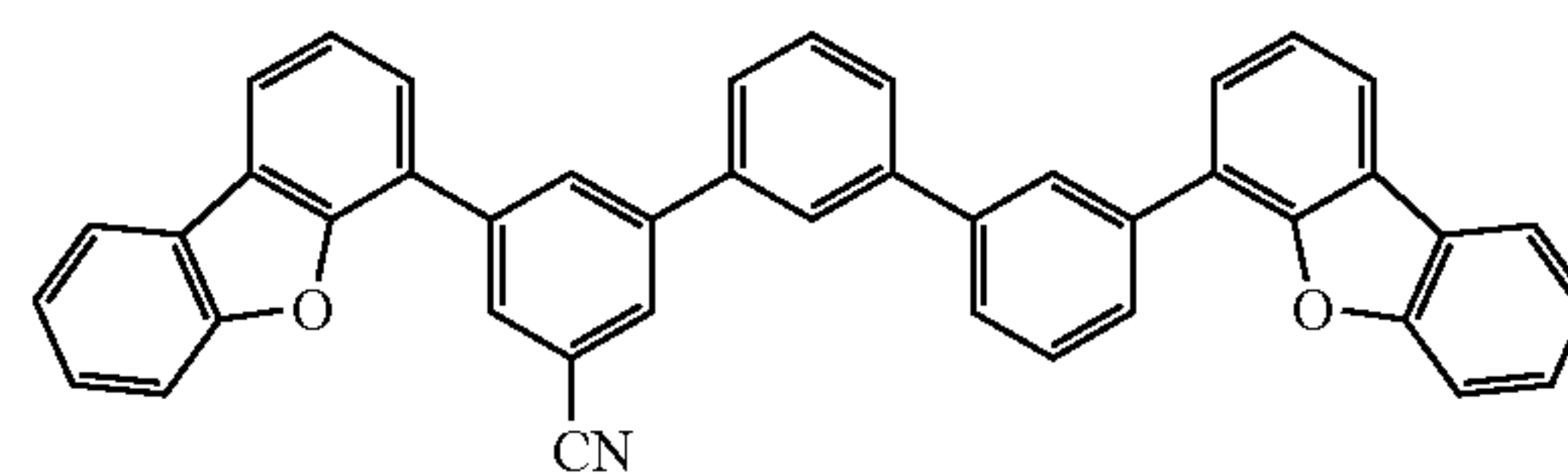
Compound 1A-7
