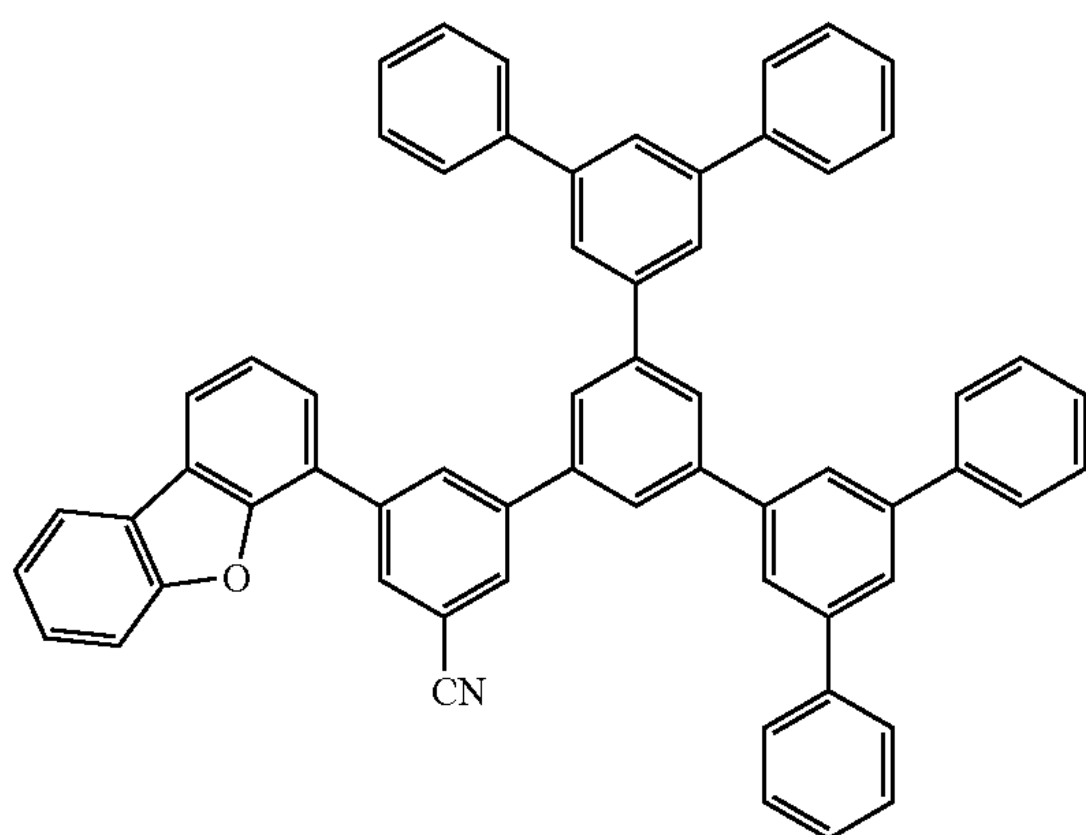
Compound 1A-3
