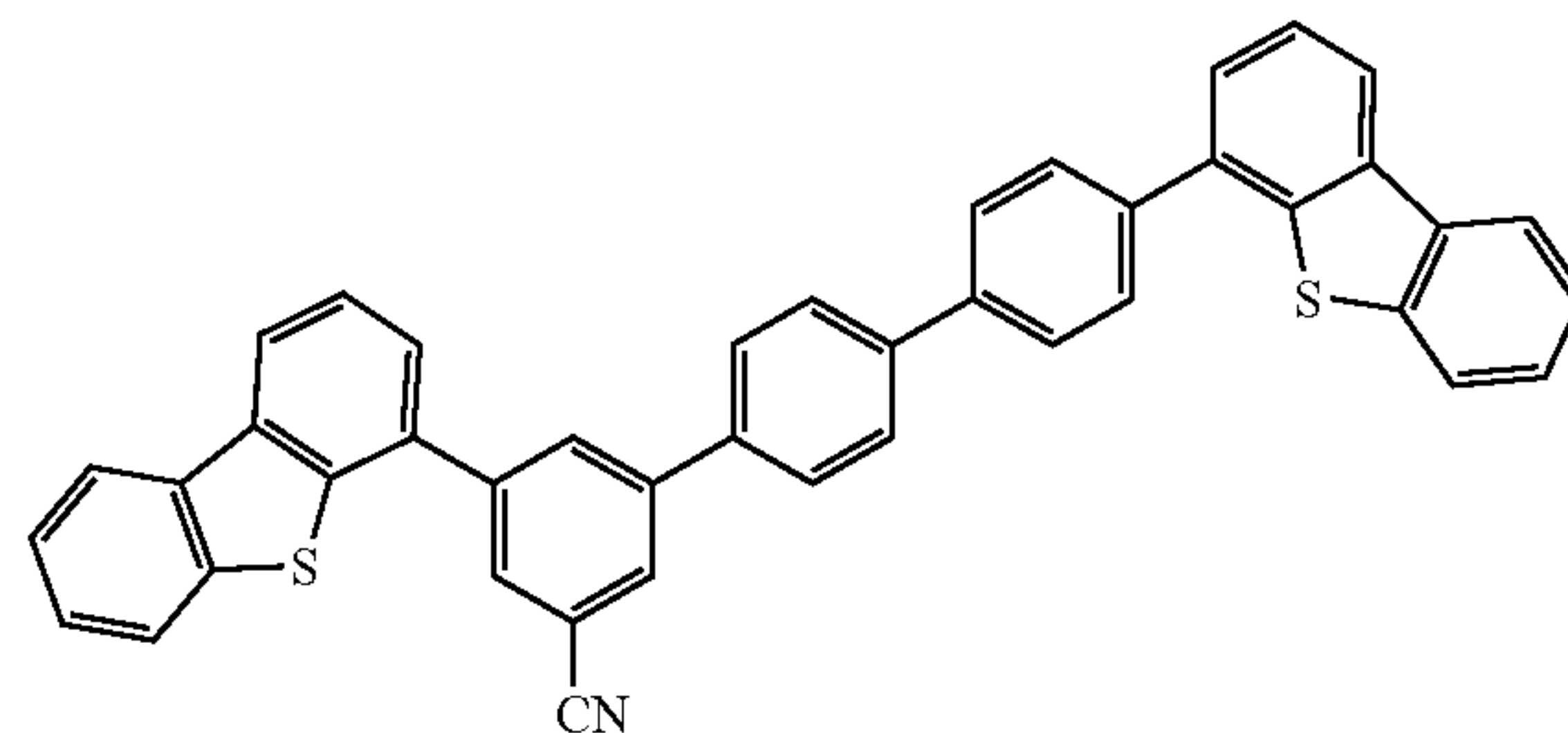
Compound 1B-16
