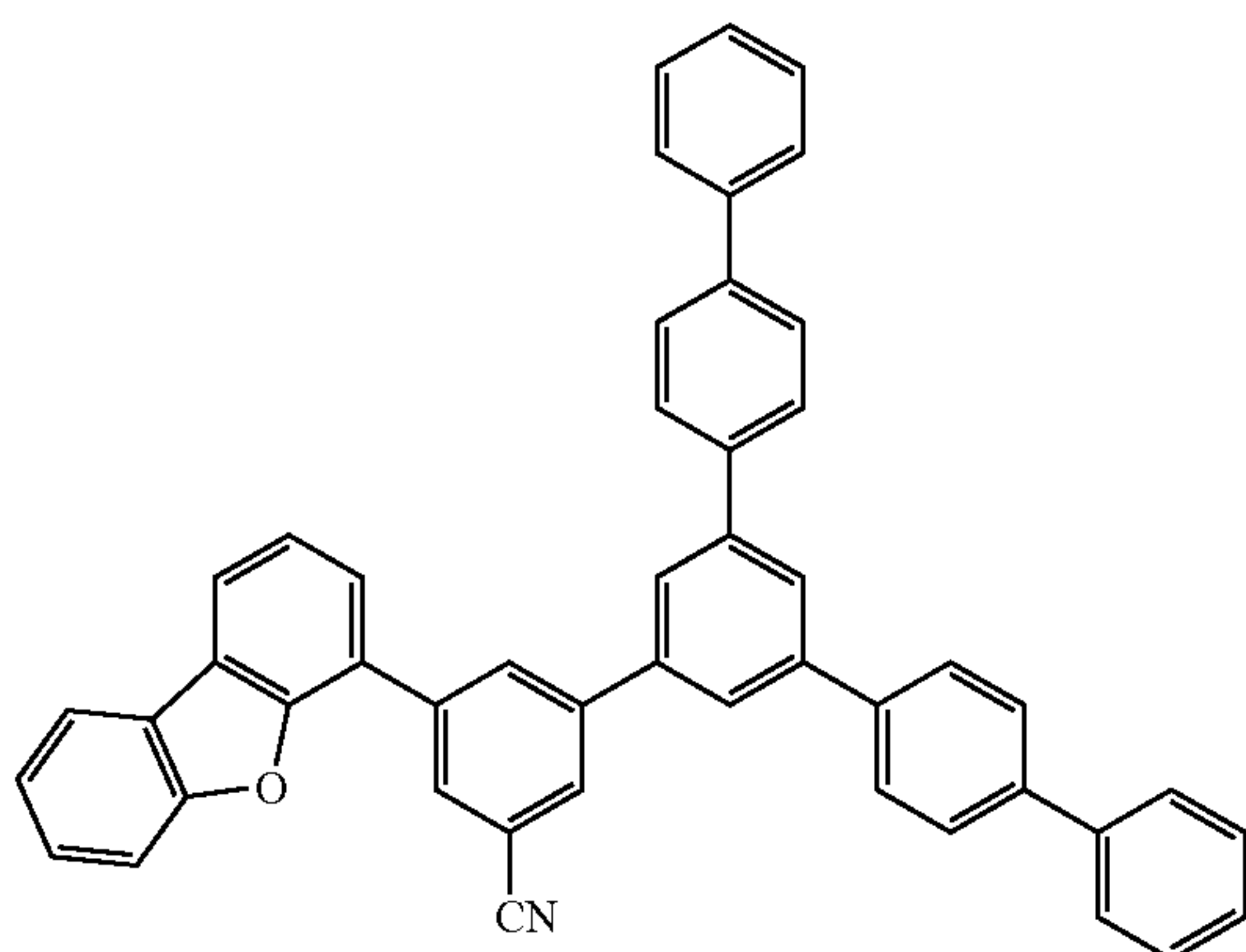
Compound 1A-3
