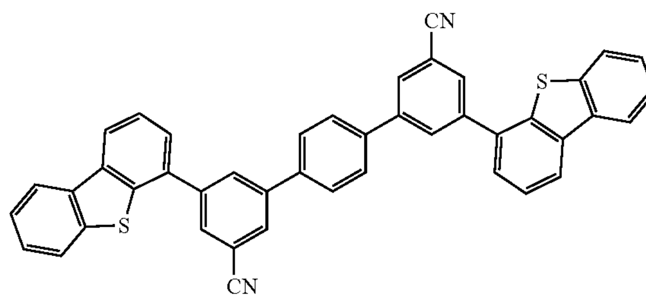
Compound 1B-15
