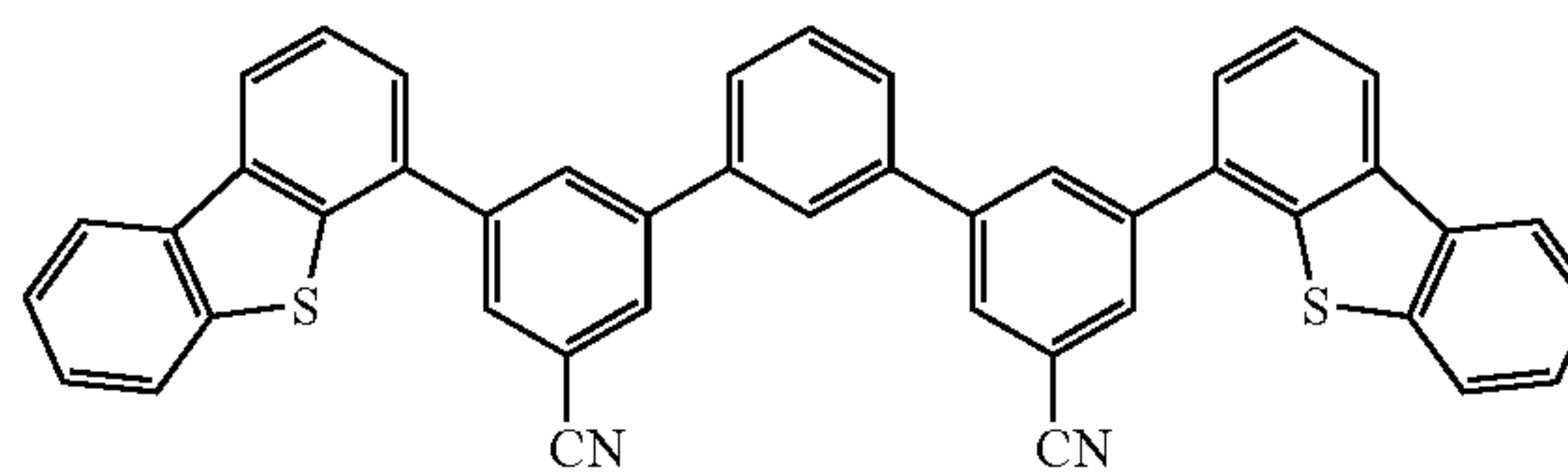
Compound 1B-5
