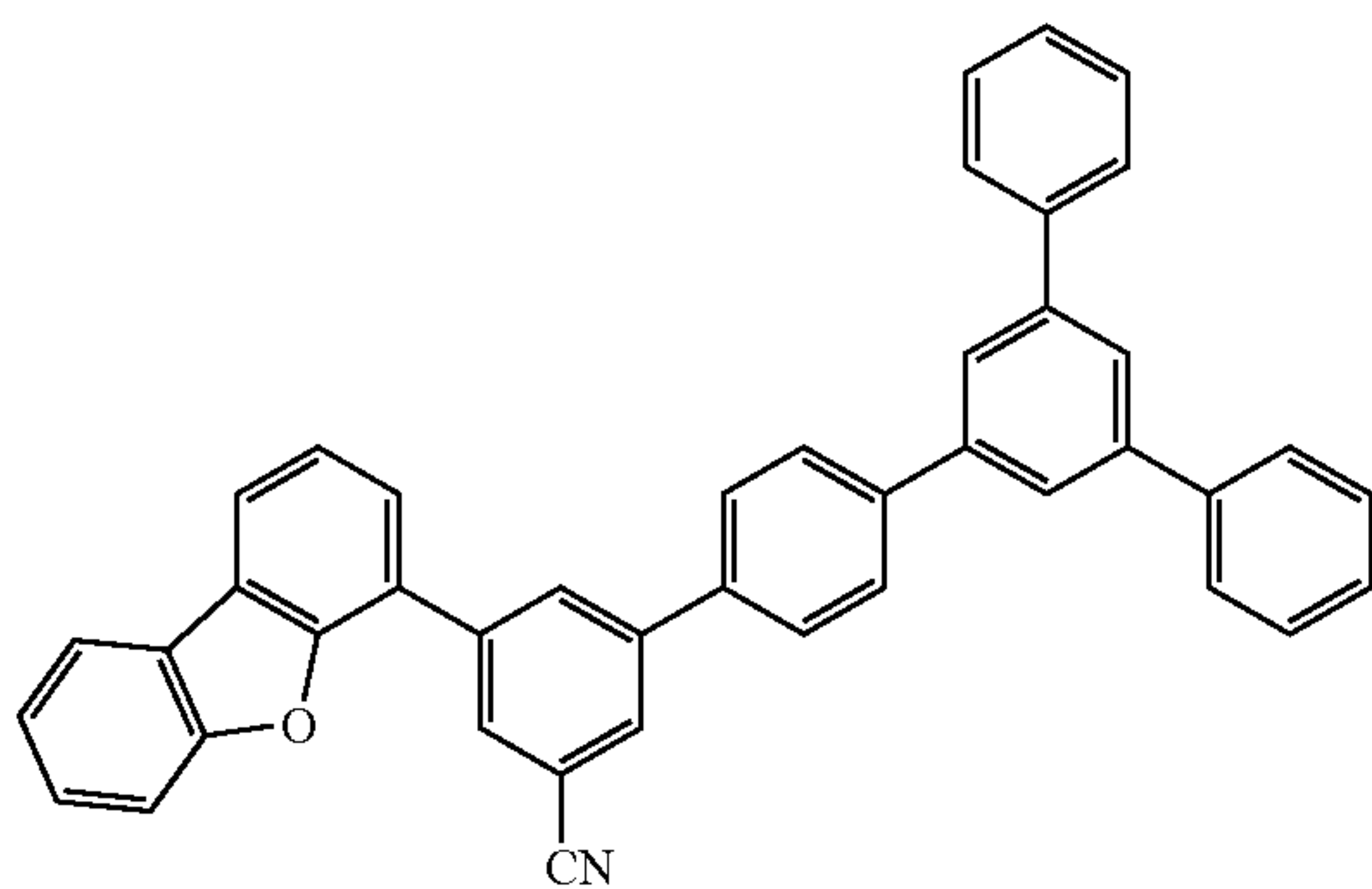
Compound 1A-4
