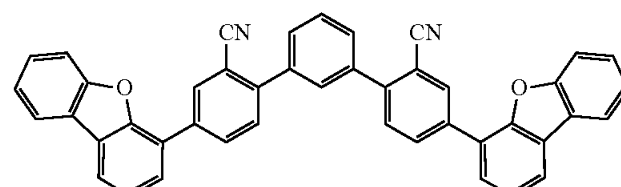
Compound 1A-9
