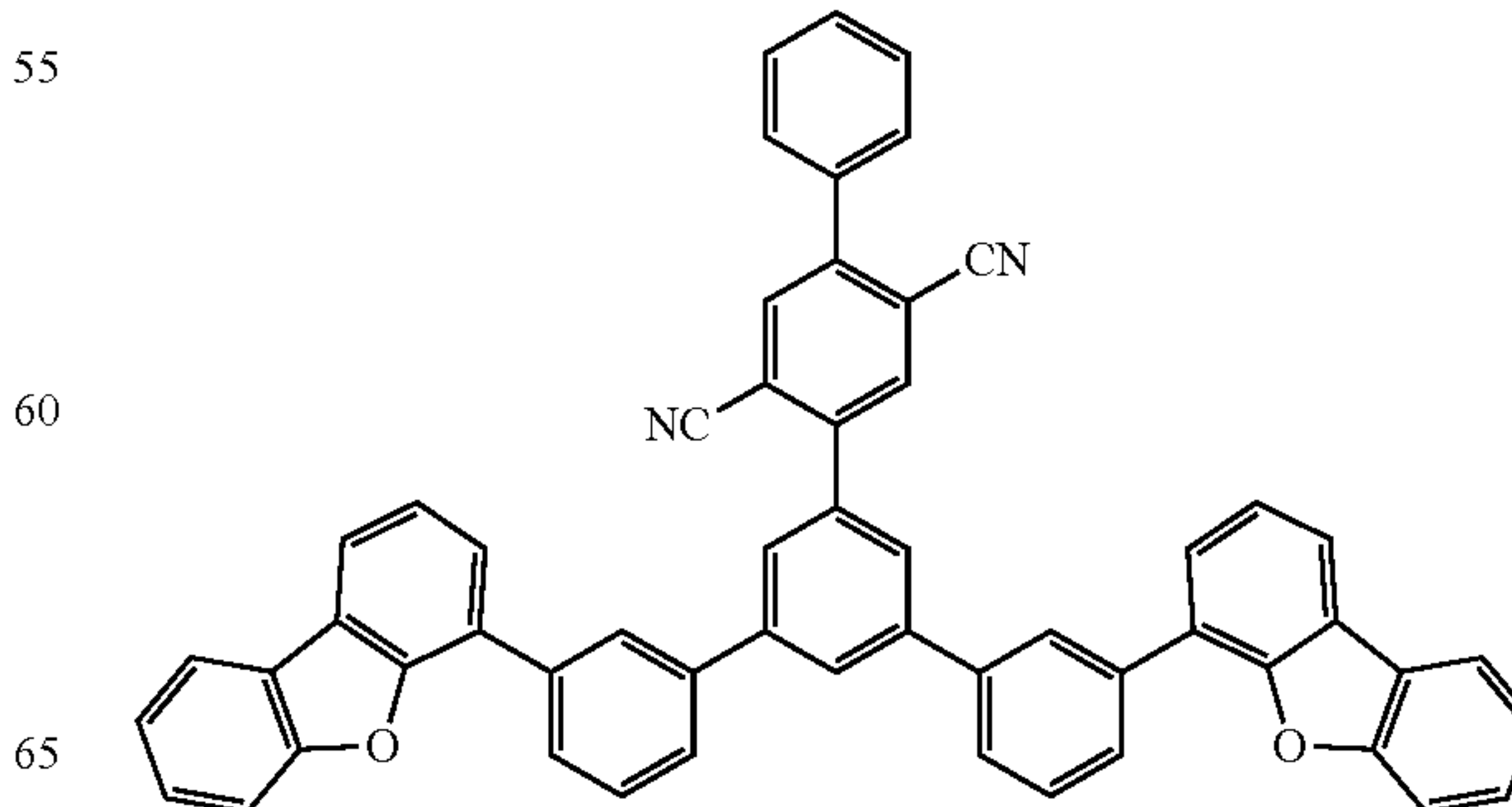
Compound 2A-13
