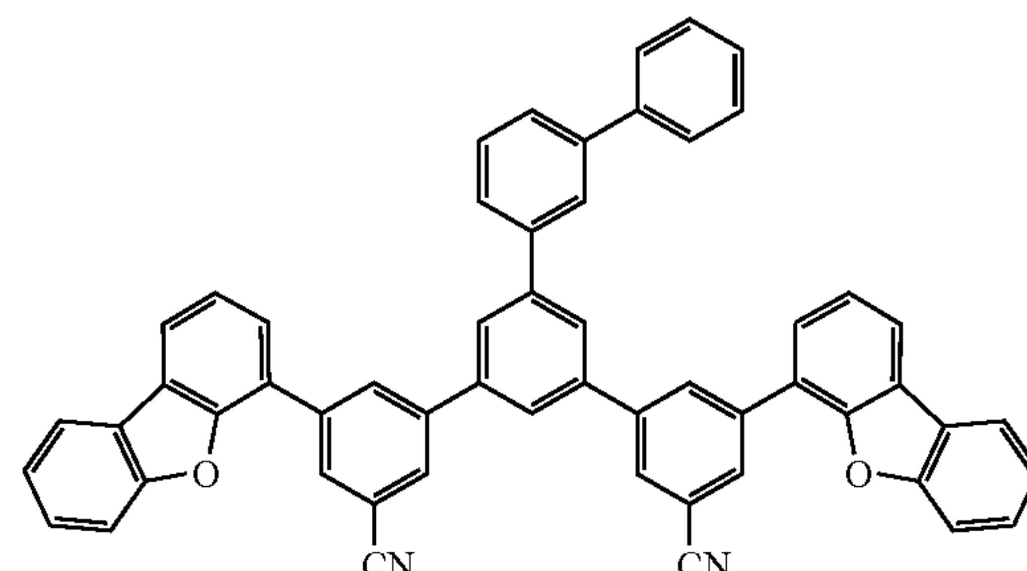
Compound 1A-11
