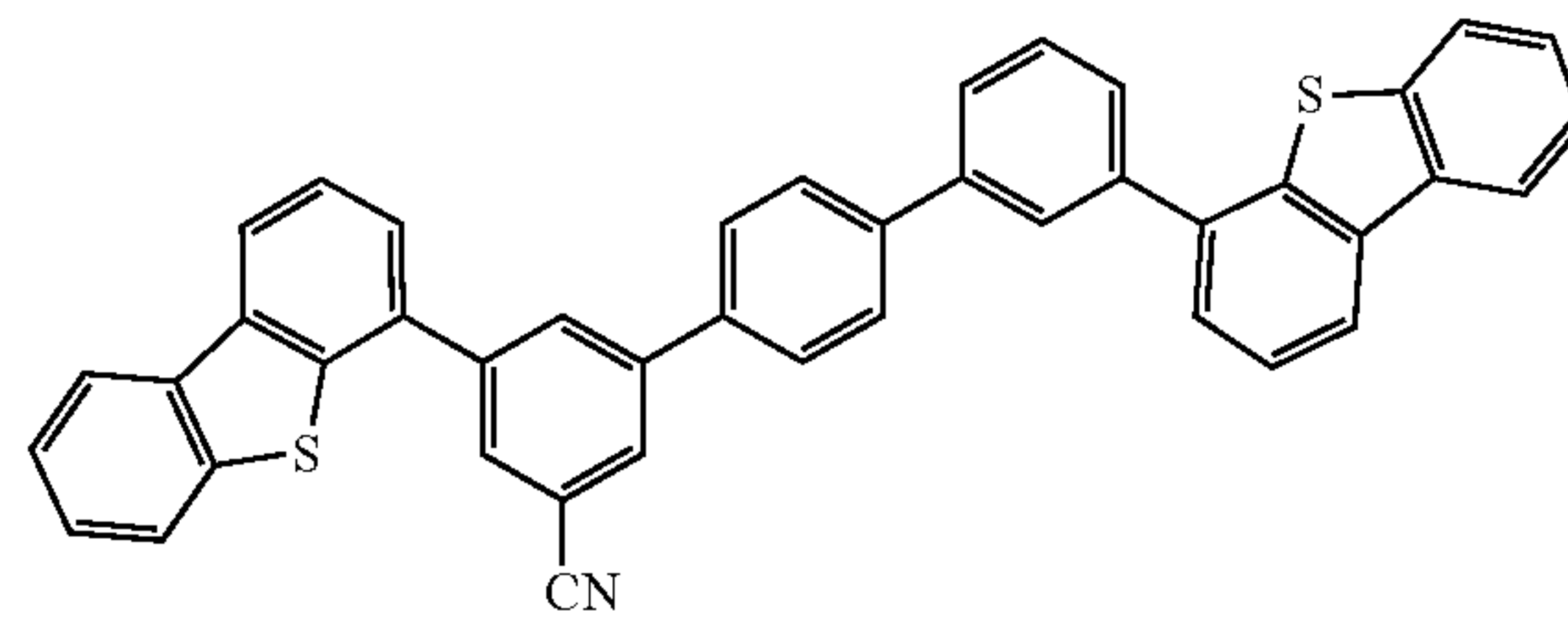
Compound 1B-16
