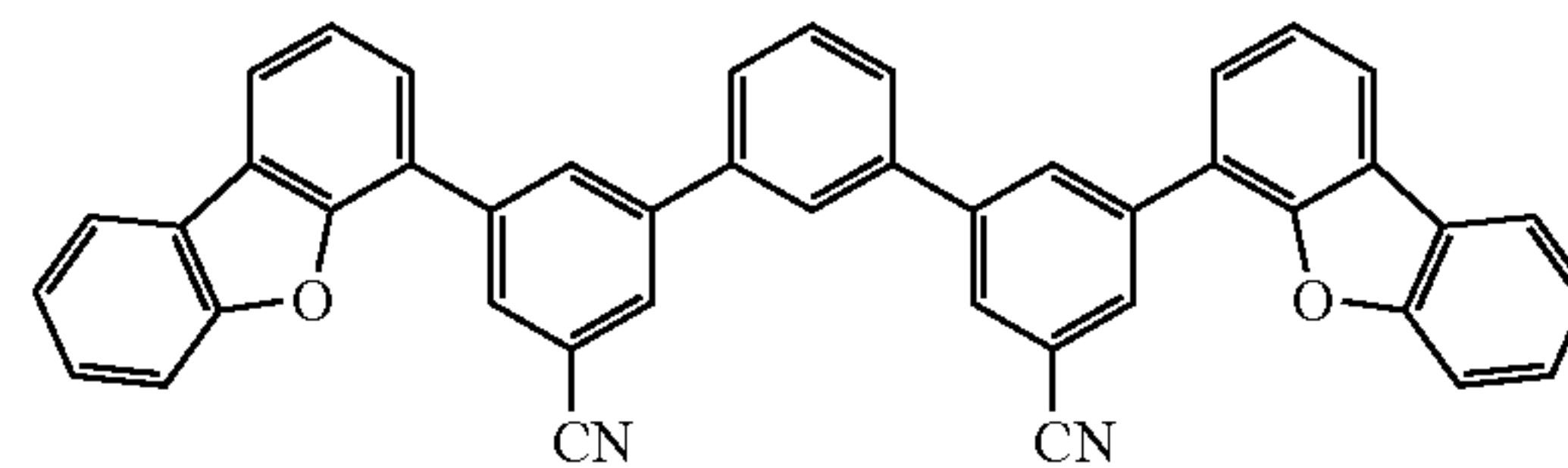
Compound 1A-6
