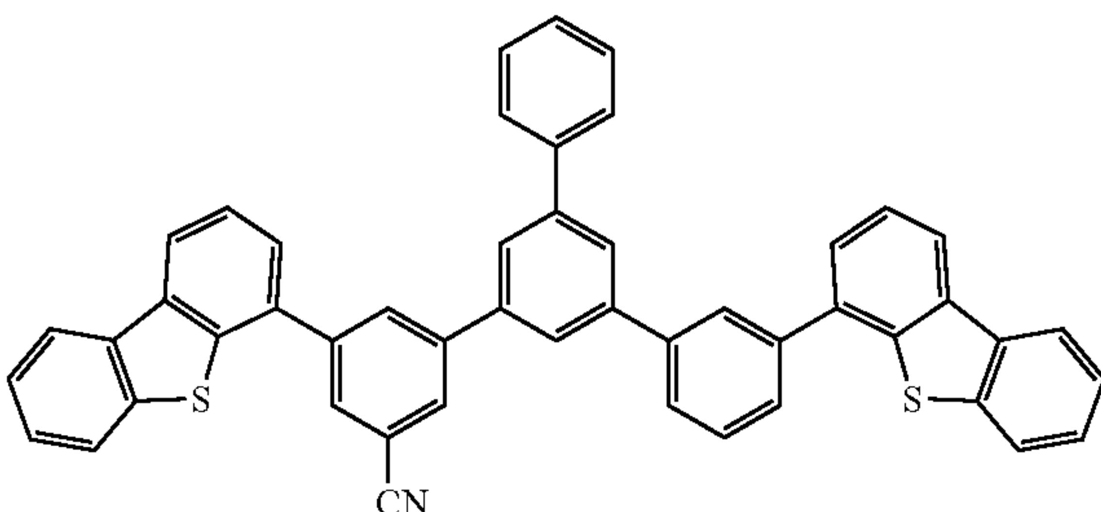
Compound 1B-12
