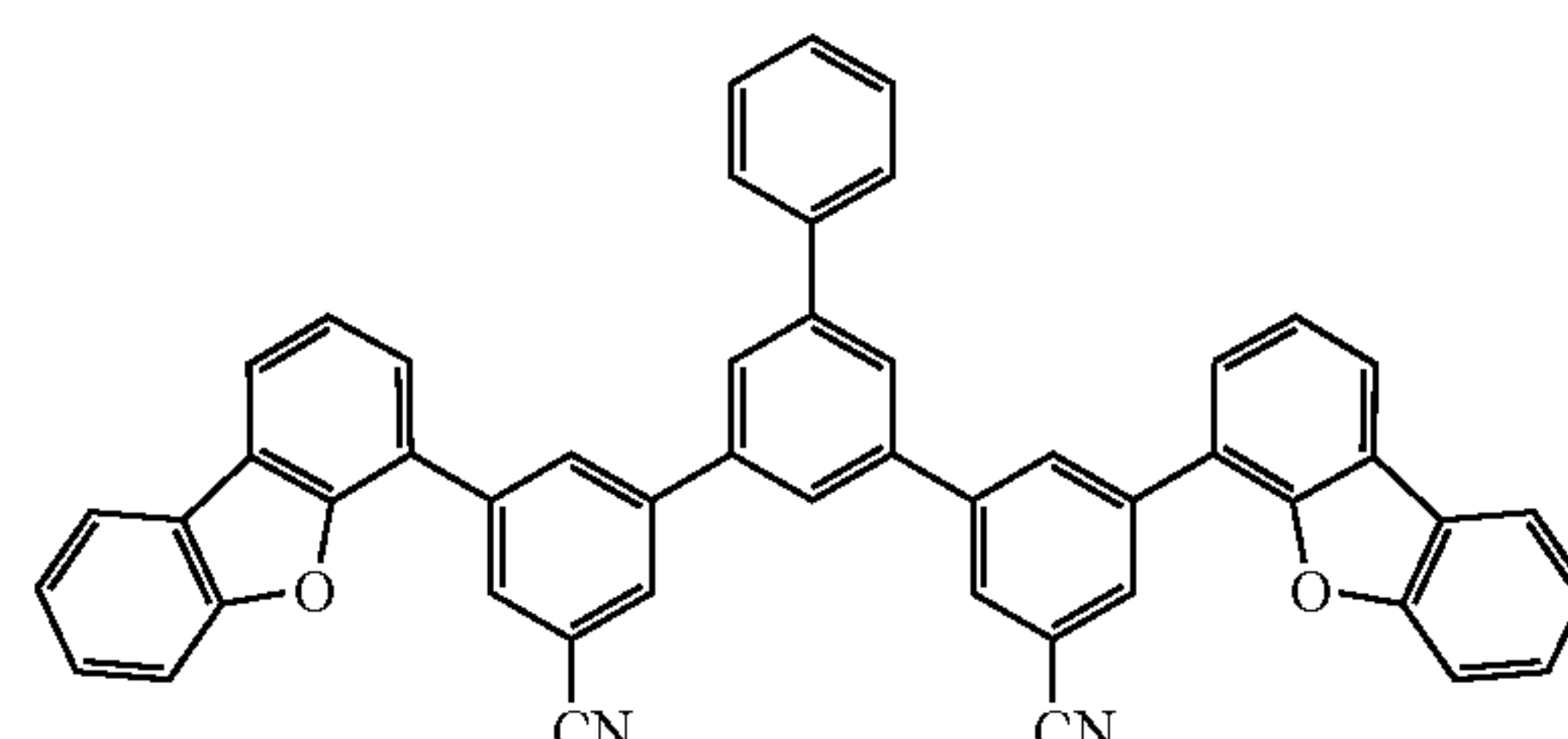
Compound 1A-10
