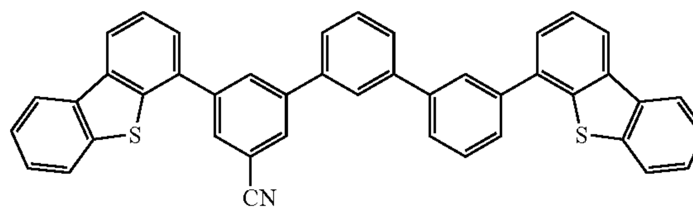
Compound 1B-6
