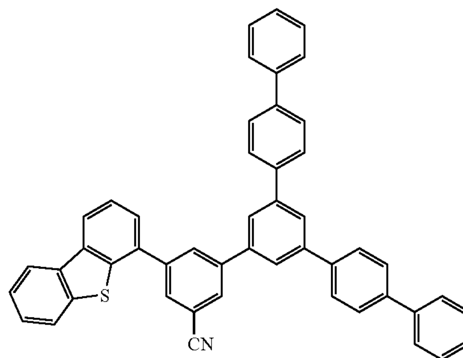
Compound 1B-3
