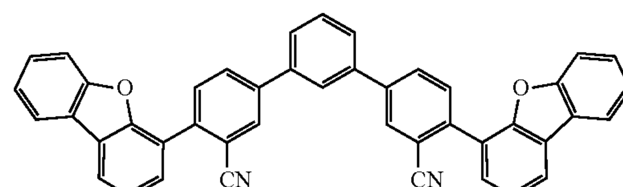
Compound 1A-10
