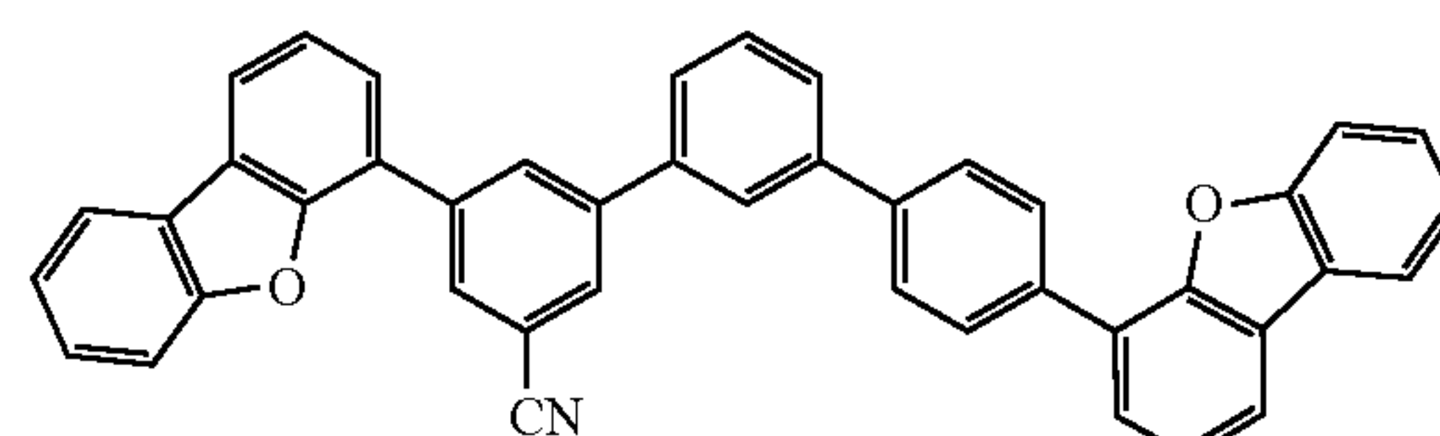
Compound 1A-8
