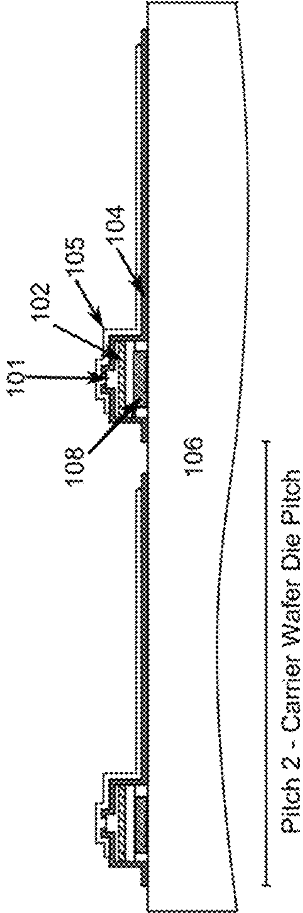
Die Expanded Laser Diode:
