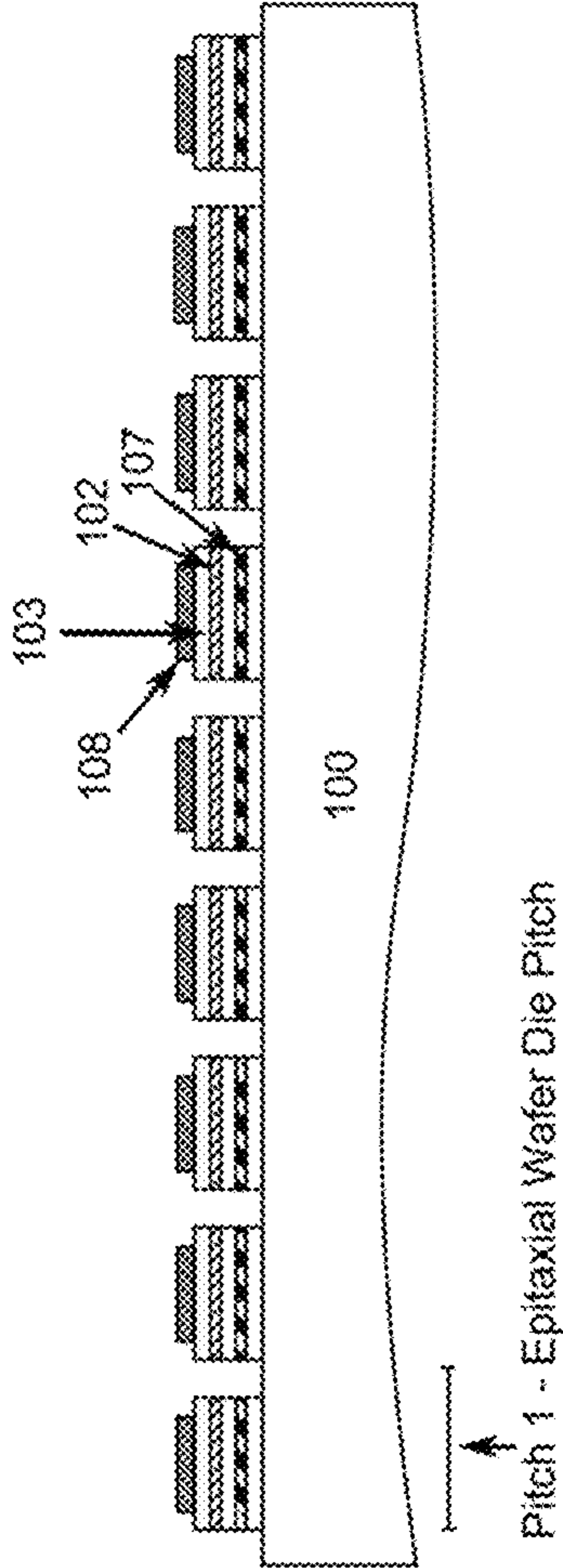
Epitaxial Wafer Before Die Expansion
