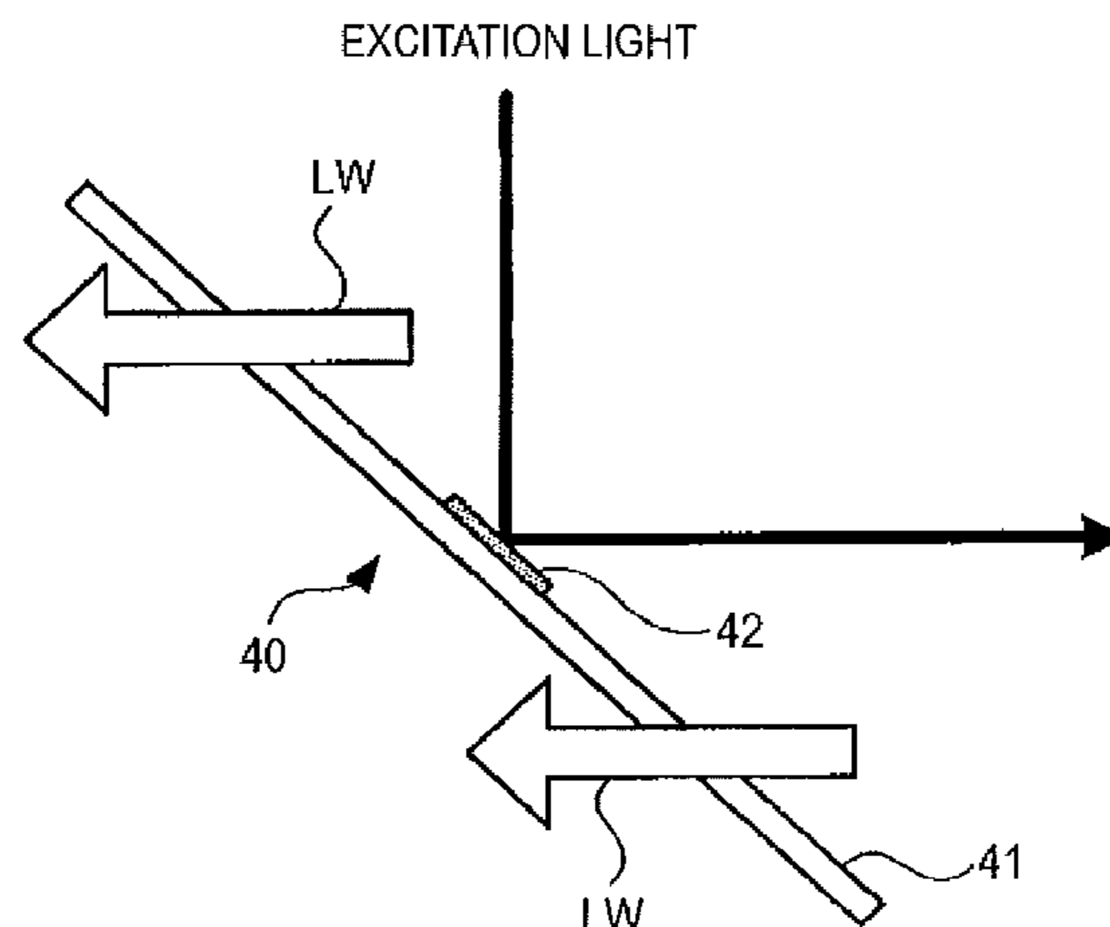
CONFIGURATION OF SPECTRAL OPTICAL SYSTEM OF MODIFIED EXAMPLE 1
