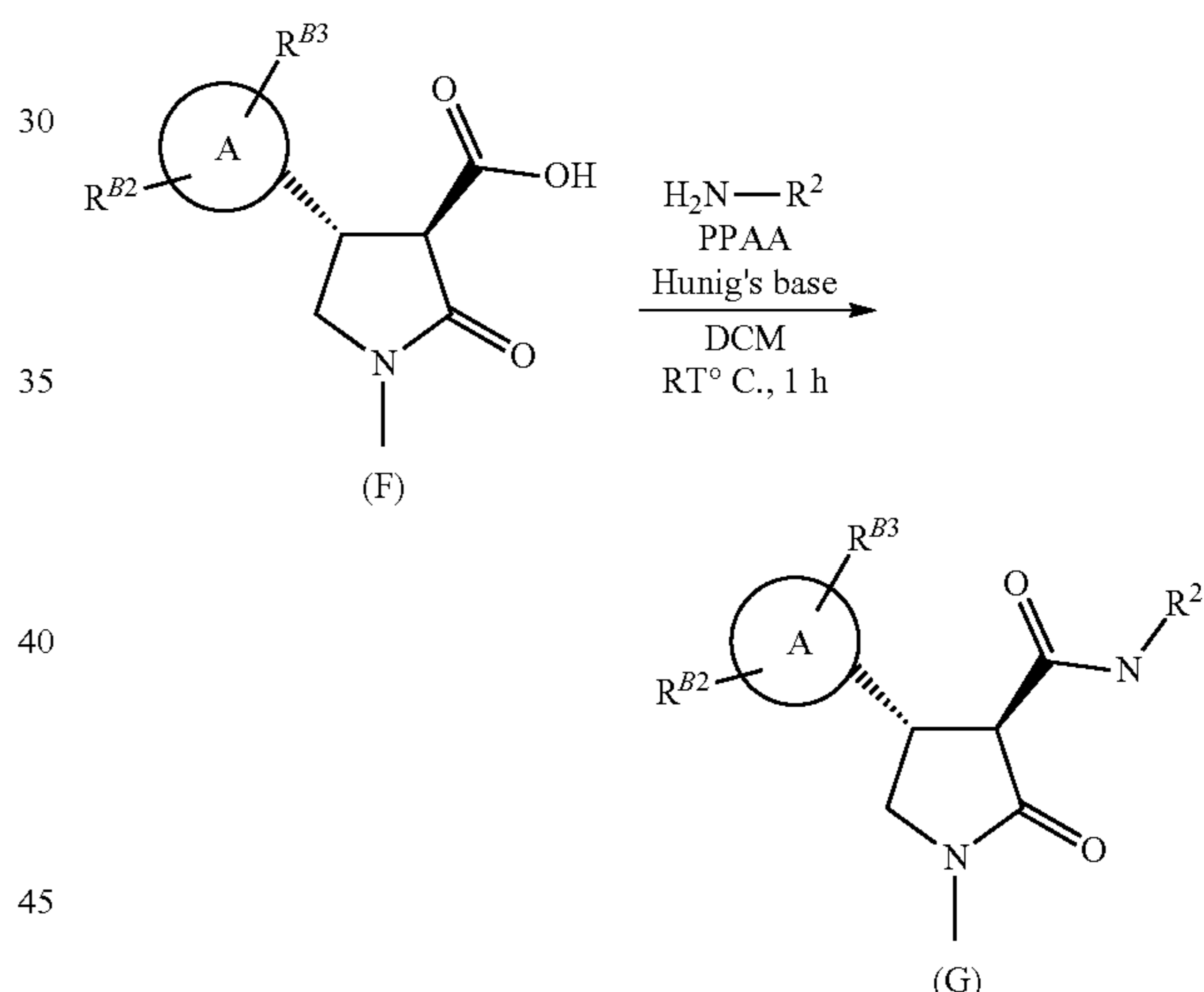
Reaction scheme 6
