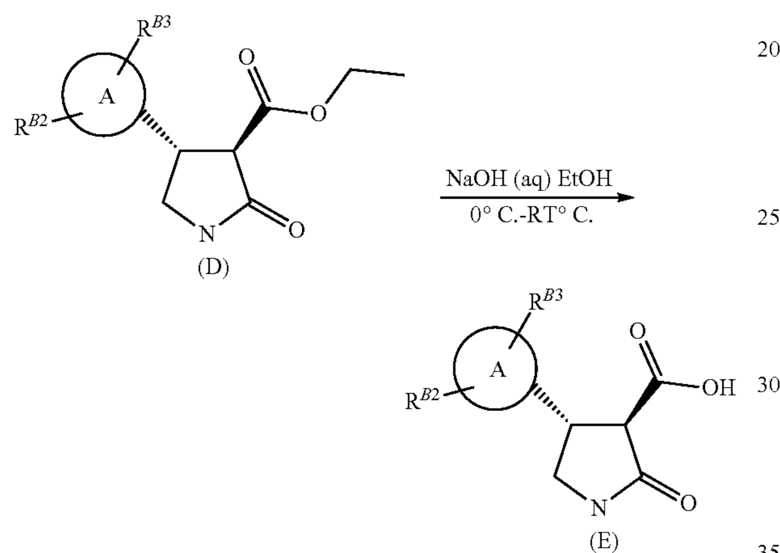
Reaction scheme 4
