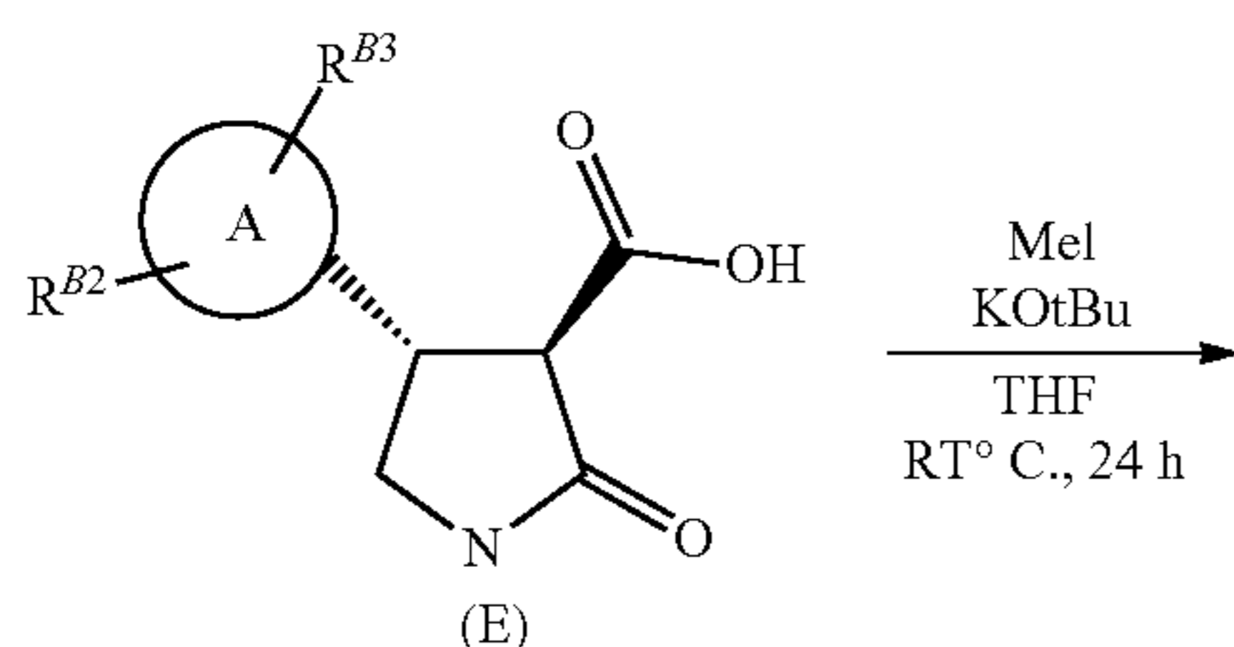
Reaction scheme 5
