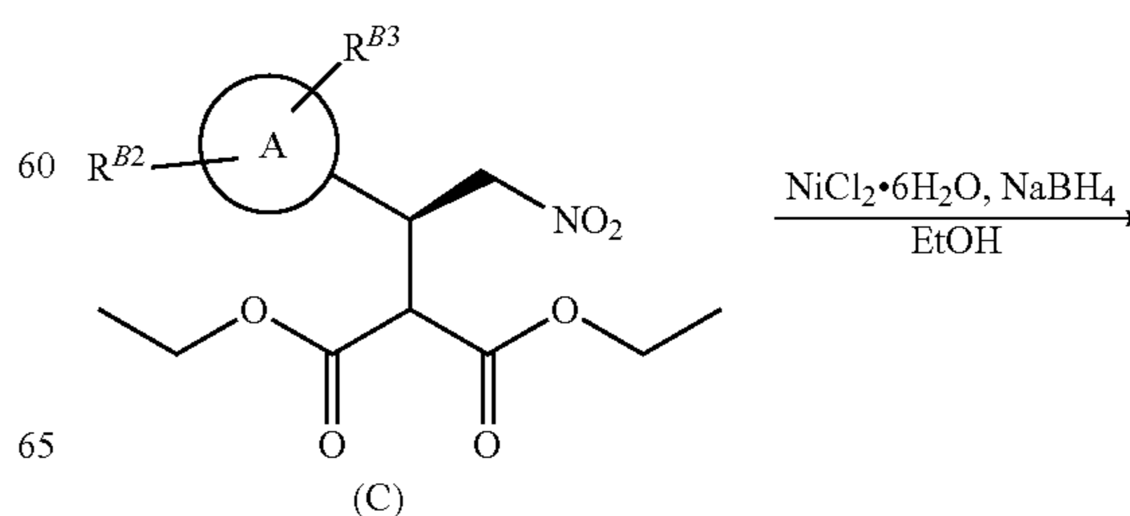
Reaction scheme 3
