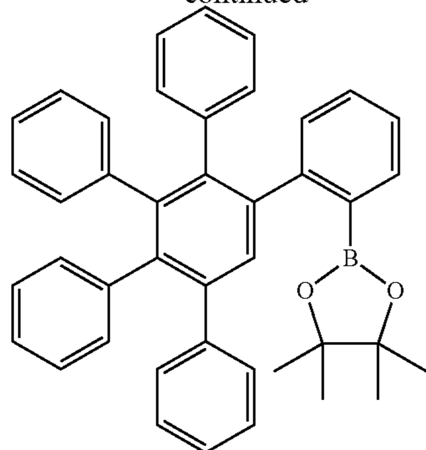
Intermediate I-25
