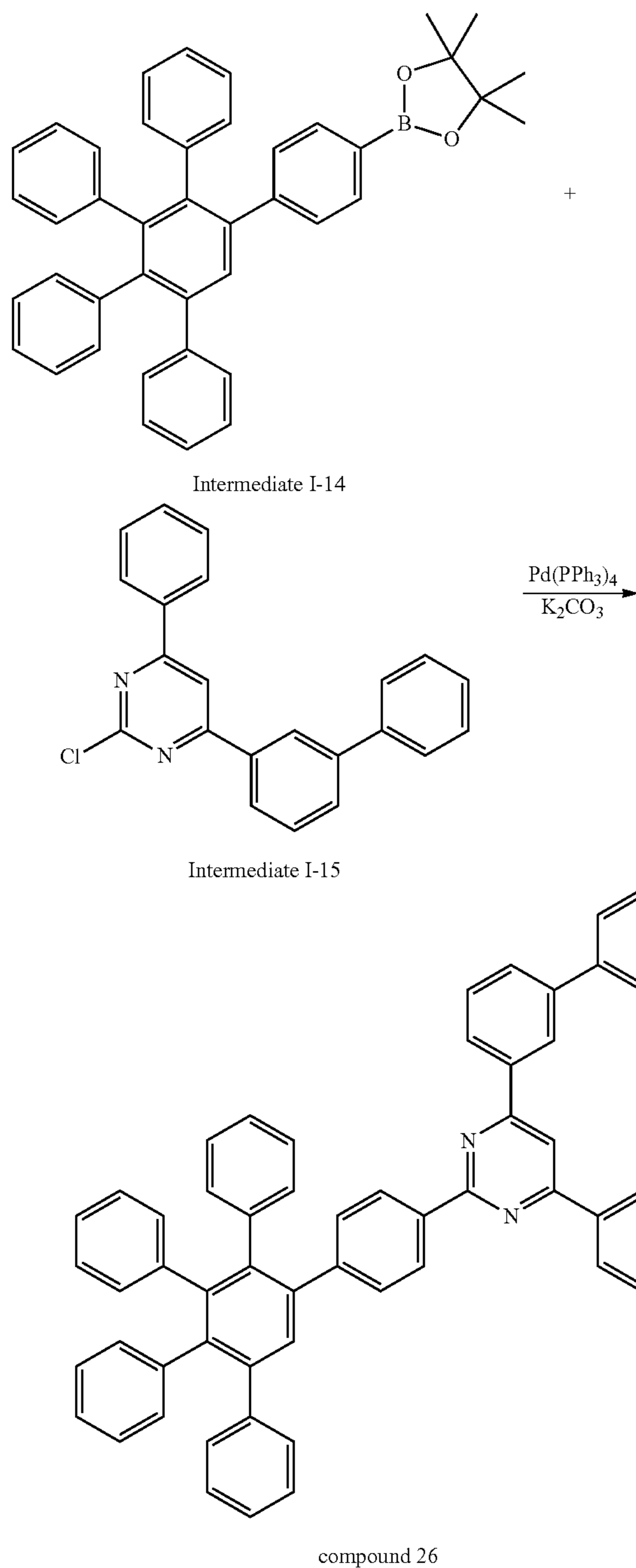
[Reaction Scheme 12]
