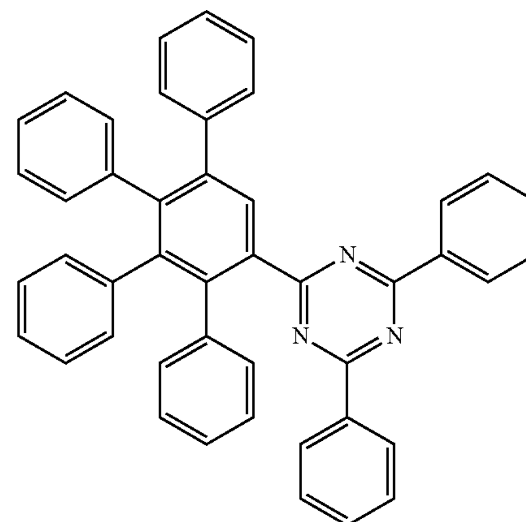
compound b
