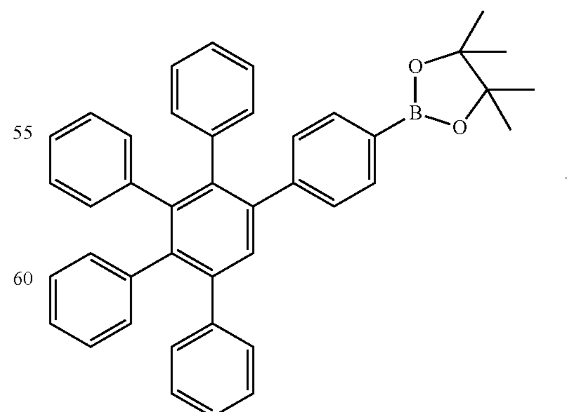
Intermediate I-14
