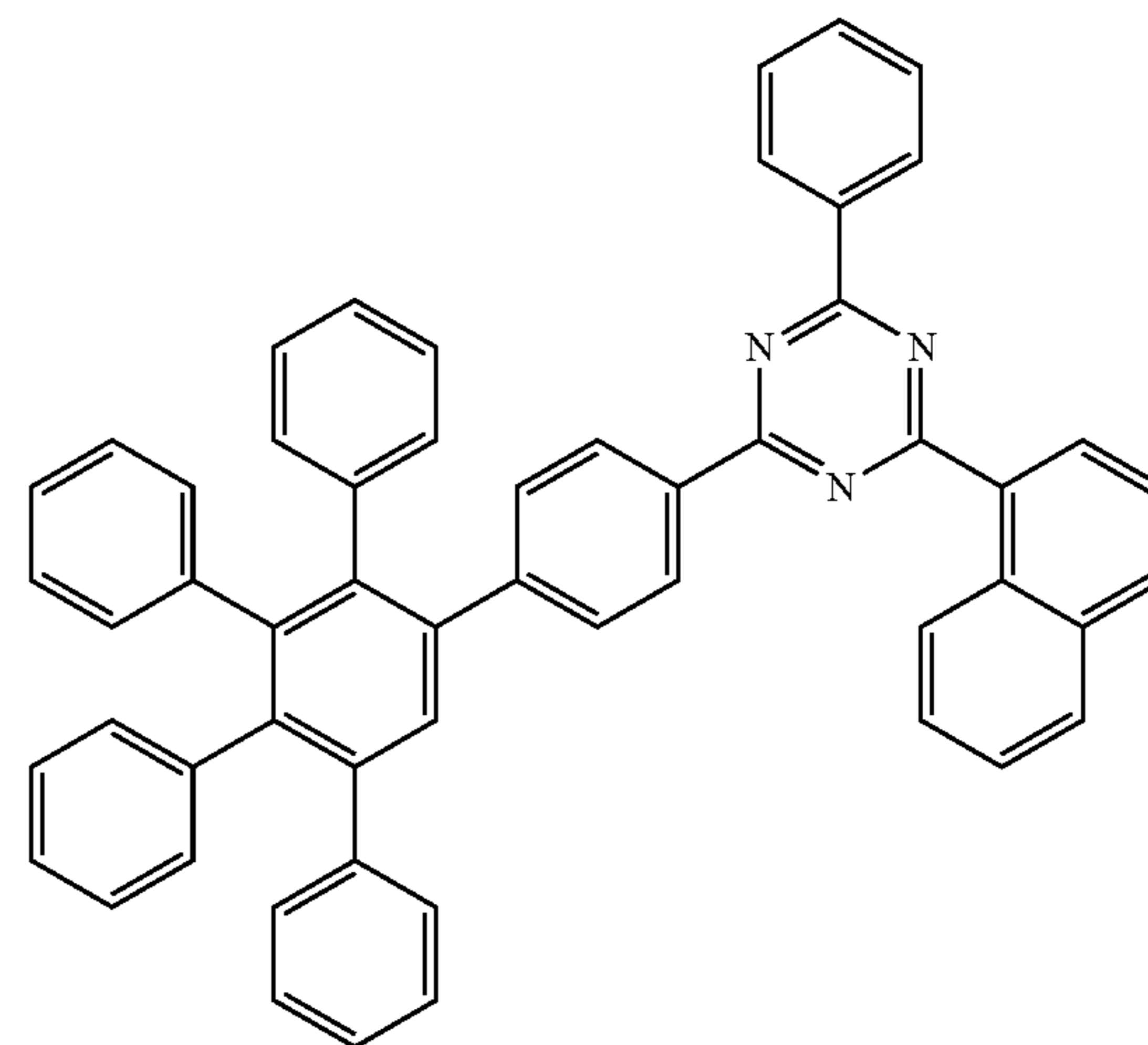
compound 125
