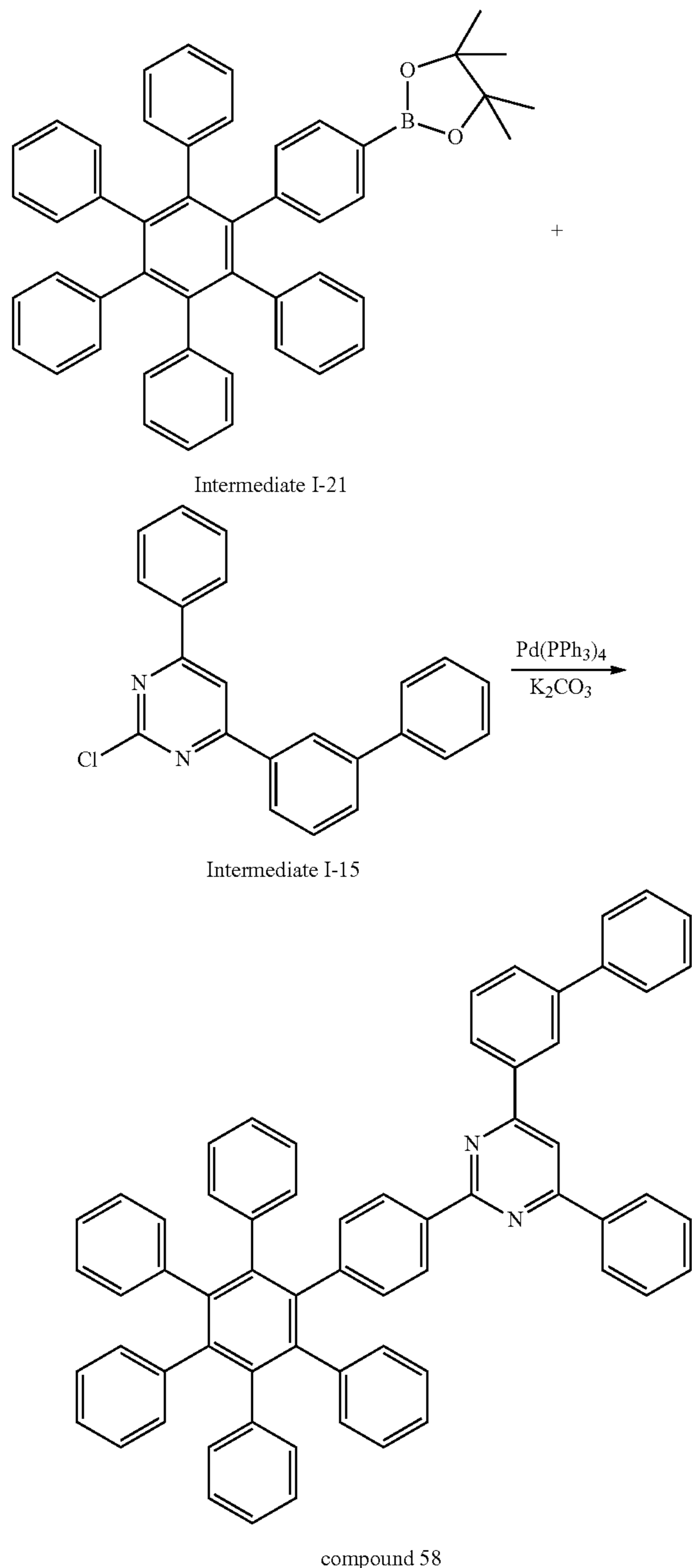
[Reaction Scheme 20]
