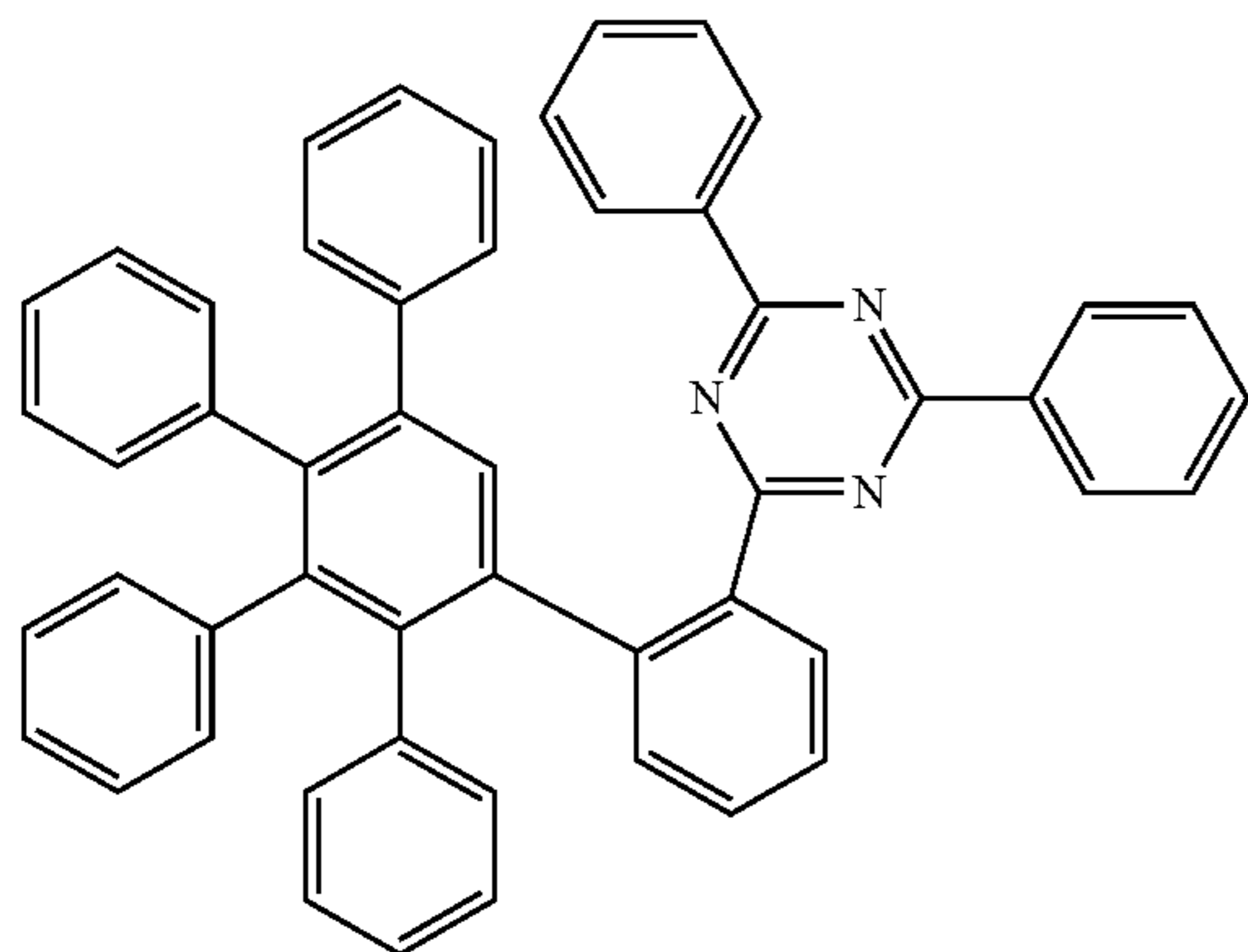
compound 65
