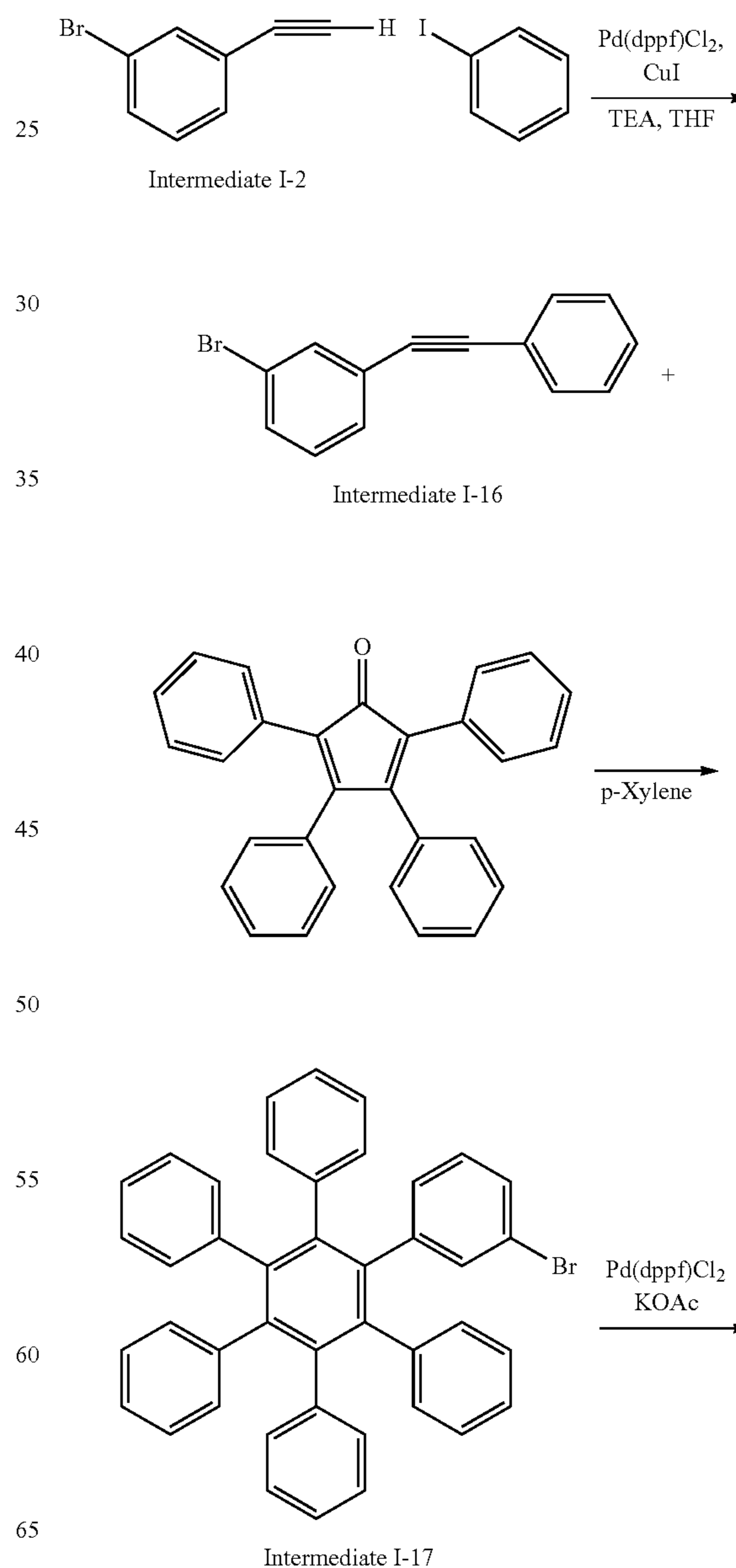
[Reaction Scheme 13]
