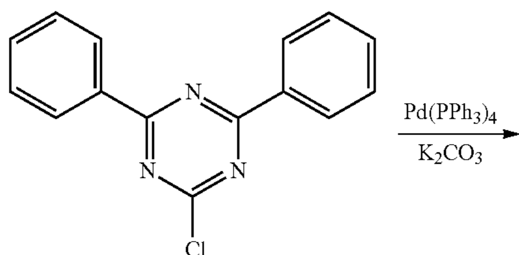
Intermediate I-5
