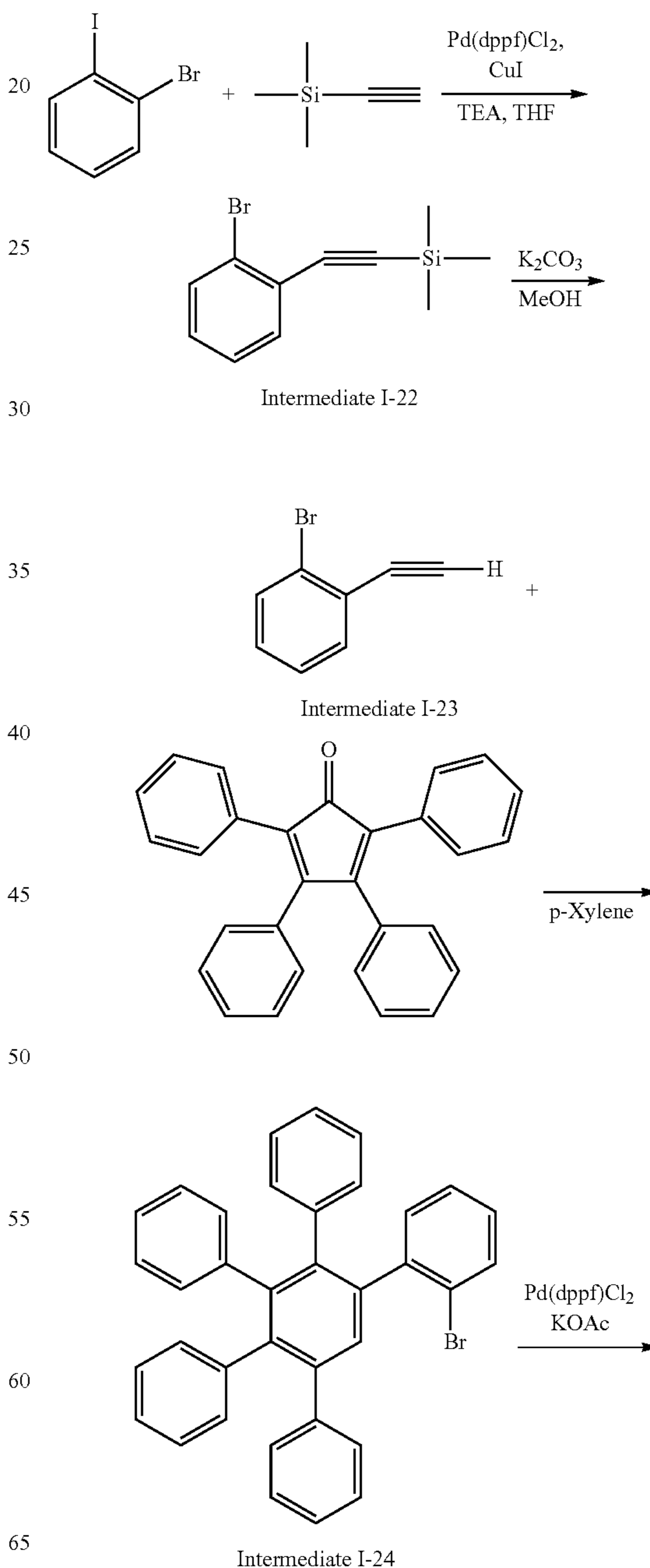
[Reaction Scheme 21]
