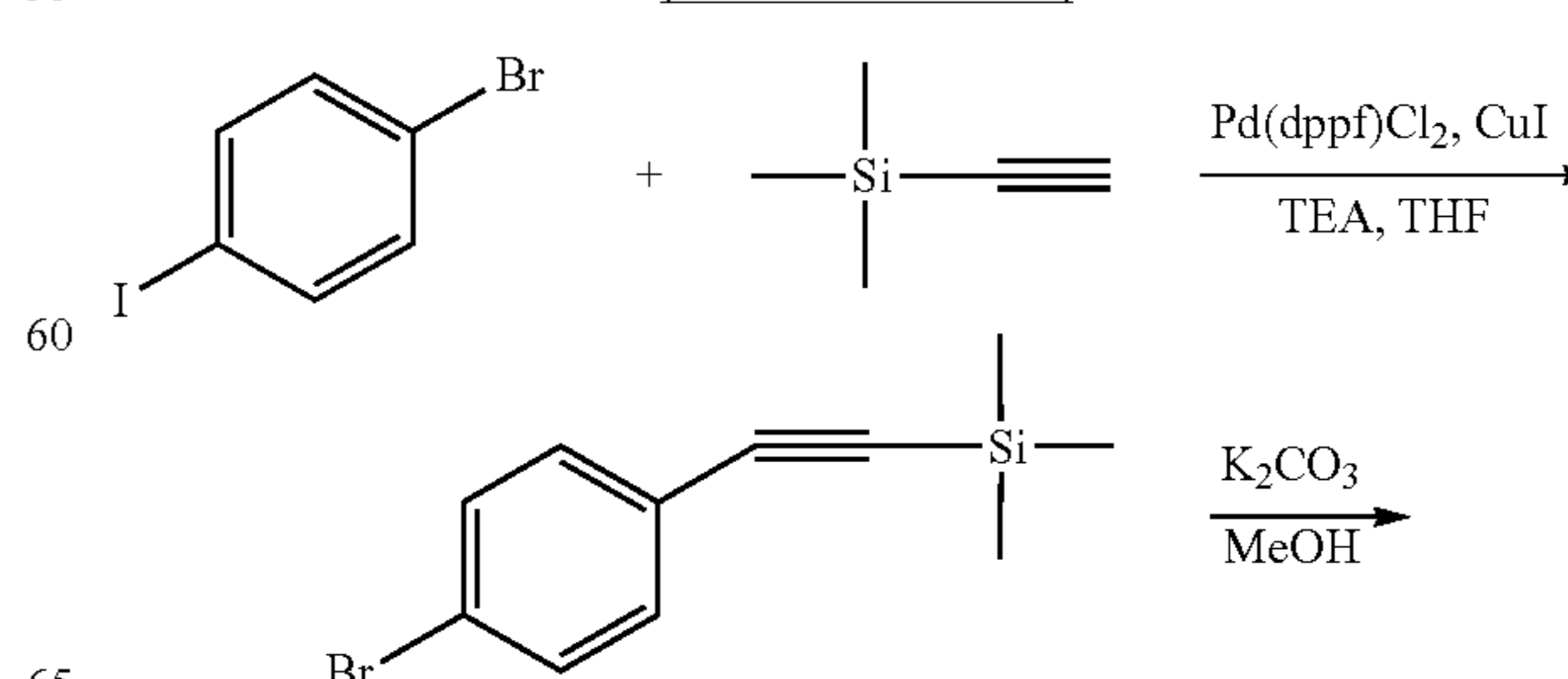
Intermediate I-11
