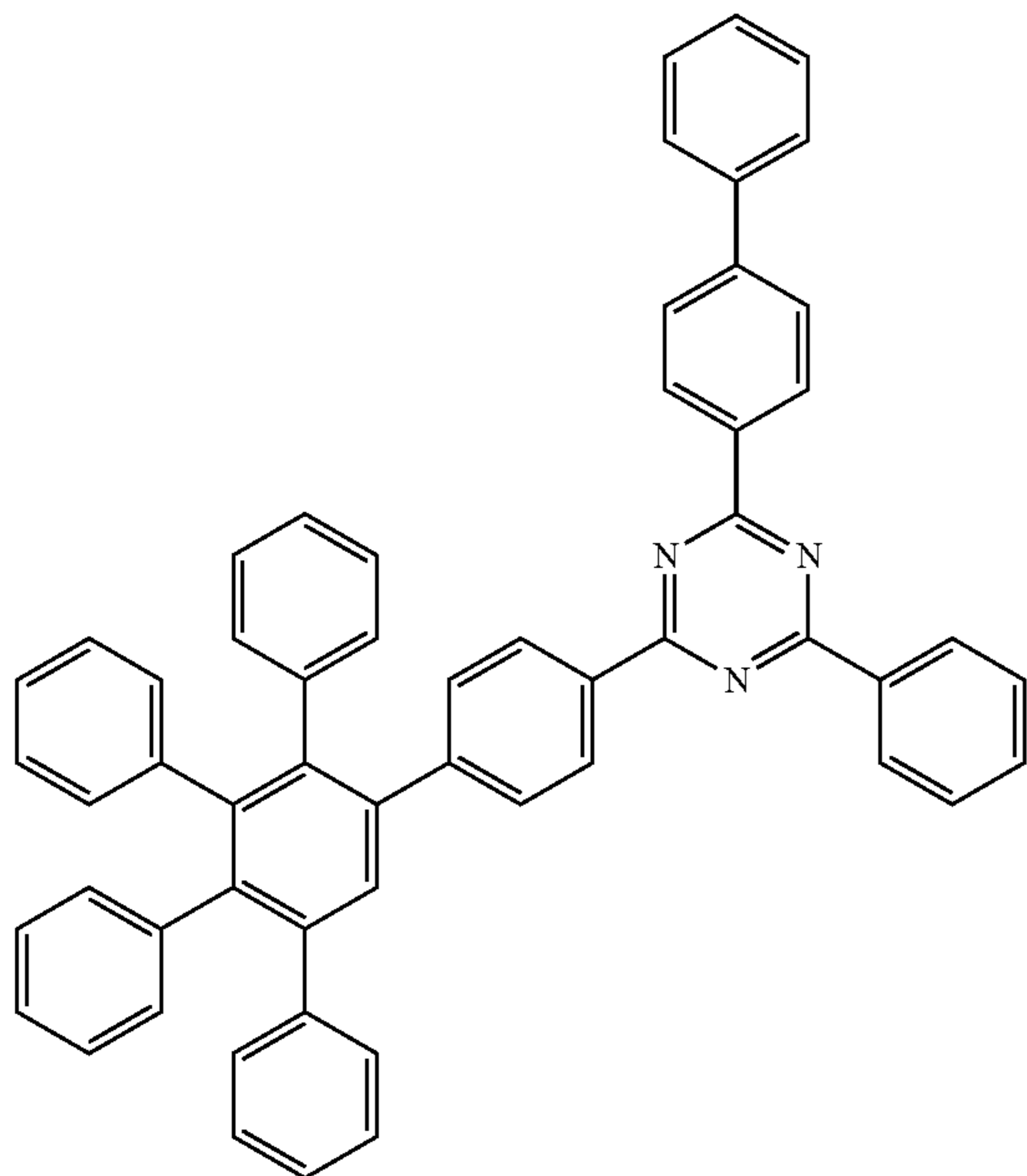
compound 11
