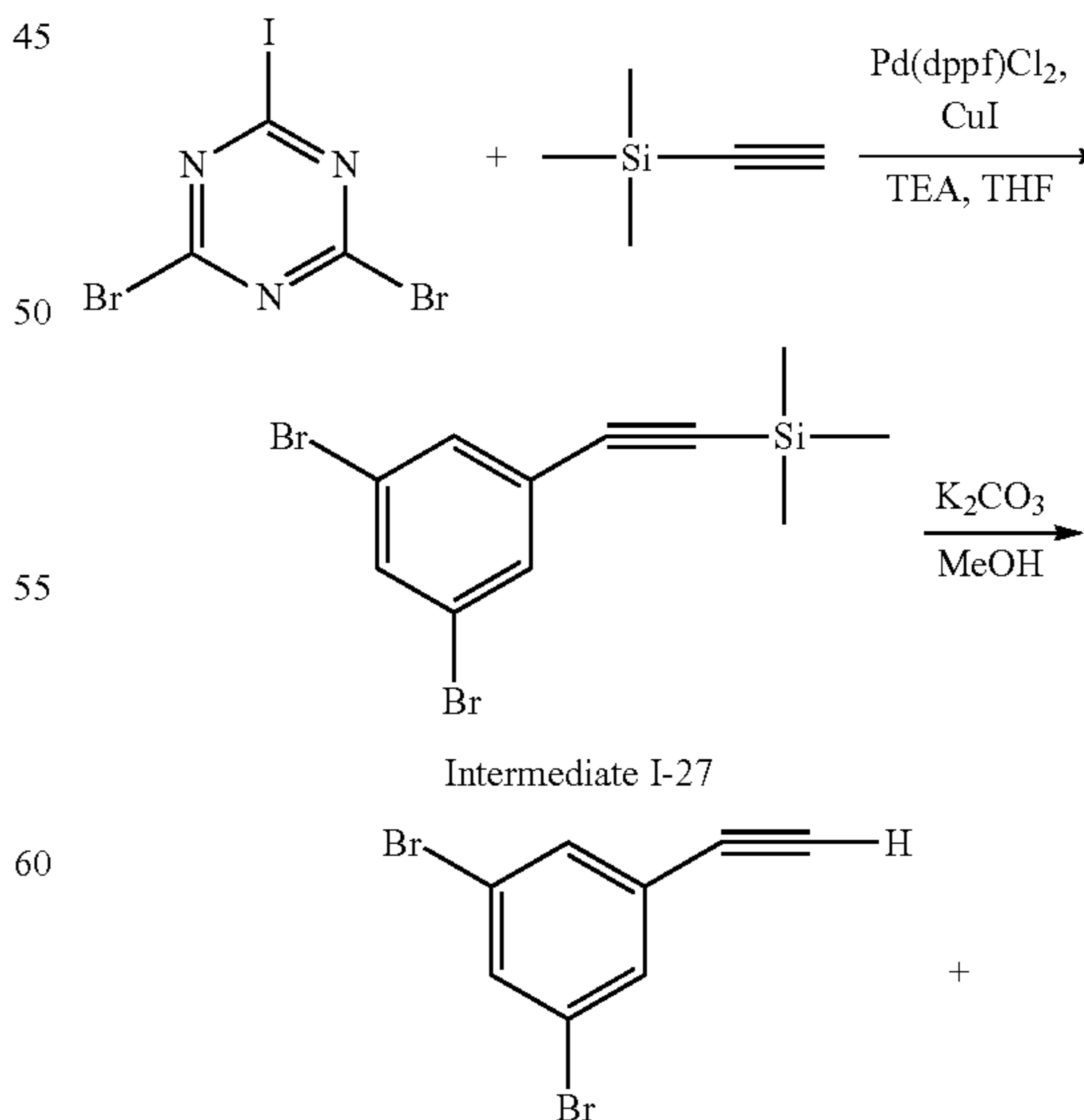
Intermediate I-28
