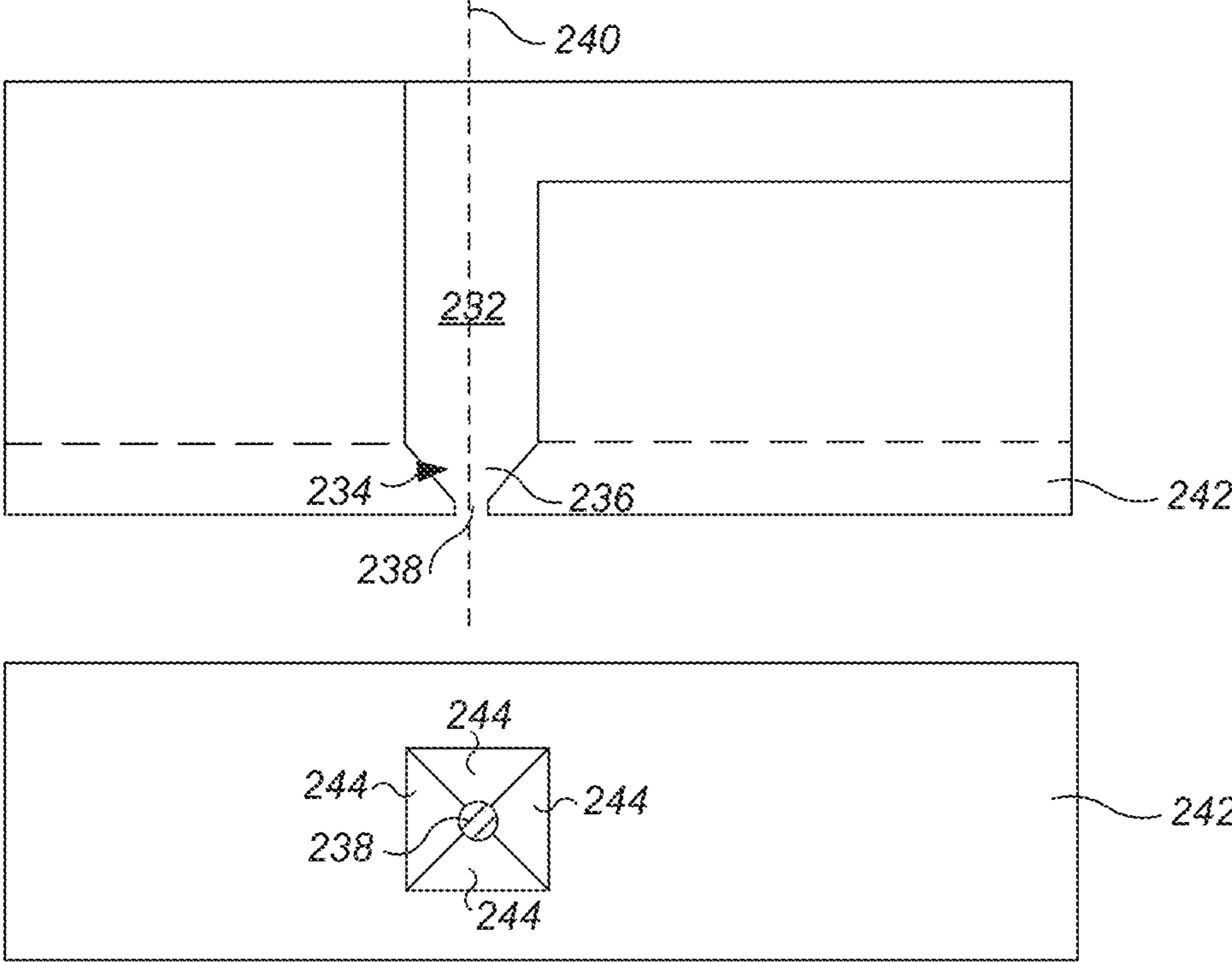
FIG. 2C Prior Art
