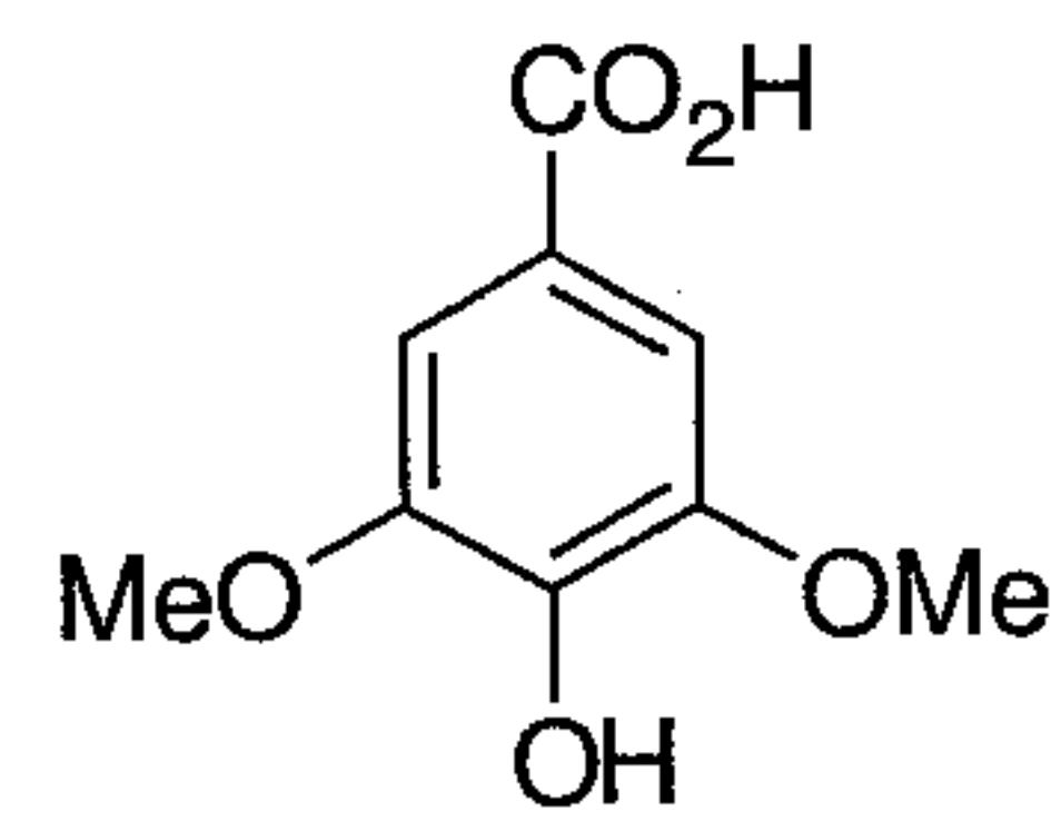
syringic acid
