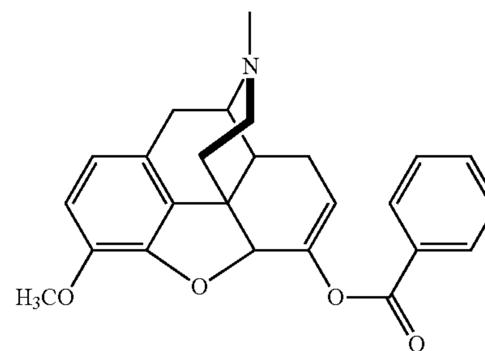
benzoate-hydrocodone (Bz-HC)
