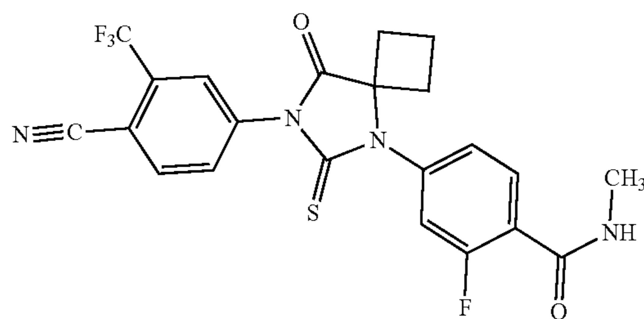
4-[7-(4-cyano-3-trifluoromethylphenyl)-8-oxo-6-thioxo-5,7-diazaspiro[3.4]oct-5-yl]-2-fluoro-N-methylbenzamide (RD162).
