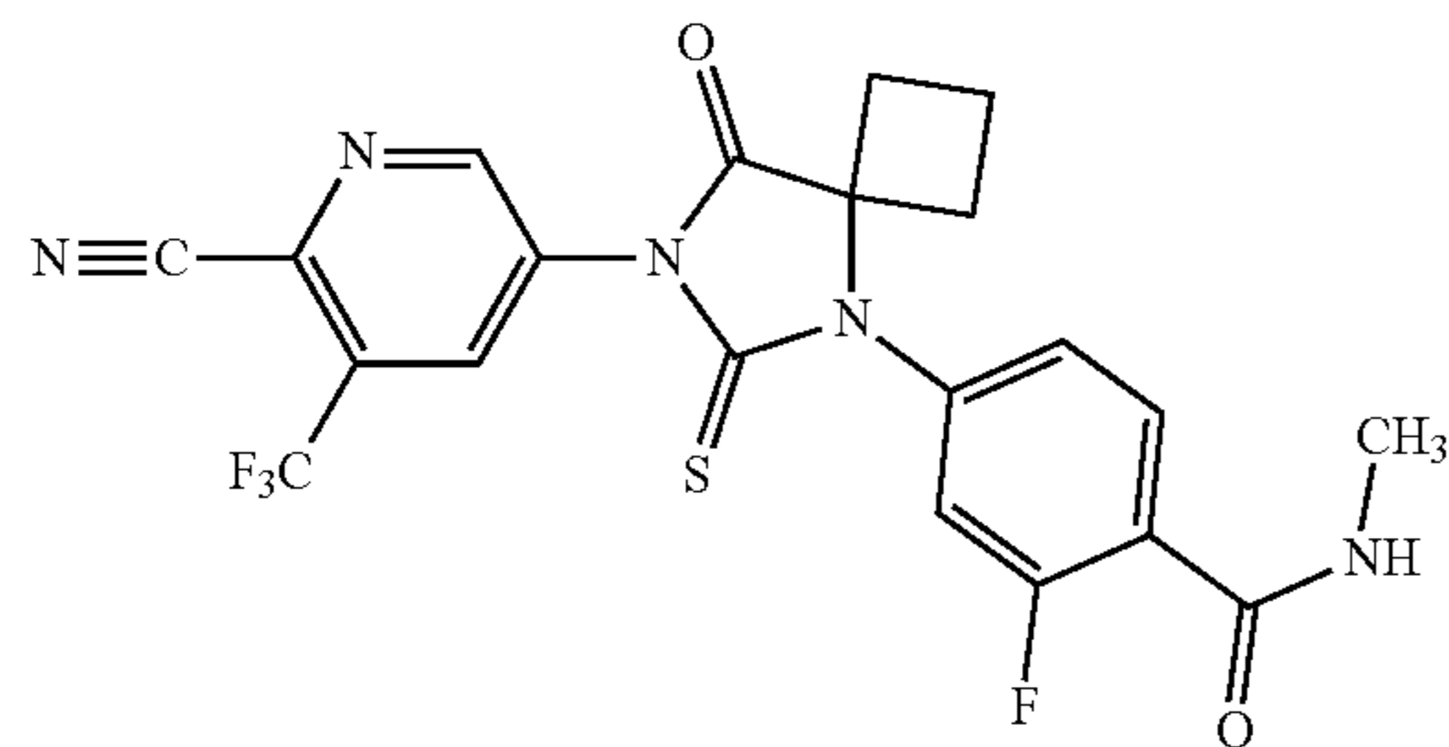
4-[7-(6-cyano-5-trifluoromethylpyridin-3-yl)-8-oxo-6-thioxo-5,7-diazaspiro[3.4]oct-5-yl]-2-fluoro-N-methylbenzamide (ARN-509)
