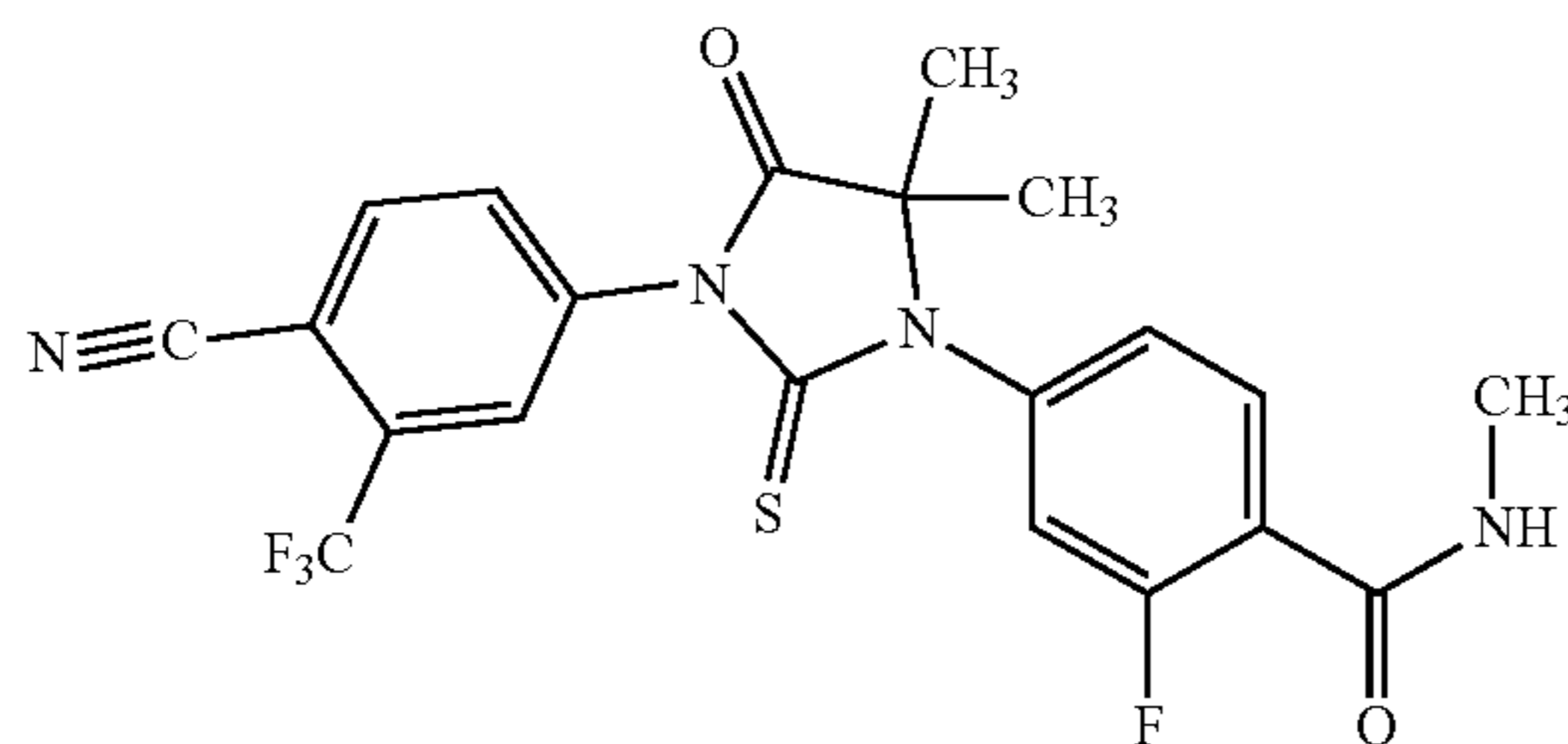
4-(3-(4-cyano-3-(trifluoromethyl)phenyl)-5,5-dimethyl-4-oxo-2-thioxoimidazolidin-1-yl)-2-fluoro-N-methylbenzamide (enzalutamide)
