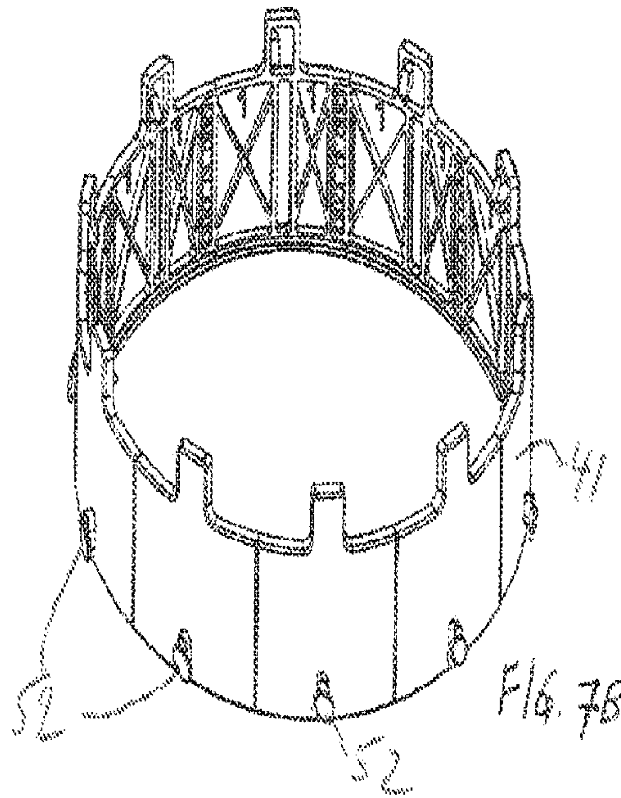
Perspective View FIG. 7B
