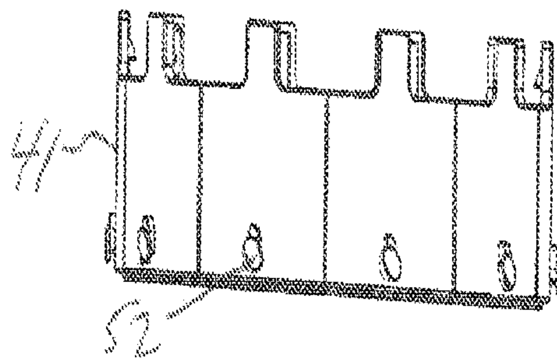
Side View FIG. 7D
