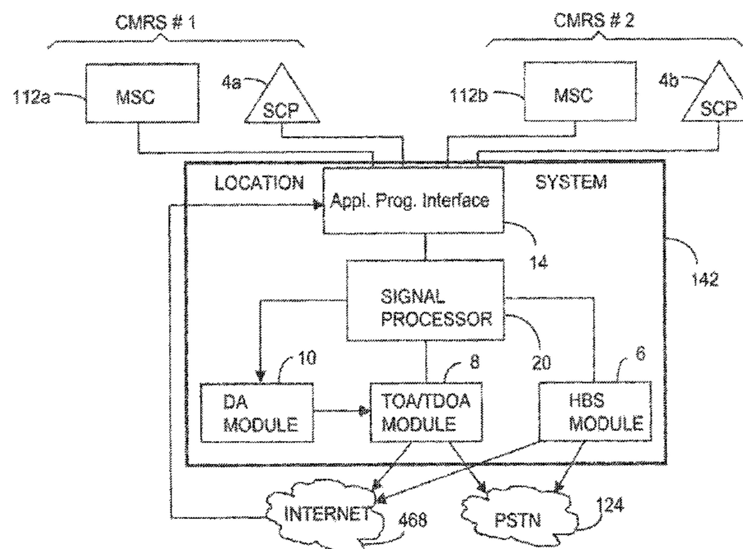
WIRELESS LOCATION USING MULTIPLE CMRSs
