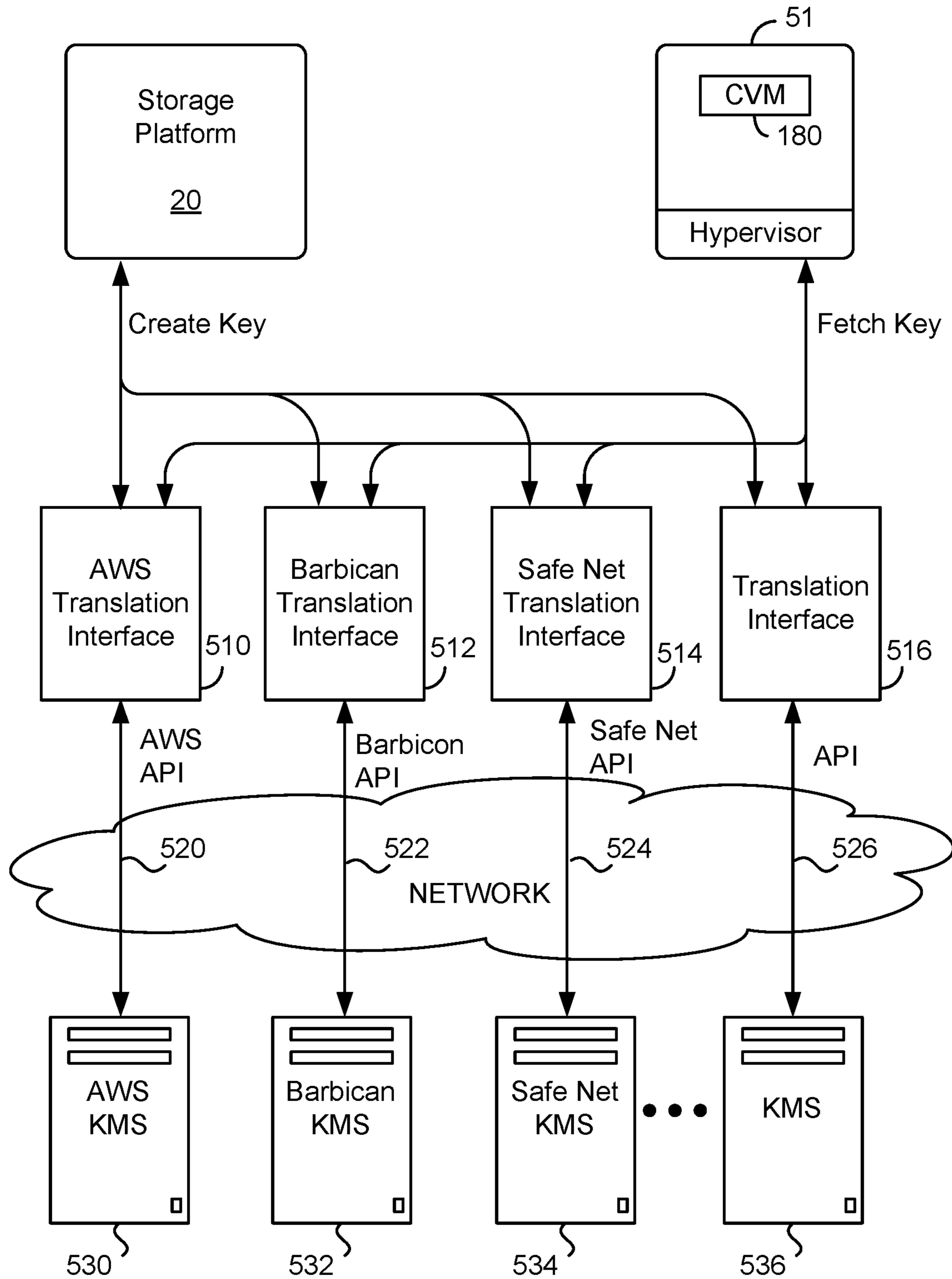
KMS Architecture
