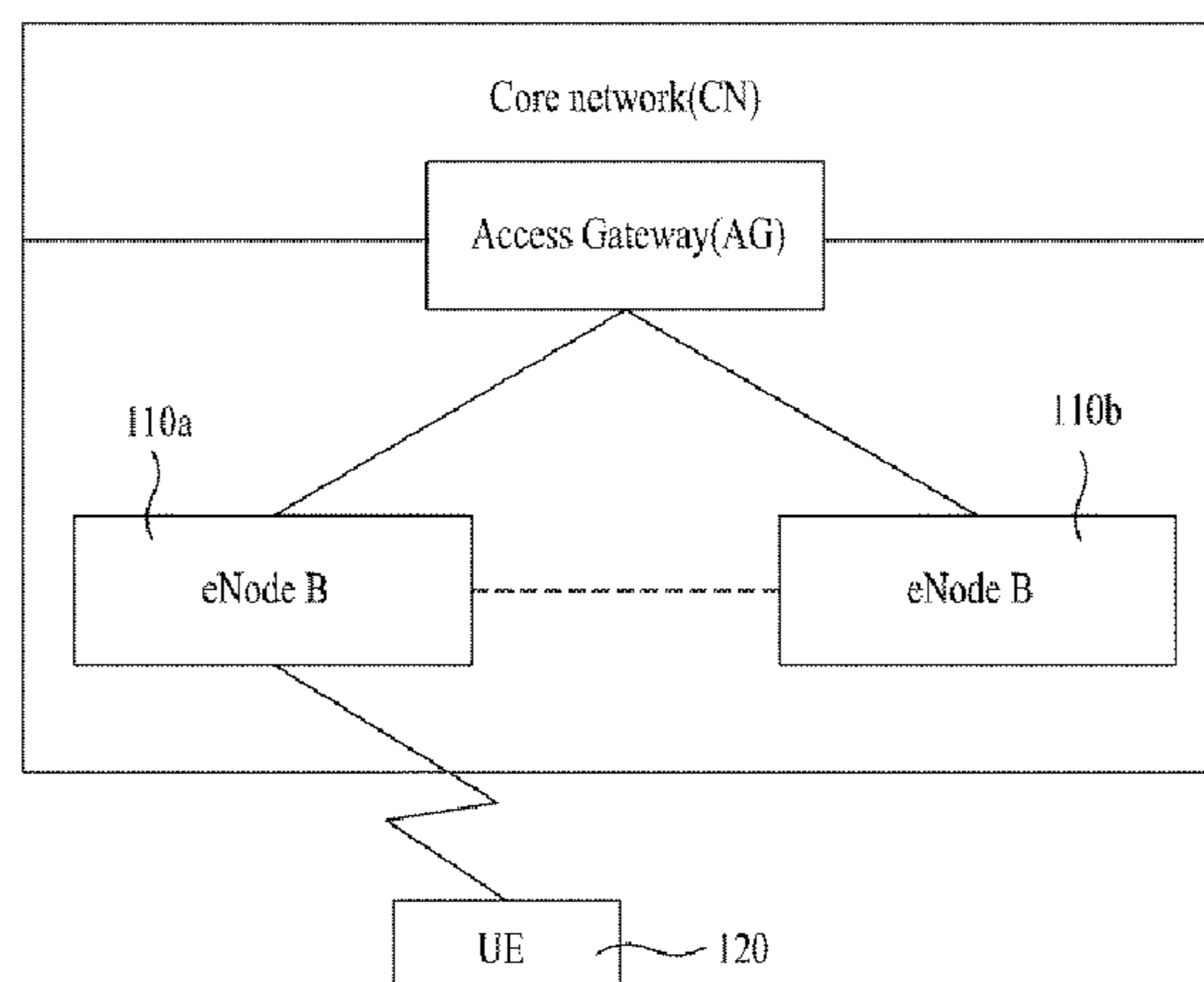
E-UMTS
