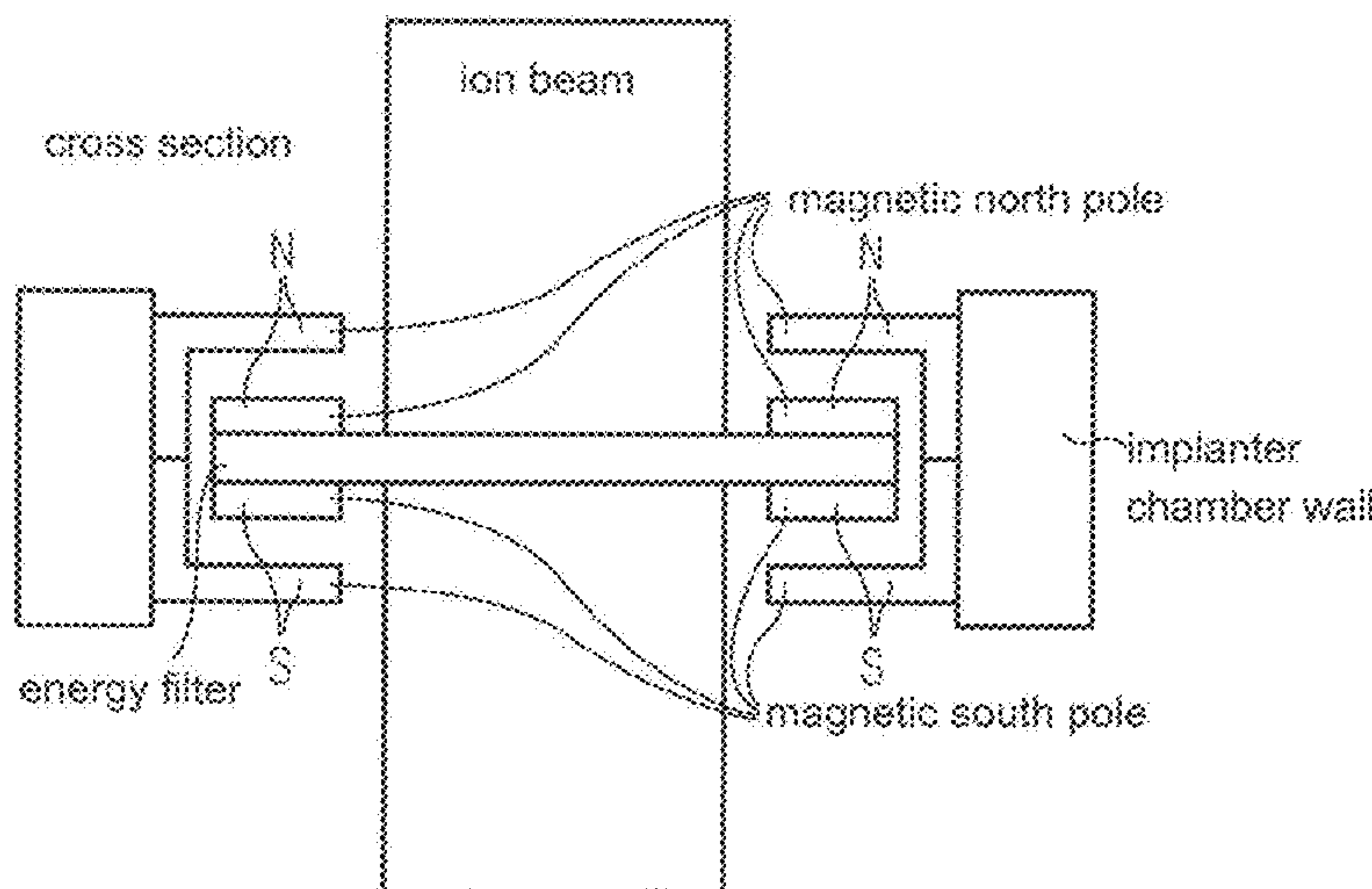
attachment of the filter by magnets
