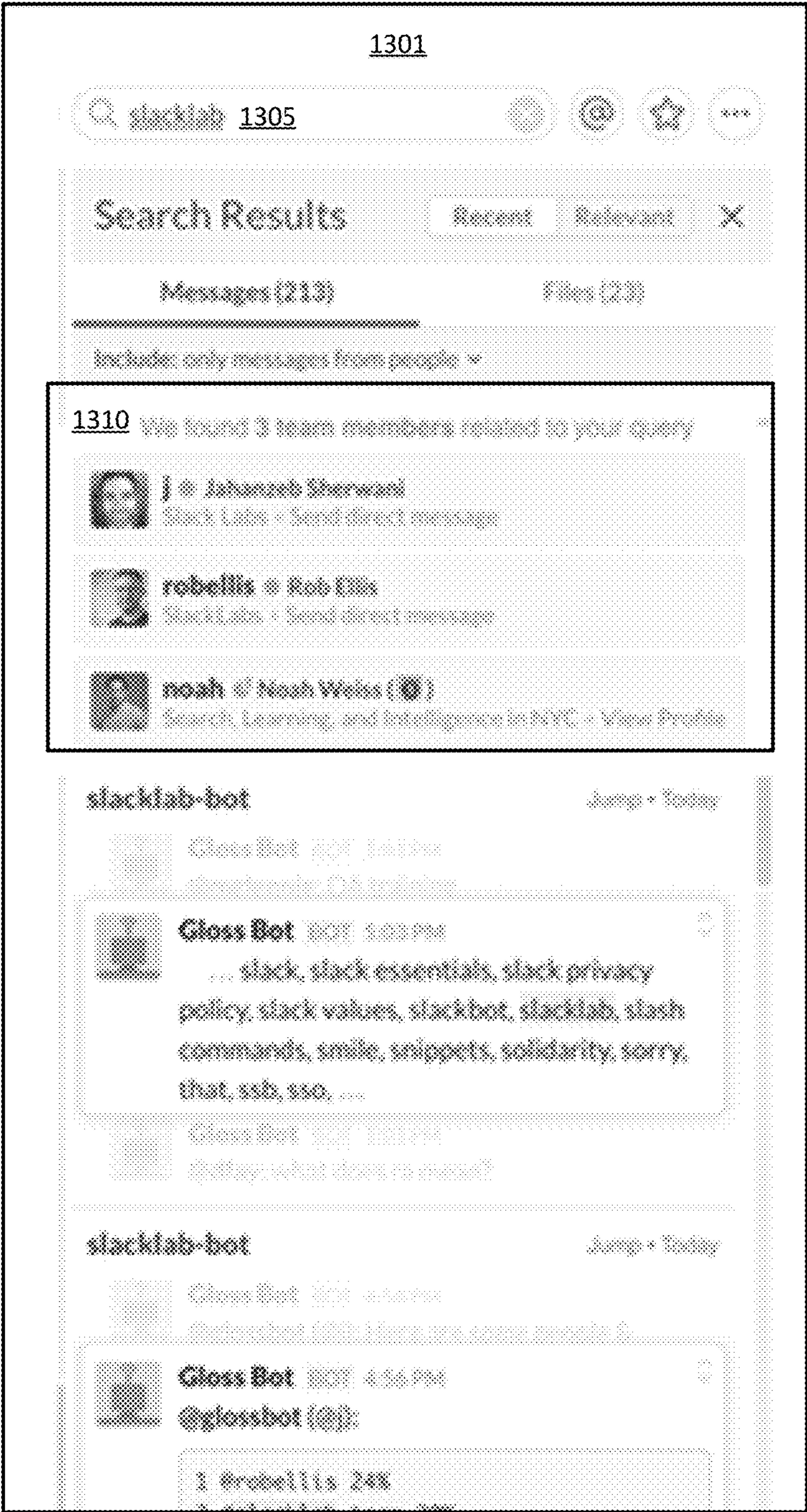
EXEMPLARY MSM SCREENSHOT
