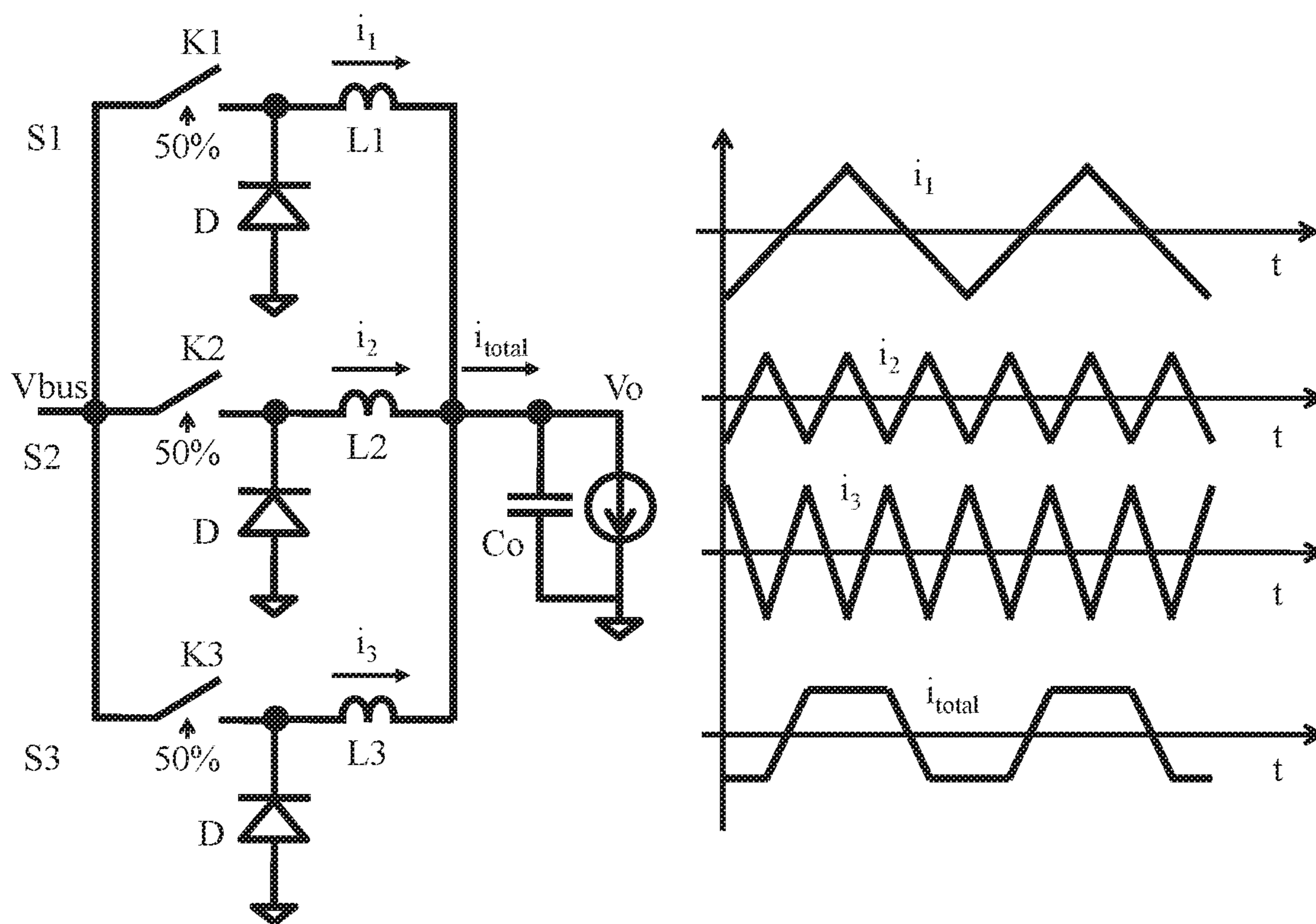
(b) Waveform diagram
