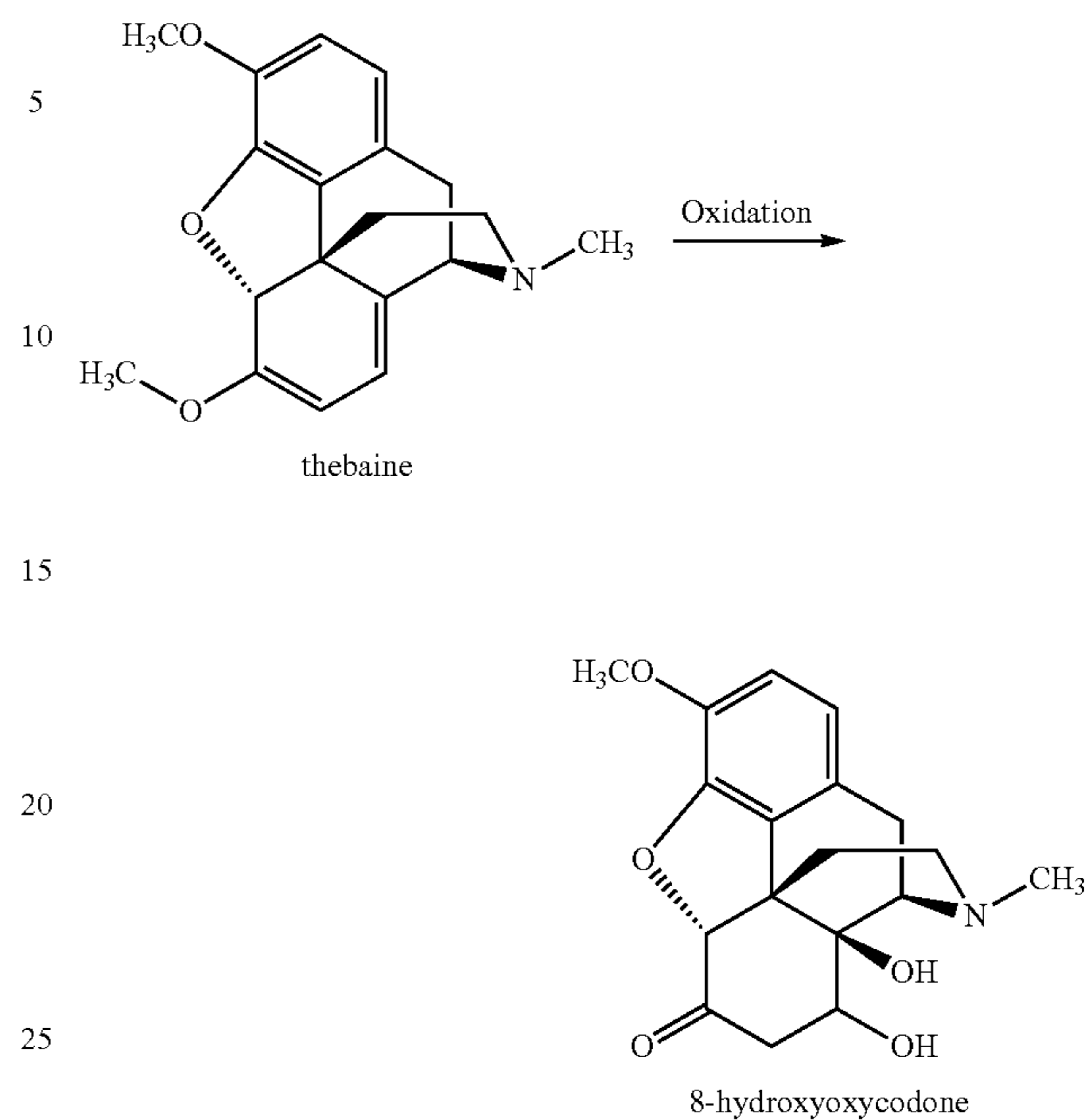
Scheme 3
