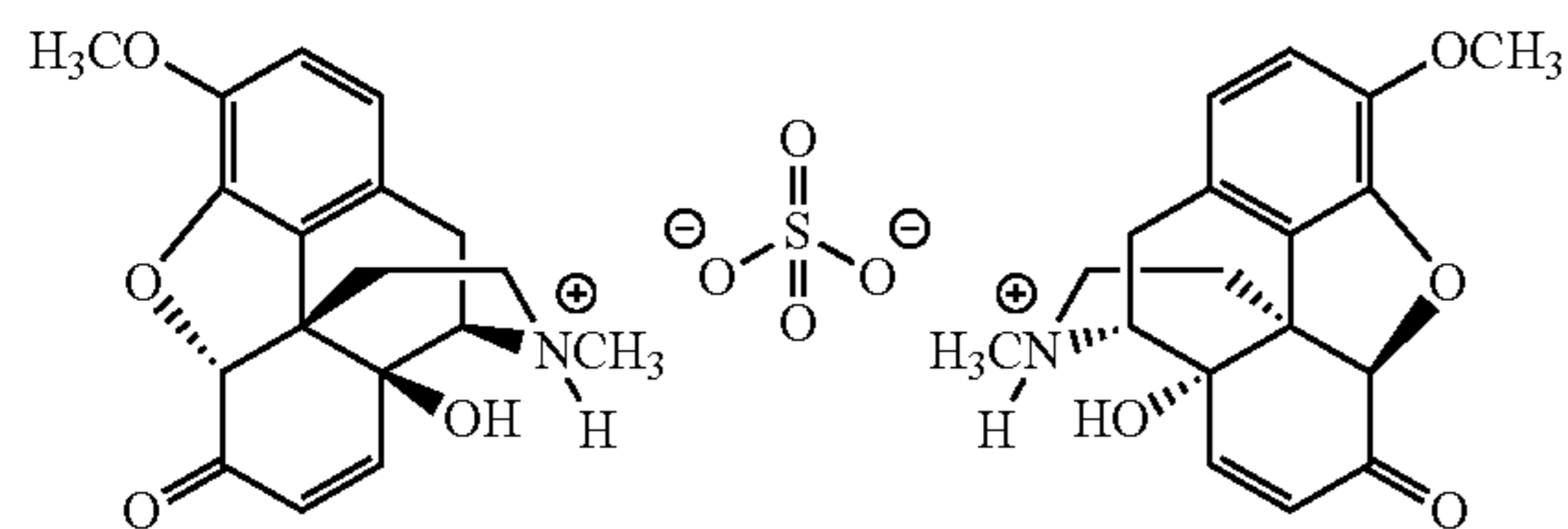
14-Hydroxycodeinone Sulfate
