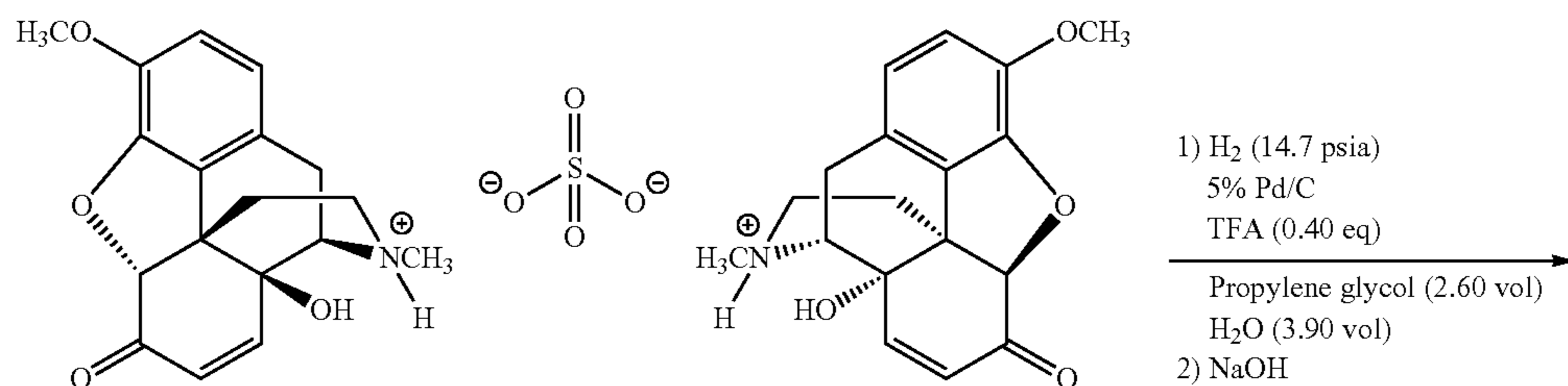
14-Hydroxycodeinone Sulfate
