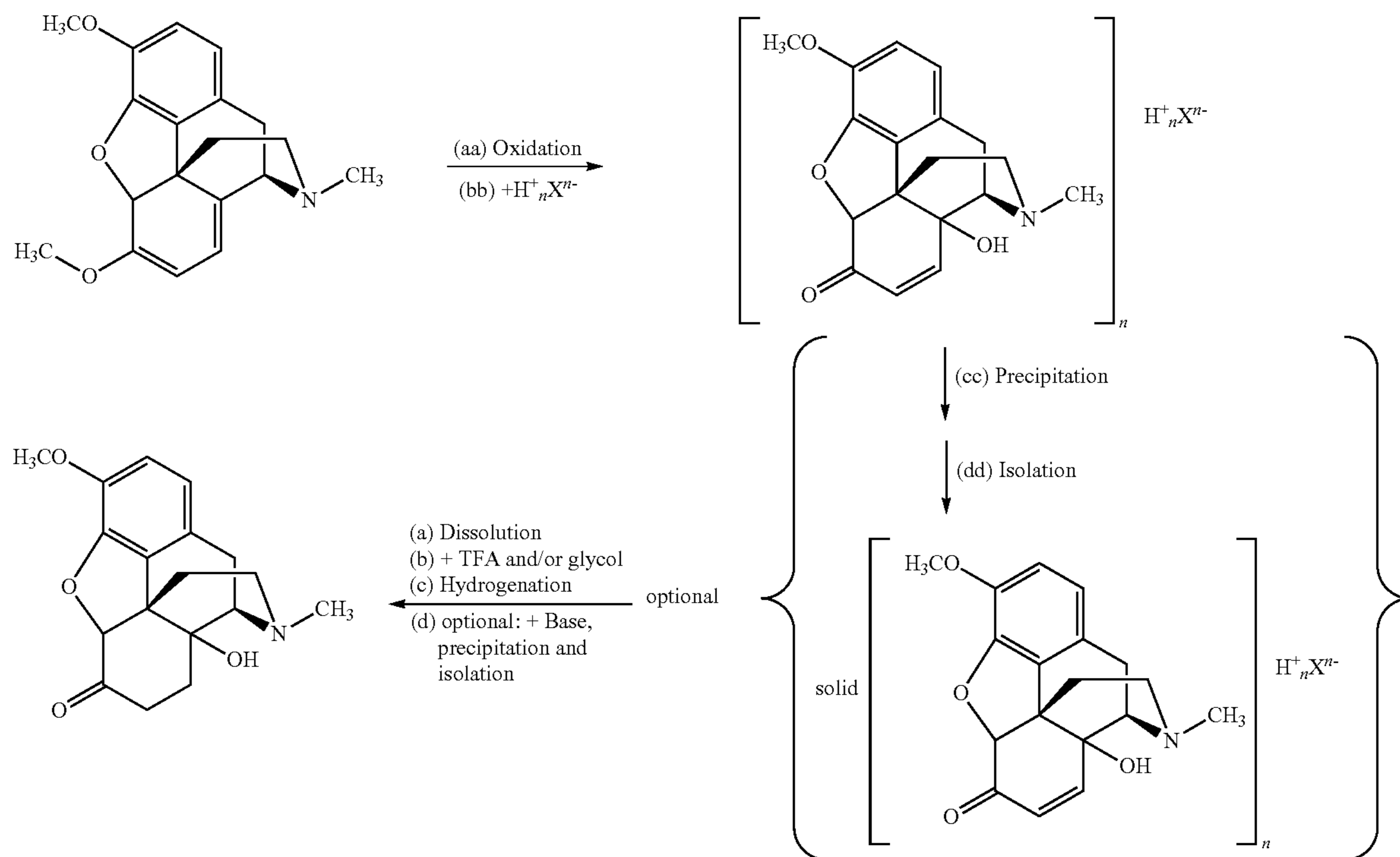
Scheme 12
