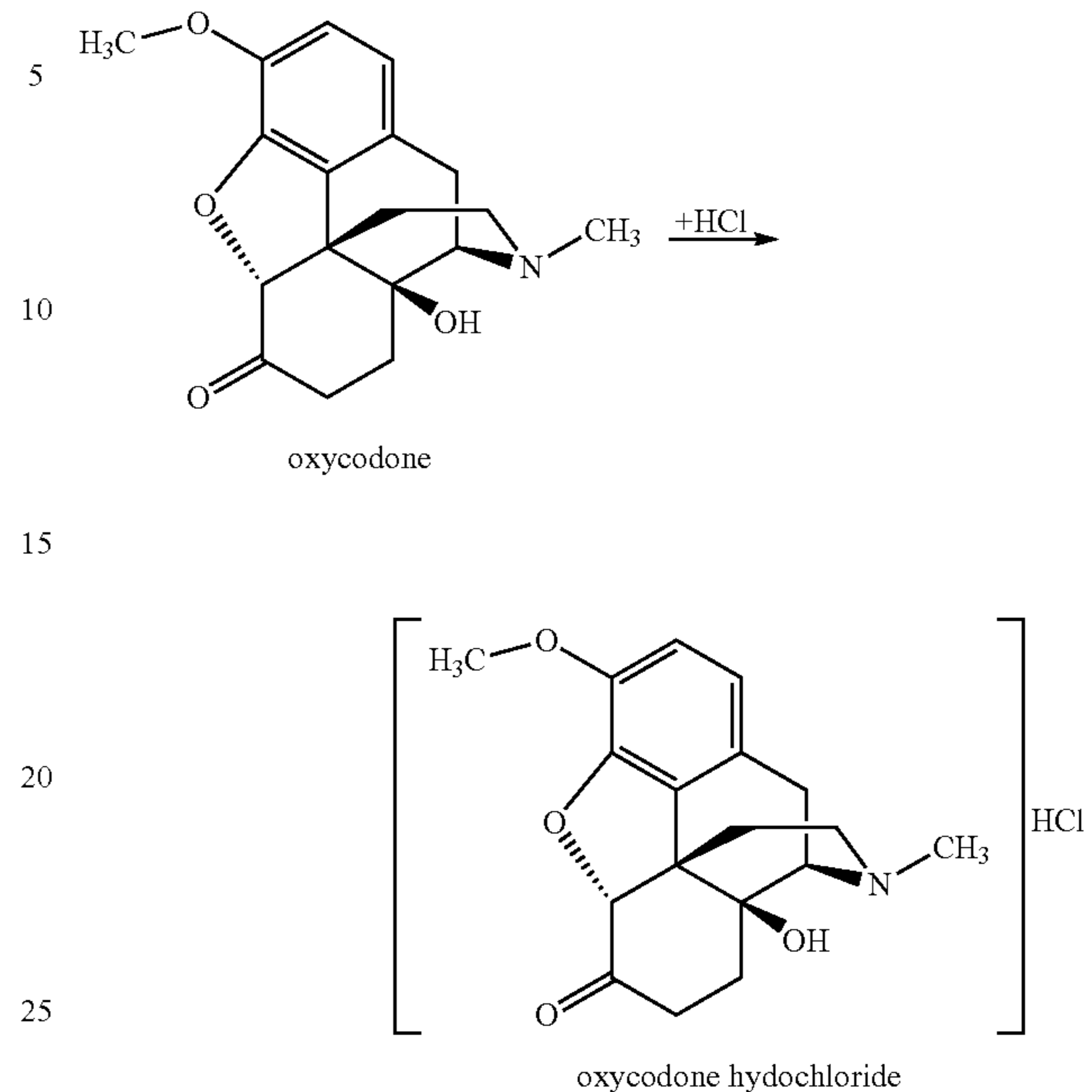
Scheme 2
