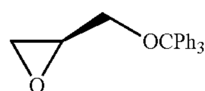
(S)-2-((trityloxy)methyl)oxirane (401)
