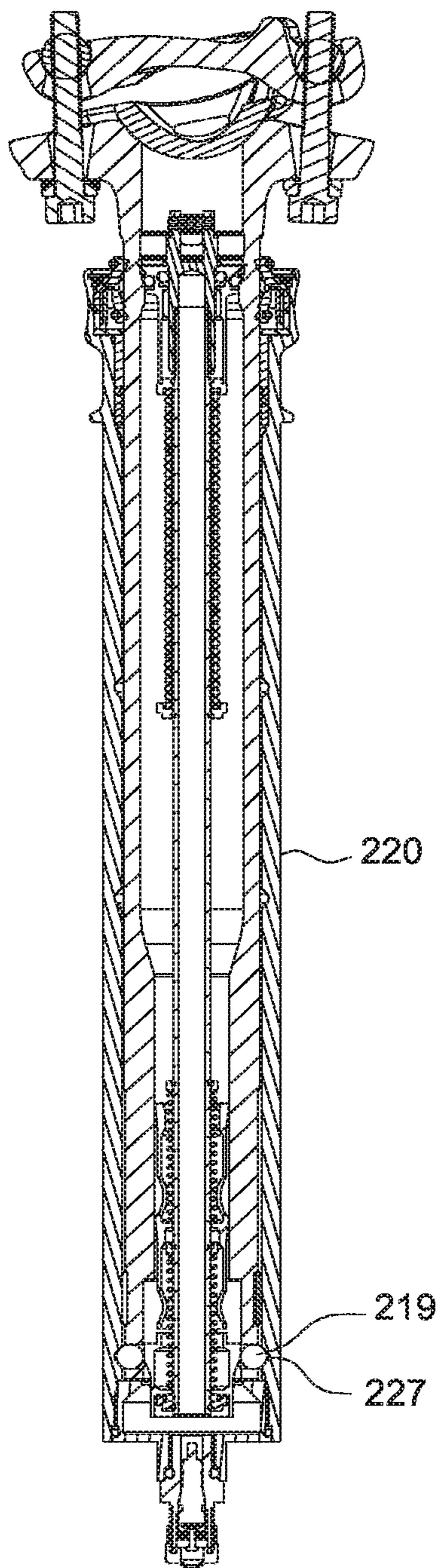
SECTION B-B
