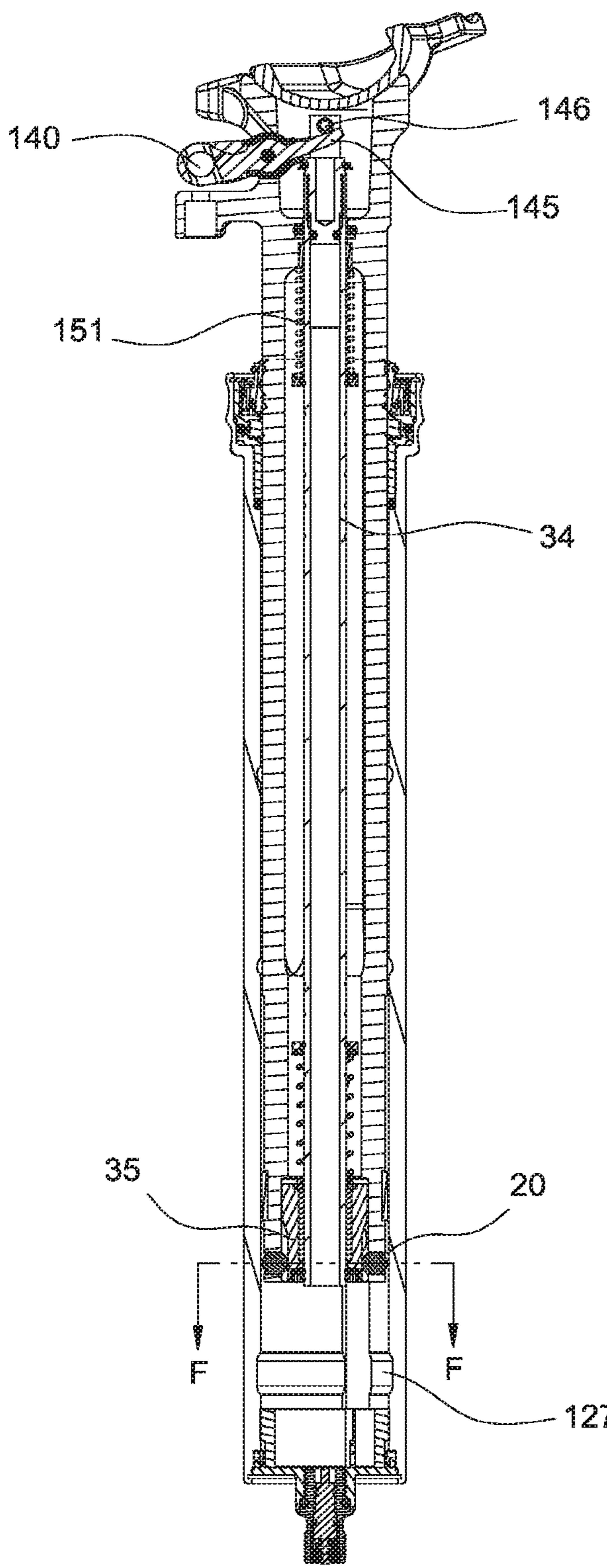
SECTION C-C
