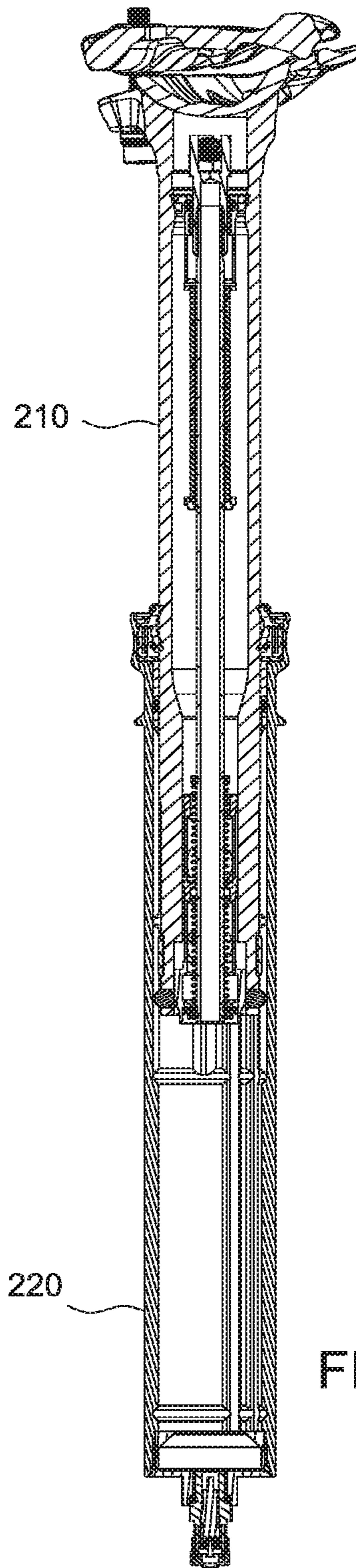
SECTION F-F
