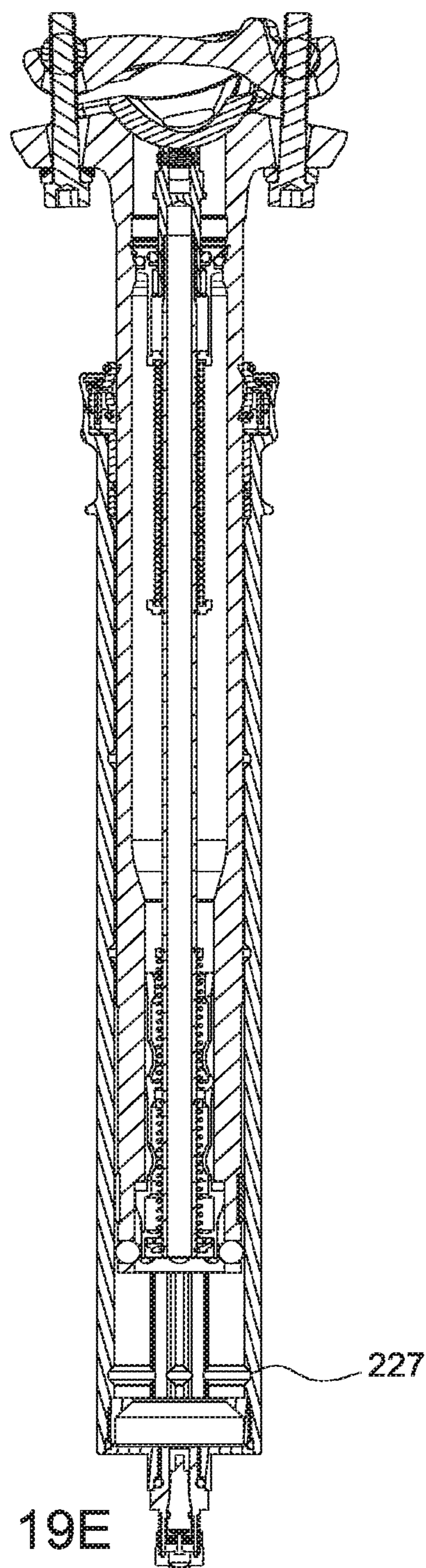
SECTION B-B
