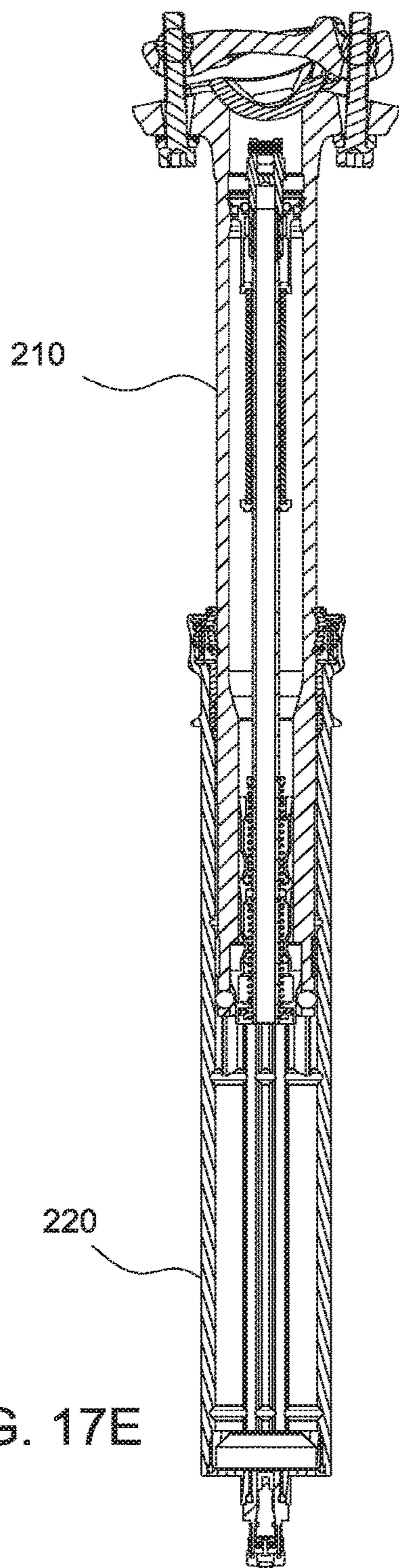
SECTION B-B
