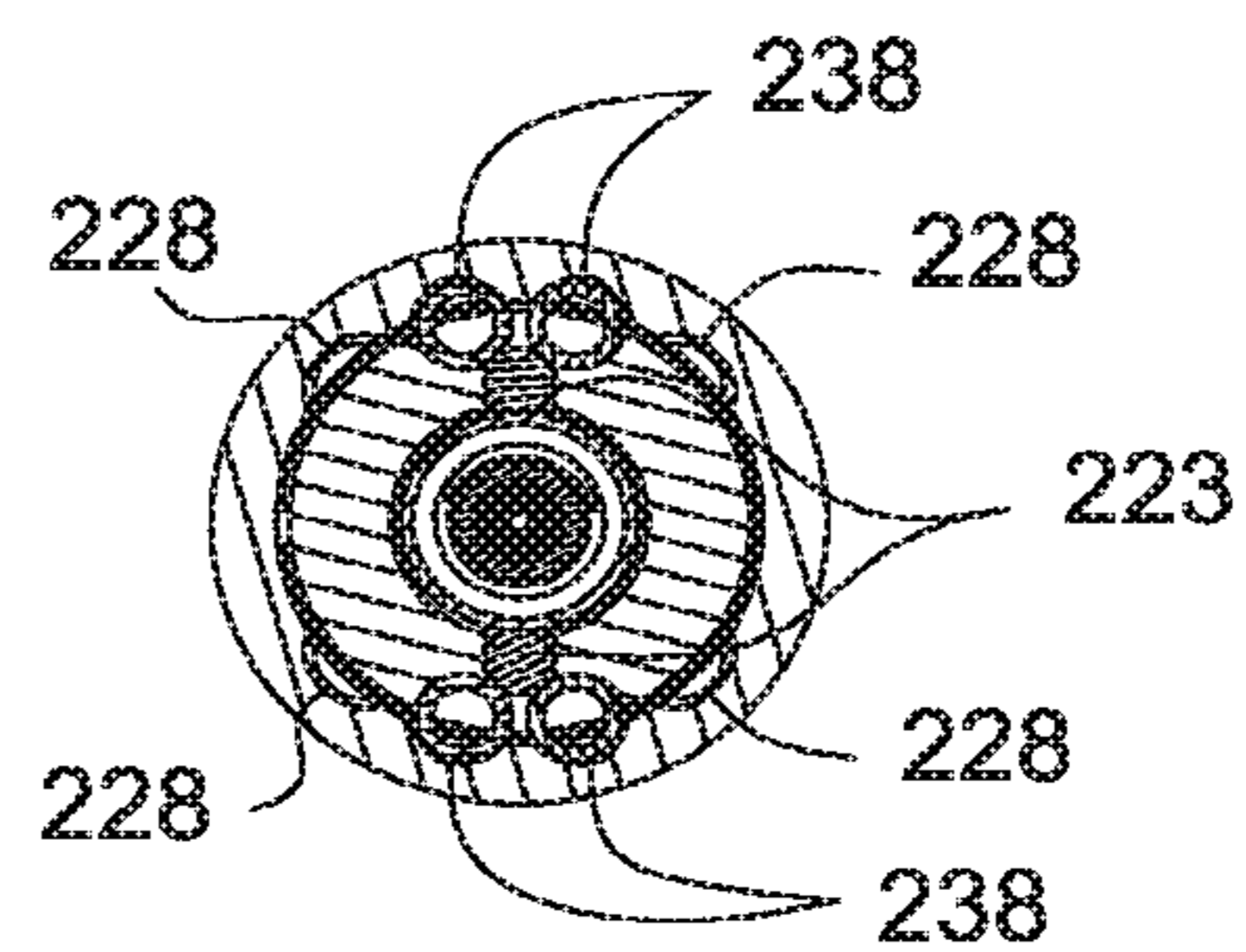
SECTION G-G
