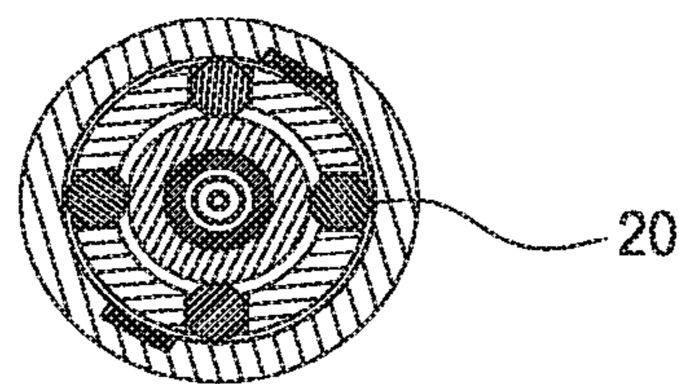
SECTION F-F
