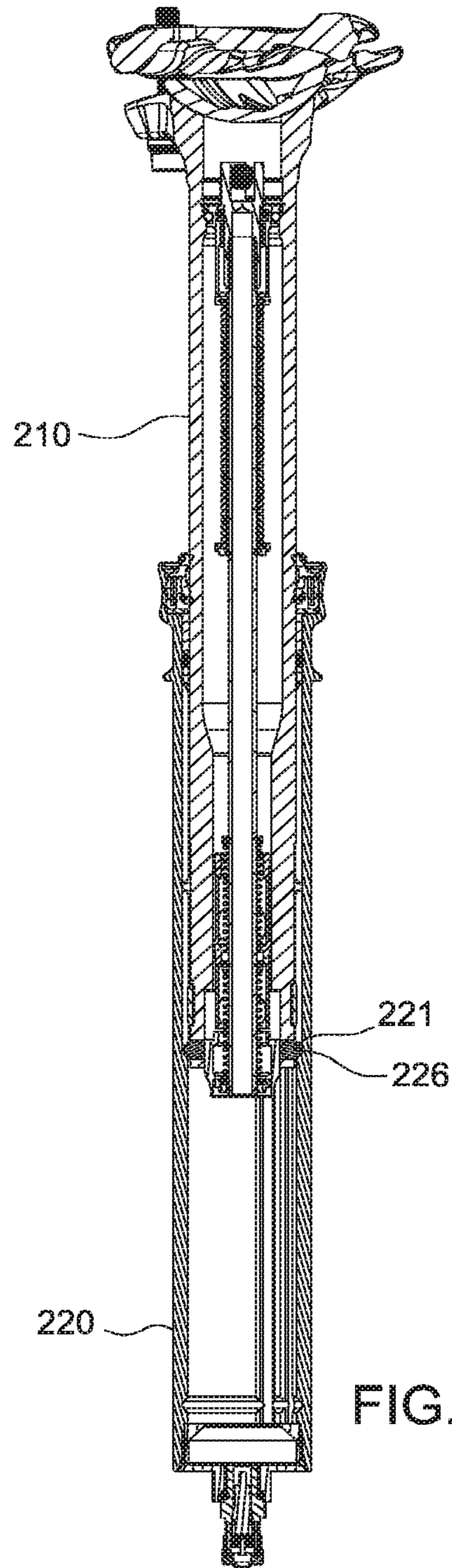
SECTION F-F
