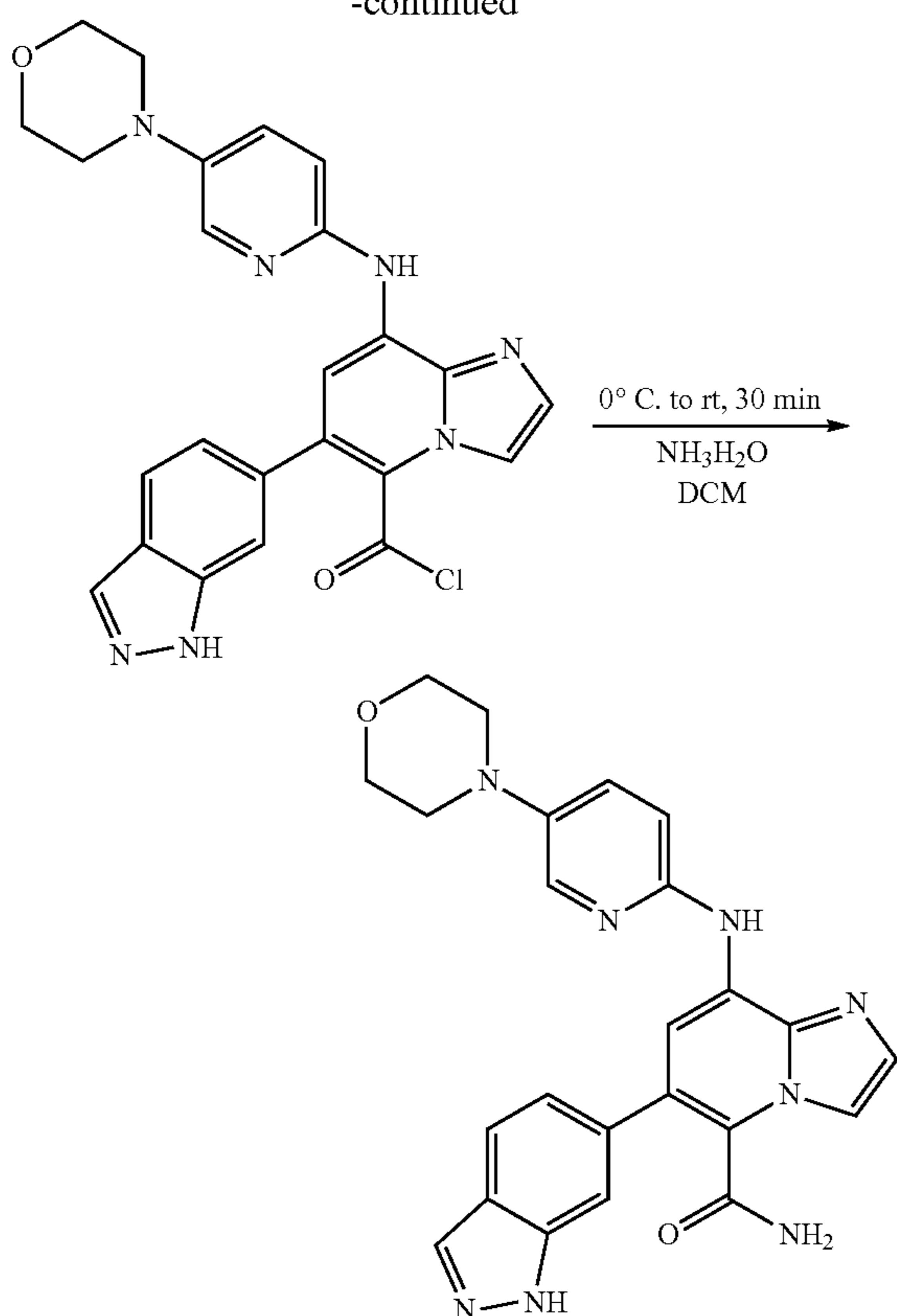
6-(1H-indazol-6-yl)-8-(5-morpholinopyridin-2-ylamino)imidazo[1,2-a]pyridine-5-carboxamide
