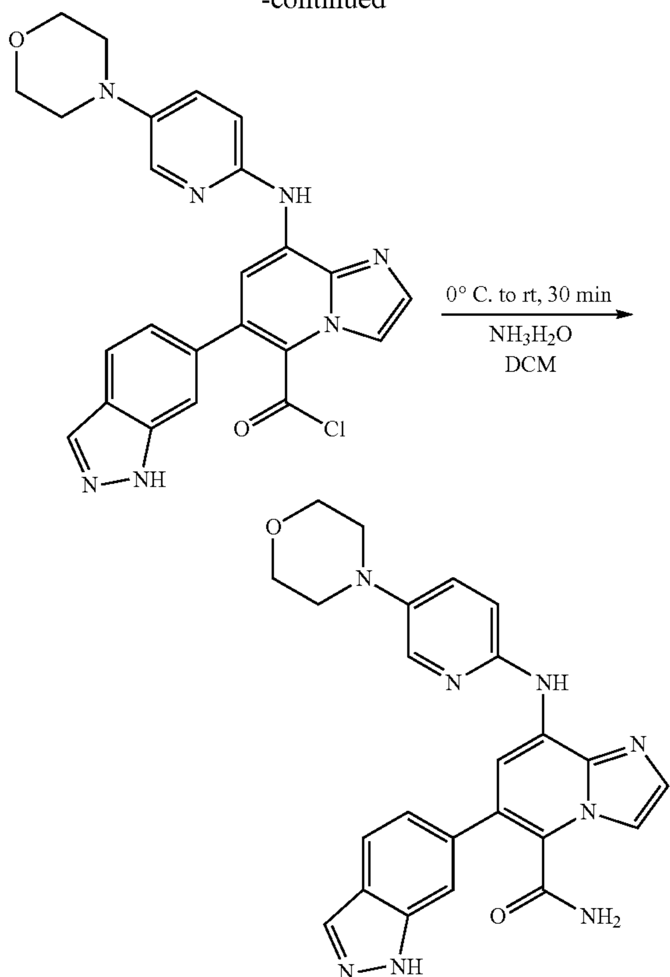
6-(1H-indazol-6-yl)-8-(5-morpholinopyridin-2-ylamino)imidazo[1,2-a]pyridine-5-carboxamide
