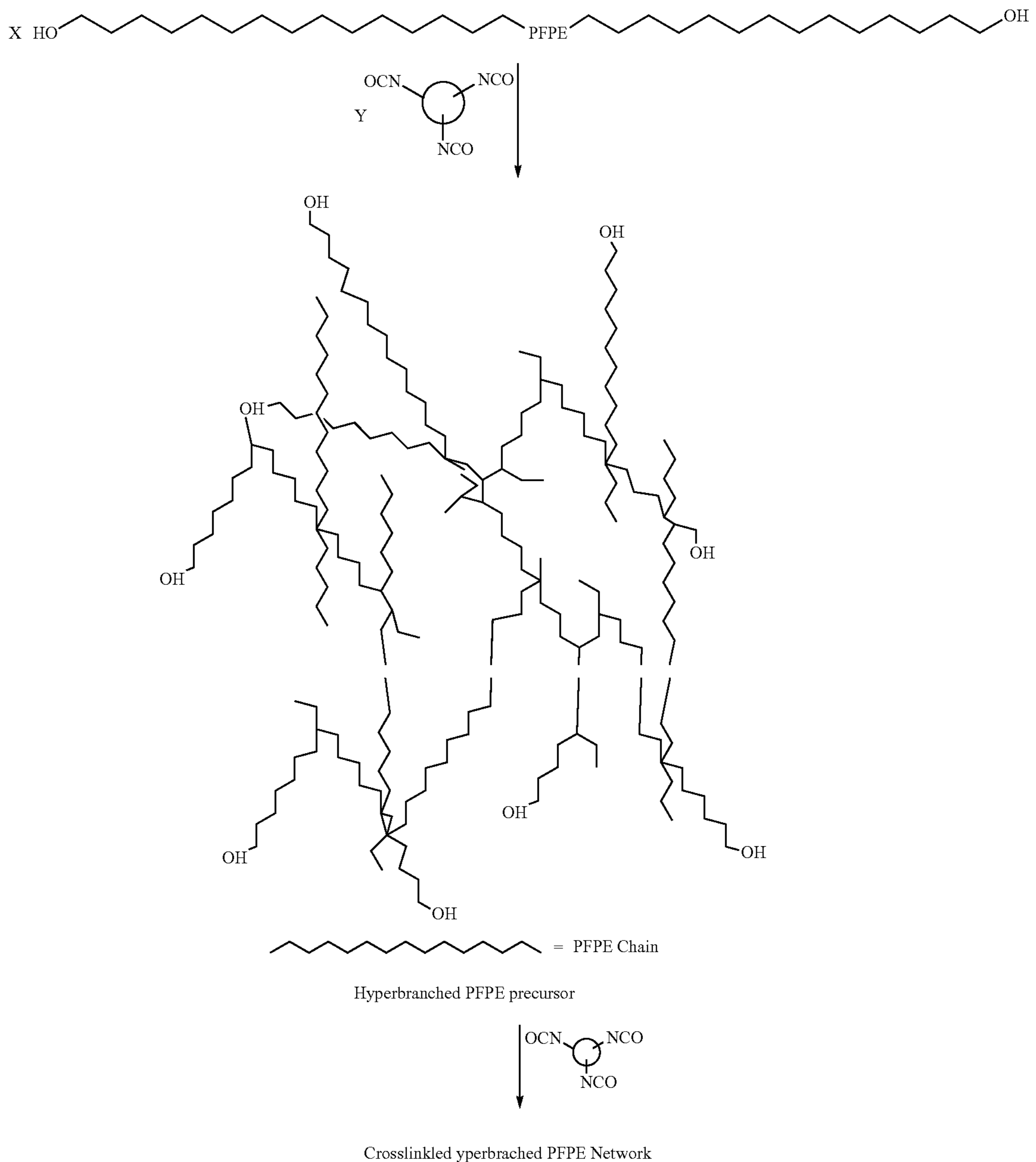
Example 7.6. Synthesis of a Hyperbranched PFPE Precursor
