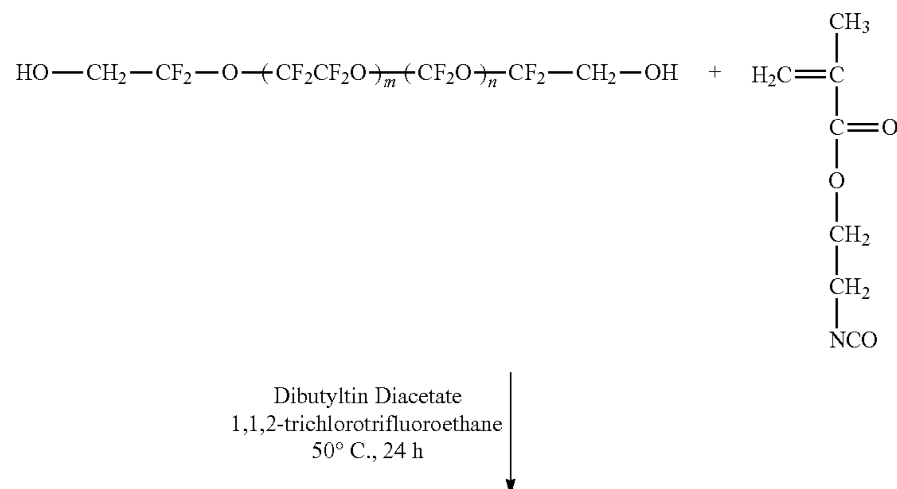
Scheme 1. Synthesis and Photocuring of Functional Perfluoropolyethers.
