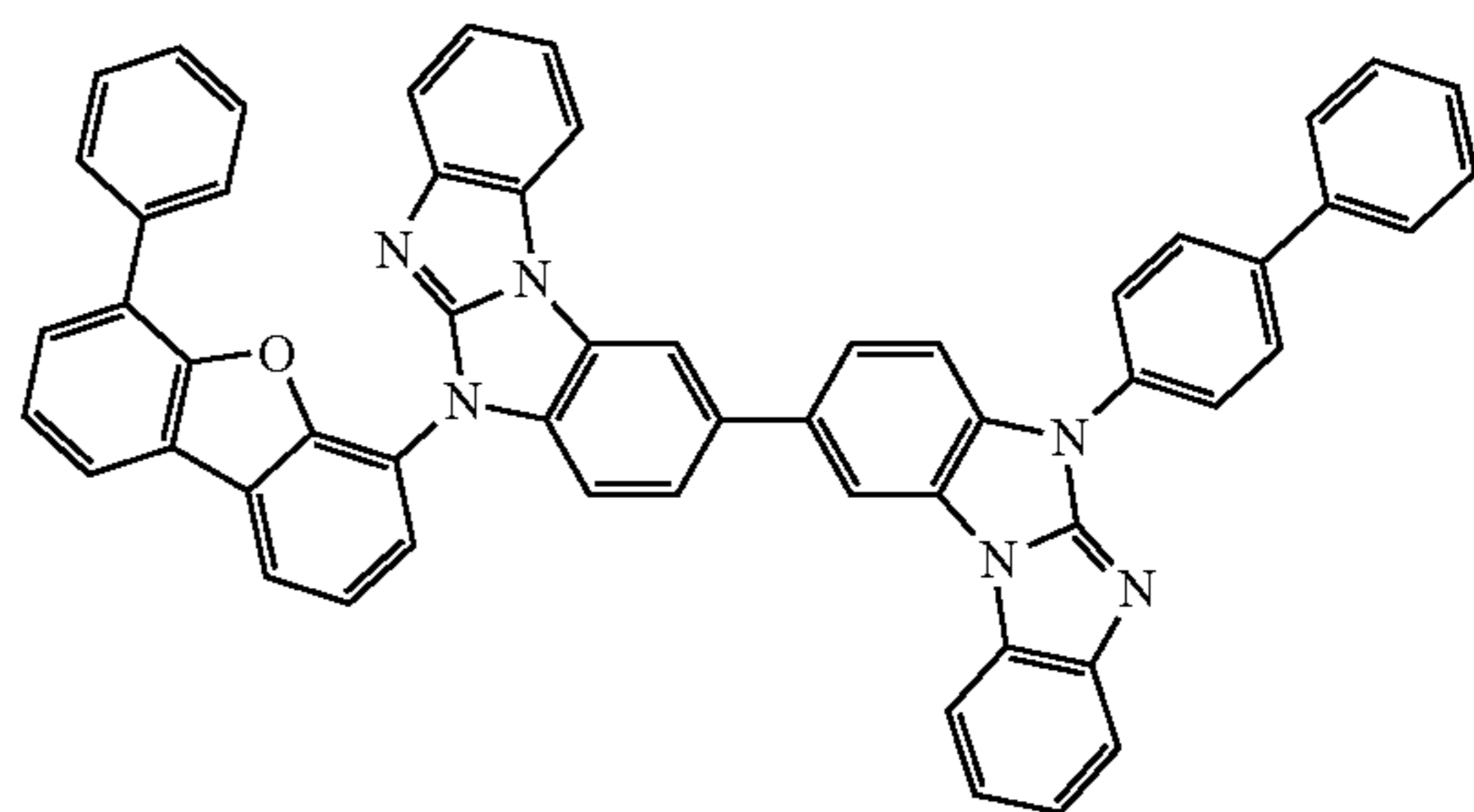
Compound 52
