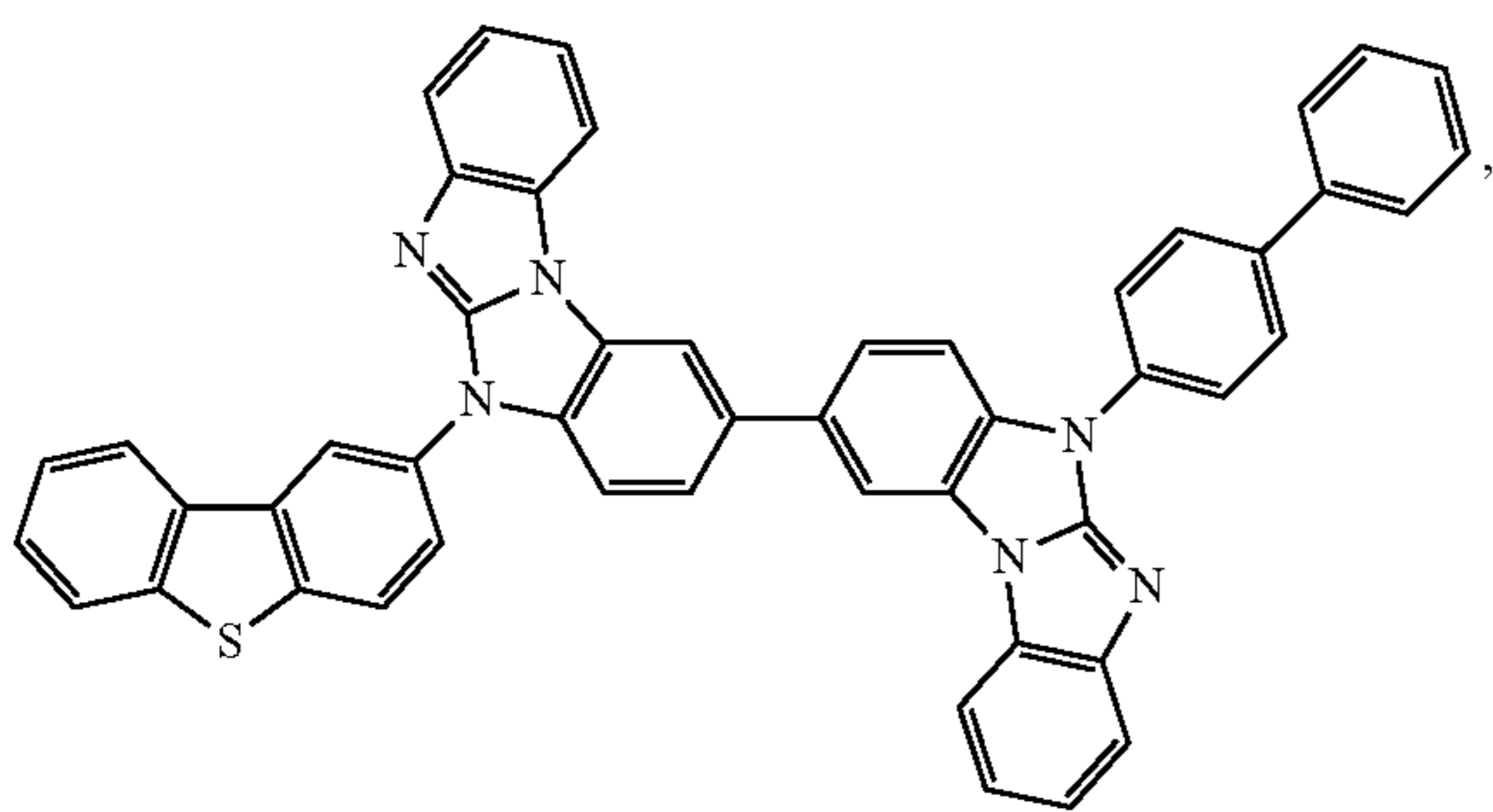
Compound 43
