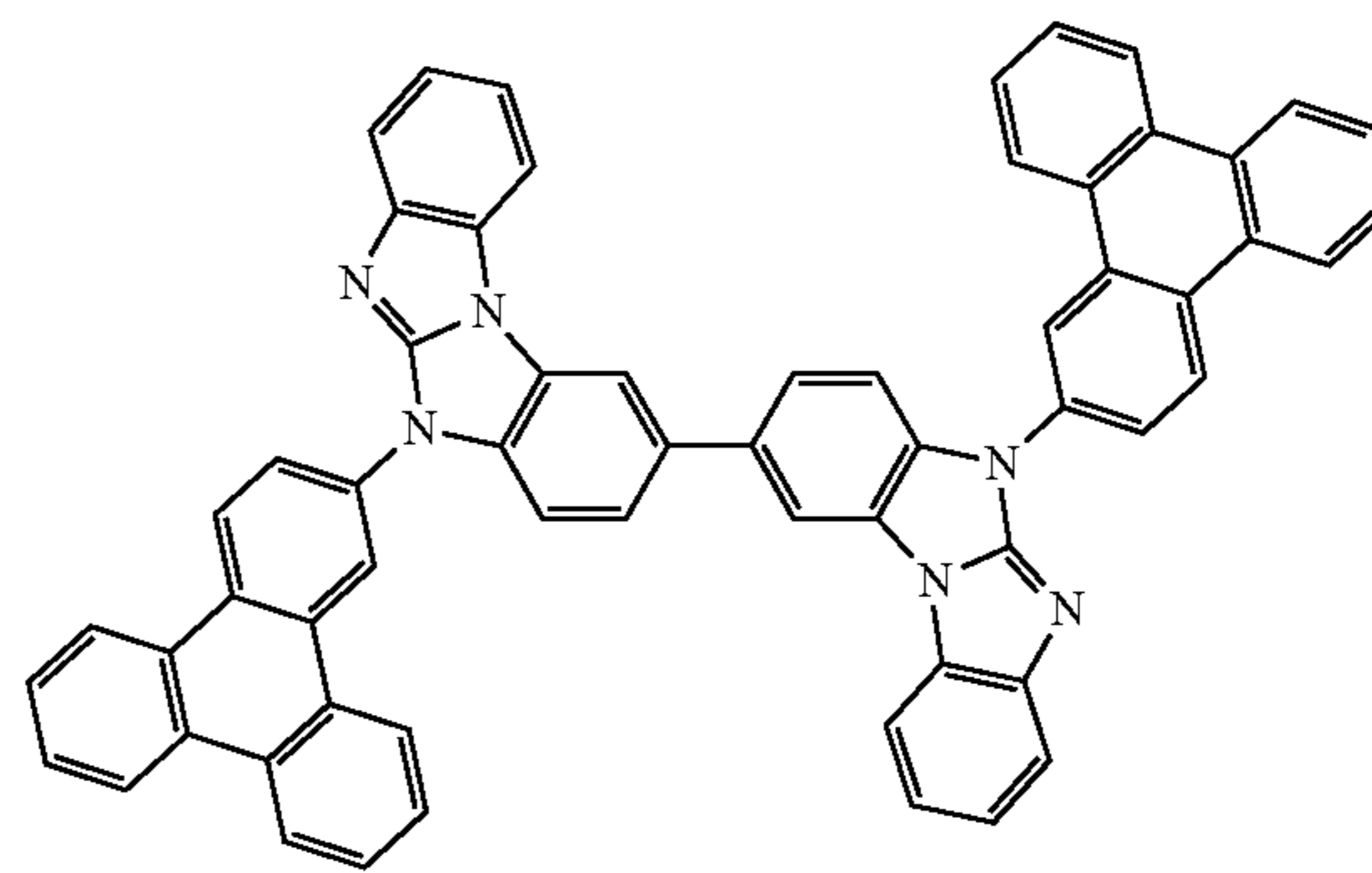
Compound 20
