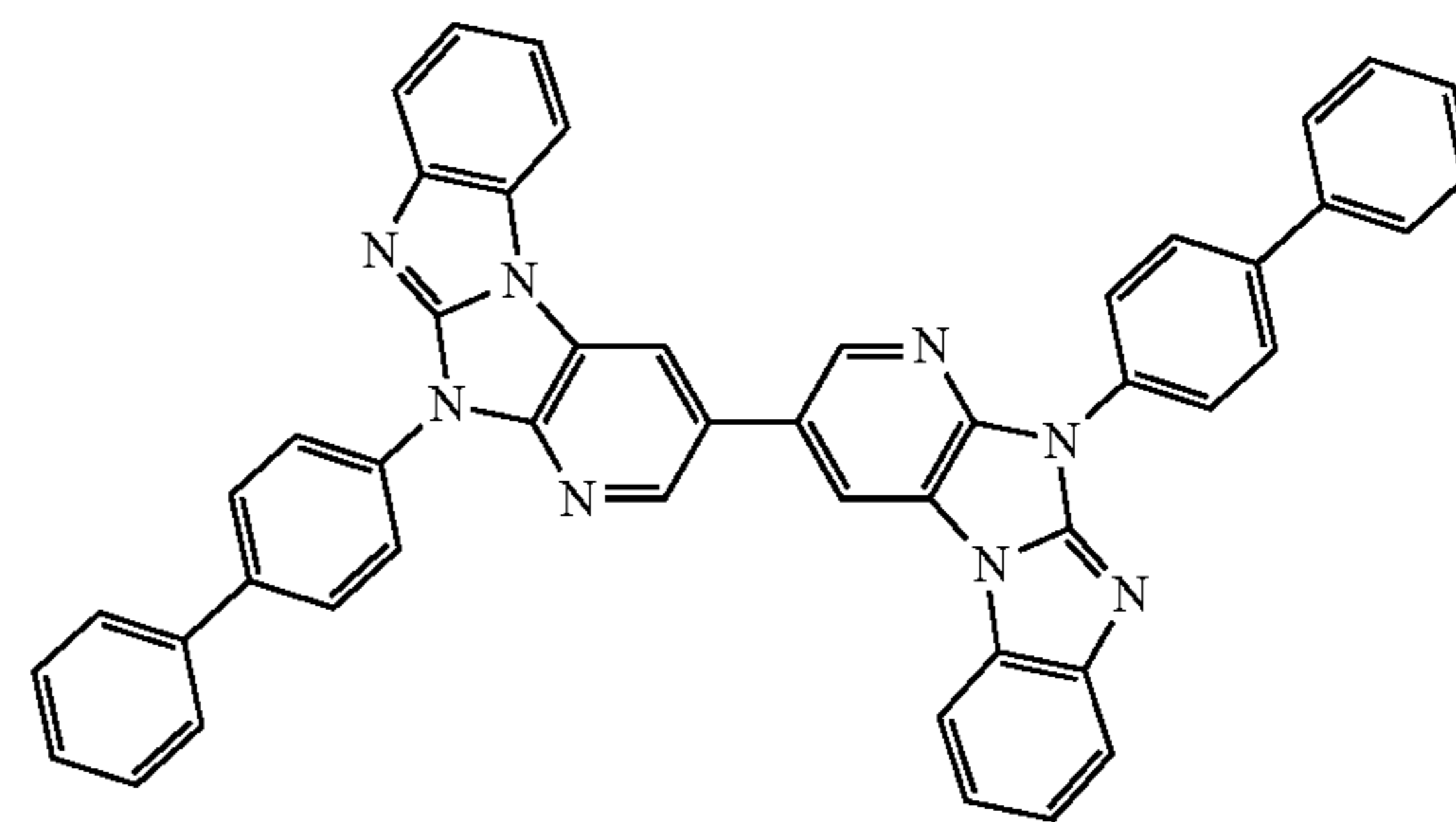
Compound 187
