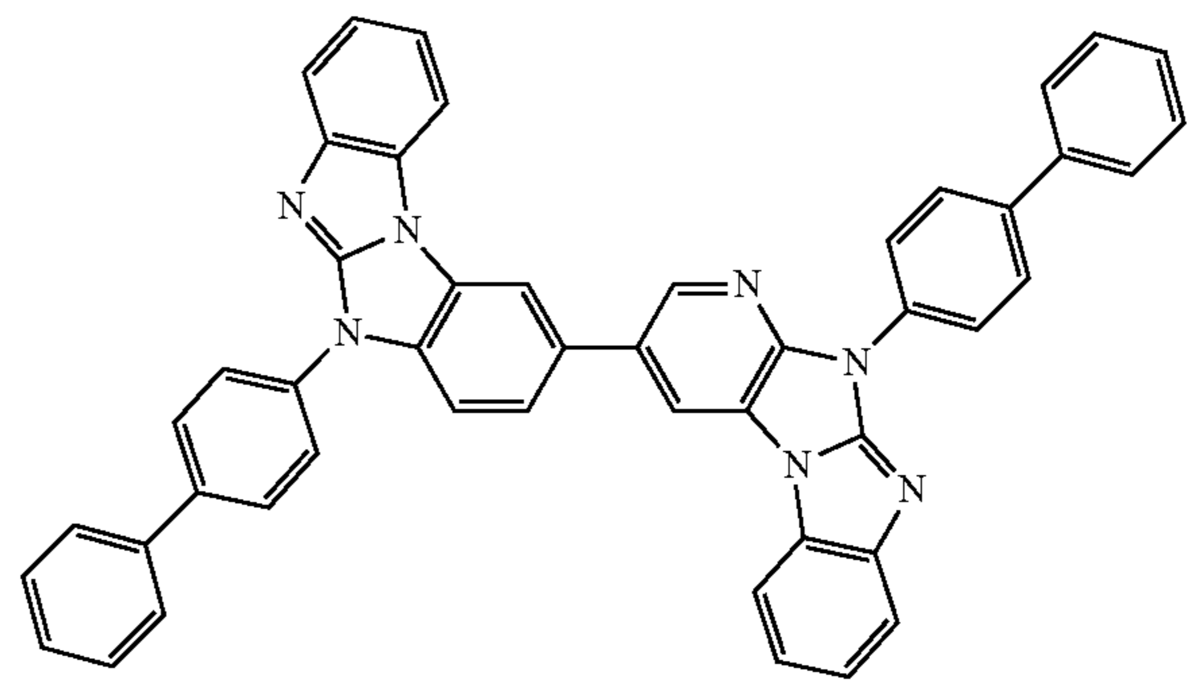
Compound 186
