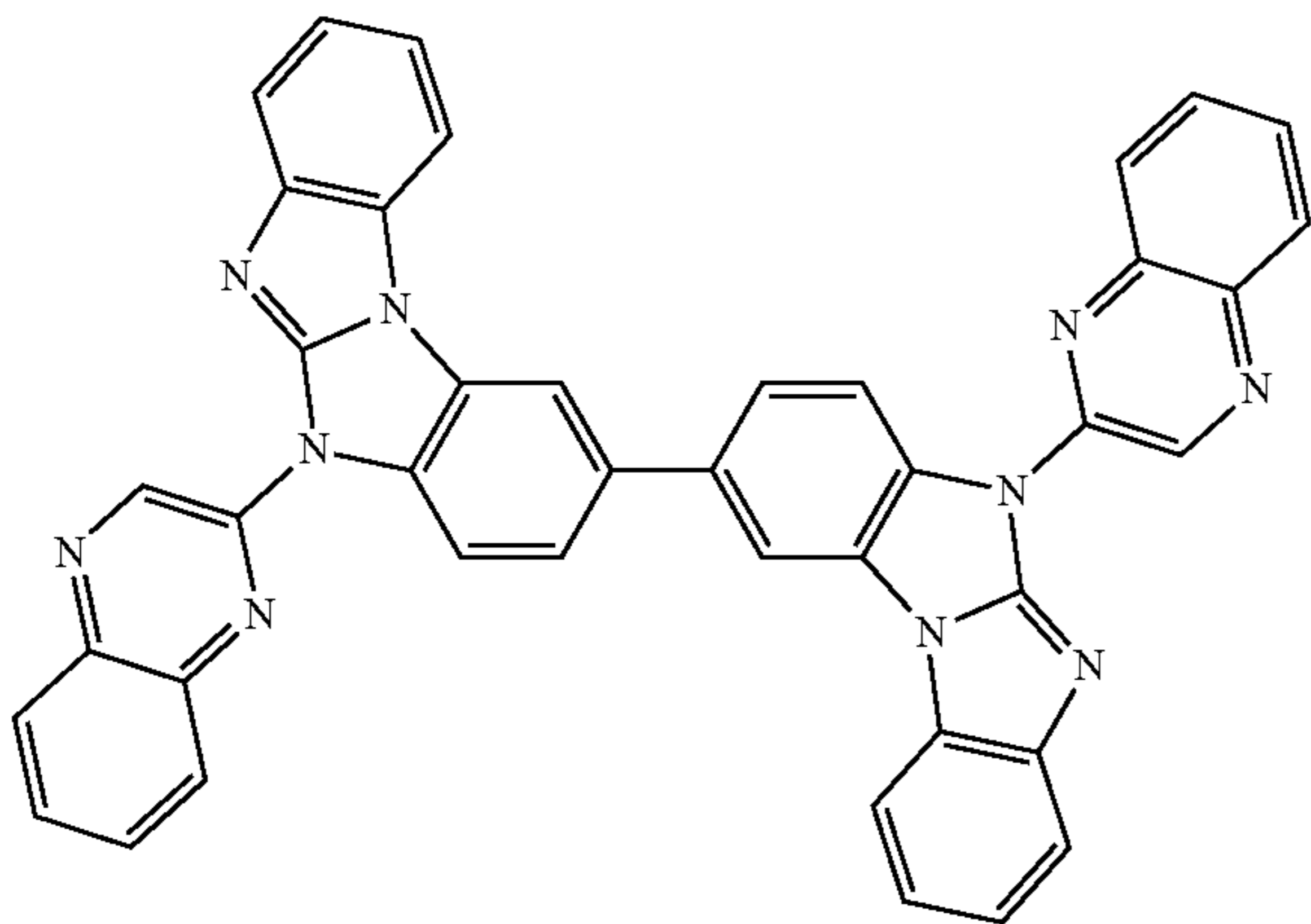
Compound 36
