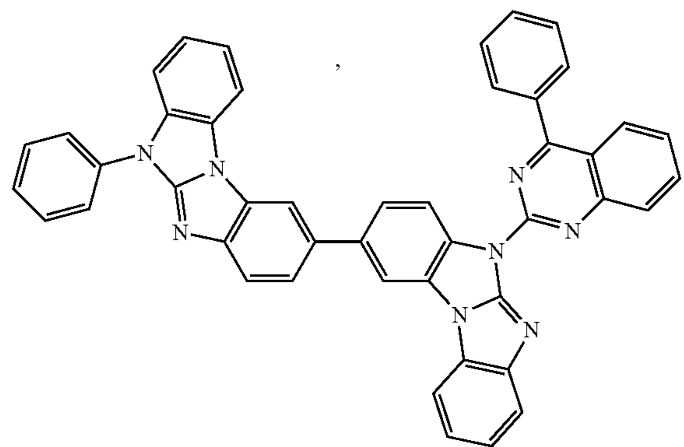
Compound 162
