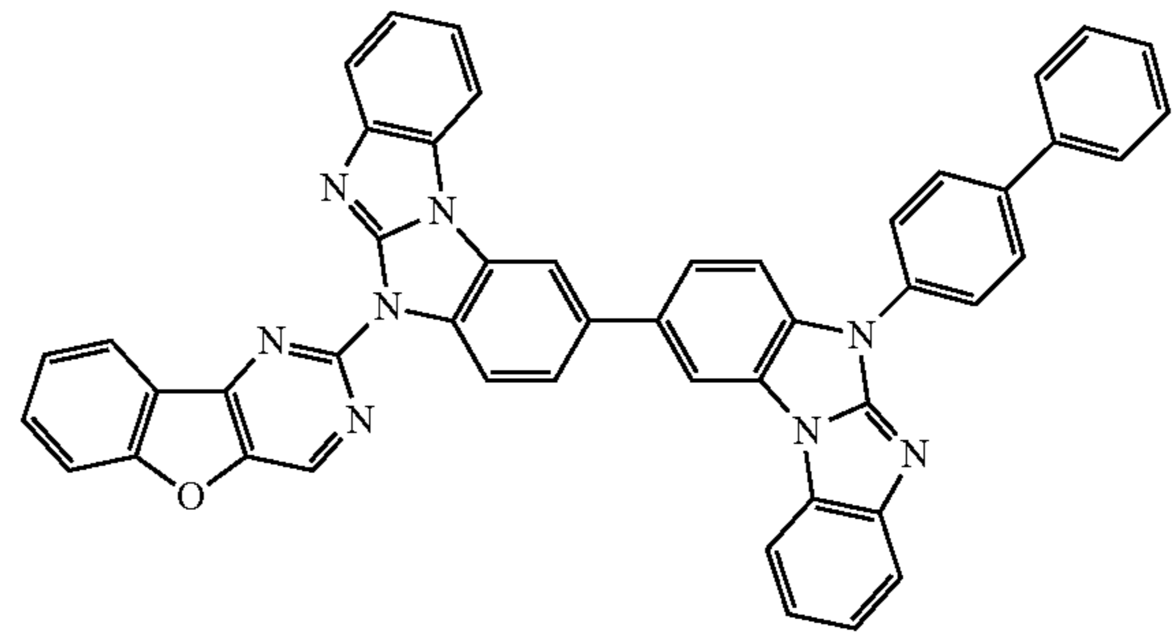
Compound 68
