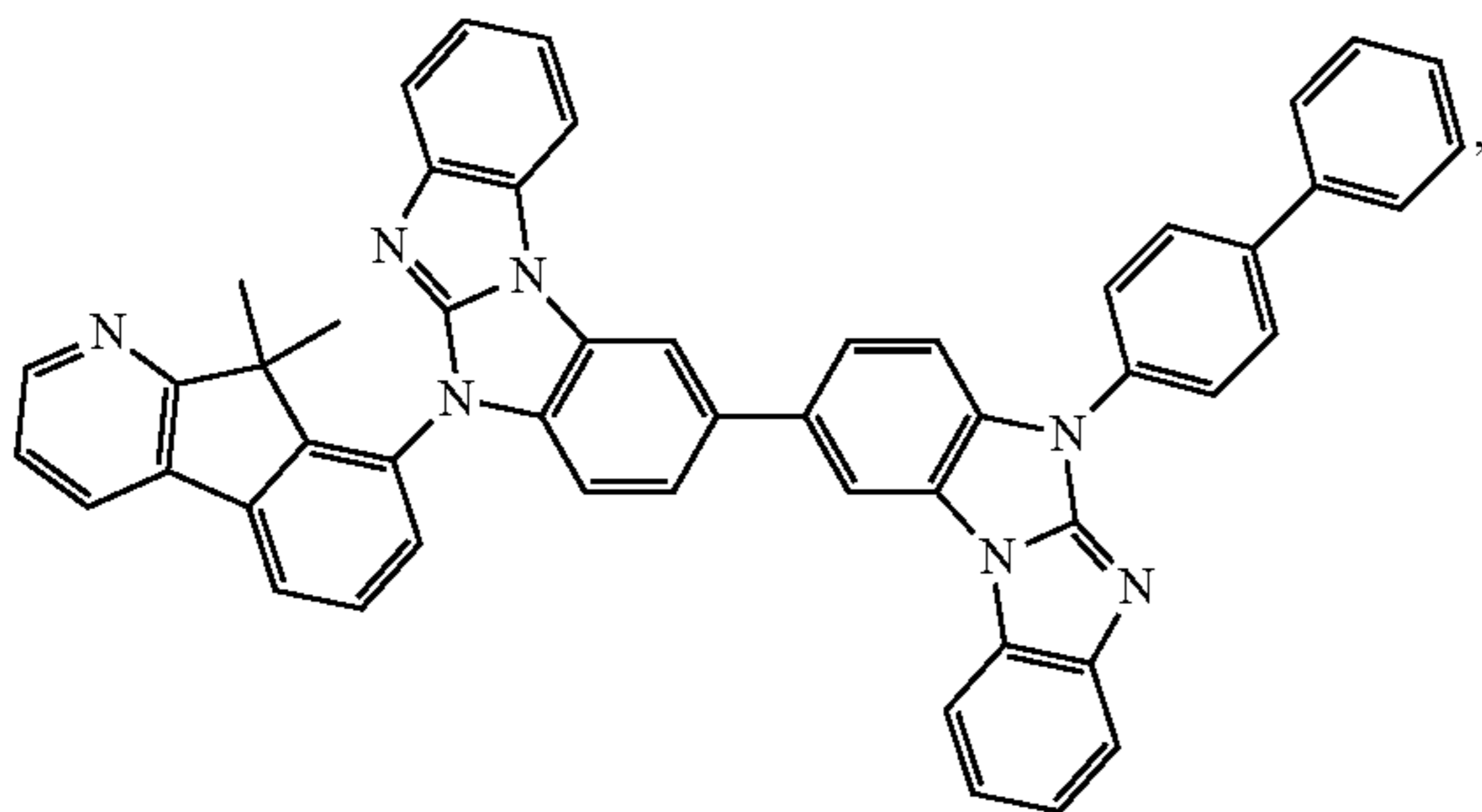
Compound 63
