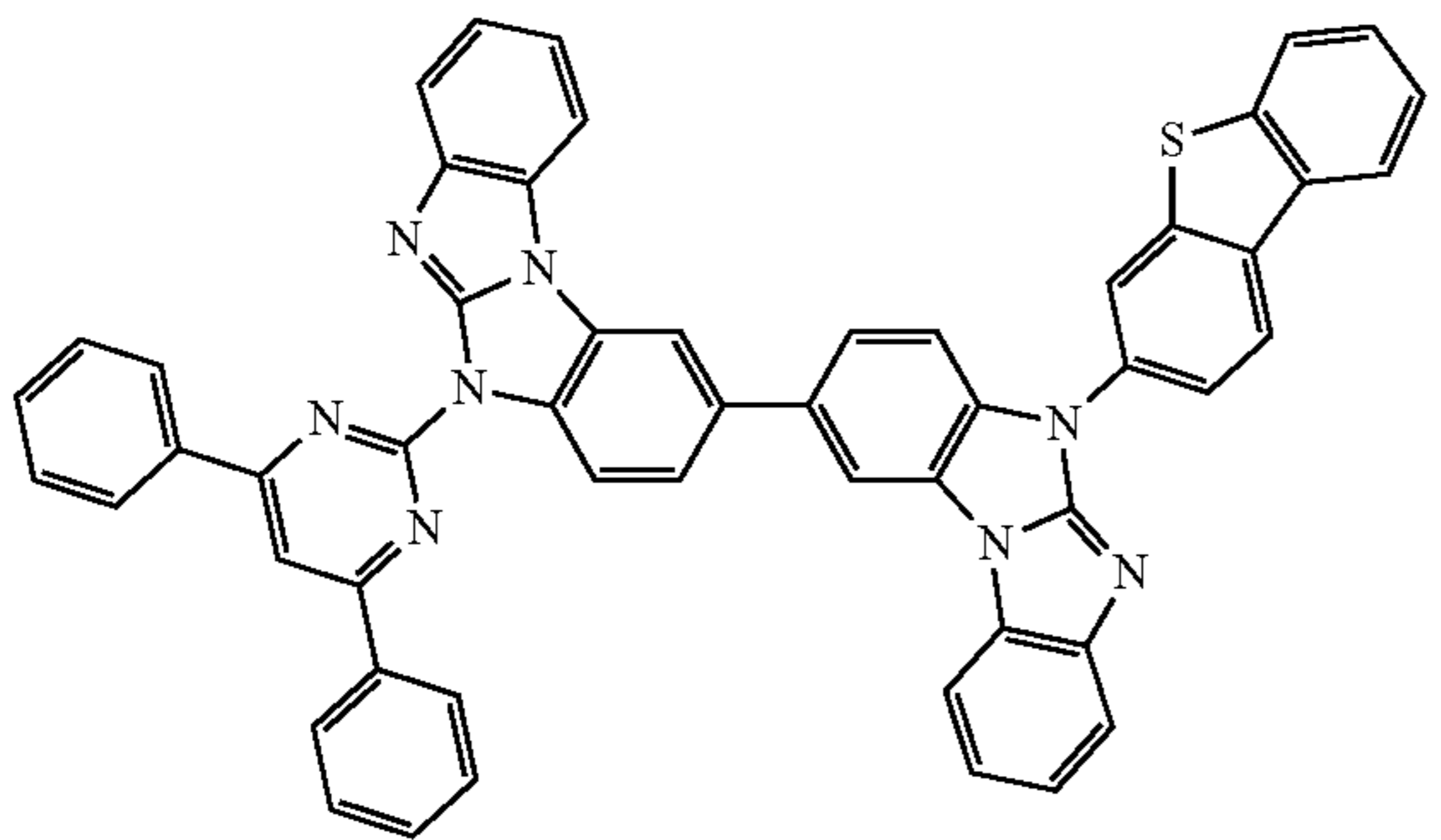
Compound 143
