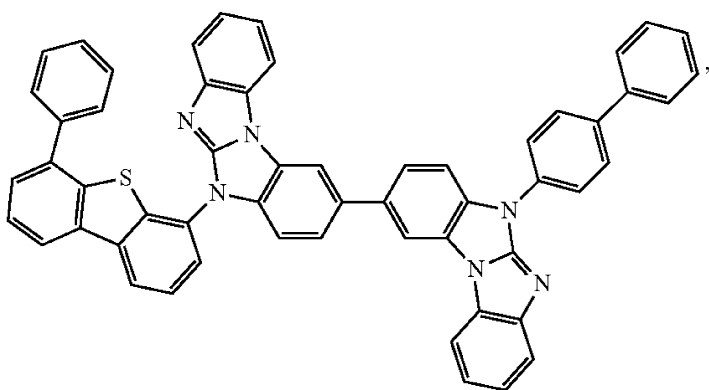
Compound 51
