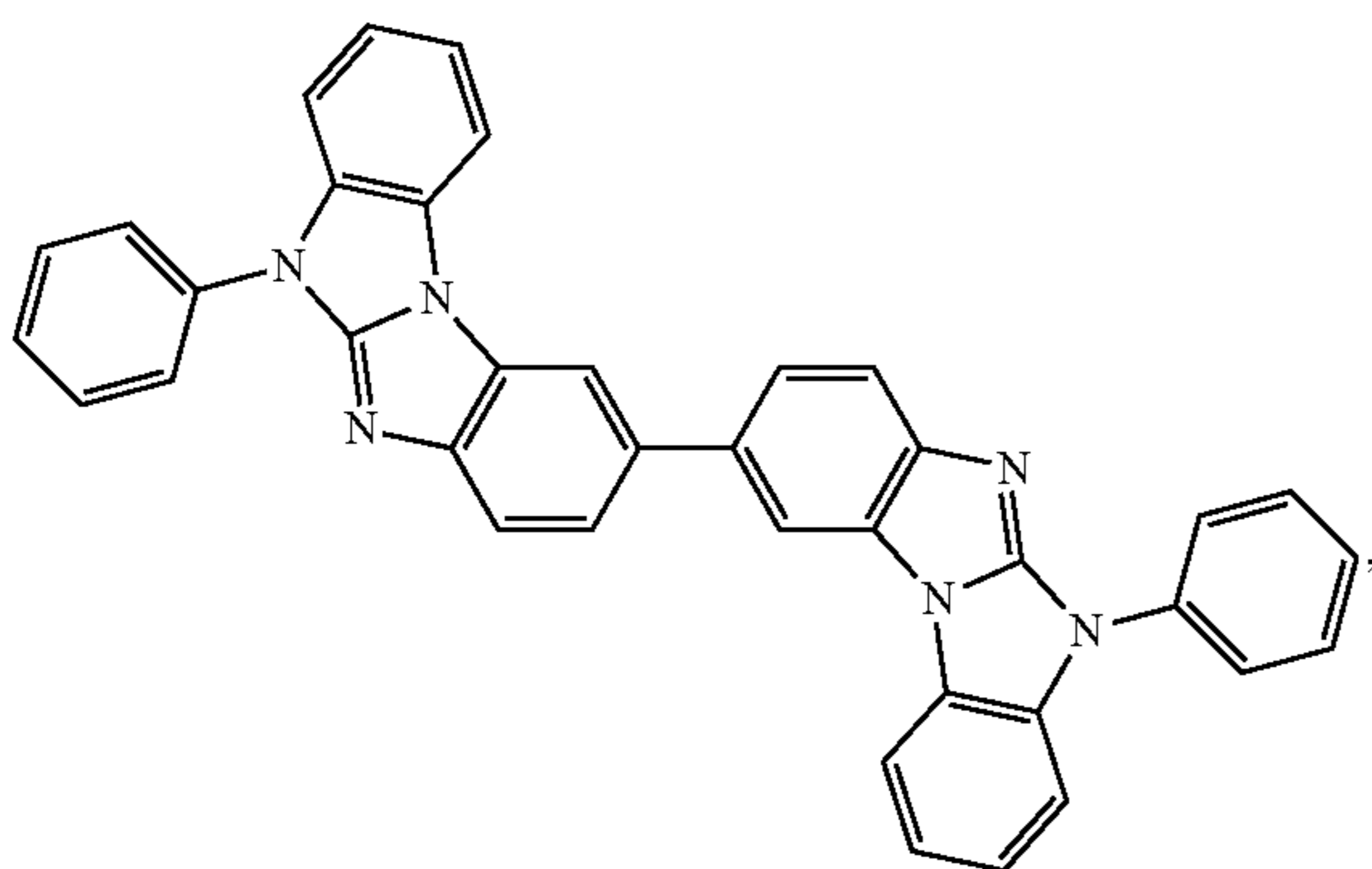
Compound 161
