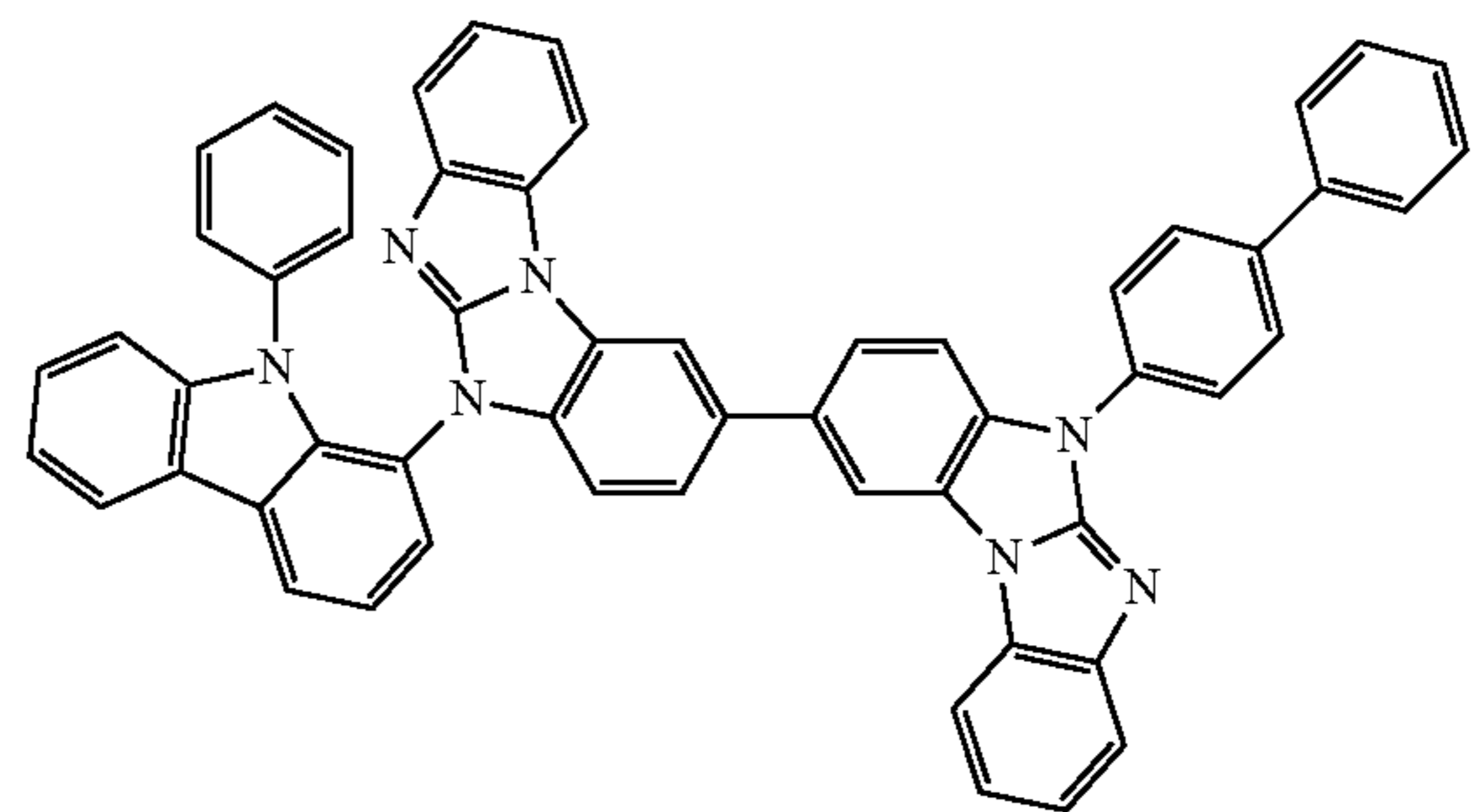
Compound 50
