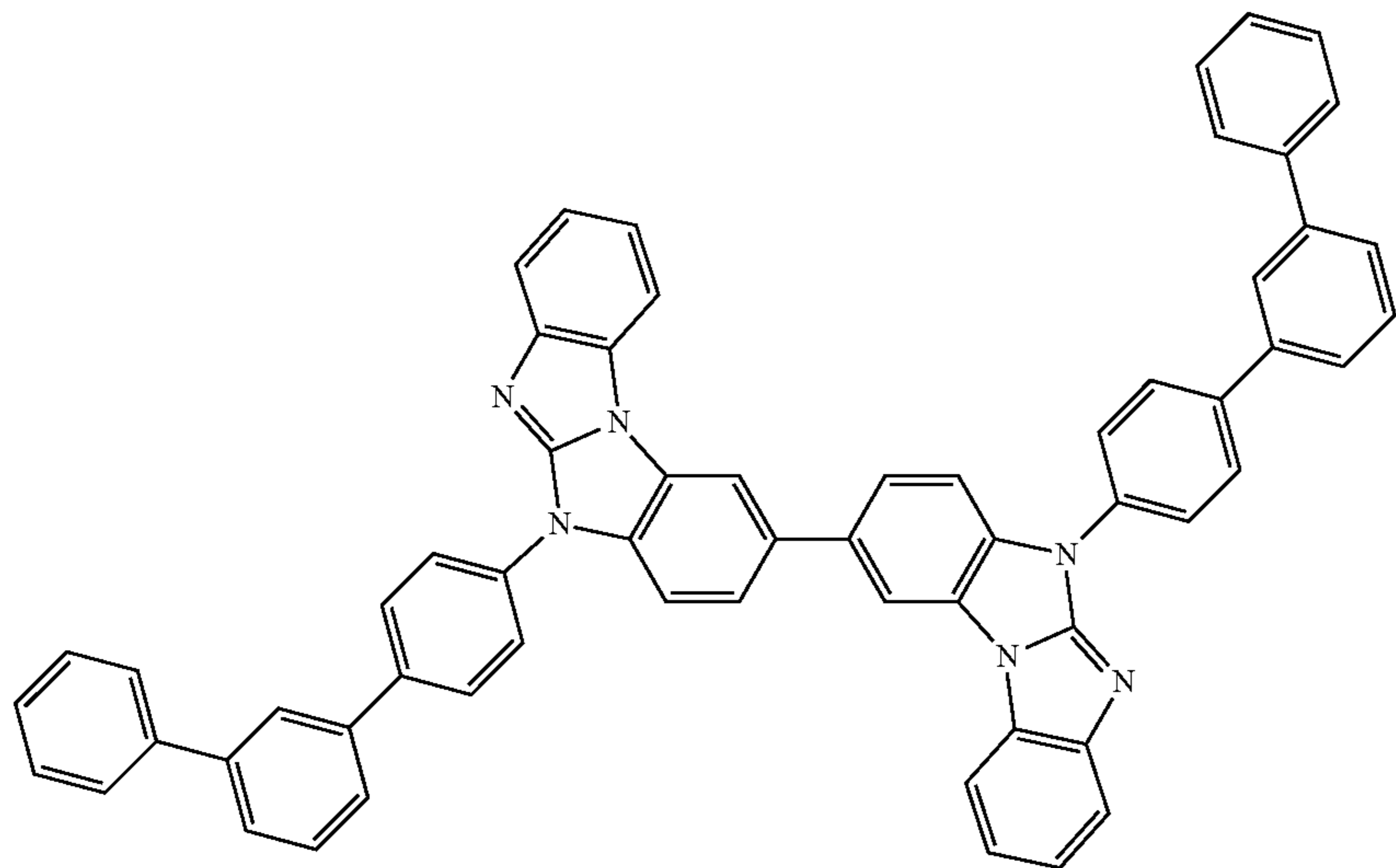
Compound 6
