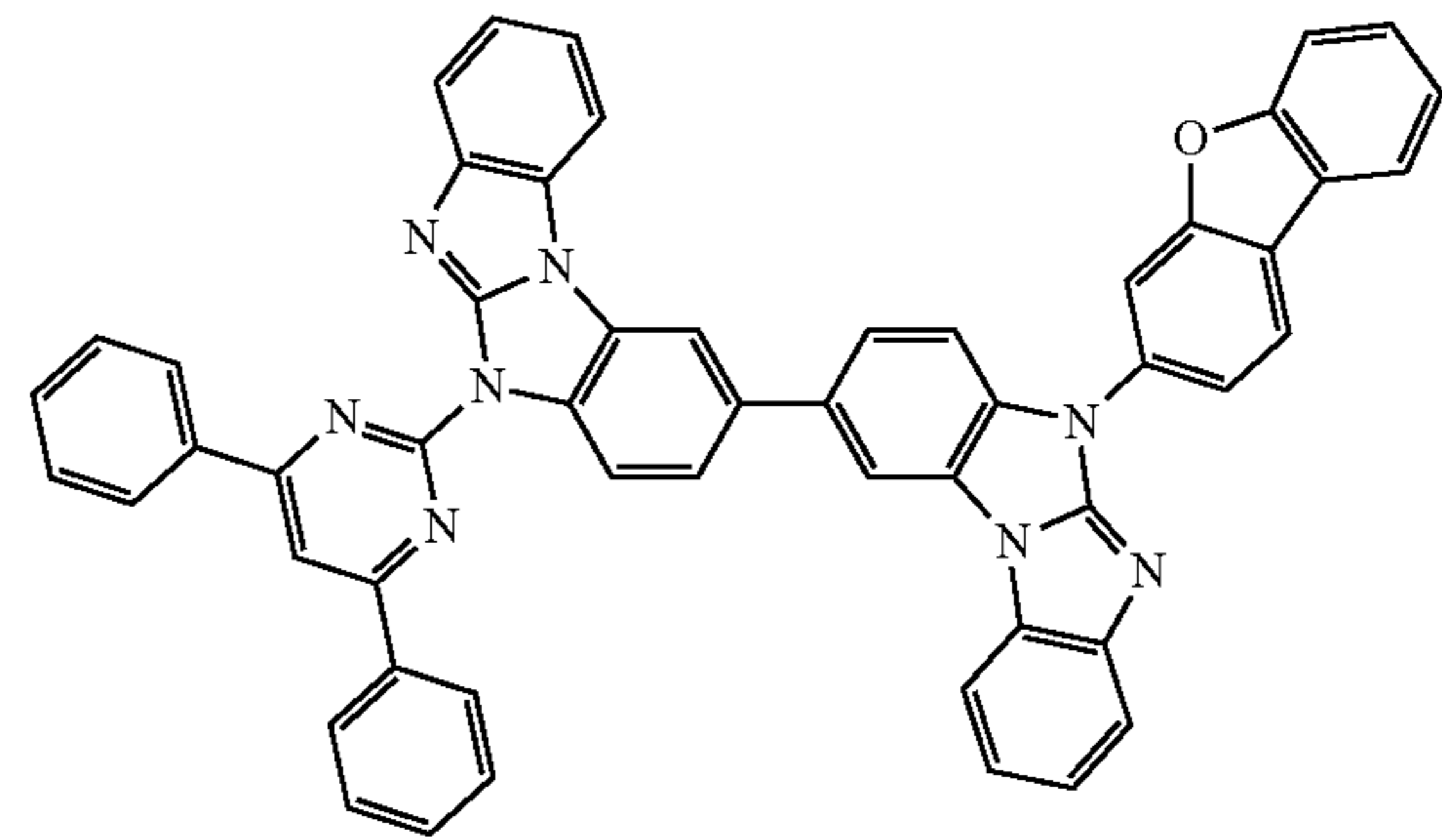
Compound 142
