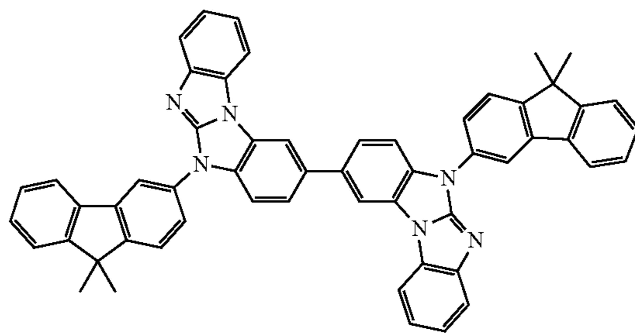
Compound 11
