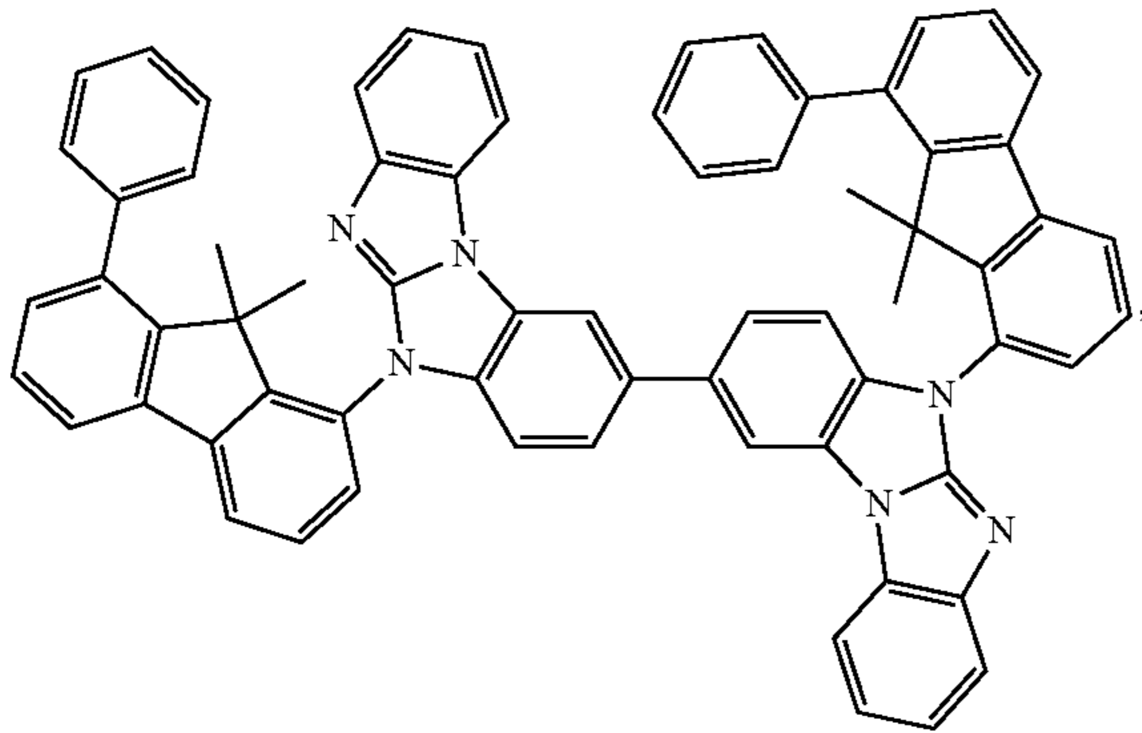
Compound 19
