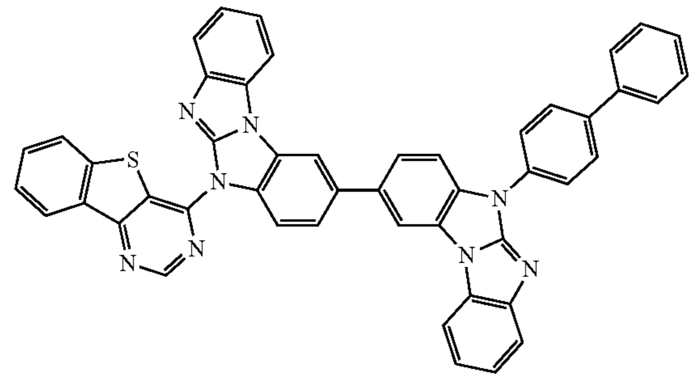
Compound 64
