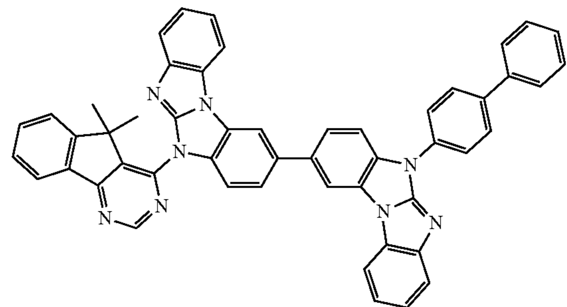
Compound 66
