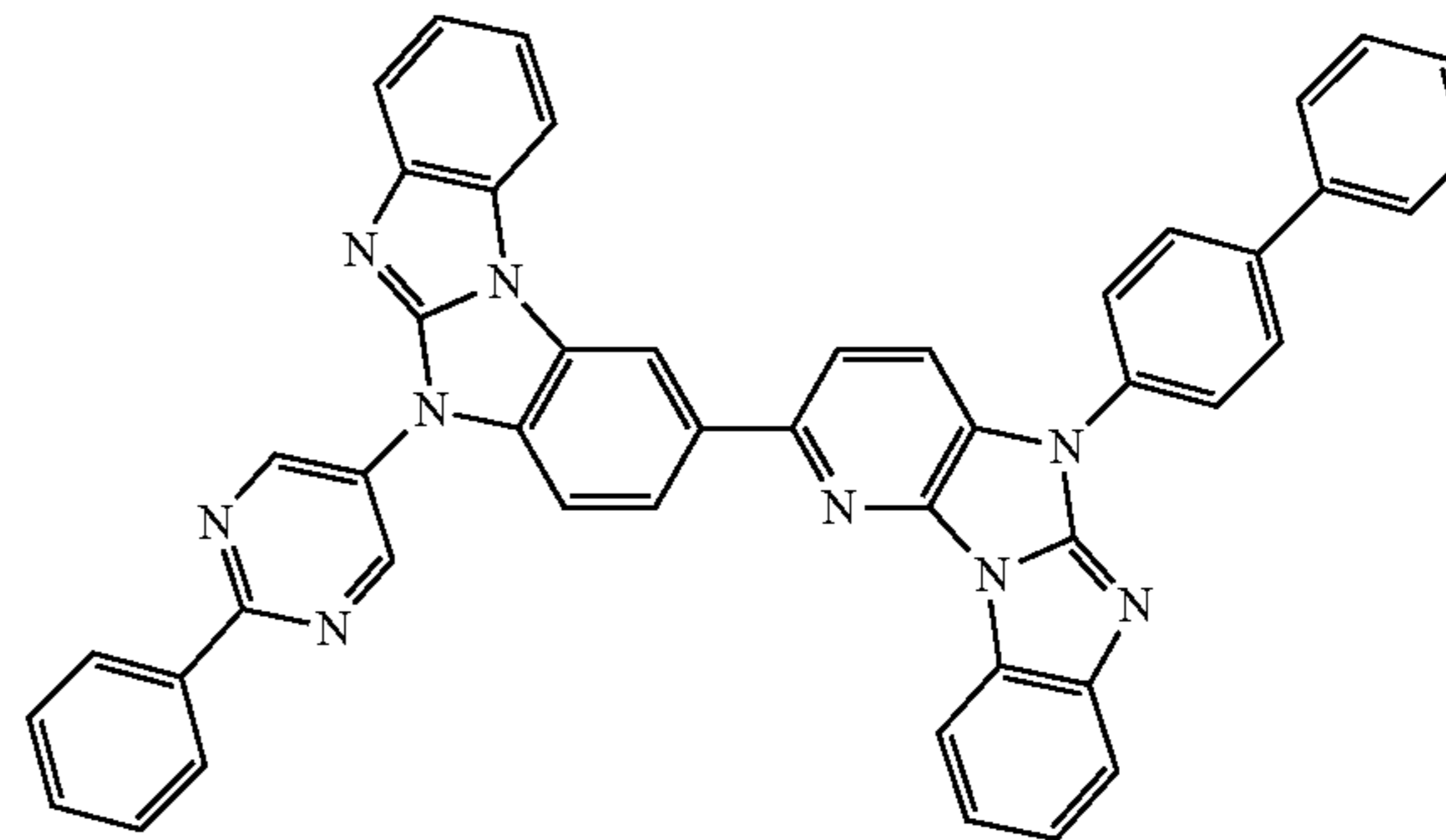
Compound 70
