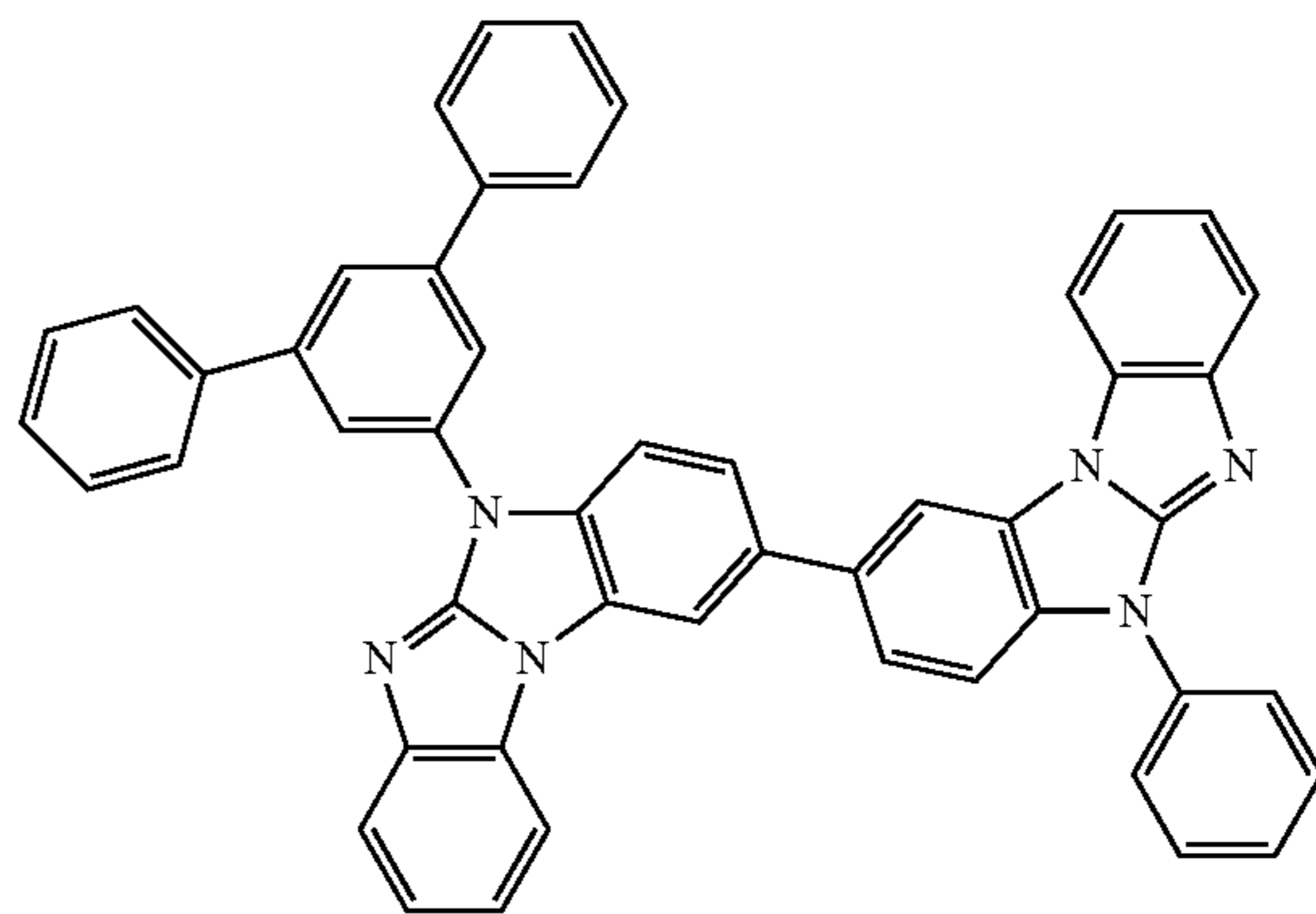
Compound 193
