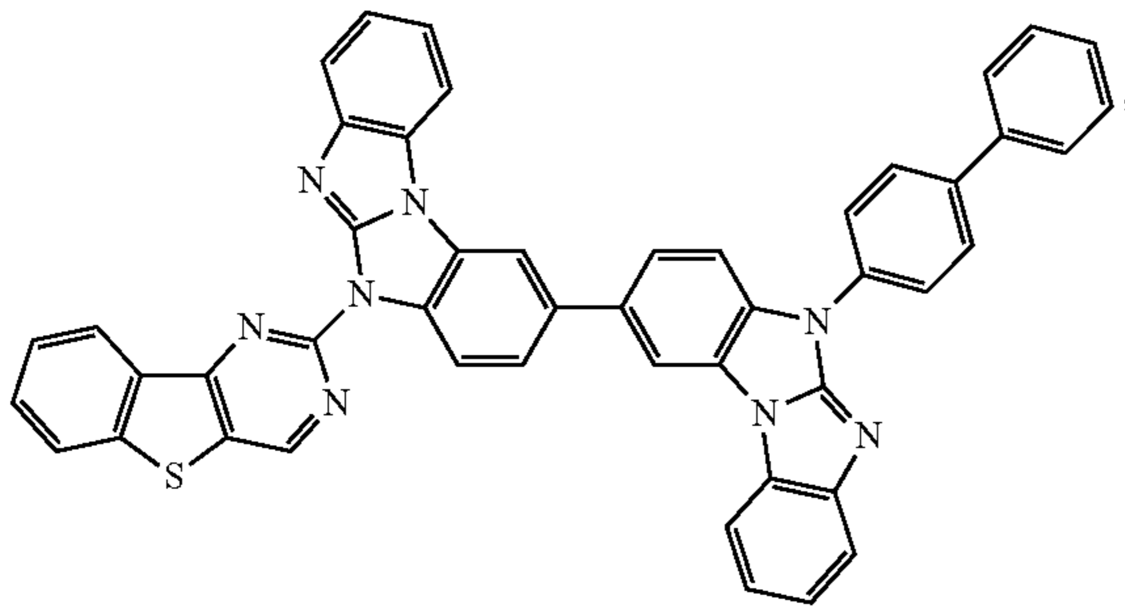
Compound 67
