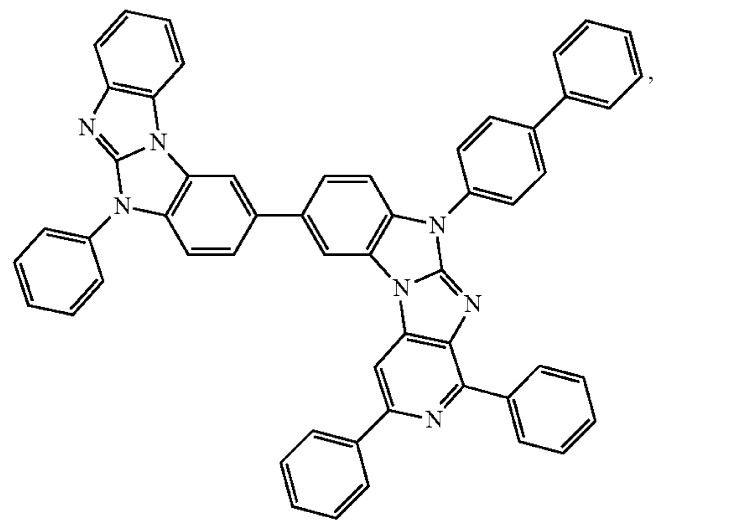
Compound 188
