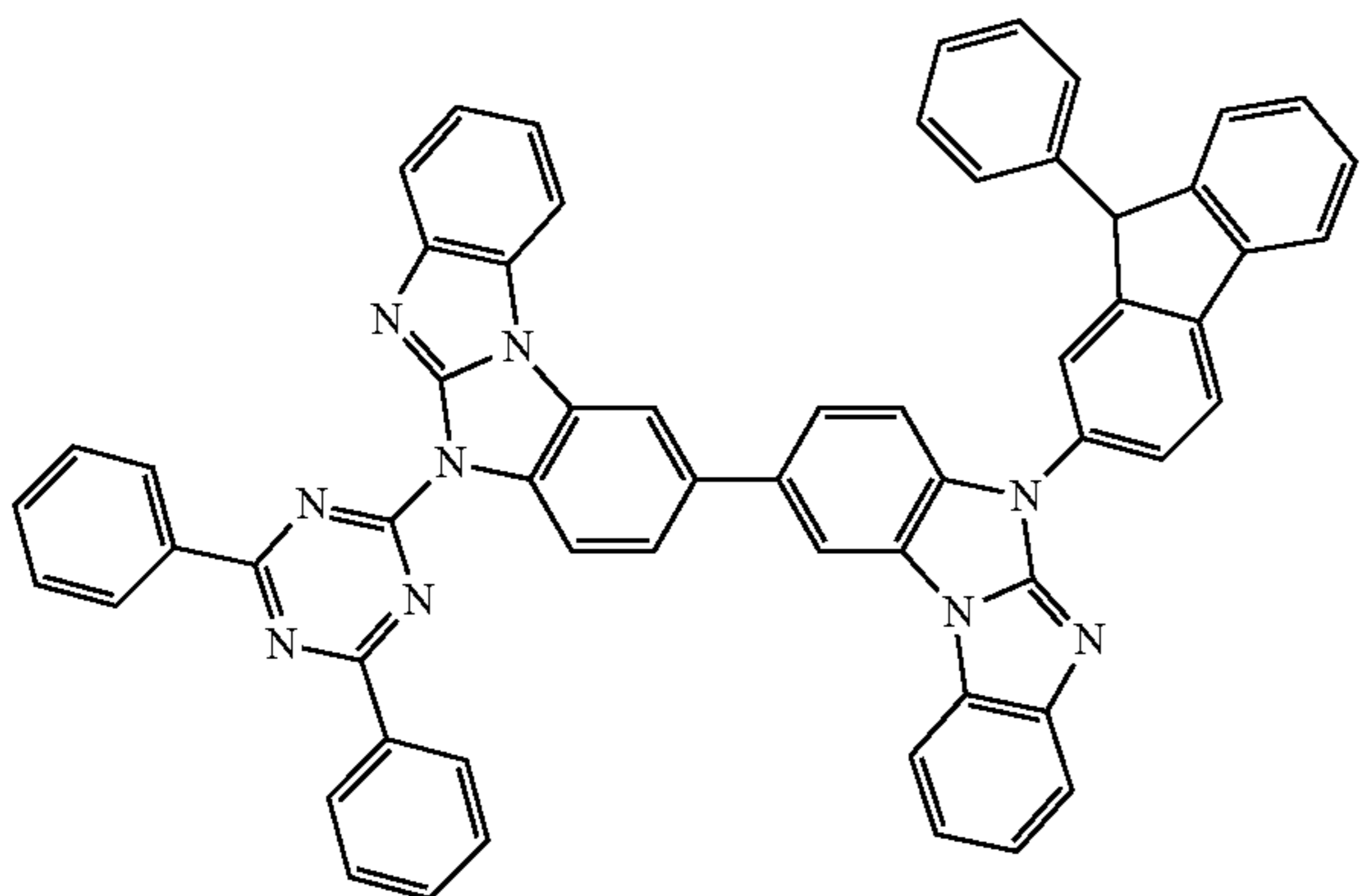
Compound 145
