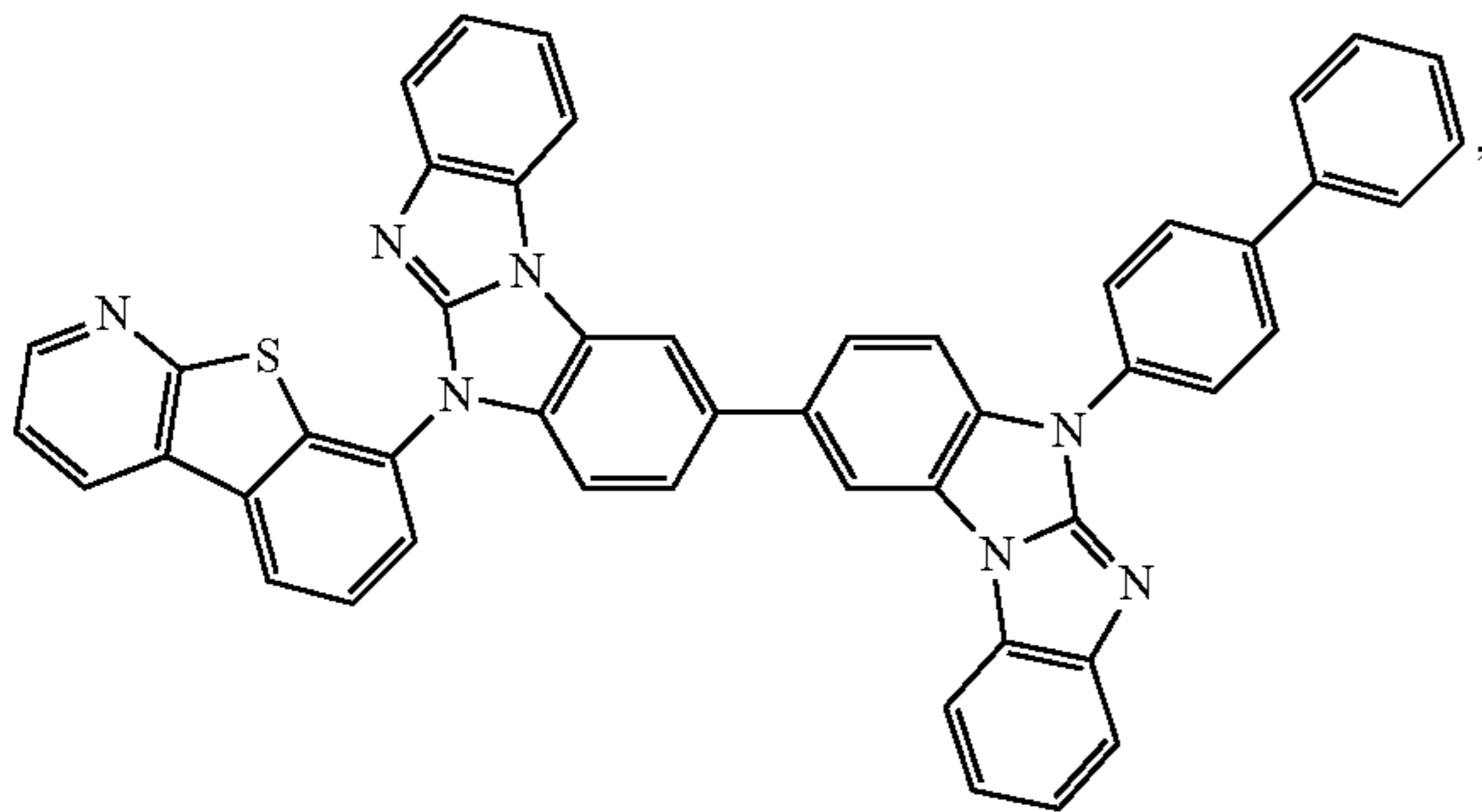
Compound 61
