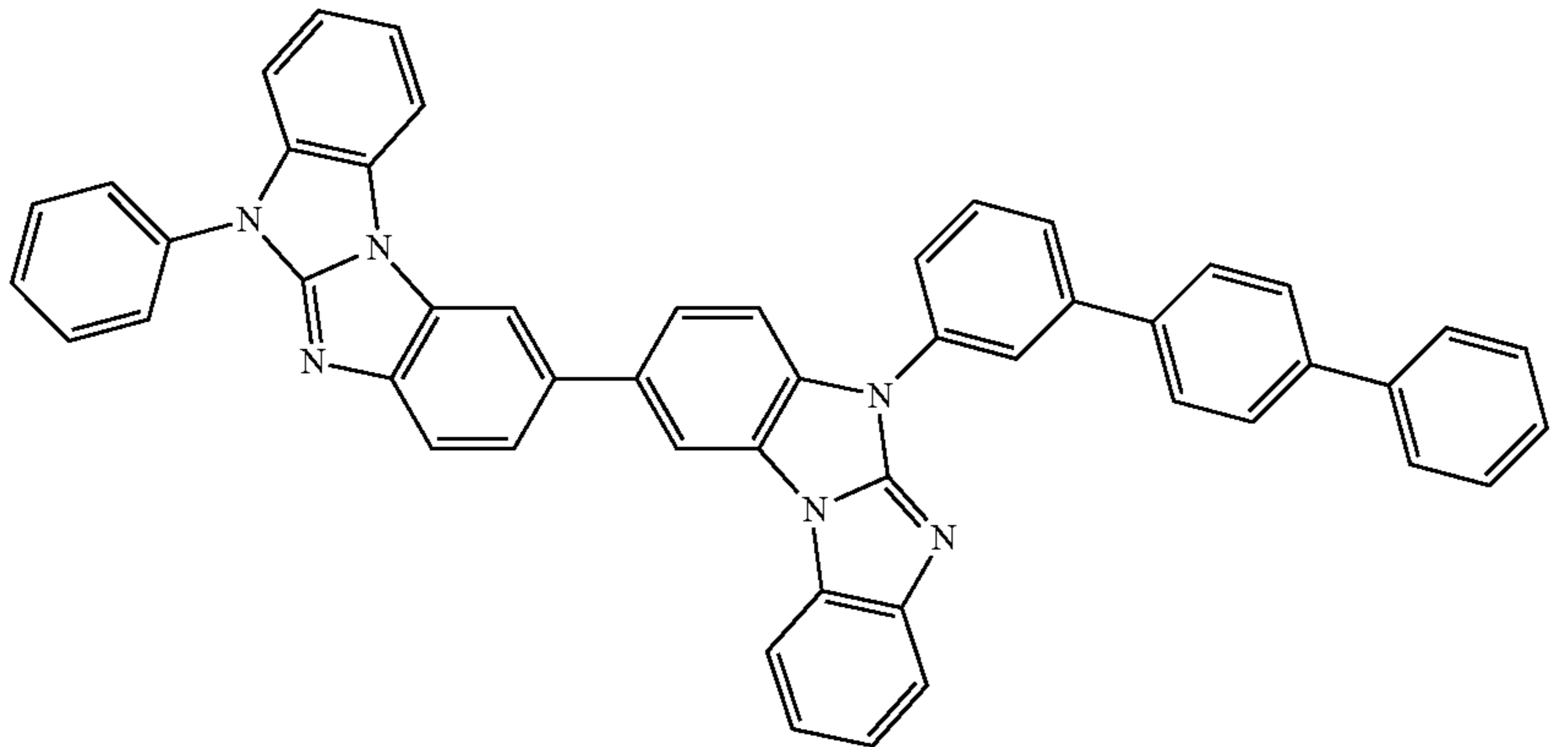
Compound 159
