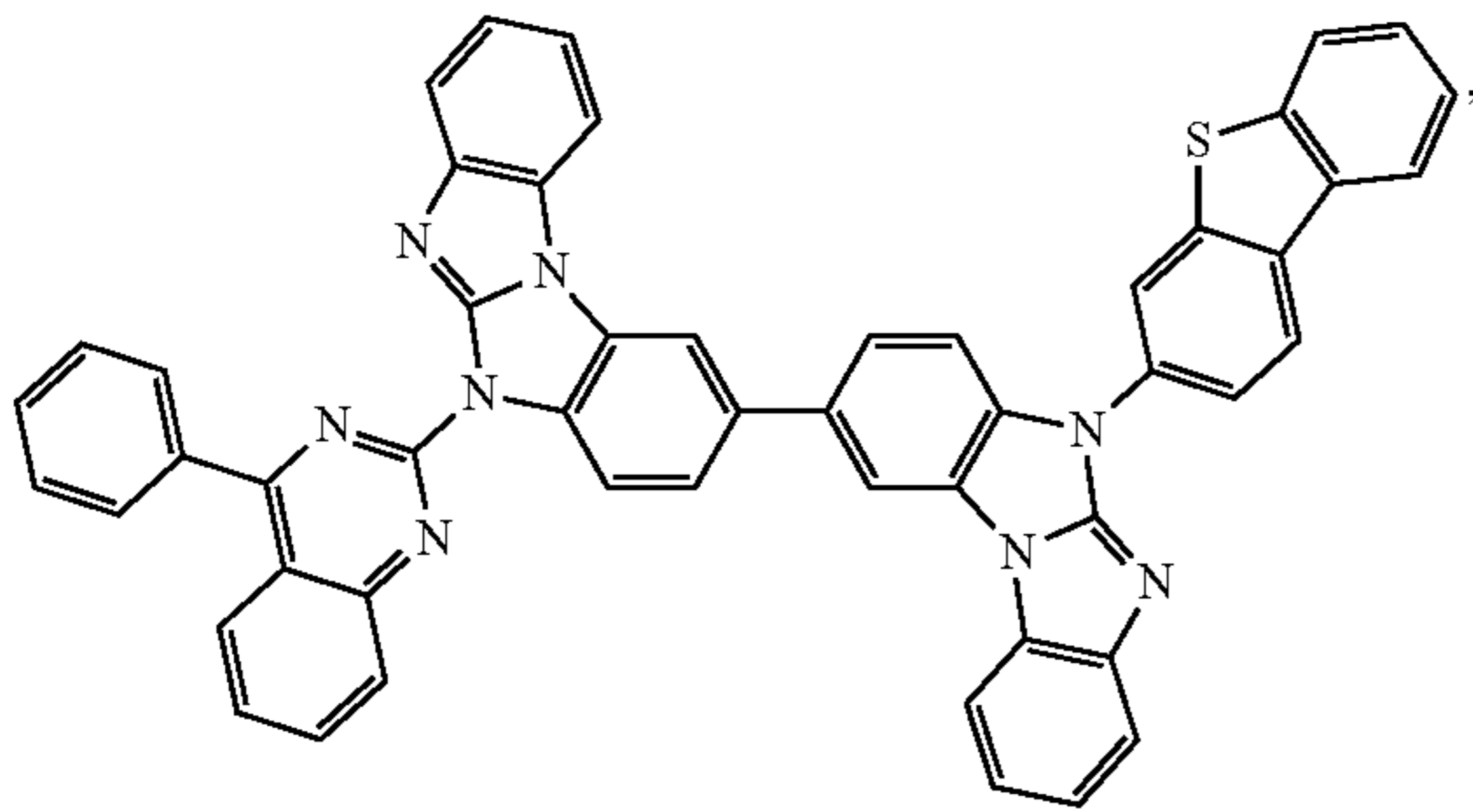
Compound 147
