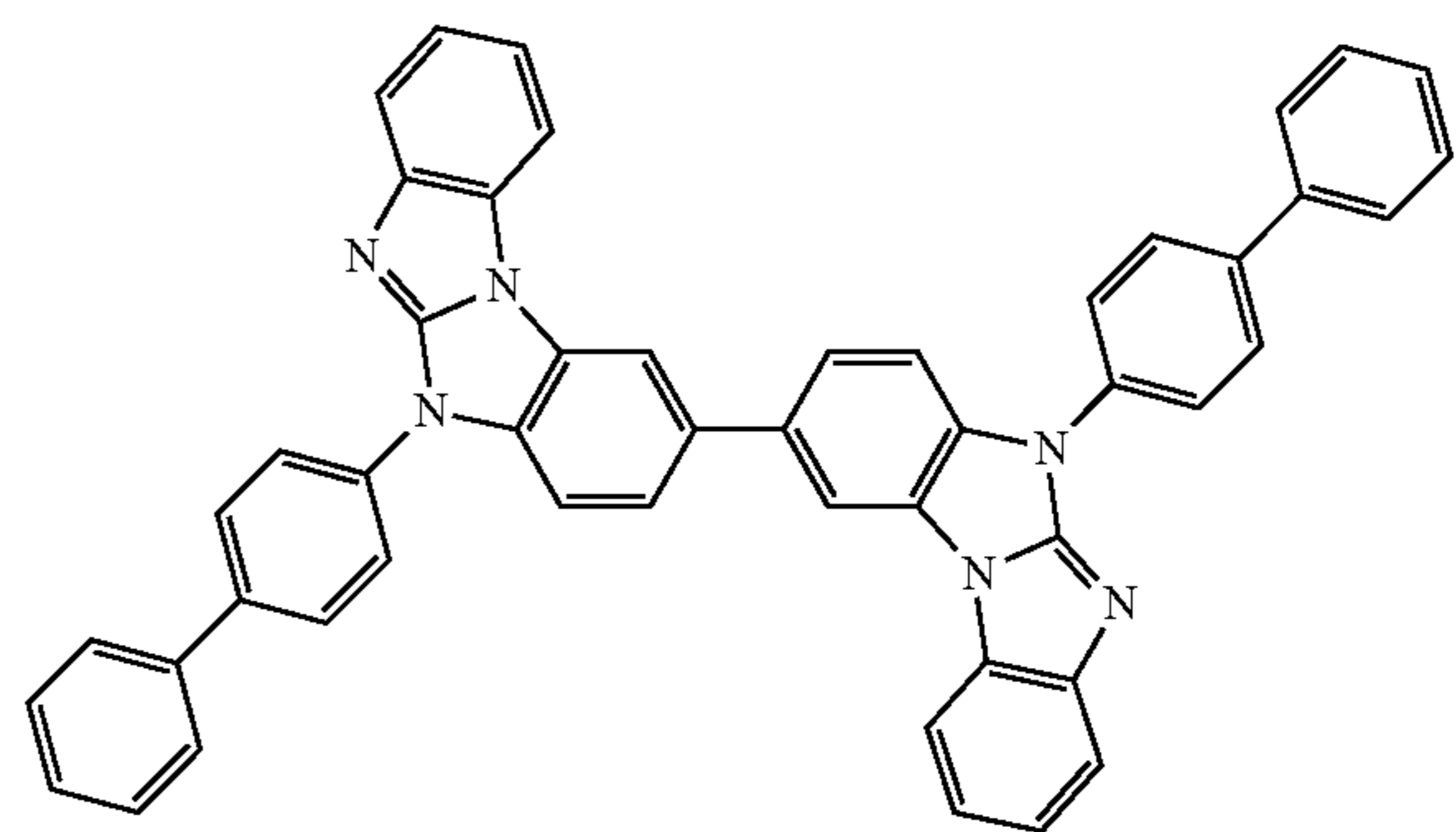
Compound 2
