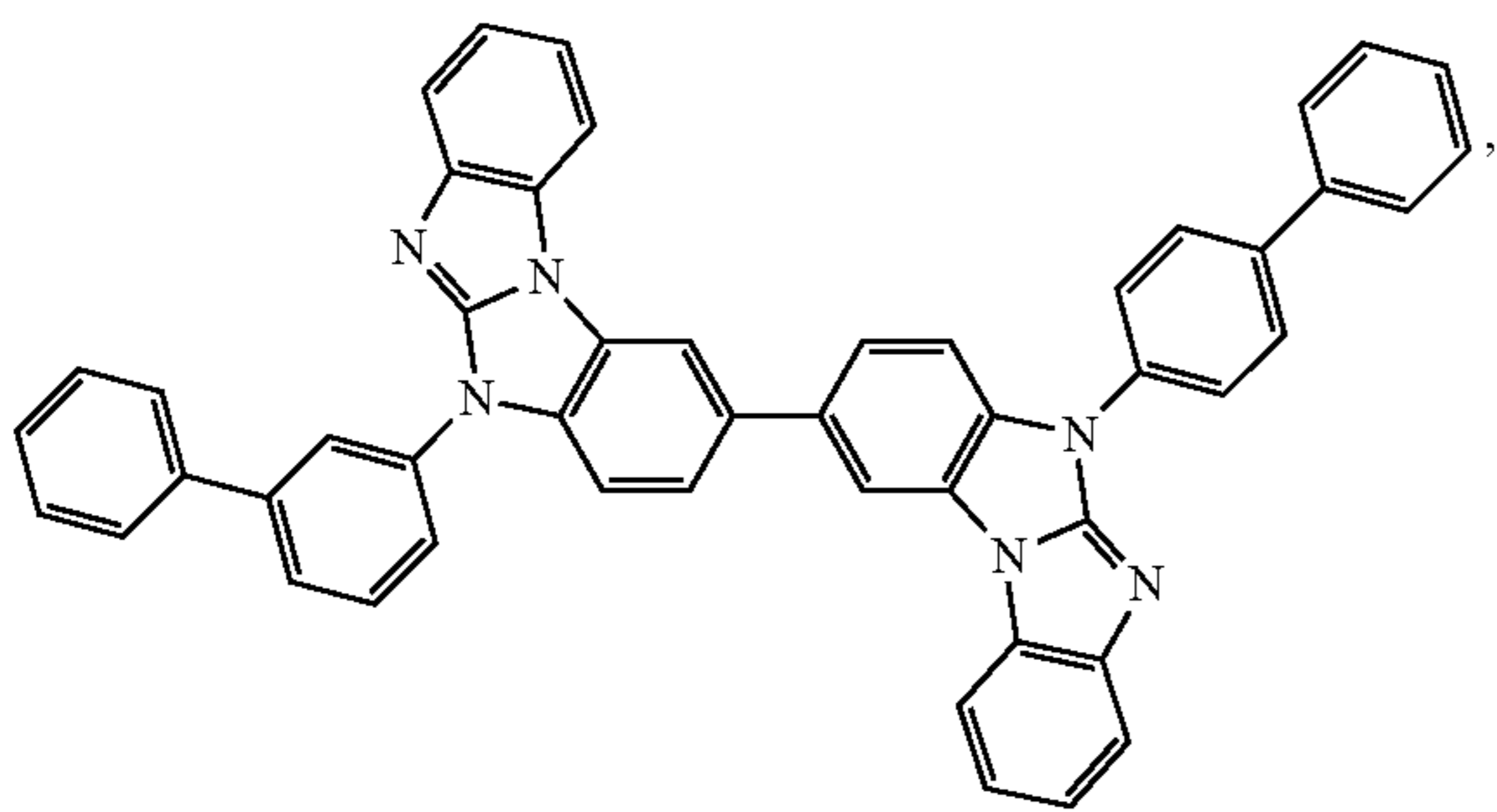
Compound 40
