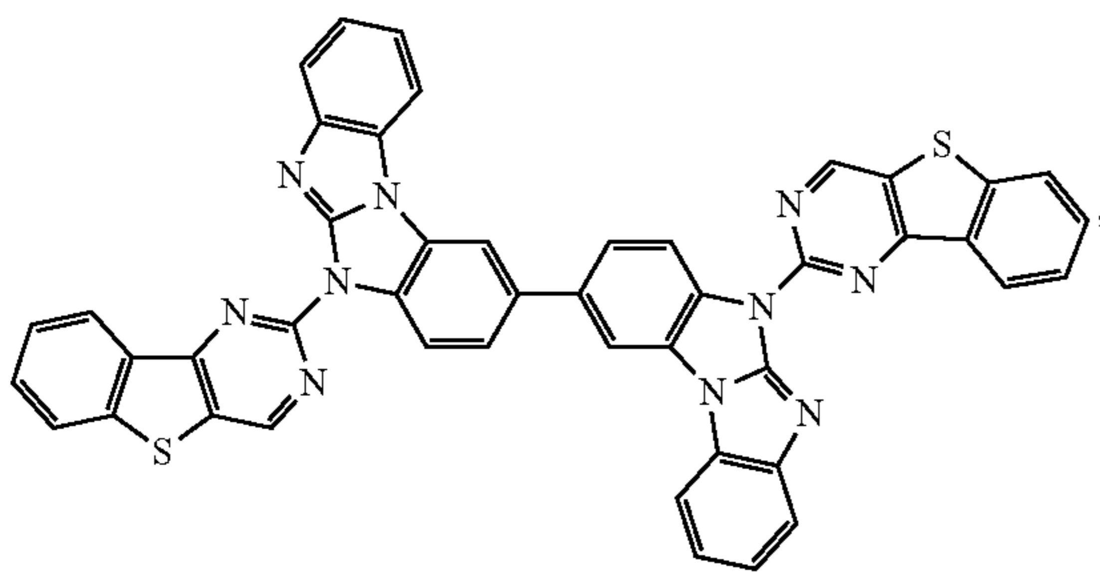
Compound 32
