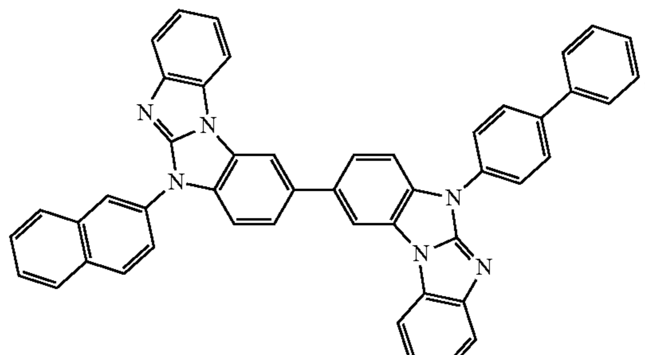
Compound 54
