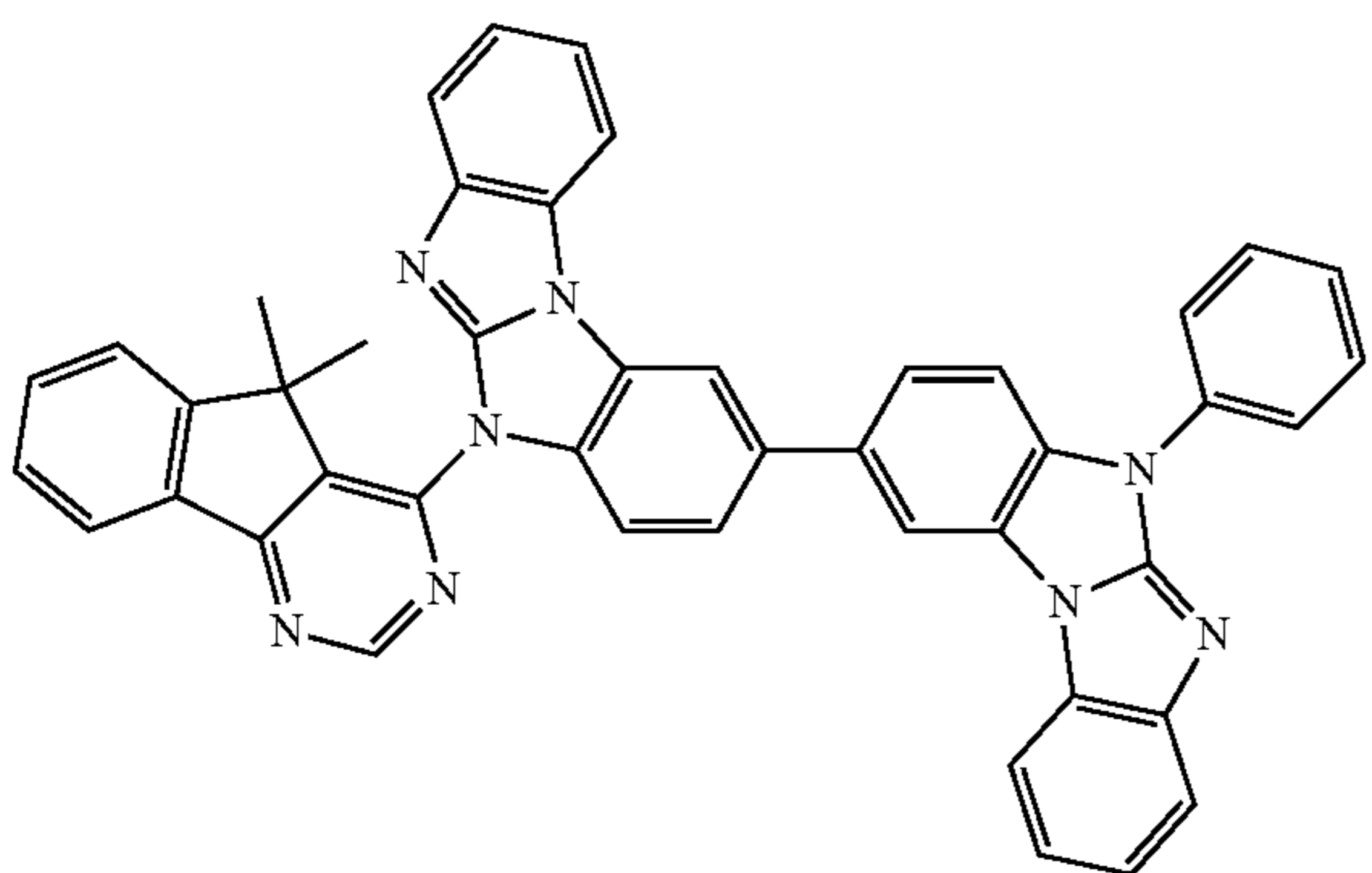
Compound 135
