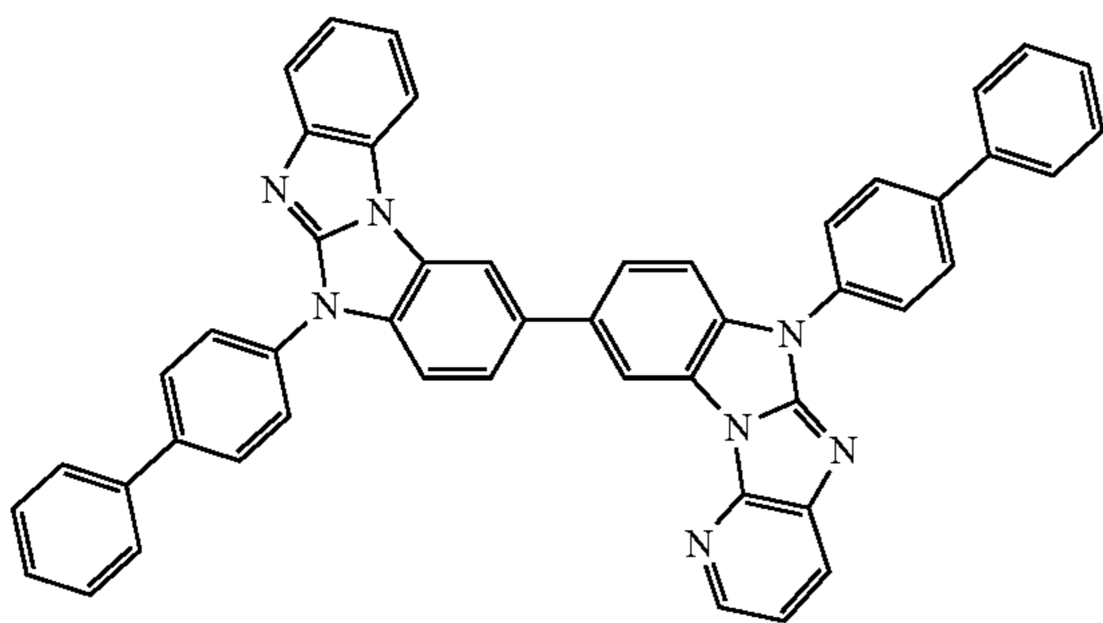
Compound 186
