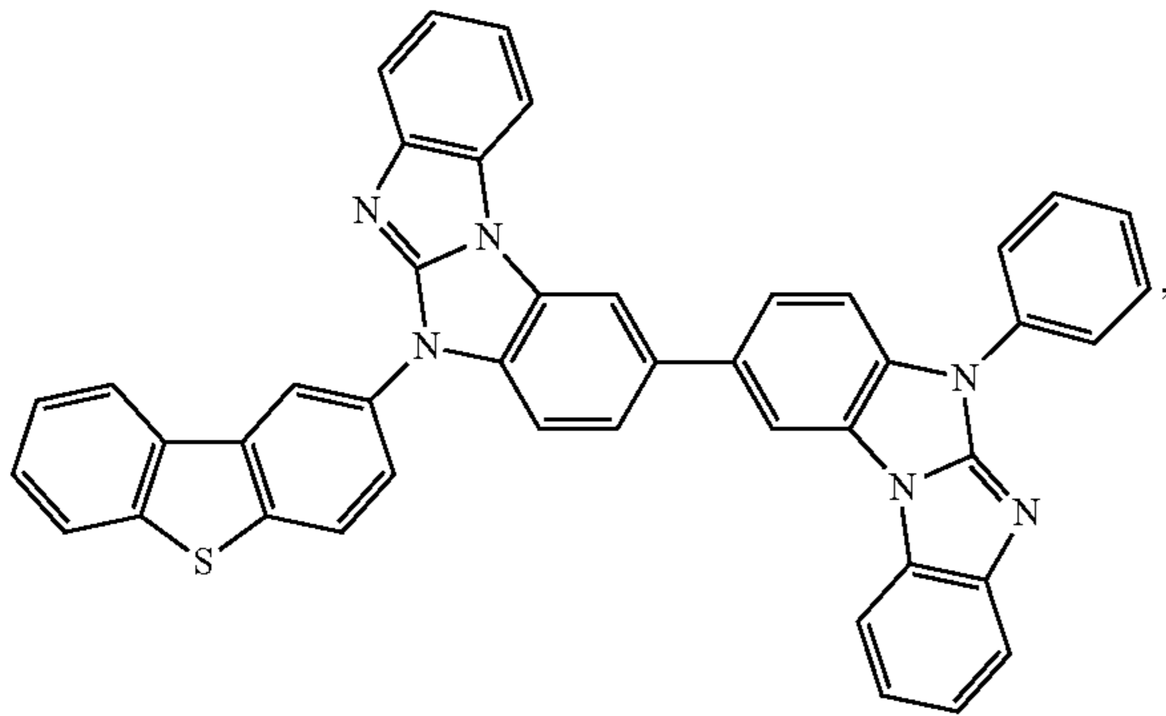
Compound 117
