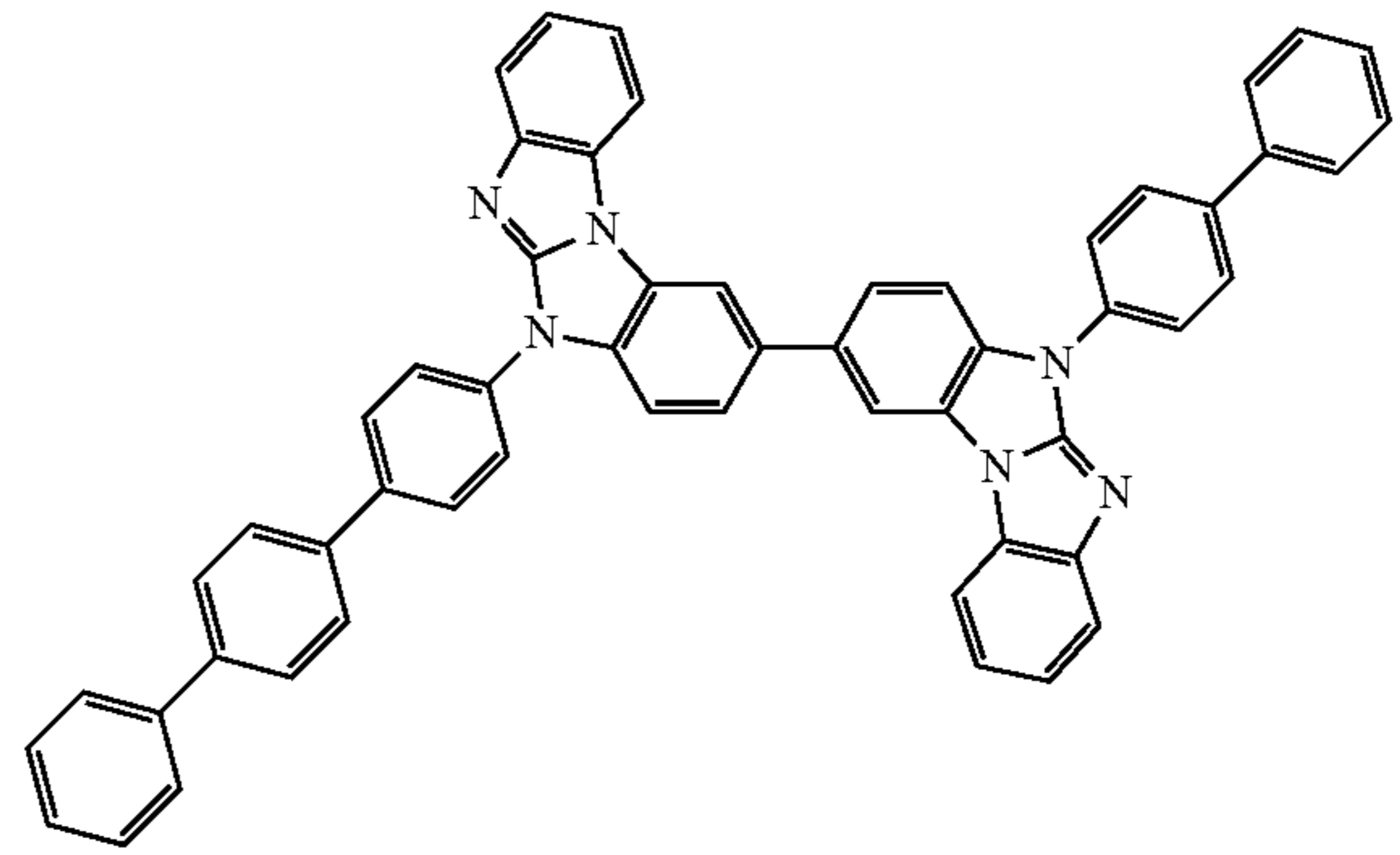
Compound 41
