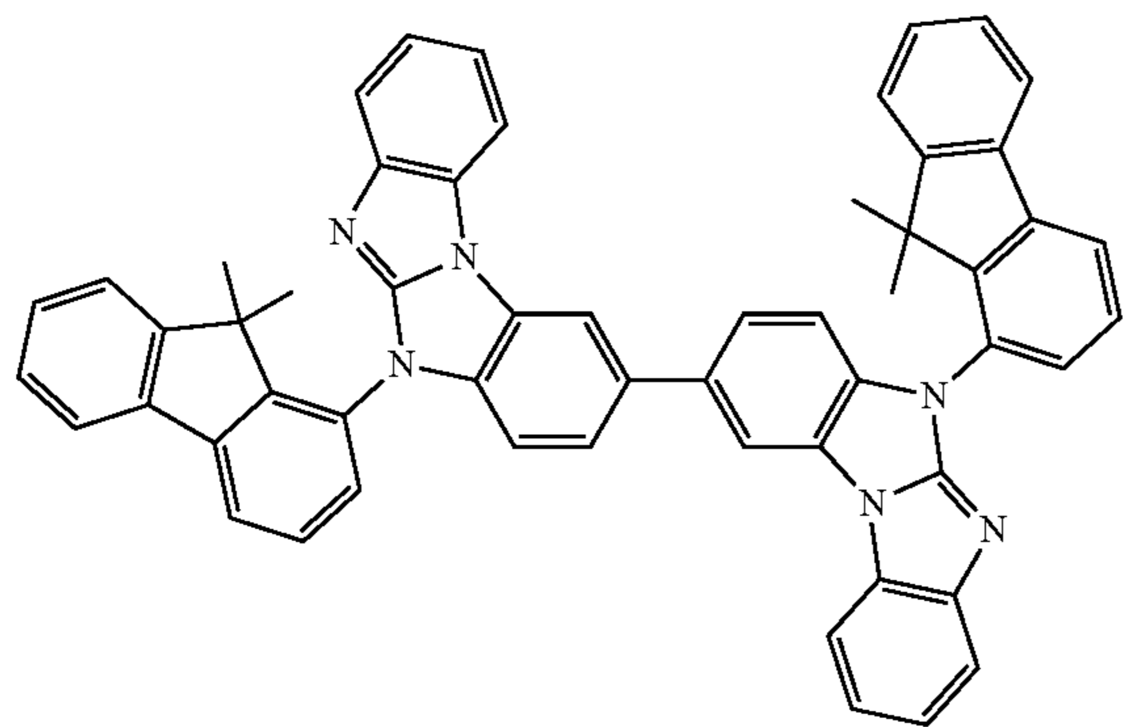
Compound 13
