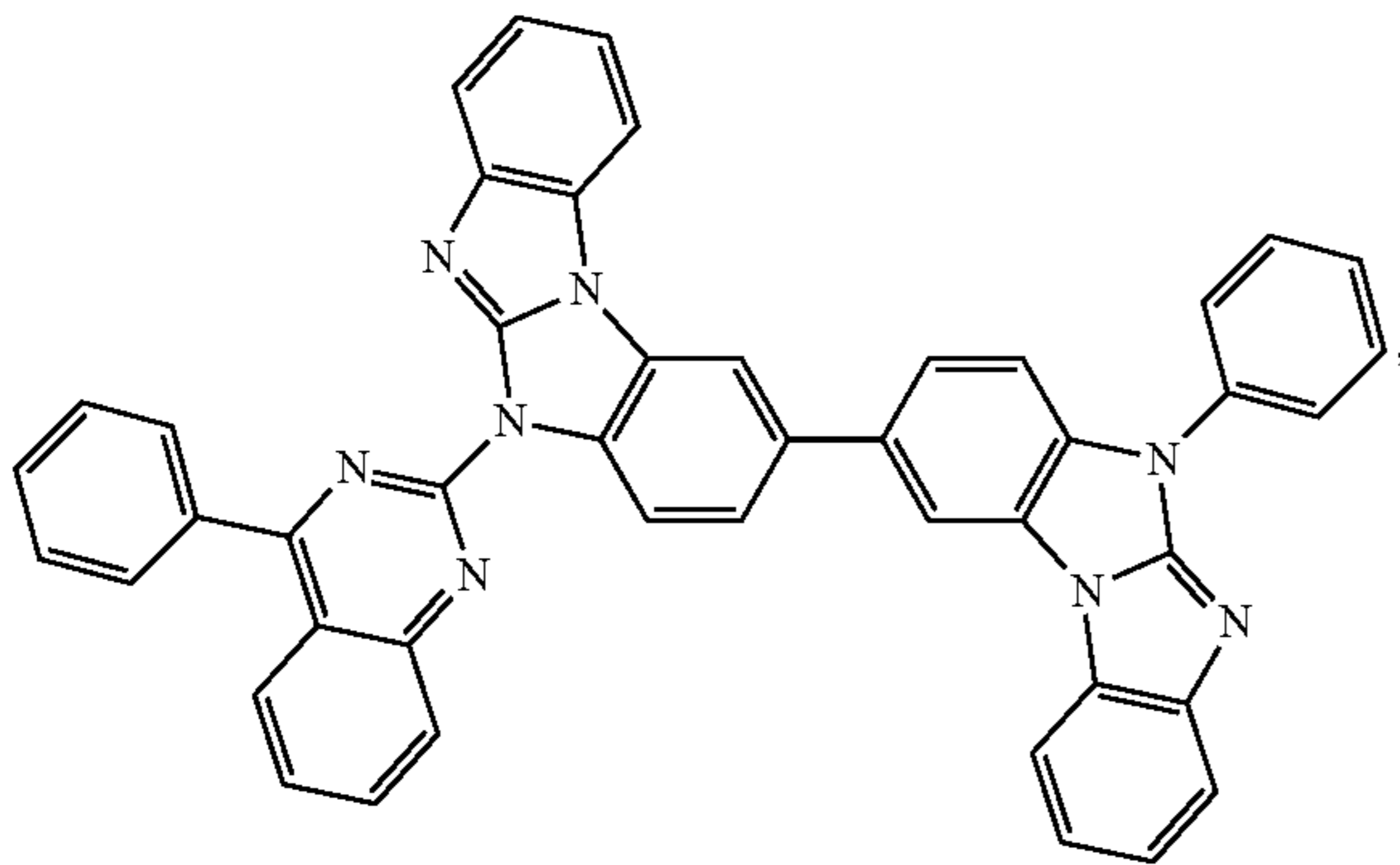
Compound 143
