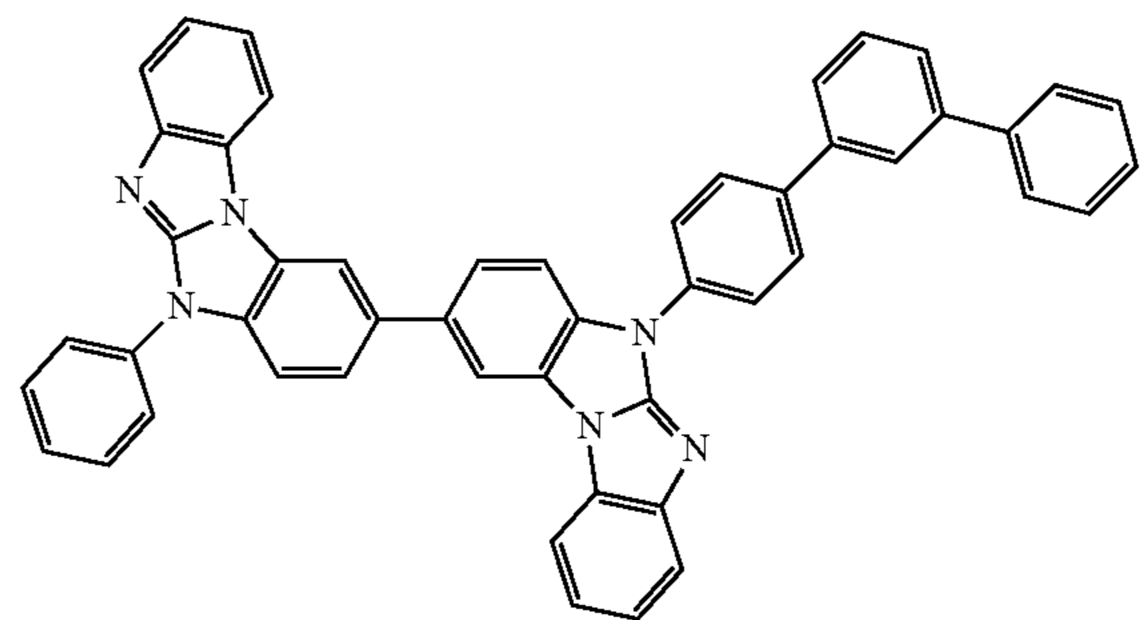
Compound 74
