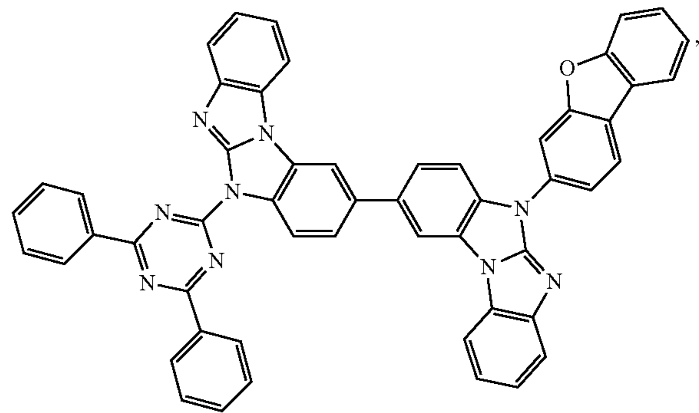
Compound 144
