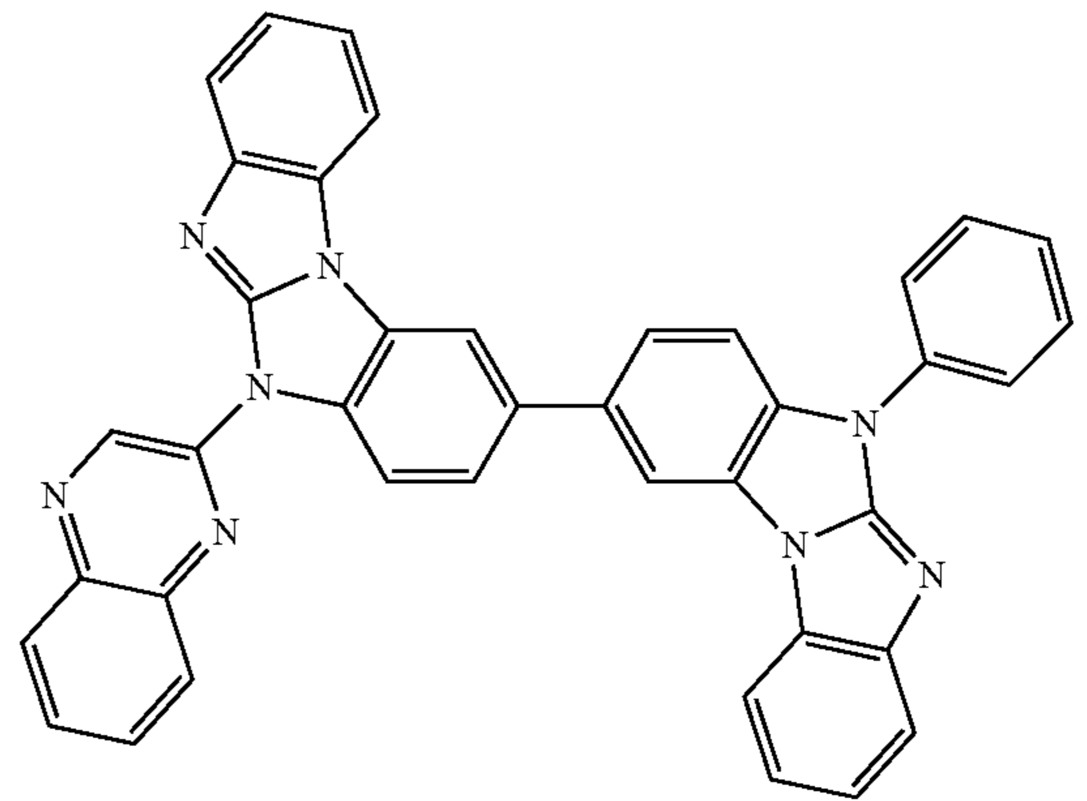
Compound 142
