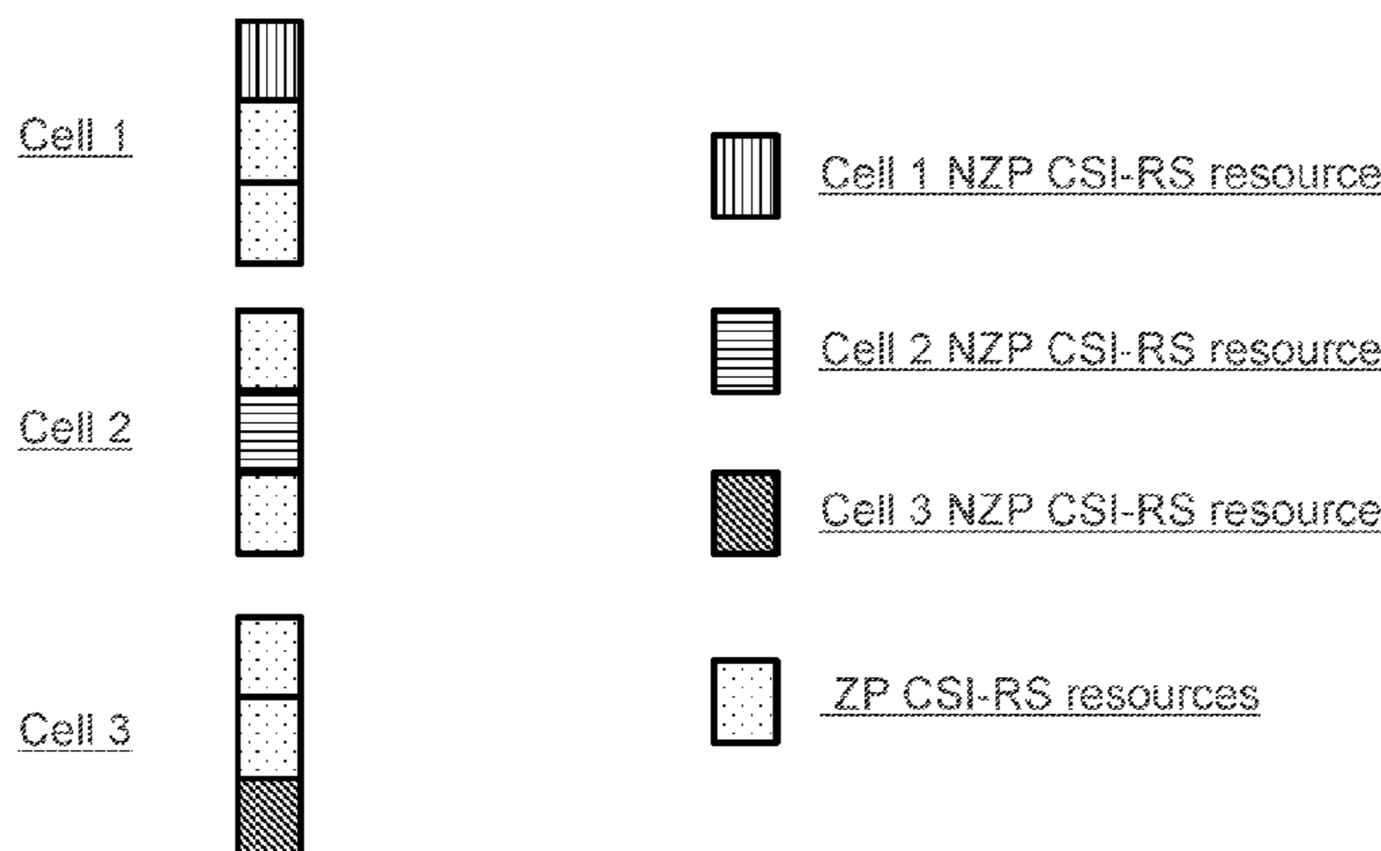
CSI-RS resources
