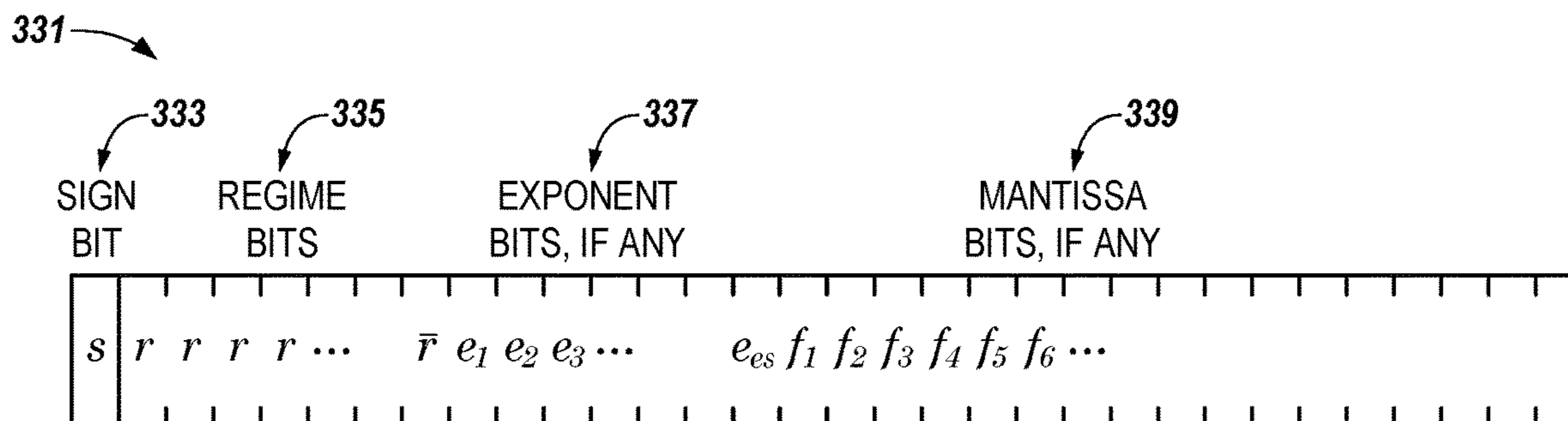
FIG. 3 (PRIOR ART)
