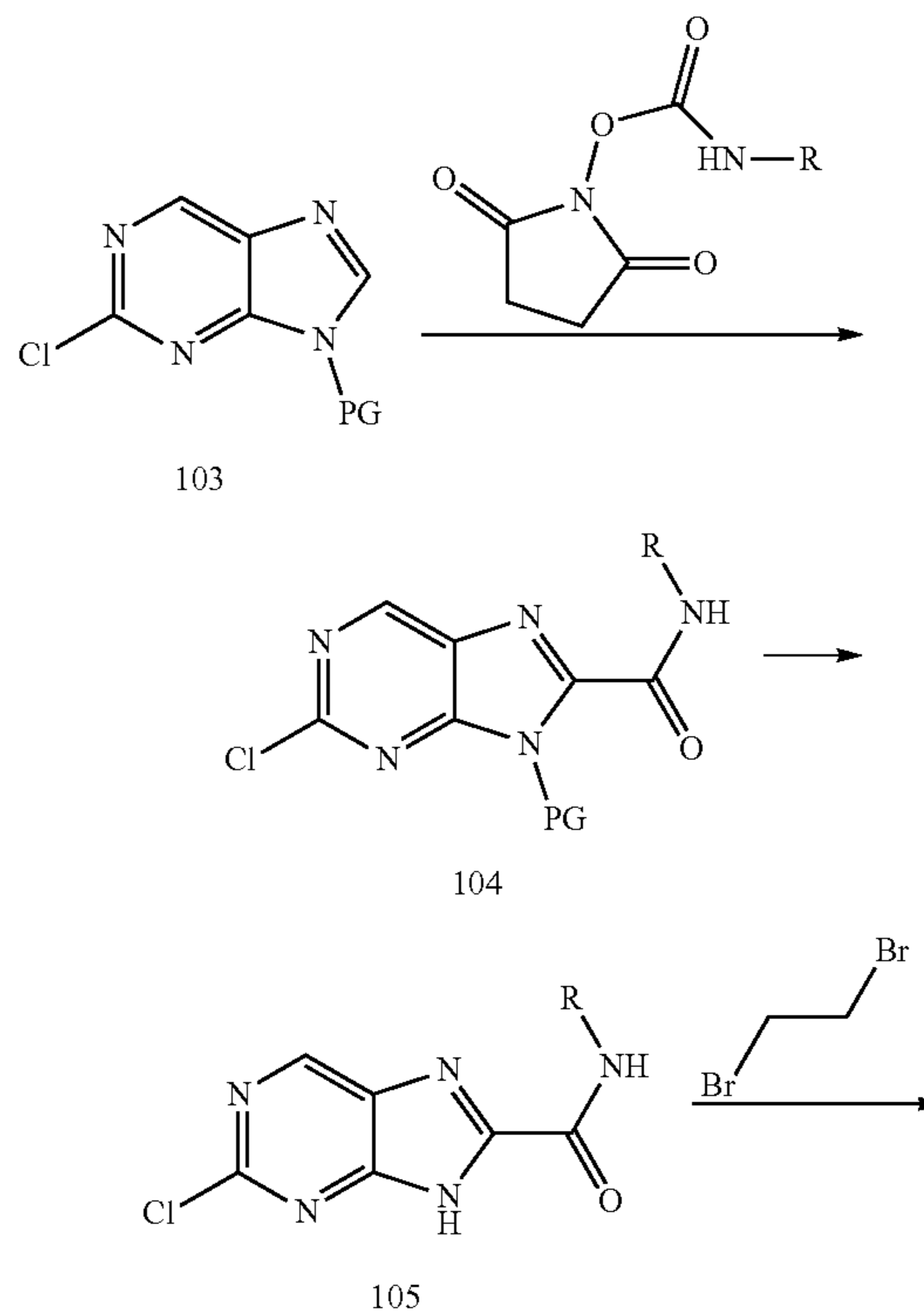
Scheme 14
