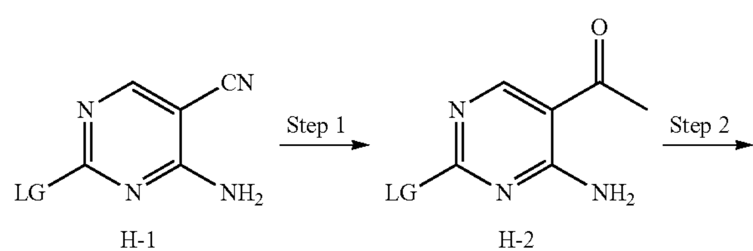
Scheme 1H
