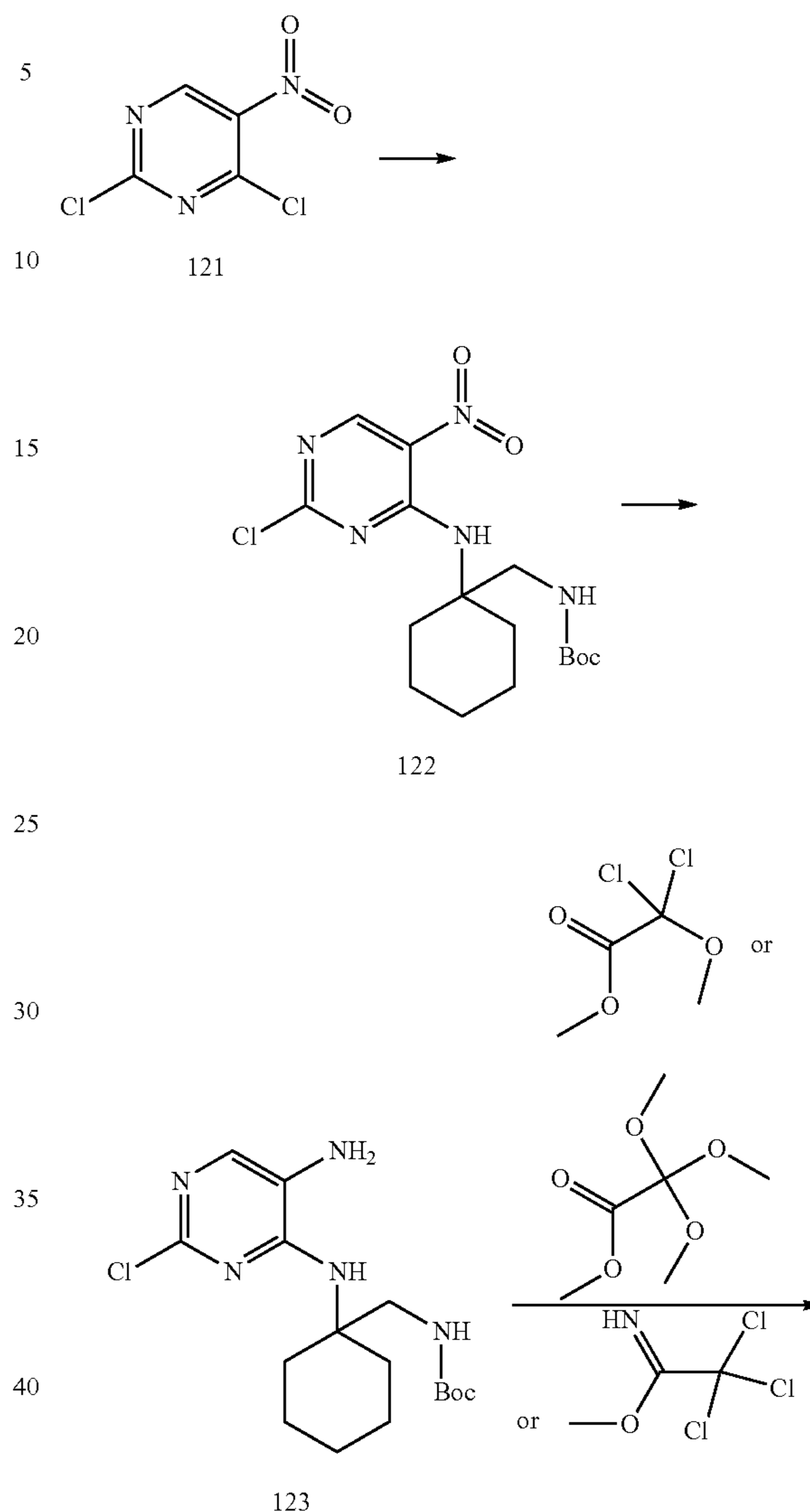
Scheme 18
