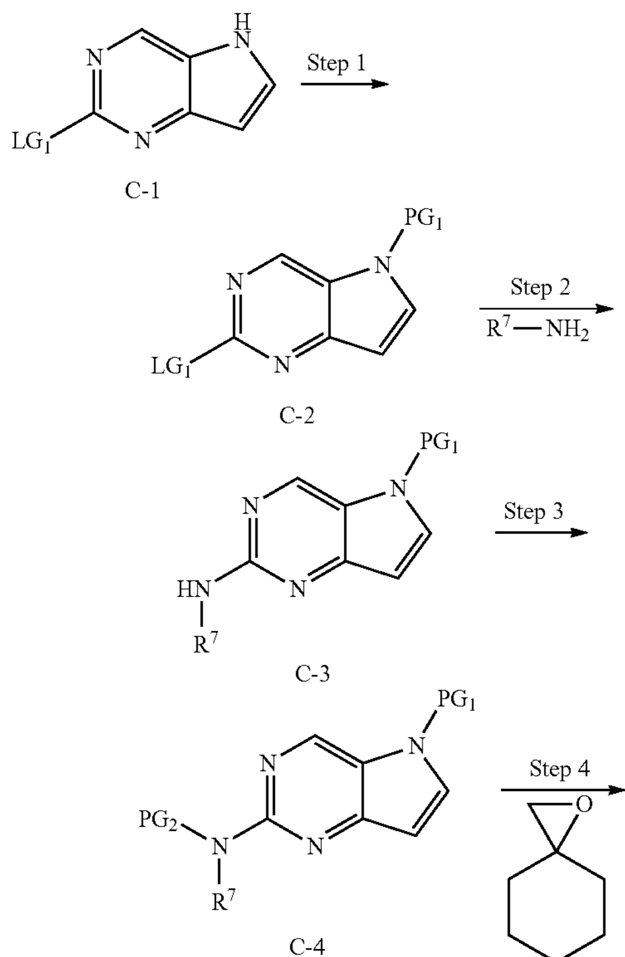
Scheme 1C
