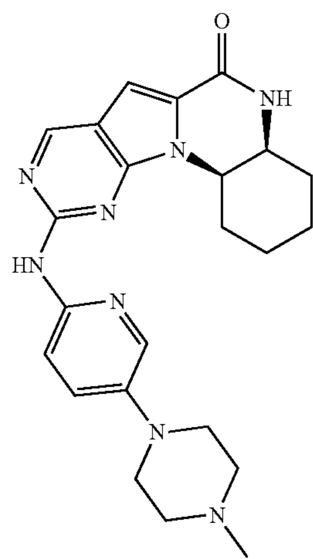
COMPOUND 24
