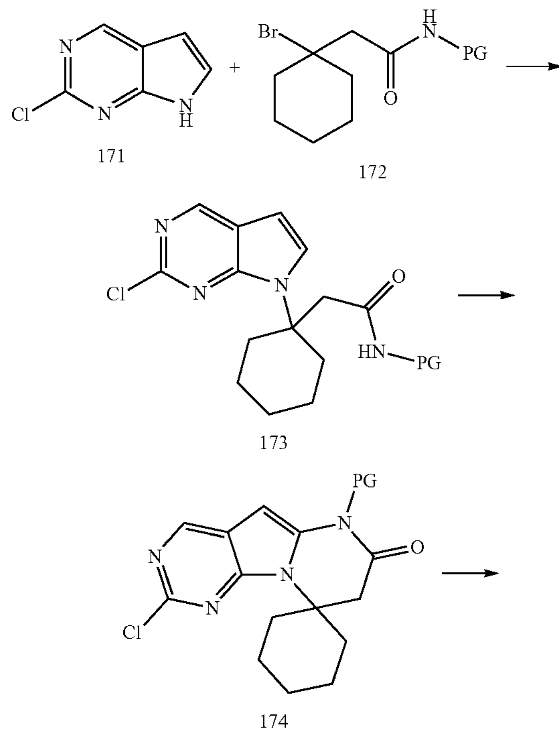
Scheme 23
