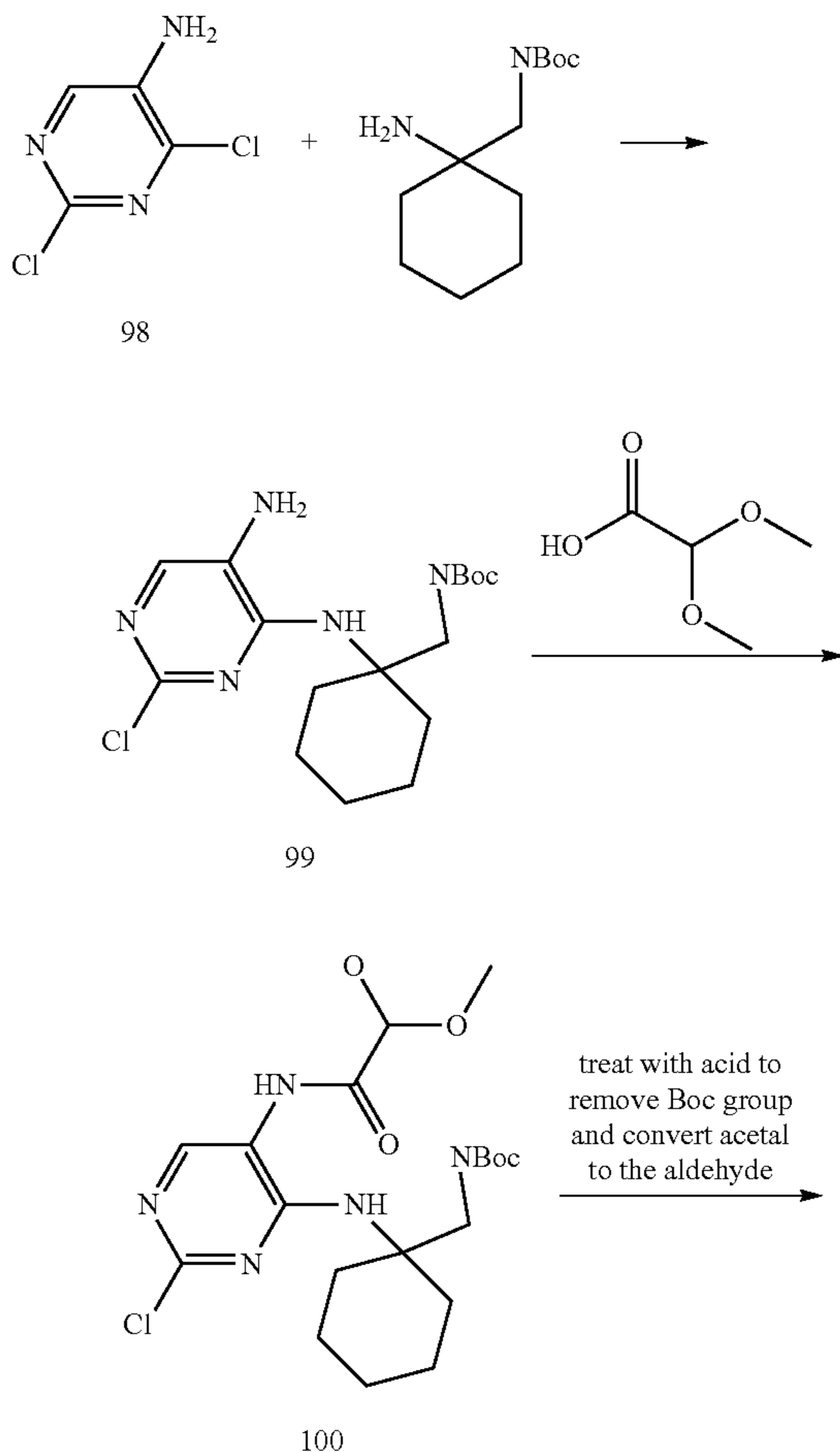
Scheme 13
