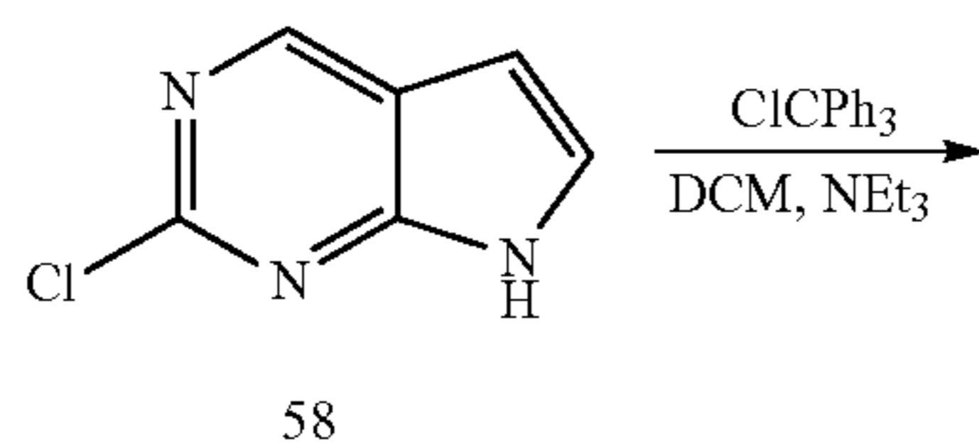
Scheme 8
