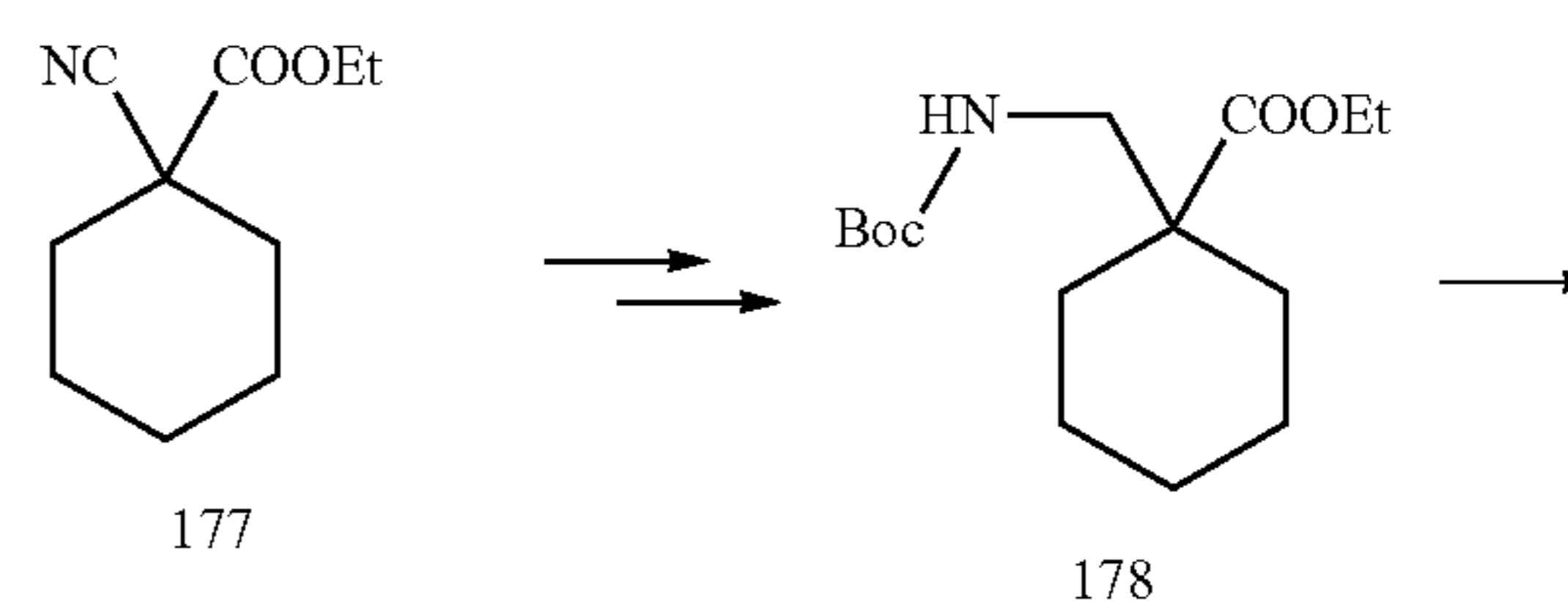
Scheme 24
