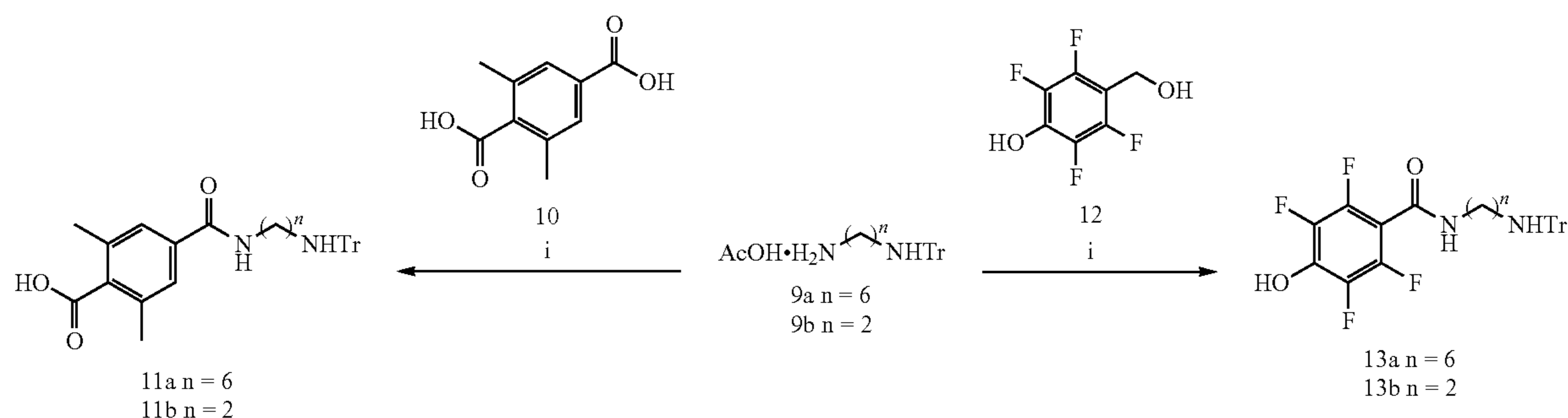
Scheme 1.
