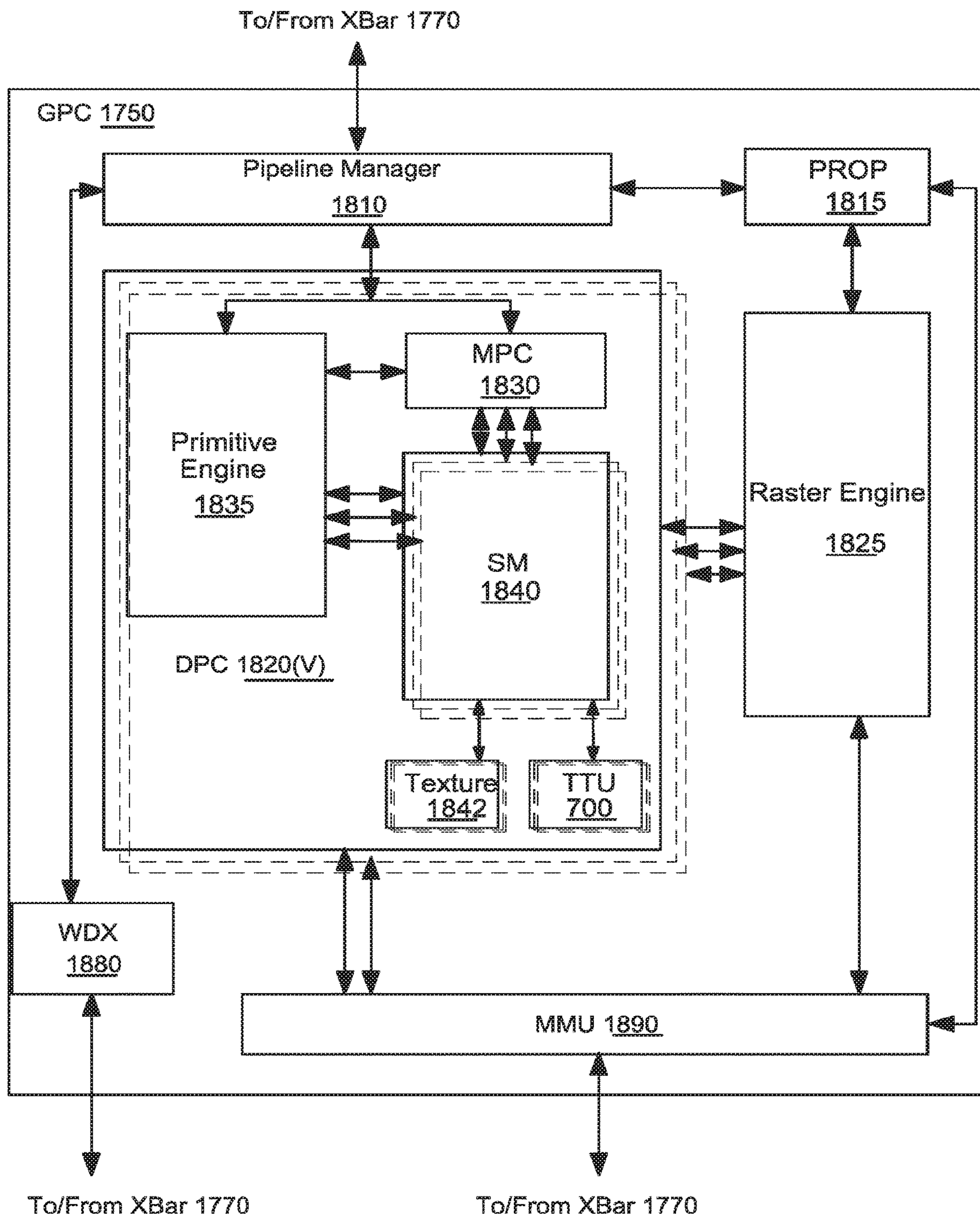
FIG. 17 Example General Processing Cluster
