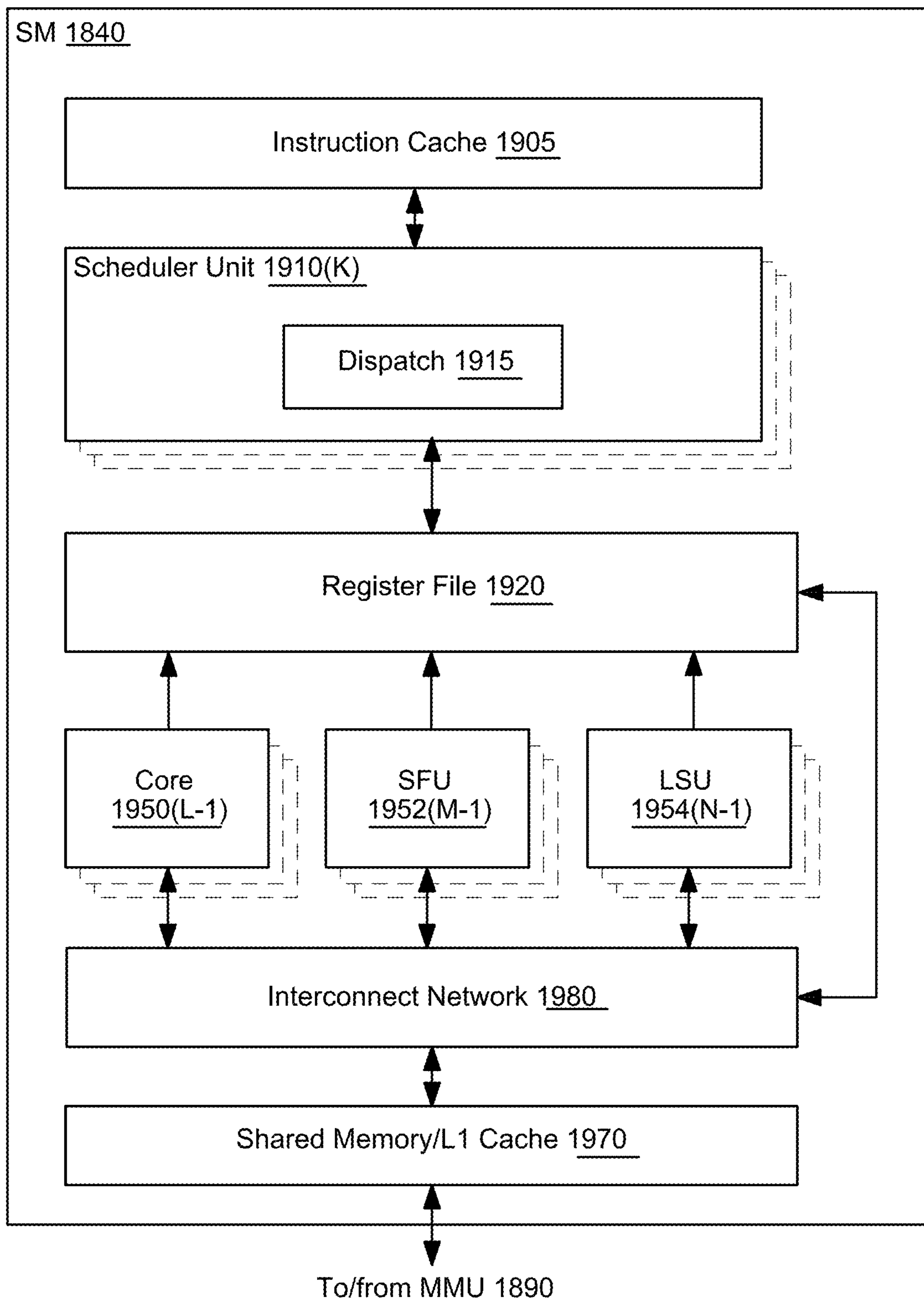
FIG. 22 Example Streaming Multiprocessor
