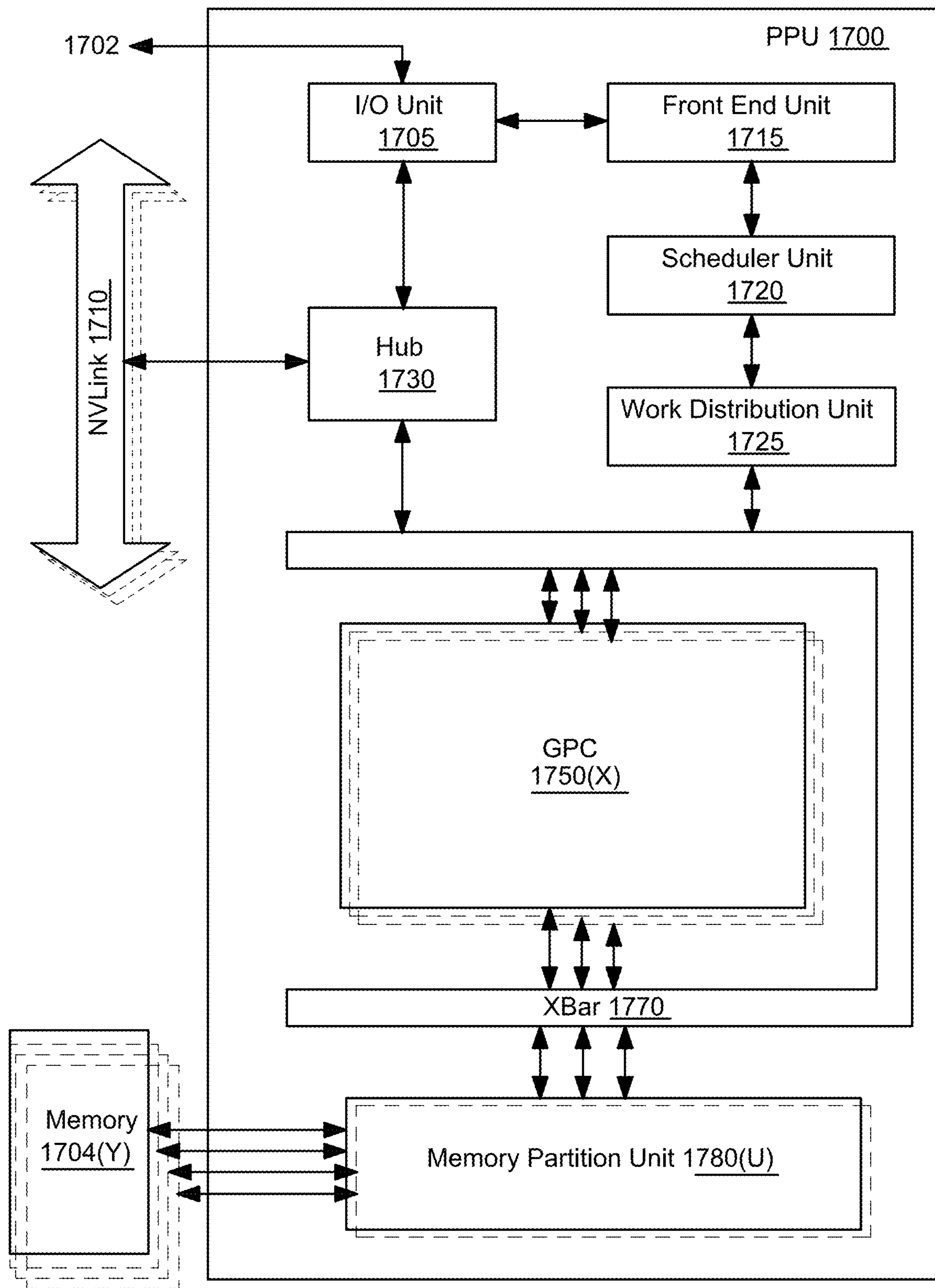
FIG. 18 Example Parallel Processing Unit
